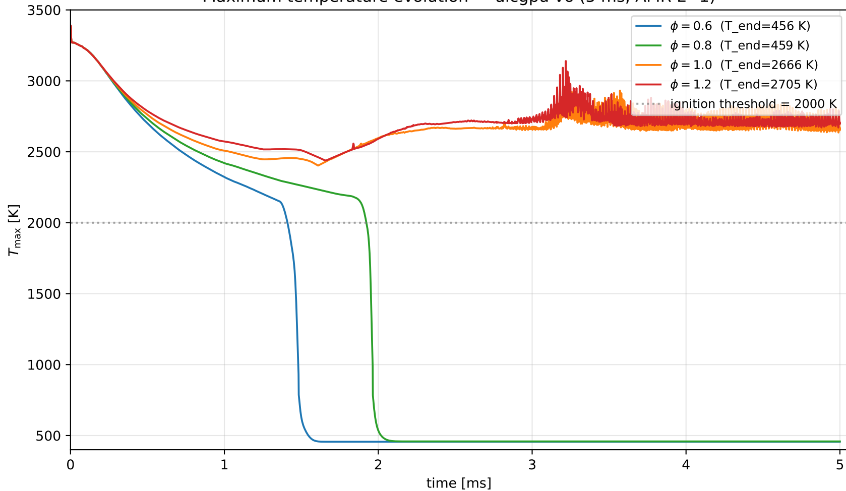
Maximum temperature evolution — uicgpu v6 (5 ms, AMR L=1)
