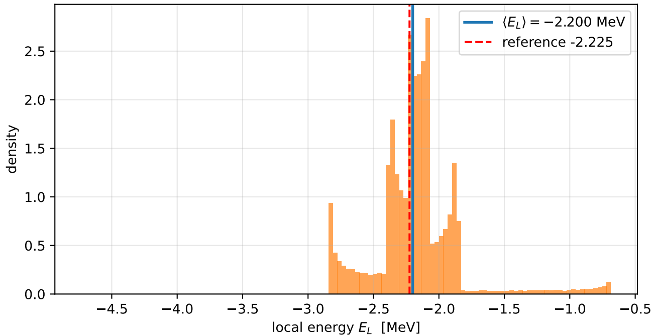
Local-energy distribution (final eval): Deuteron (N=655360)
