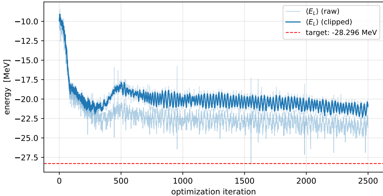
VMC convergence: {}^4\text{He} (Minnesota central, even-state avg)
