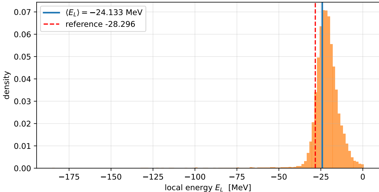
Local-energy distribution (final eval): {}^4\text{He} (N=163840)
