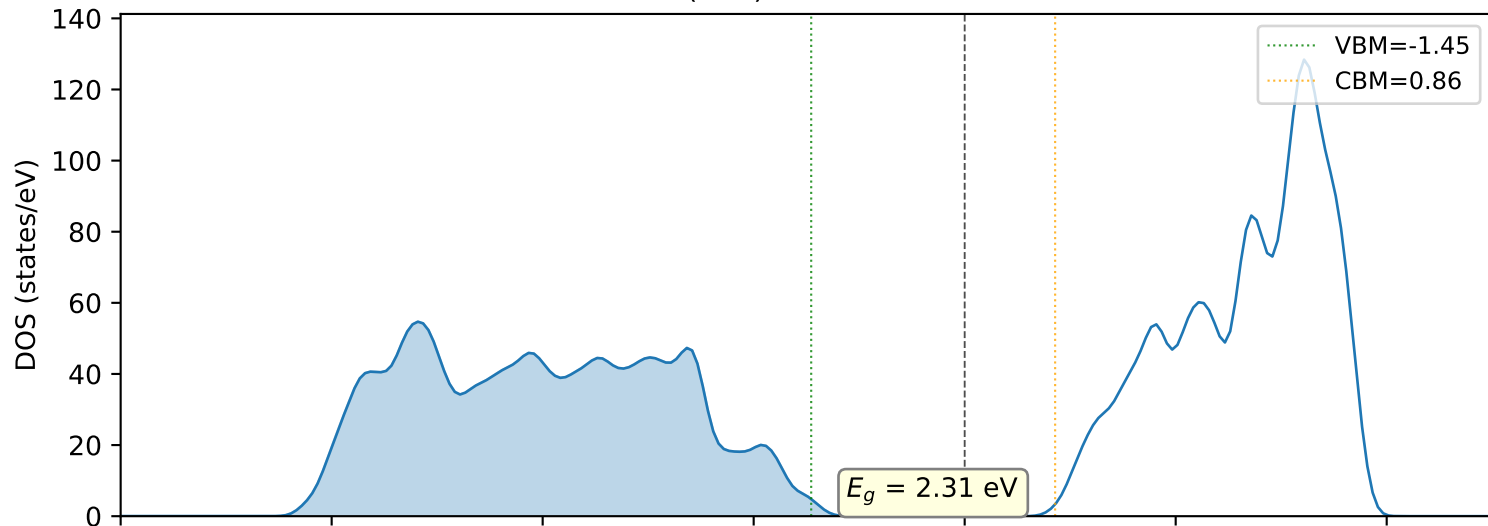
(001) Pt-doped slab
