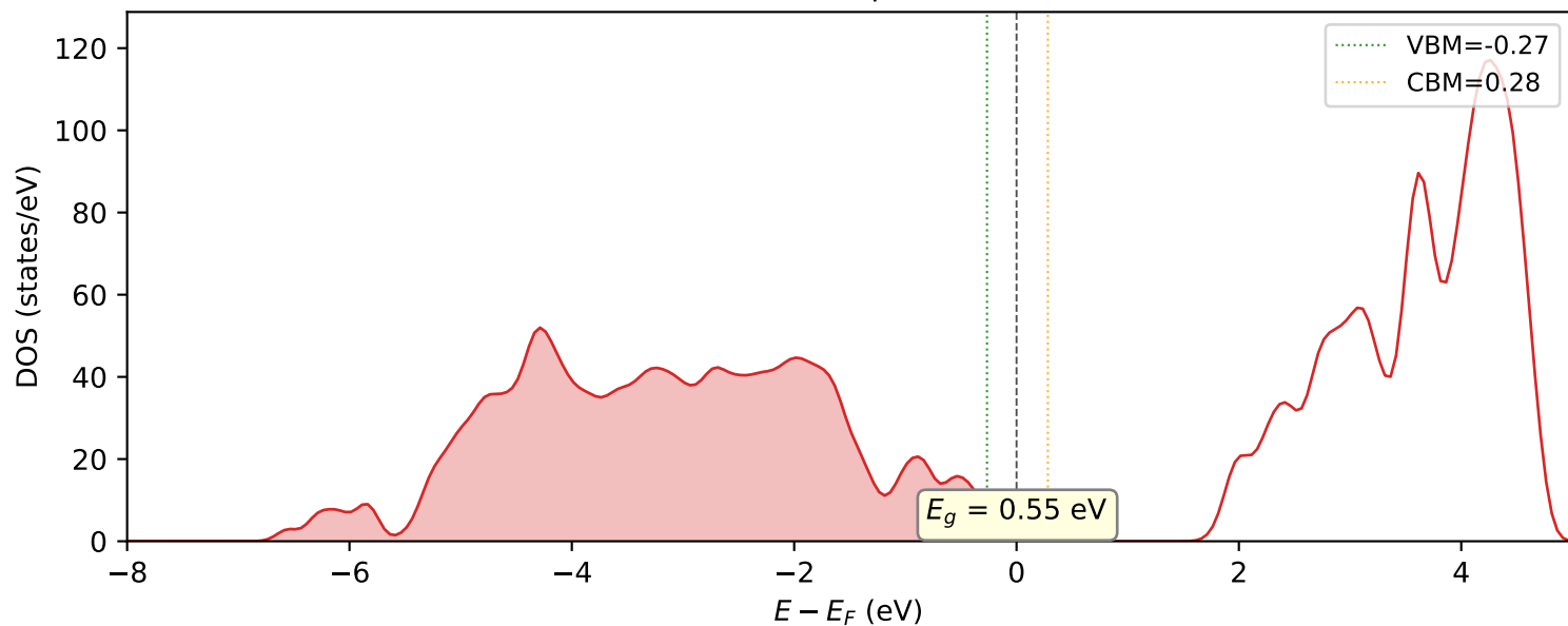
(001) Pt-doped slab
