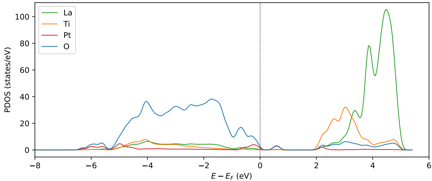
(001) Pt-doped
