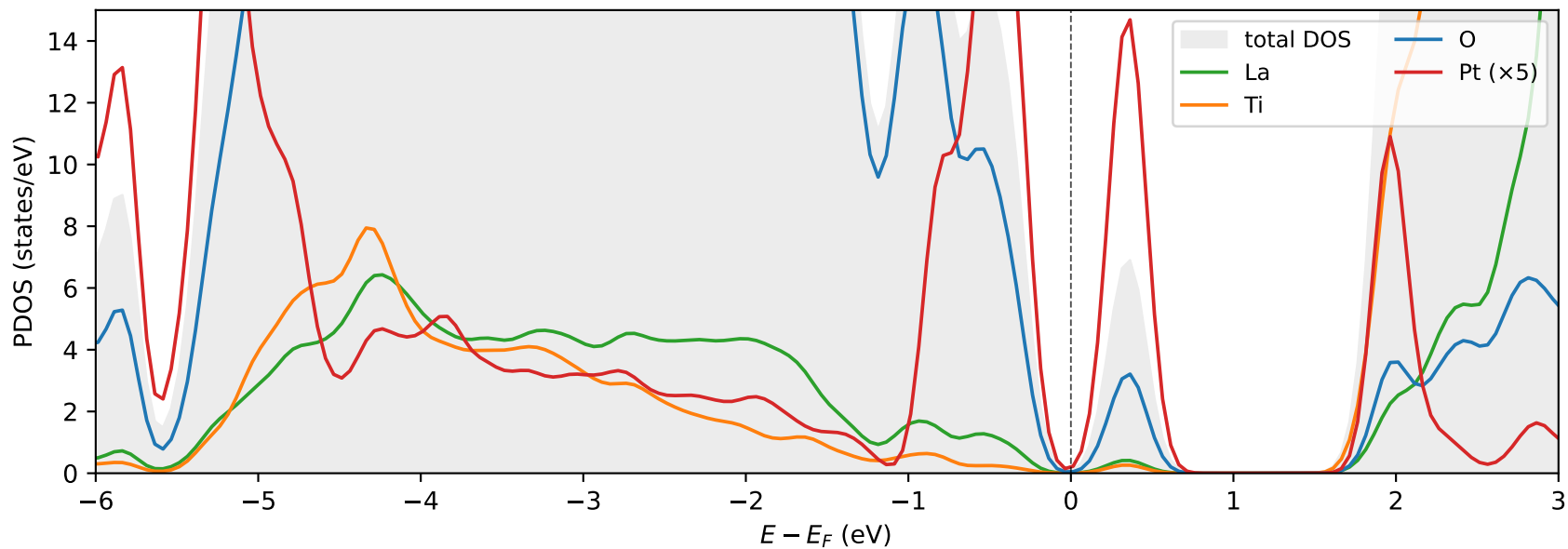
(001) Pt-doped ( \text{Ti} \rightarrow \text{Pt} surface substitution)
