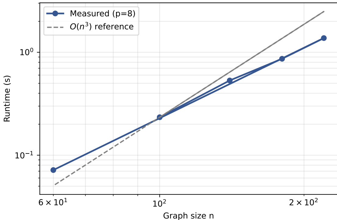
Problem-size scaling — fitted slope = 2.27
