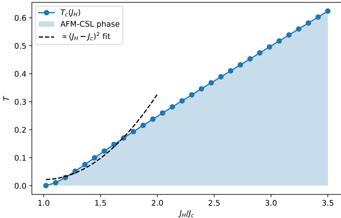
Phase diagram: disordered / AFM-CSL (paper Fig. 3)
