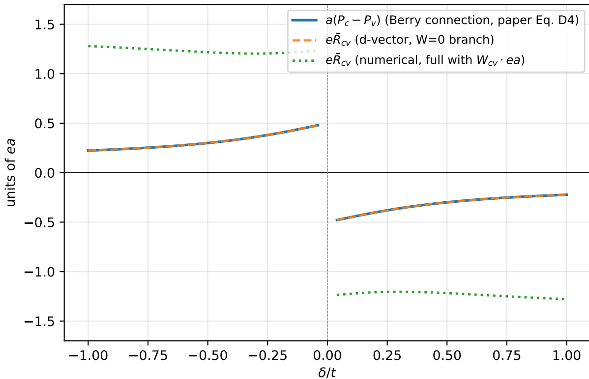
Rice-Mele: Fig. 1(b) replica ( \Delta/t = 0.5 , N_k = 4001 )
