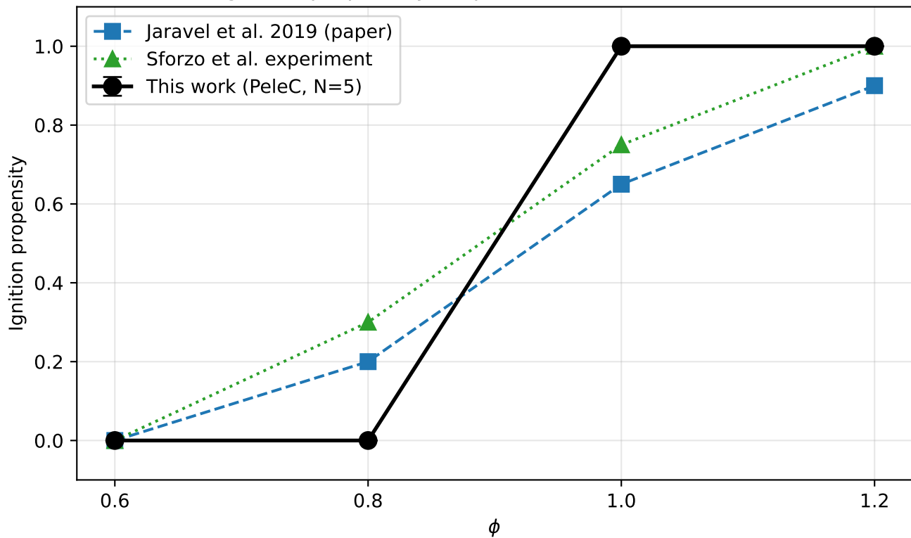
Ignition propensity vs \phi (ours: T(1\text{ ms}) > 2525\text{ K} )
