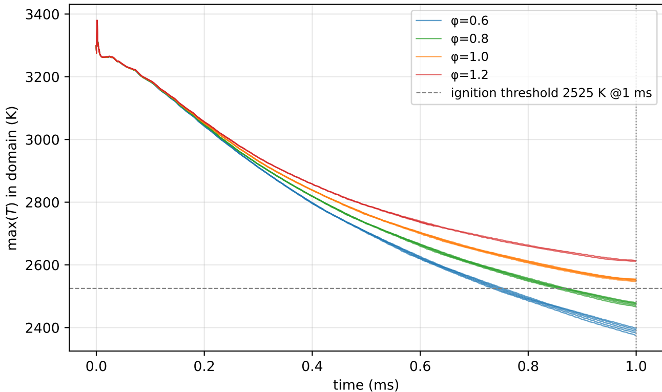
Ensemble T_{max}(t) — 4 \phi \times 5 realizations (Polaris, PeleC)
