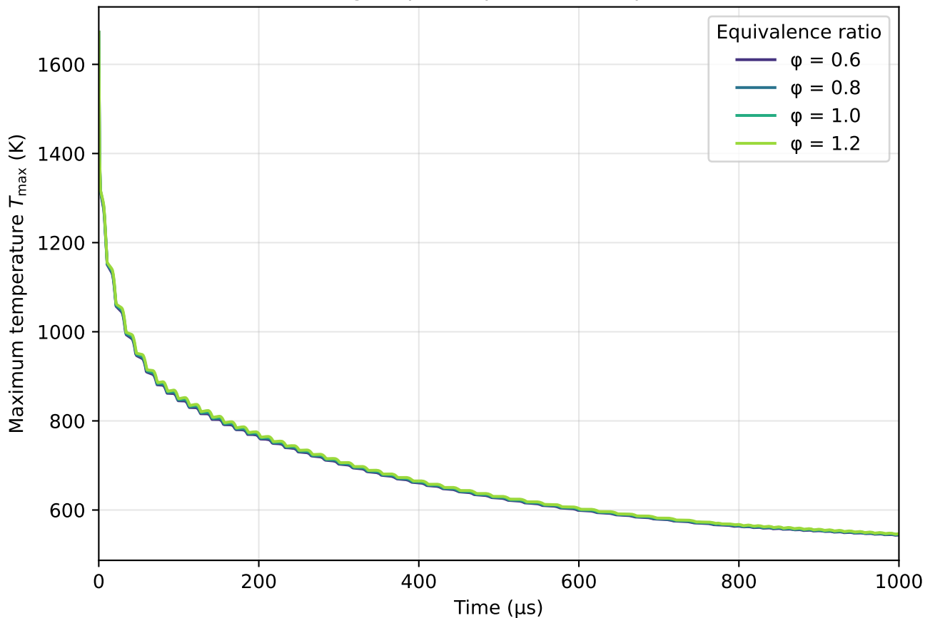
Kernel cooling: 4- \phi sweep (PeleC compressible LES)
