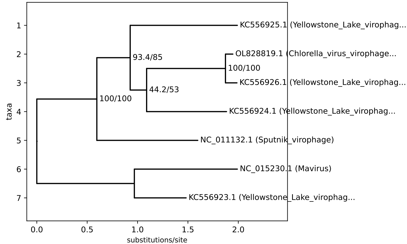
PRO — Maturation Protease
