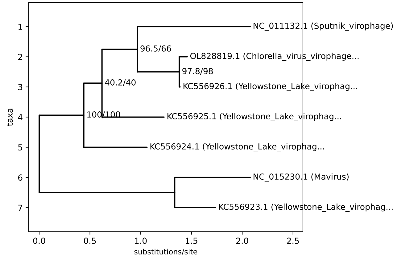
Penton — Minor Capsid (Penton)
