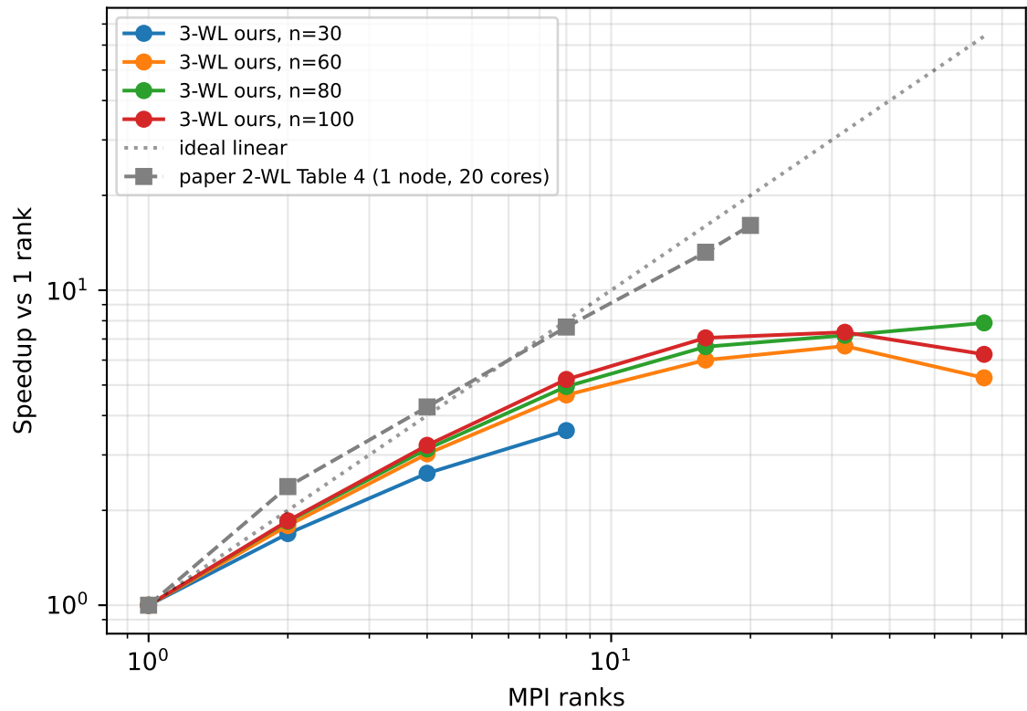
Strong-scaling speedup
