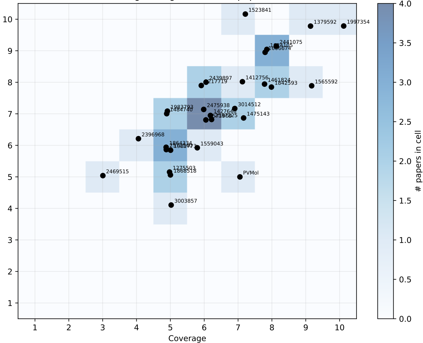
Coverage vs Agreement (30 papers)
