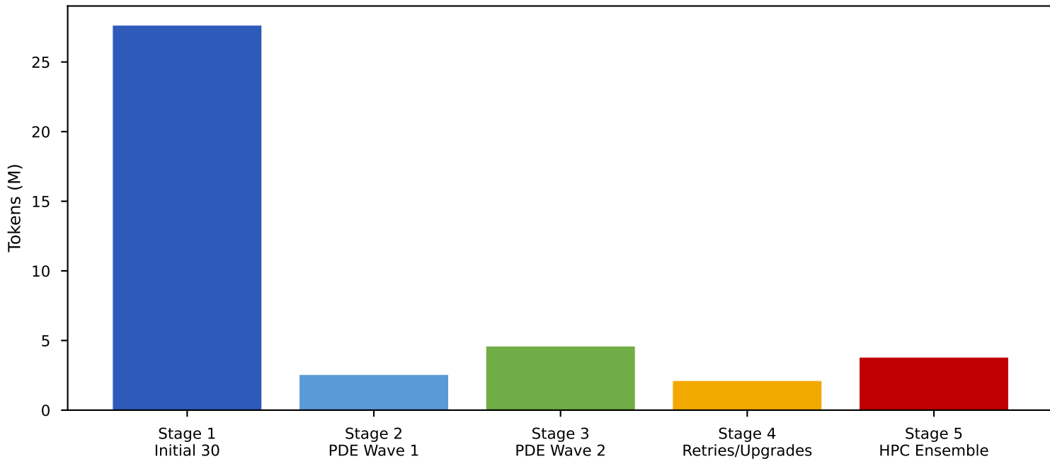
Token usage by stage — total 40.7 M tokens
