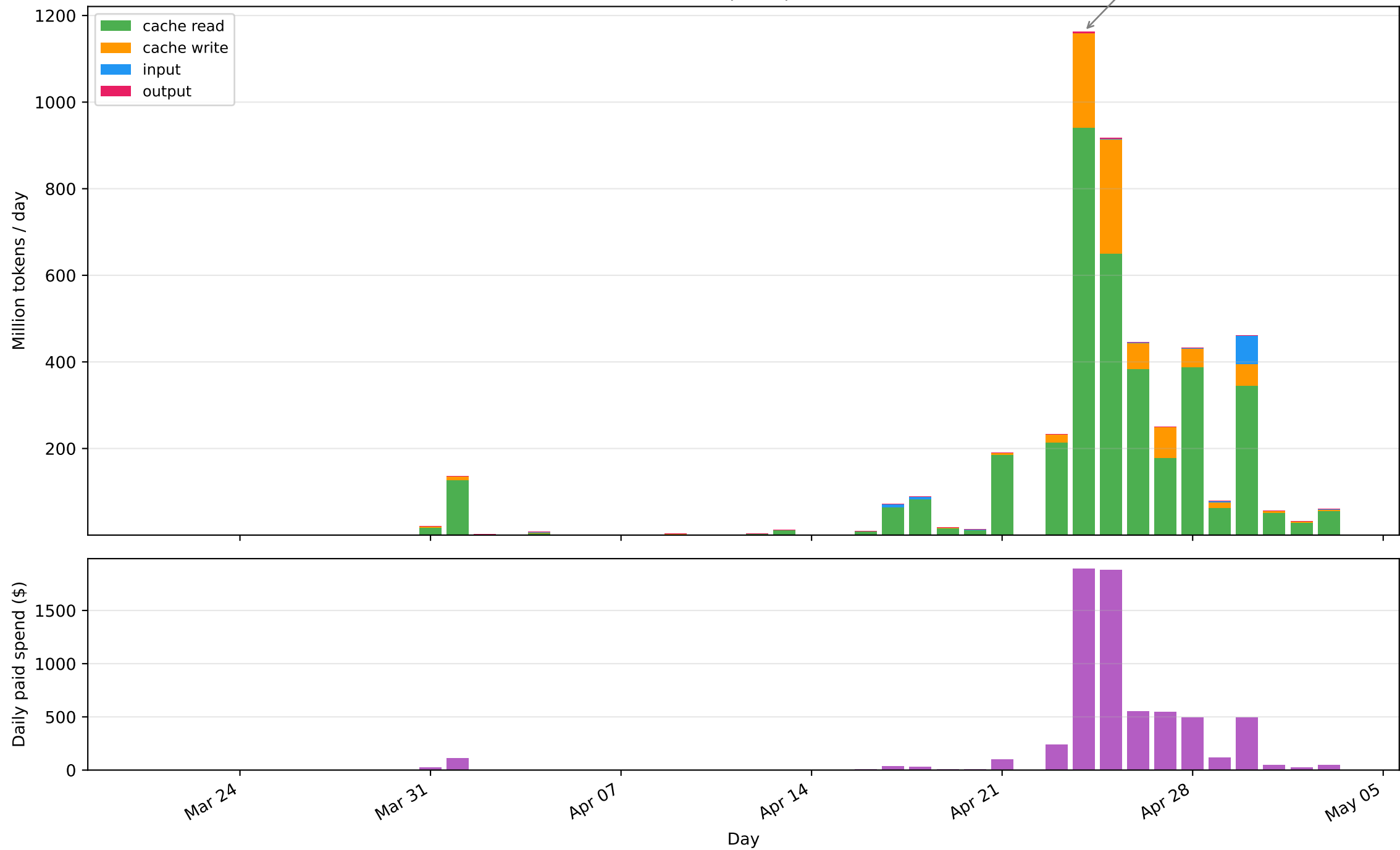
OpenClaw token usage by day — 2026-03-21 to 2026-05-03 total: 4.71B tokens / $6,720 paid spend across 725 sessions
