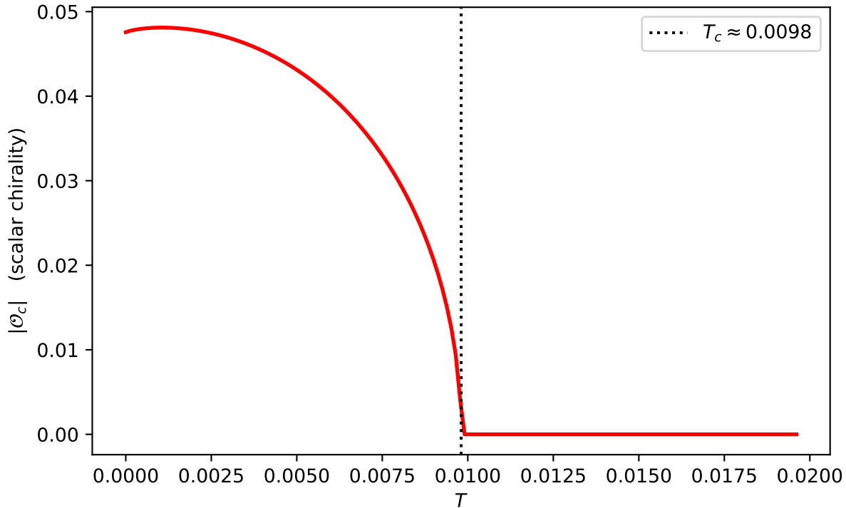
Scalar spin chirality vs T at J_H = 1.1J_c
