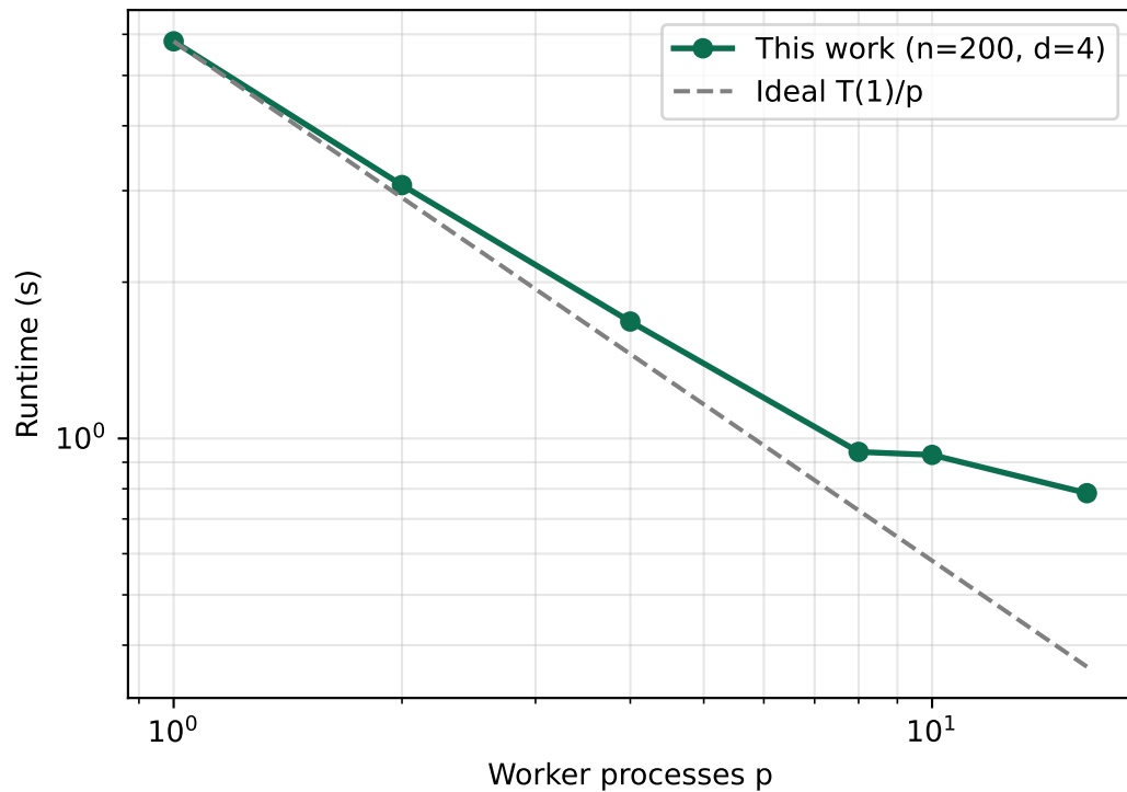
Strong scaling — runtime
