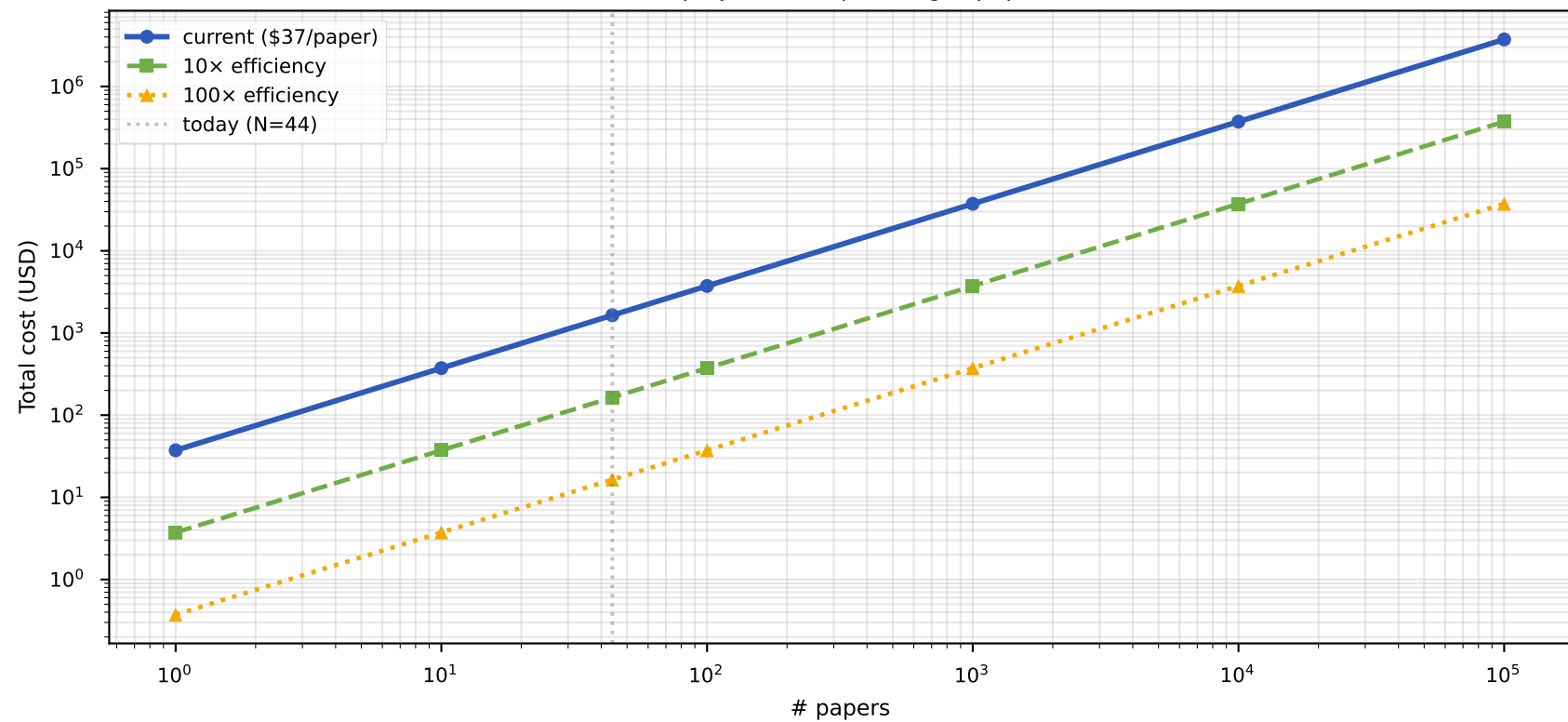
Cost projection: replicating N papers
