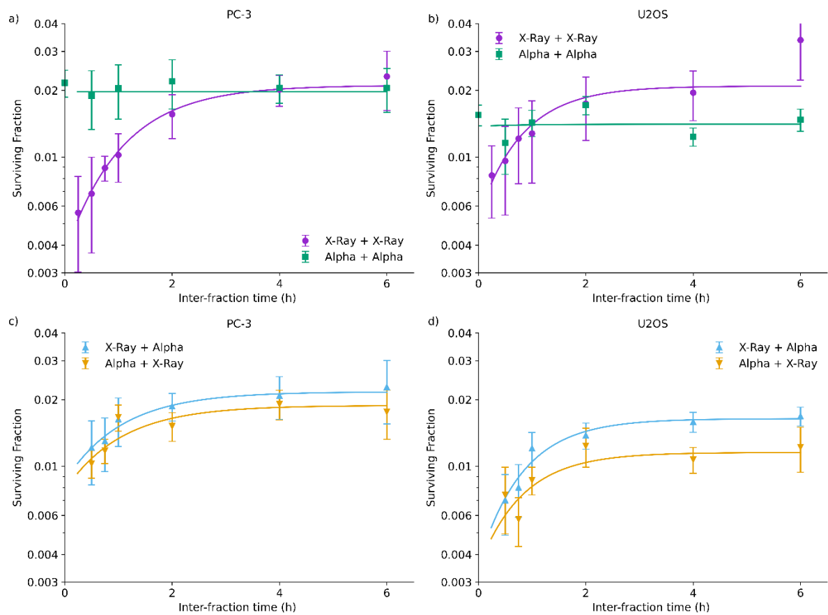
Figure S 1 Sublethal damage repair curves for PC-3 (left) and U2OS (right) cells following exposure to two identical fractions (3 Gy X-rays or 0.75 Gy alpha particles, top) or mixed exposures (bottom), as in Figure 3. Here, instead of a different repair rate for each exposure and cell line, only a single repair rate is fit for all irradiations in each cell line. This can be seen to remain in good agreement with the data, and is not statistically significantly different to the independent repair models presented in Figure 3.
