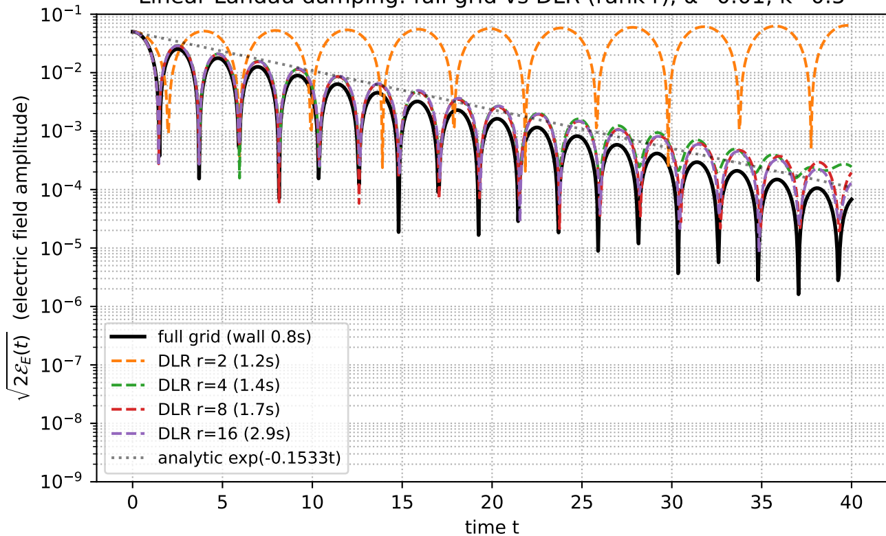
Linear Landau damping: full grid vs DLR (rank r), \alpha=0.01 , k=0.5
