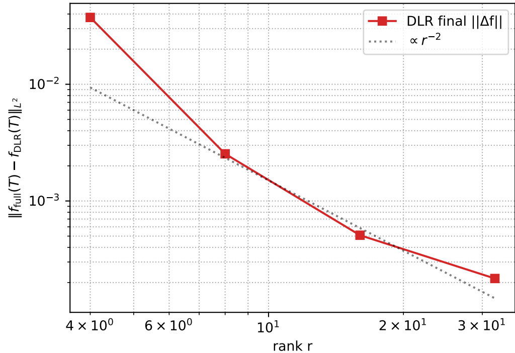
Two-stream: distribution error vs rank
