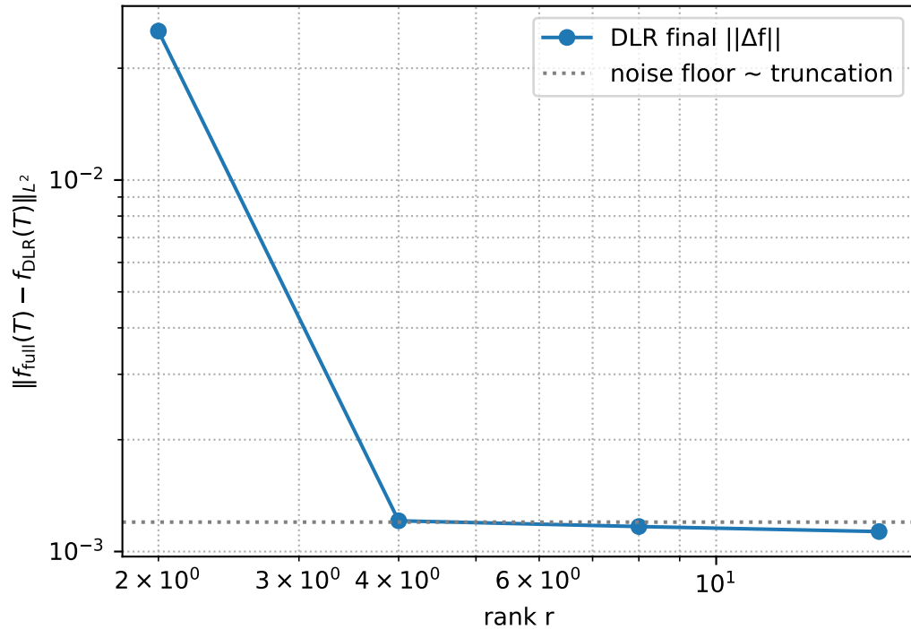
Landau: distribution error vs rank
