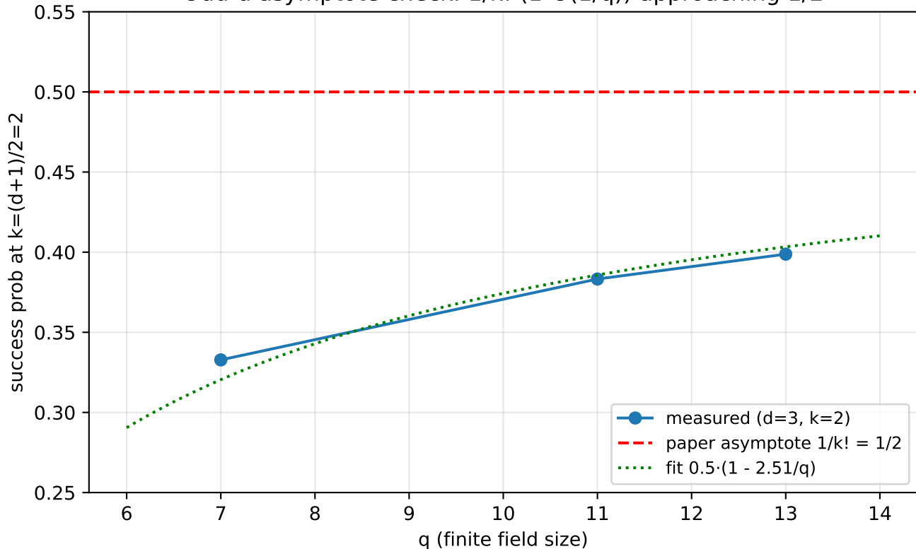
Odd-d asymptote check: 1/k! \cdot (1 - O(1/q)) approaching 1/2
