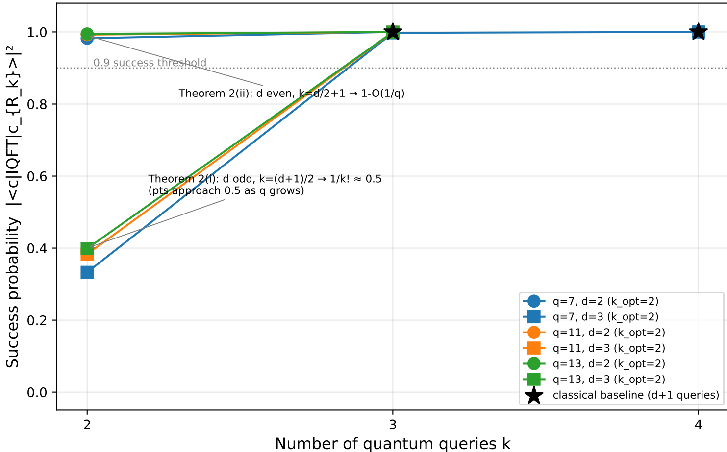
Childs-van Dam-Hung-Shparlinski (arXiv:1509.09271): Quantum polynomial interpolation over F_q , real numpy statevector
