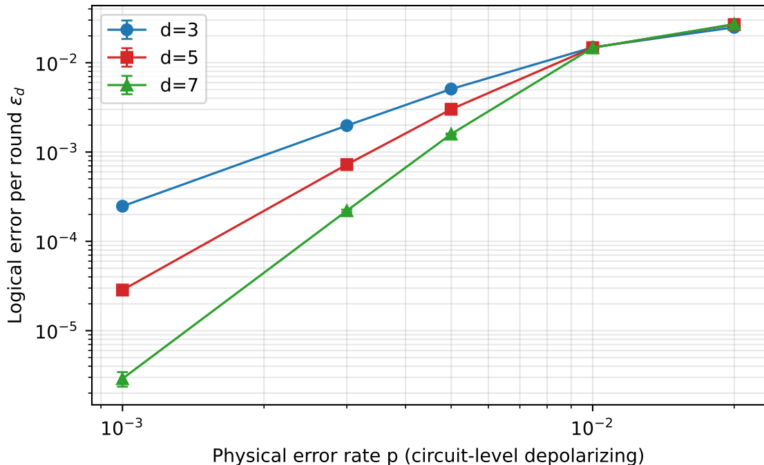
Surface code memory: logical error per round vs p Replication of Google arXiv:2207.06431 (Stim + PyMatching)
