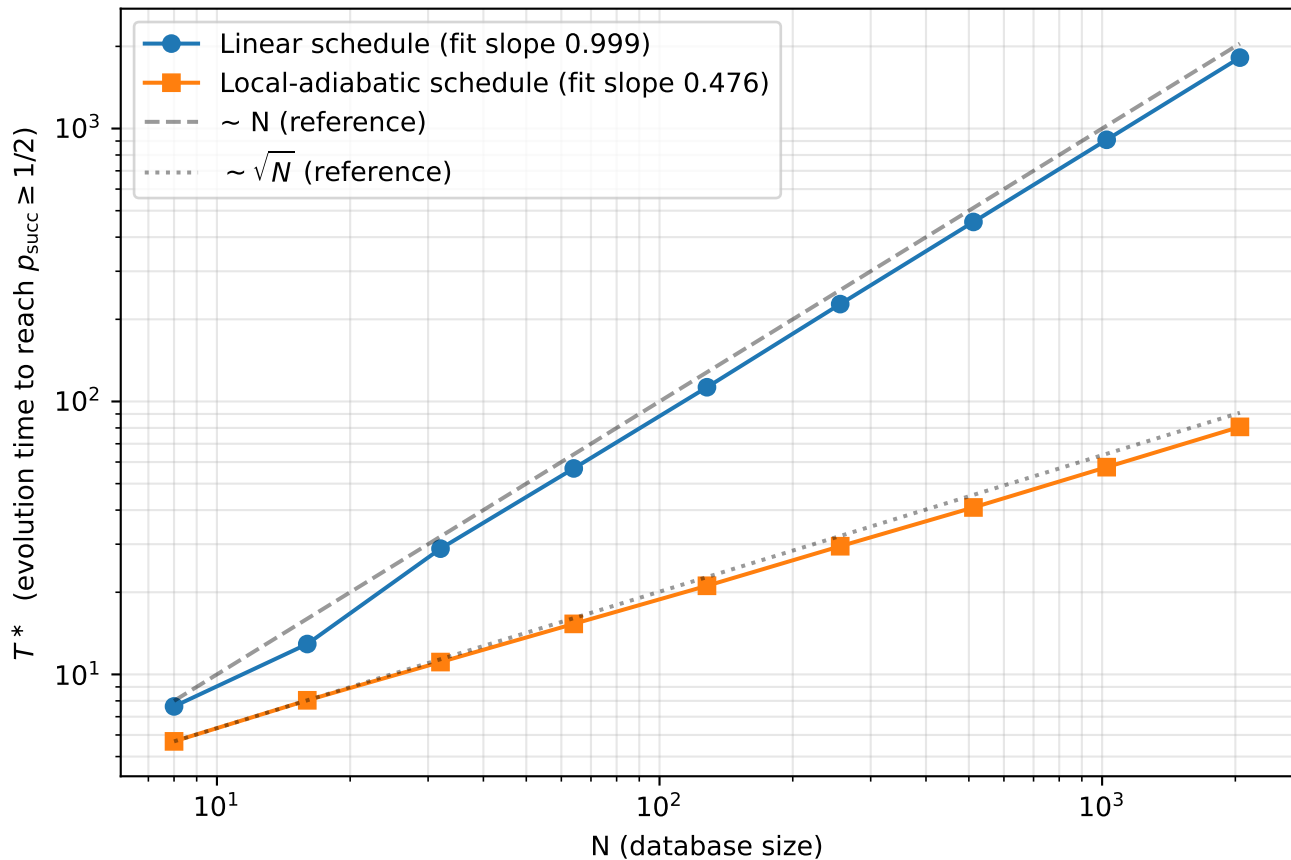
Roland-Cerf (2001) replication: adiabatic Grover scaling
