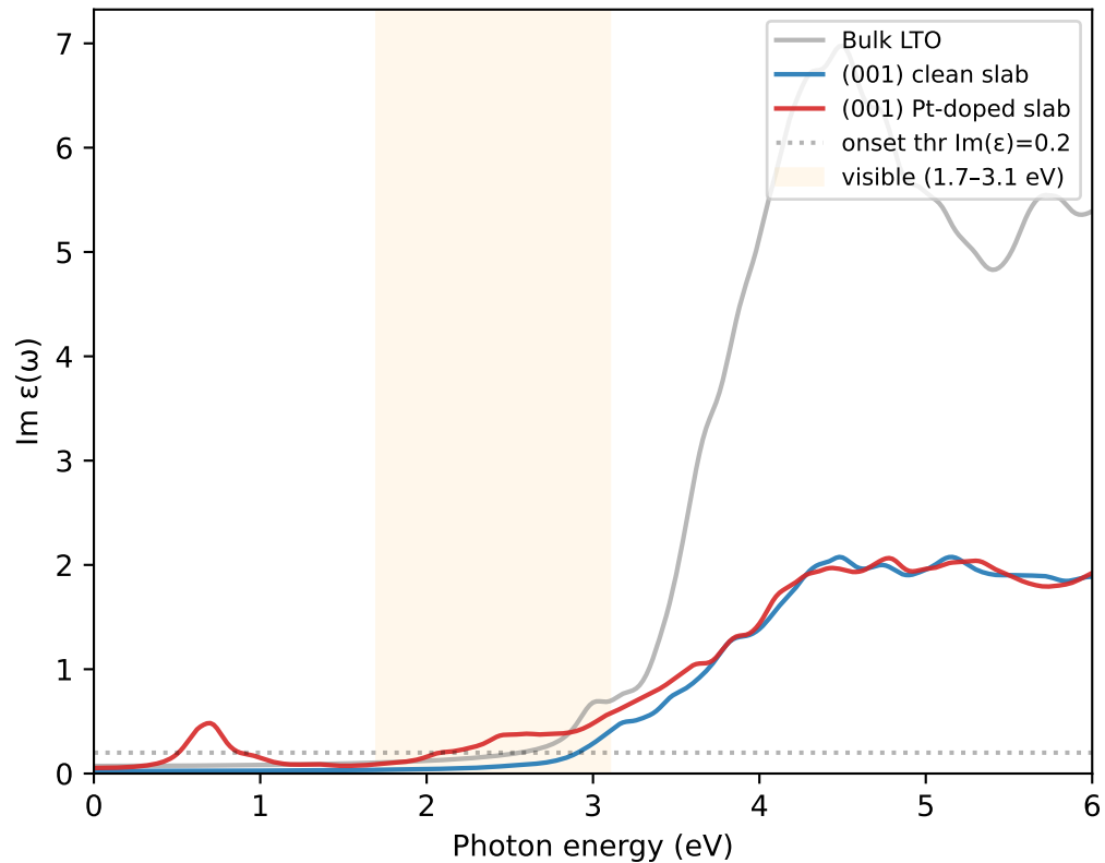
Yambo PBE/RPA dielectric function
