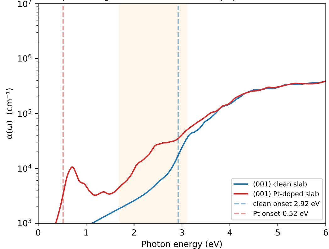
Absorption edge — redshift 2.40 eV (paper 2.2 eV, 9% diff)
