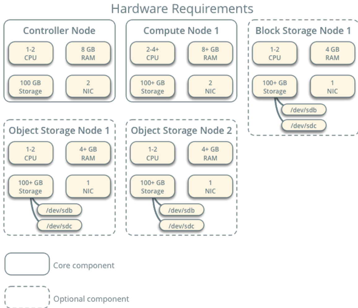
Fig. 2: Hardware requirements.
