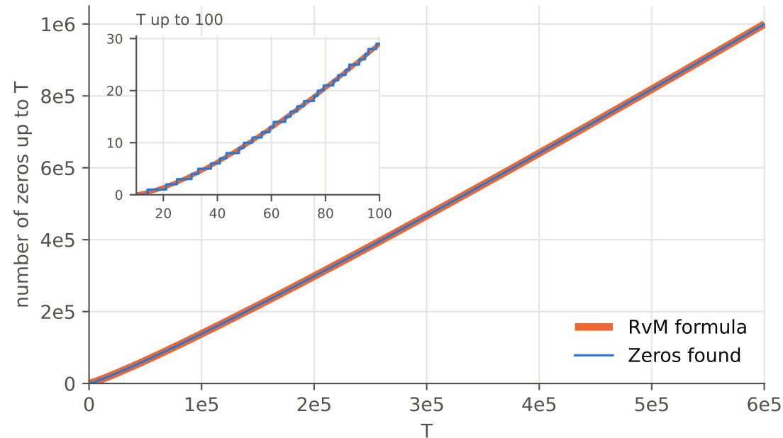
All zeros found, against the Riemann-von Mangoldt formula
