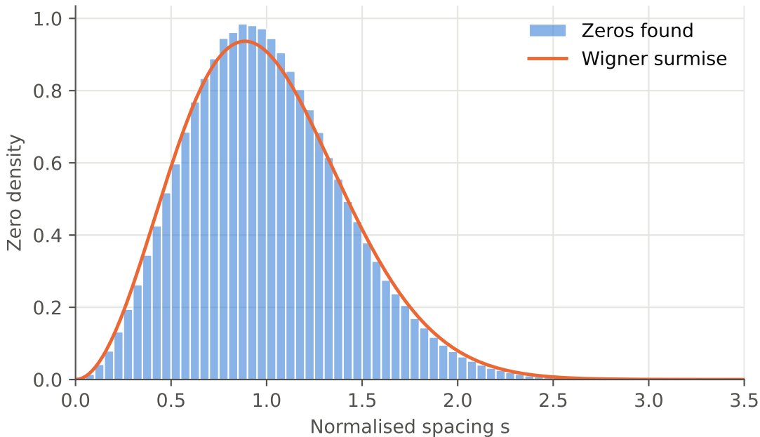
Spacings between consecutive zeros (1 = average spacing)
