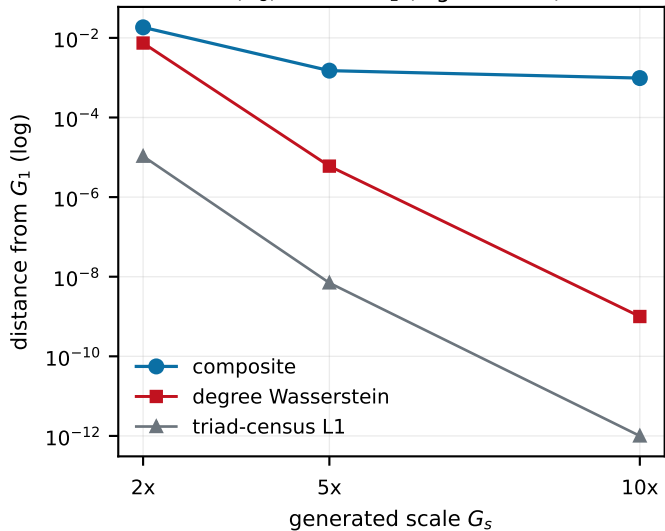
R(G_s) toward G_1 (log distance)
