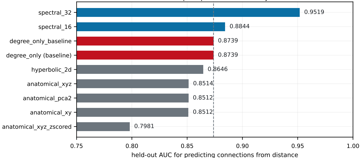
Which space predicts connectivity?
