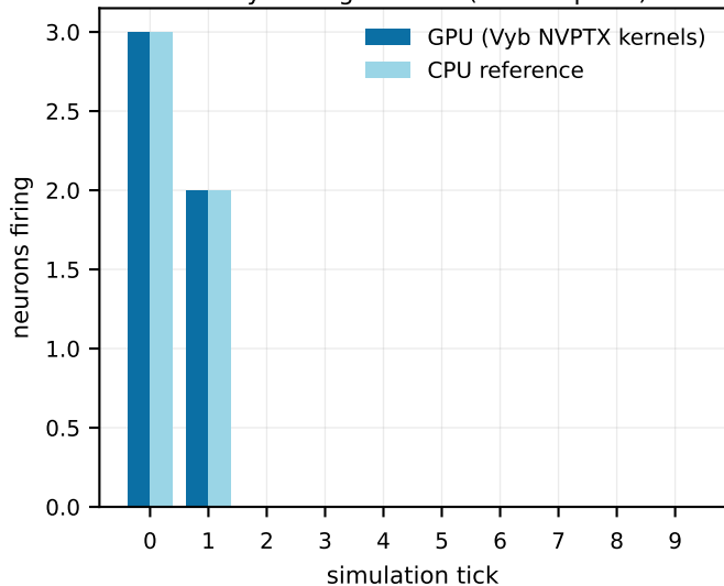
tick-by-tick agreement (5 vs 5 spikes)
