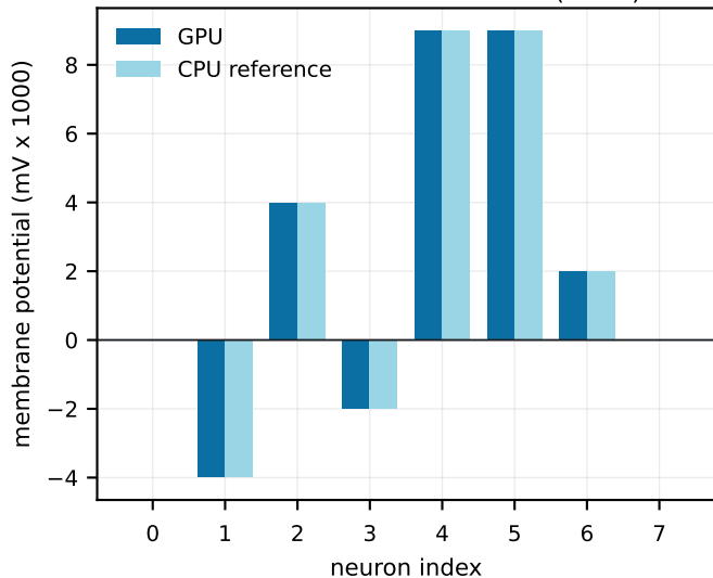
membrane trace after 30 ticks (exact)
