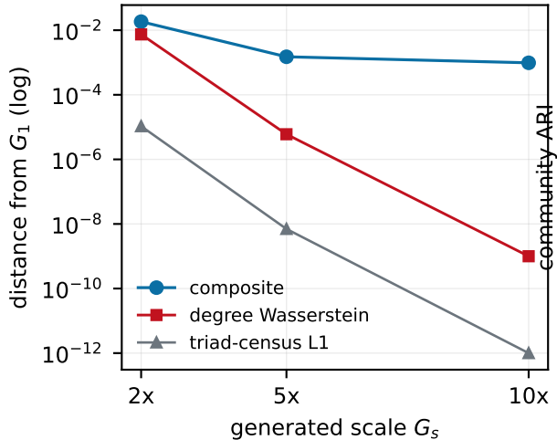
R(G_s) approaches the biological graph
