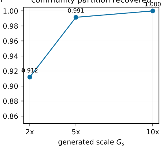
community partition recovered
