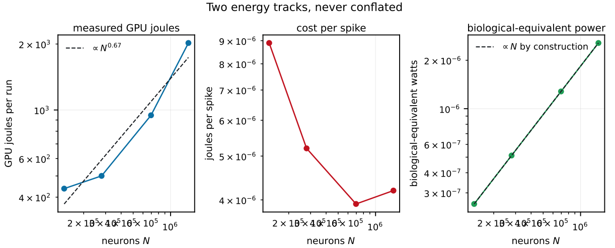
Figure 9: Energy across scales. Left: measured GPU joules grow sublinearly. Center: cost per spike falls by a factor of two — a device-utilisation effect, not biological efficiency. Right: the biological-equivalent track is linear in N by construction ; it is a model identity, reported separately precisely so that it cannot be mistaken for a measurement.
