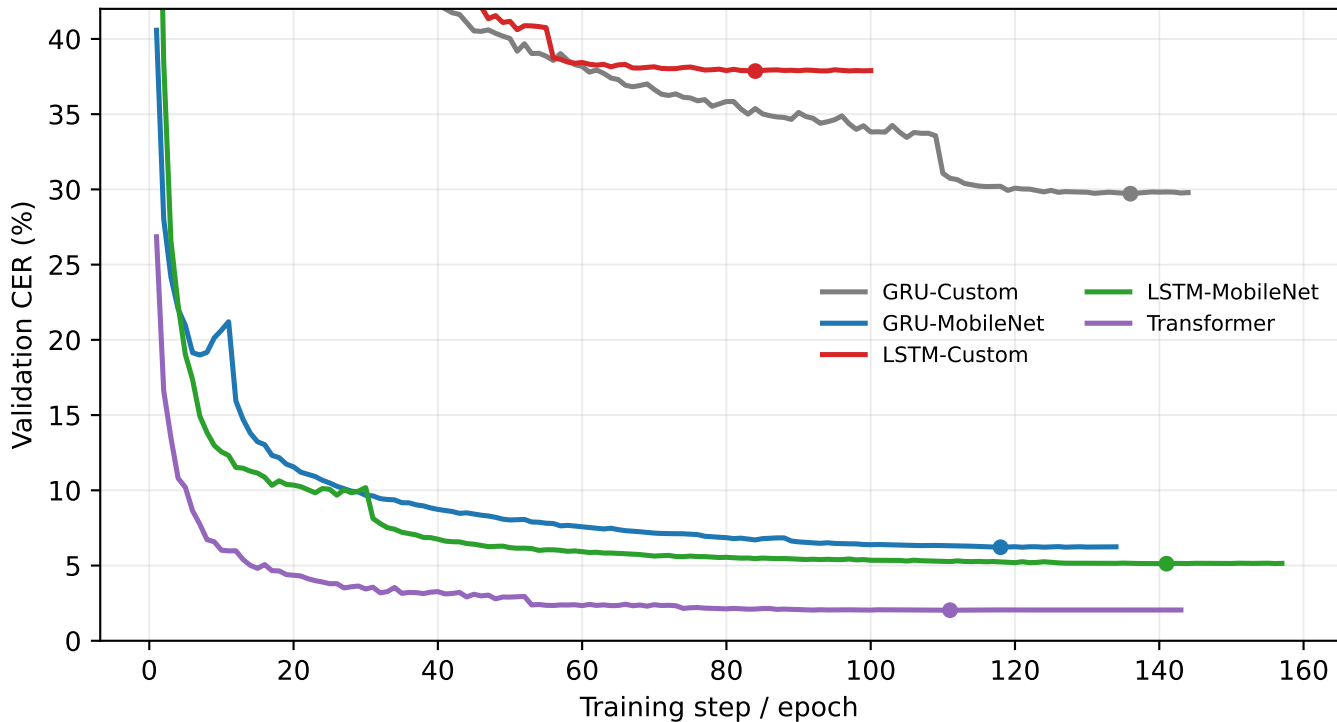
OCR validation CER from preserved TensorBoard scalars
