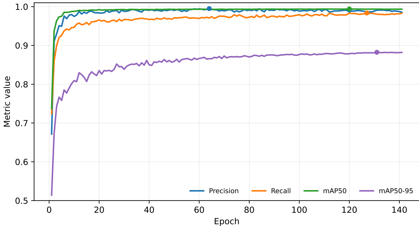
YOLOv11n-OBB internal validation metrics over epochs
