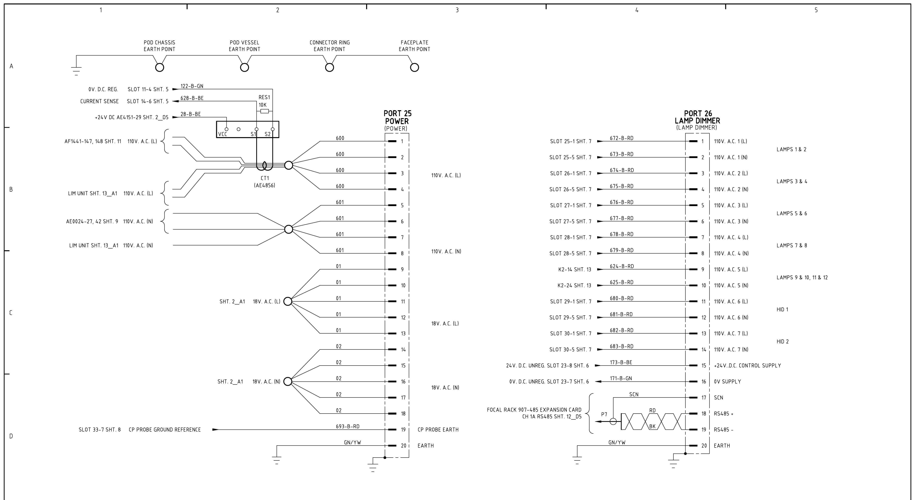
DRAWING Q CORE POD WIRING (FACEPLATE CONNECTORS - POD POWER & LAMP DIMMER)
