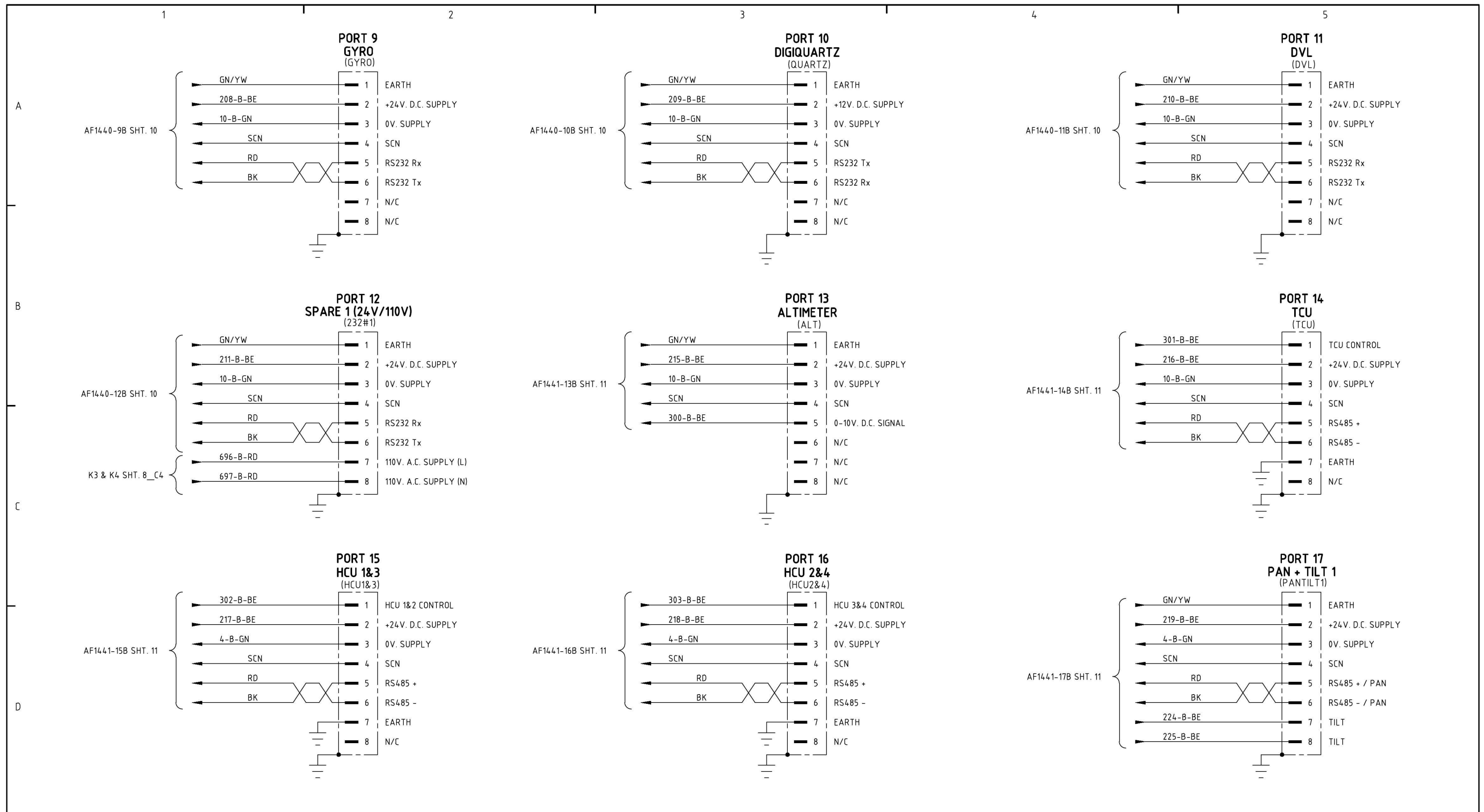
DRAWING Q CORE POD WIRING (FACEPLATE CONNECTORS - PORTS 9-17)
