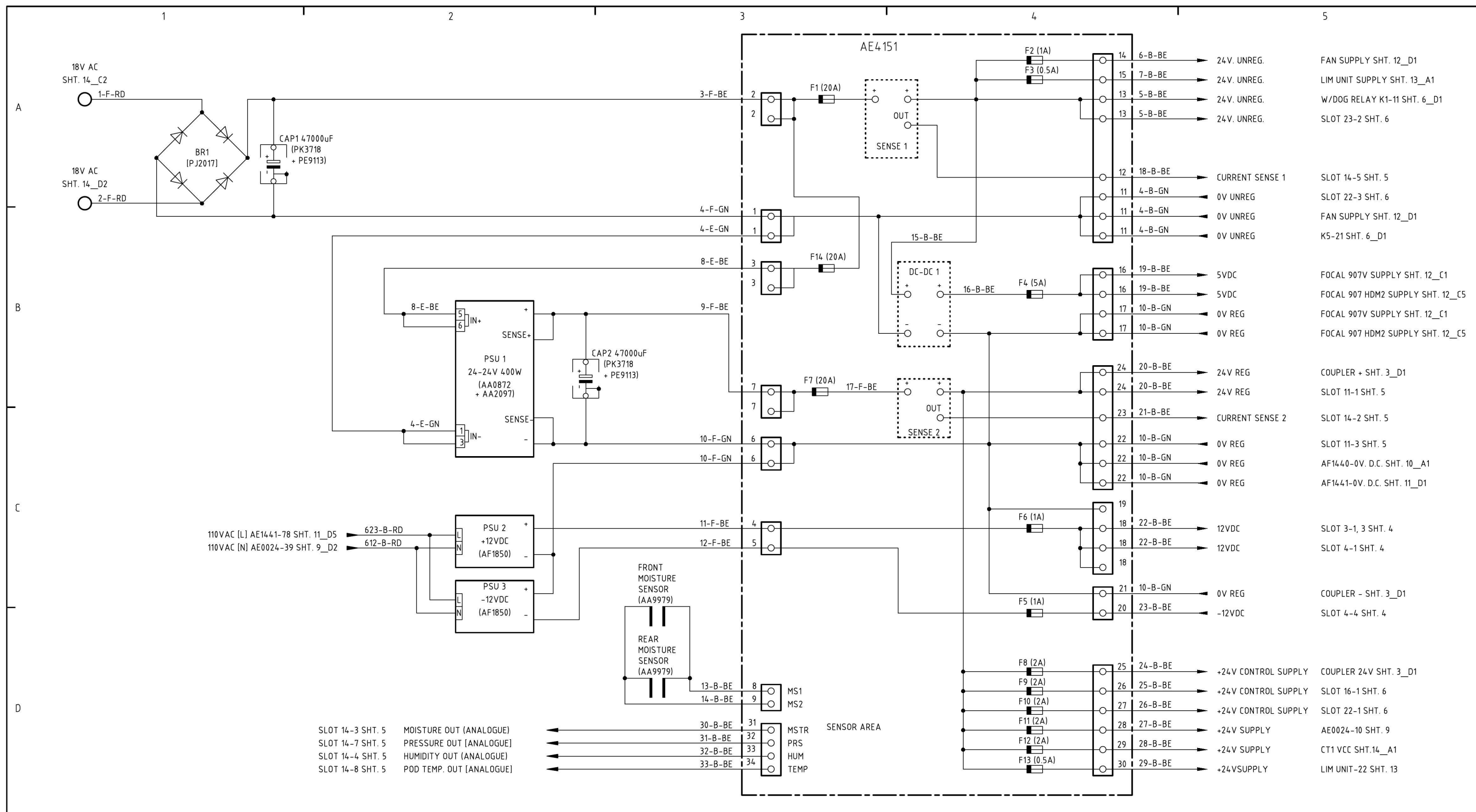
DRAWING Q CORE POD WIRING (24V PSU BOARD AE4151 [REGULATED & UNREGULATED])
