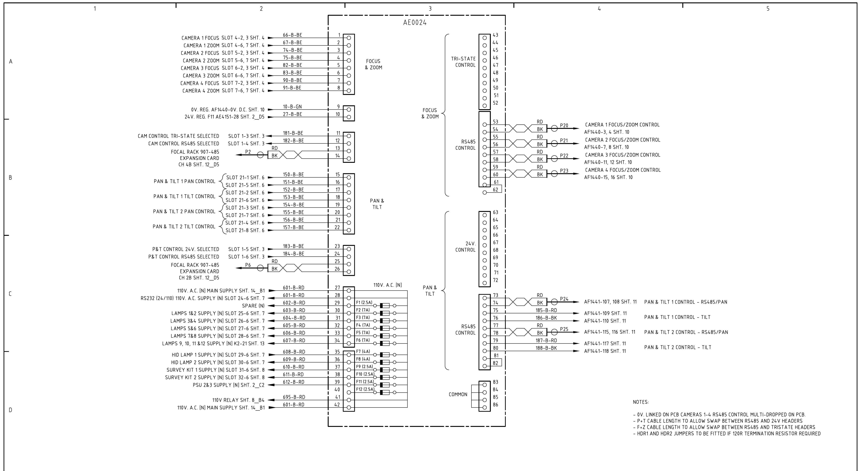
DRAWING Q CORE POD WIRING (CAMERA CONTROL CARD AE0024/110VAC NEUTRAL DIST.)
