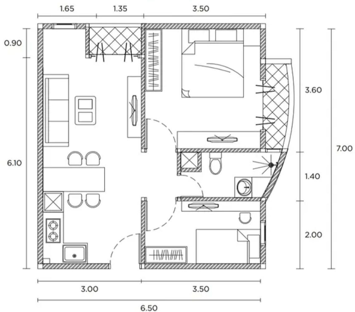
FLOOR PLAN
