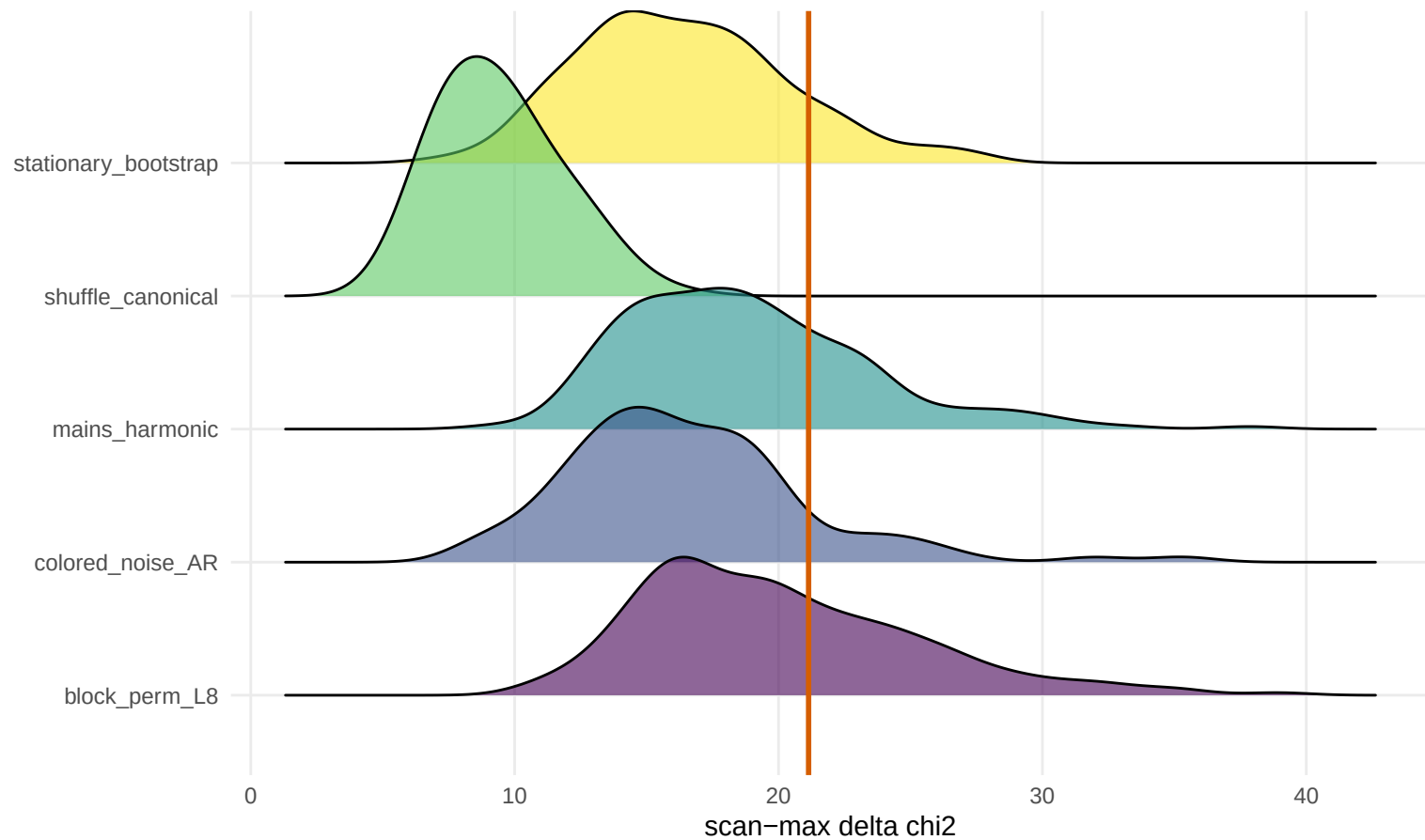
fig12 Null distributions (red = observed)
