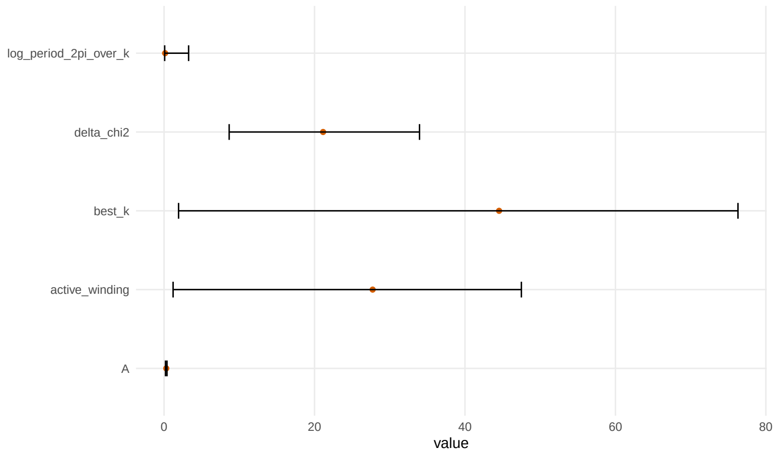
fig13 Log-cos bootstrap CIs
