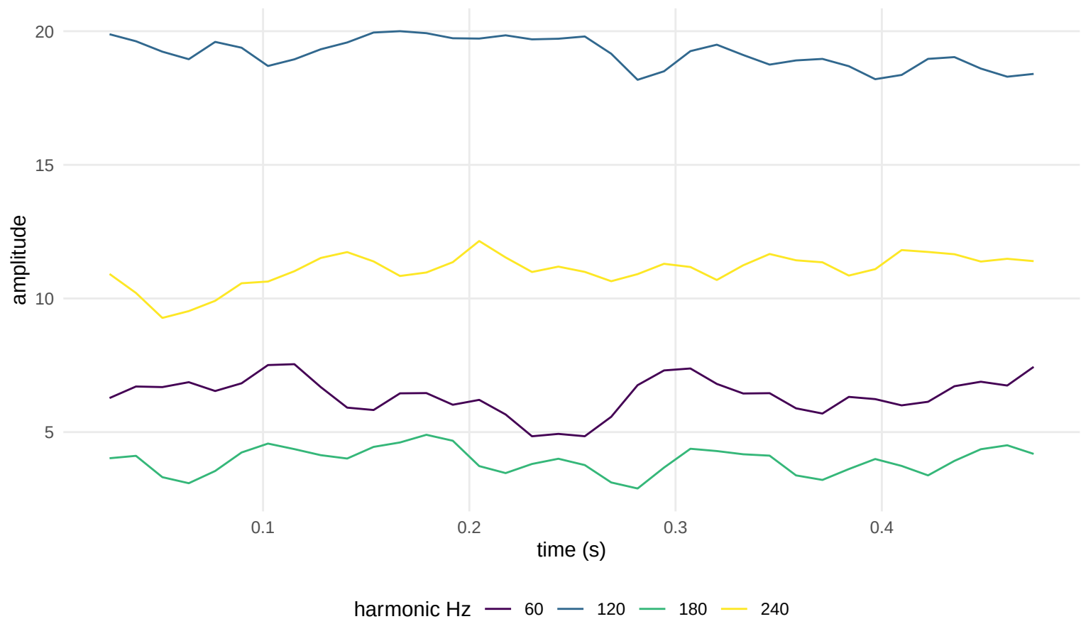
fig16 Harmonic amplitude vs time (within 0.5 s capture only)
