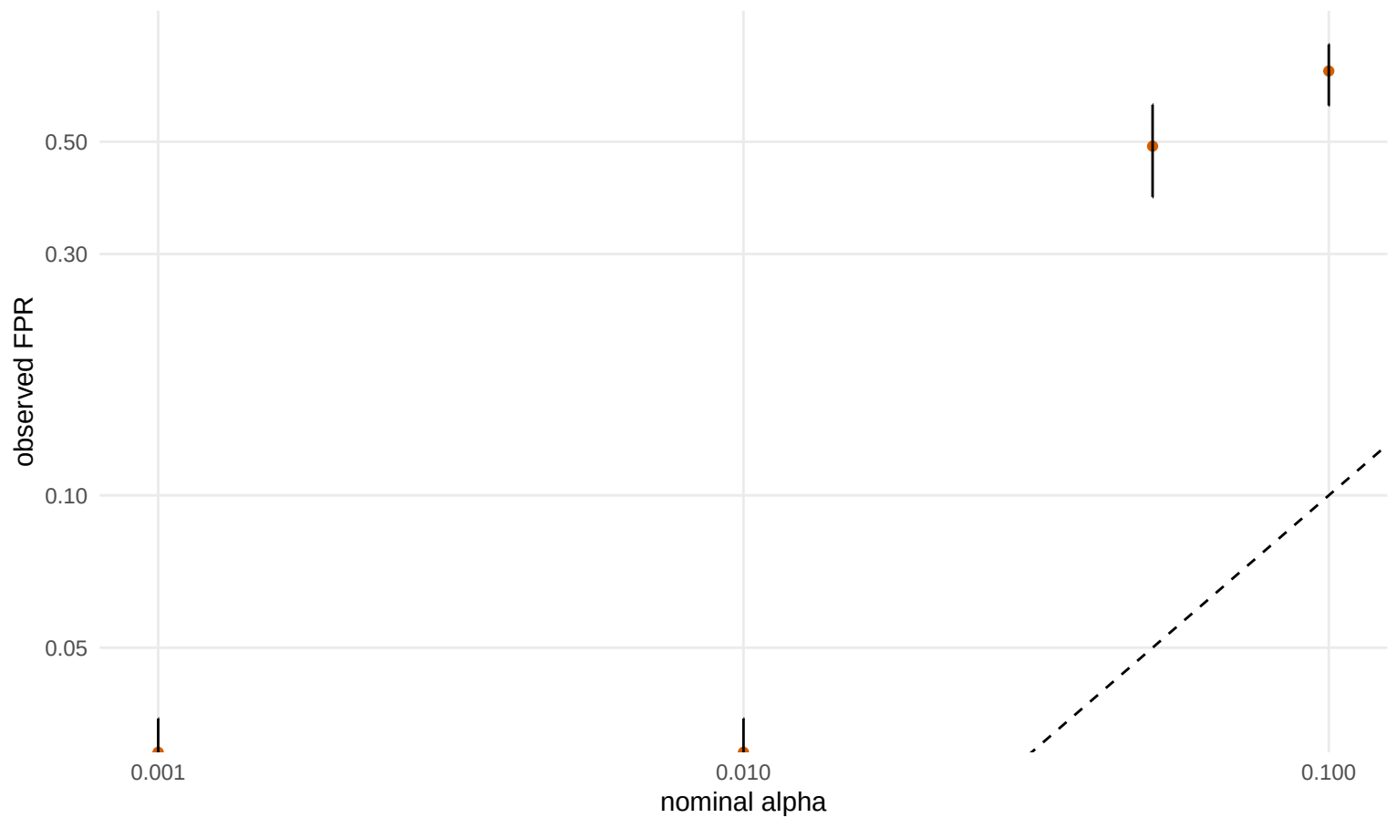
fig18 Null calibration
