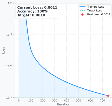
Training Loss
