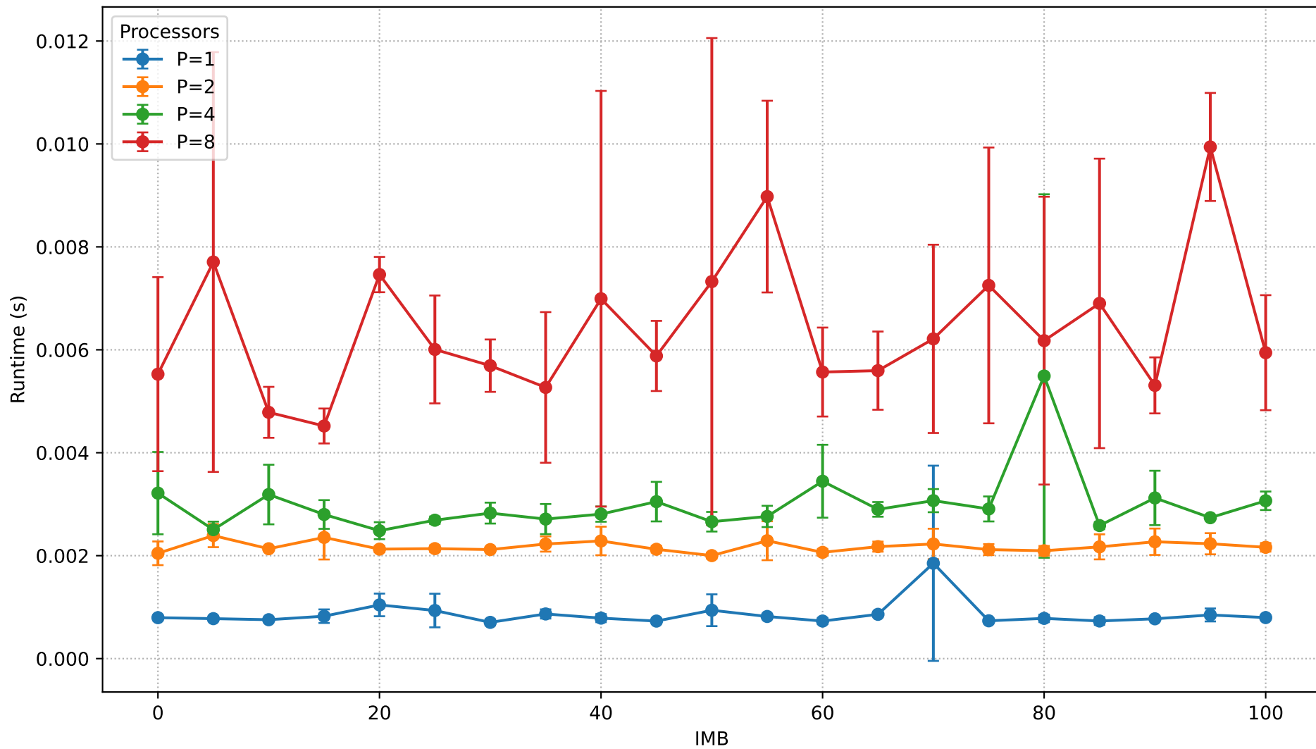
Runtime vs IMB (N=700,000)
