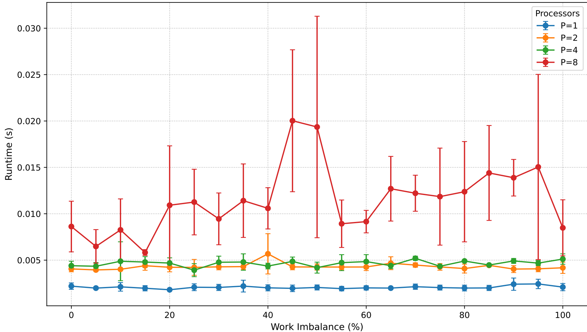
Dyck Path Validation: Runtime vs Work Imbalance (N=600,000)
