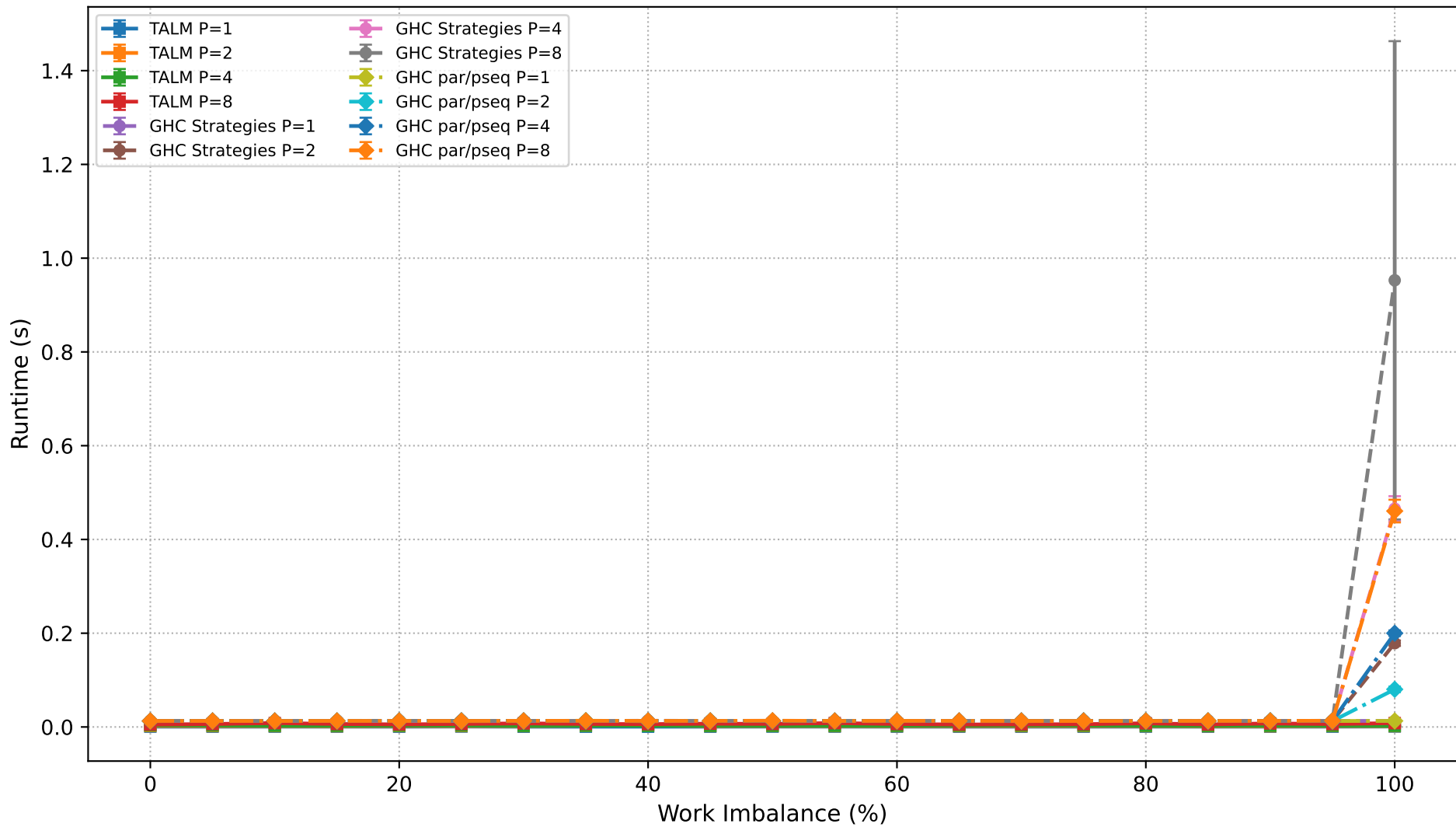
Dyck Path Validation: Runtime Comparison (N=350,000)
