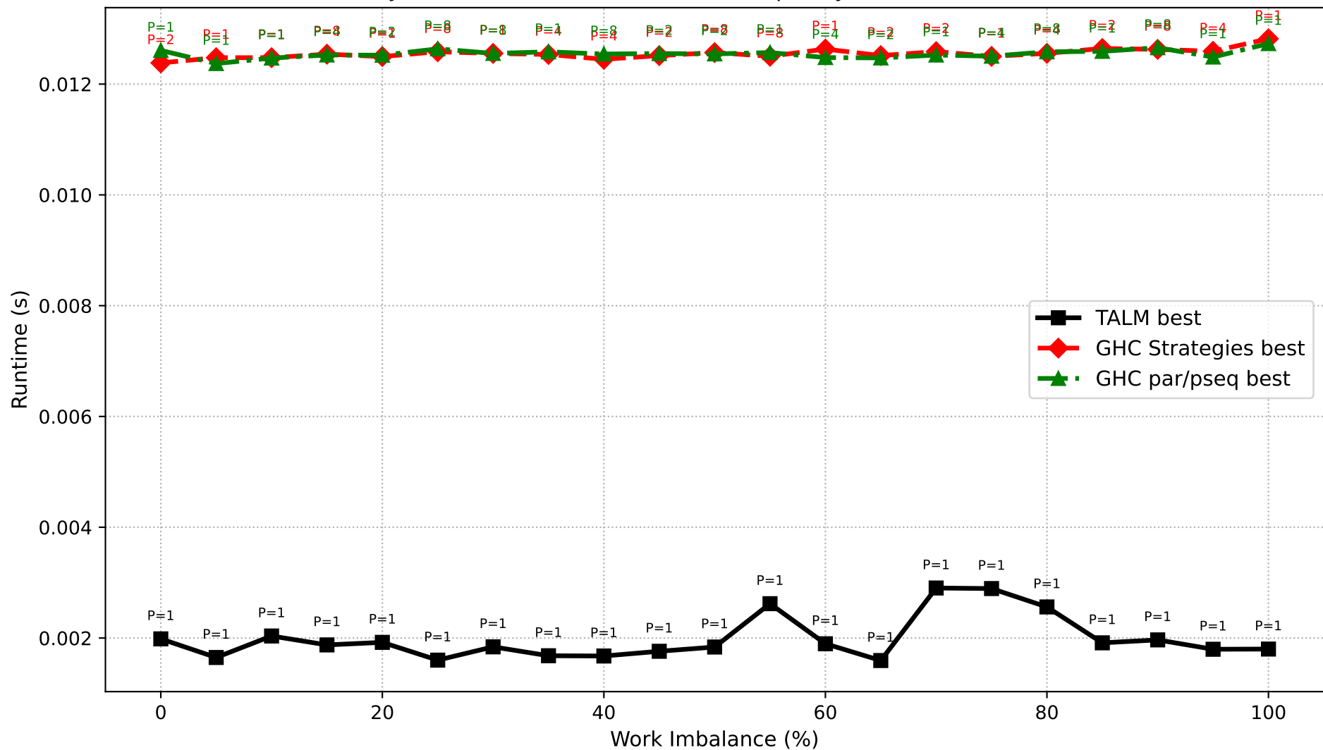
Dyck Path Validation: Best Runtime per System (N=500,000)
