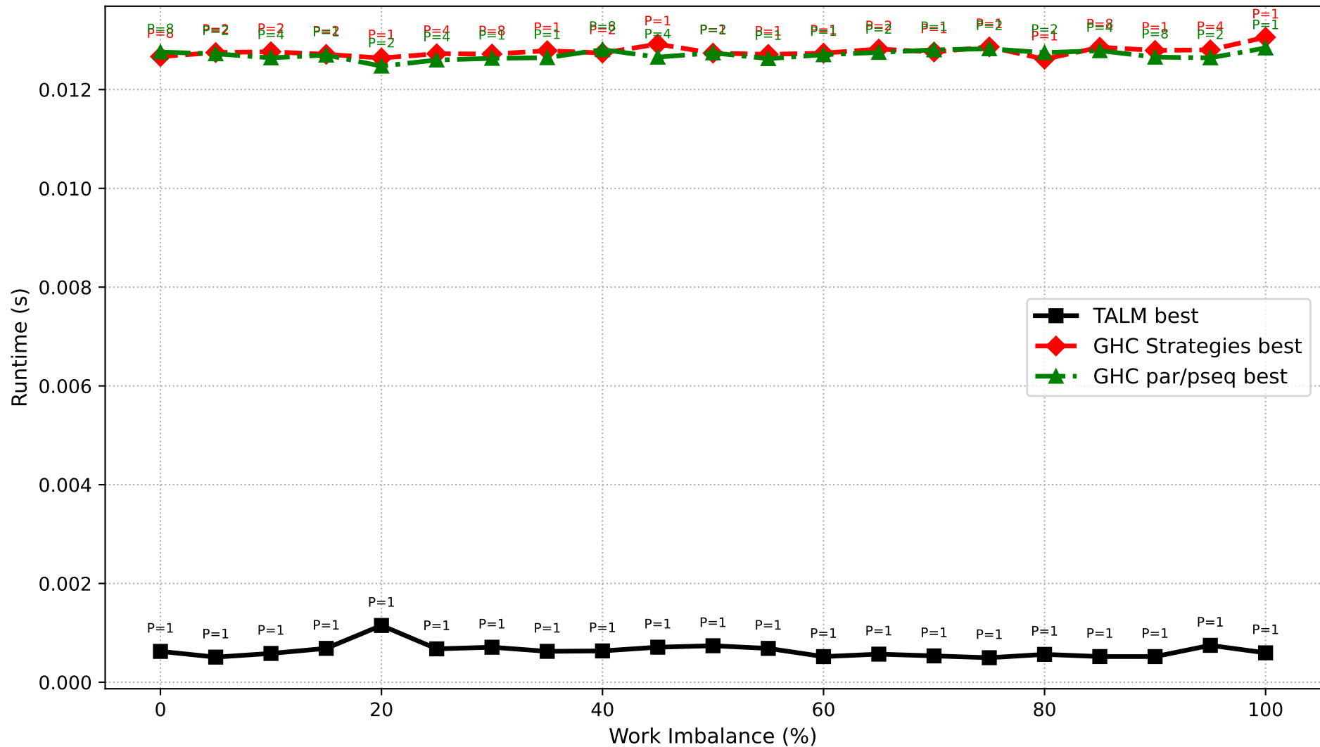
Dyck Path Validation: Best Runtime per System (N=250,000)
