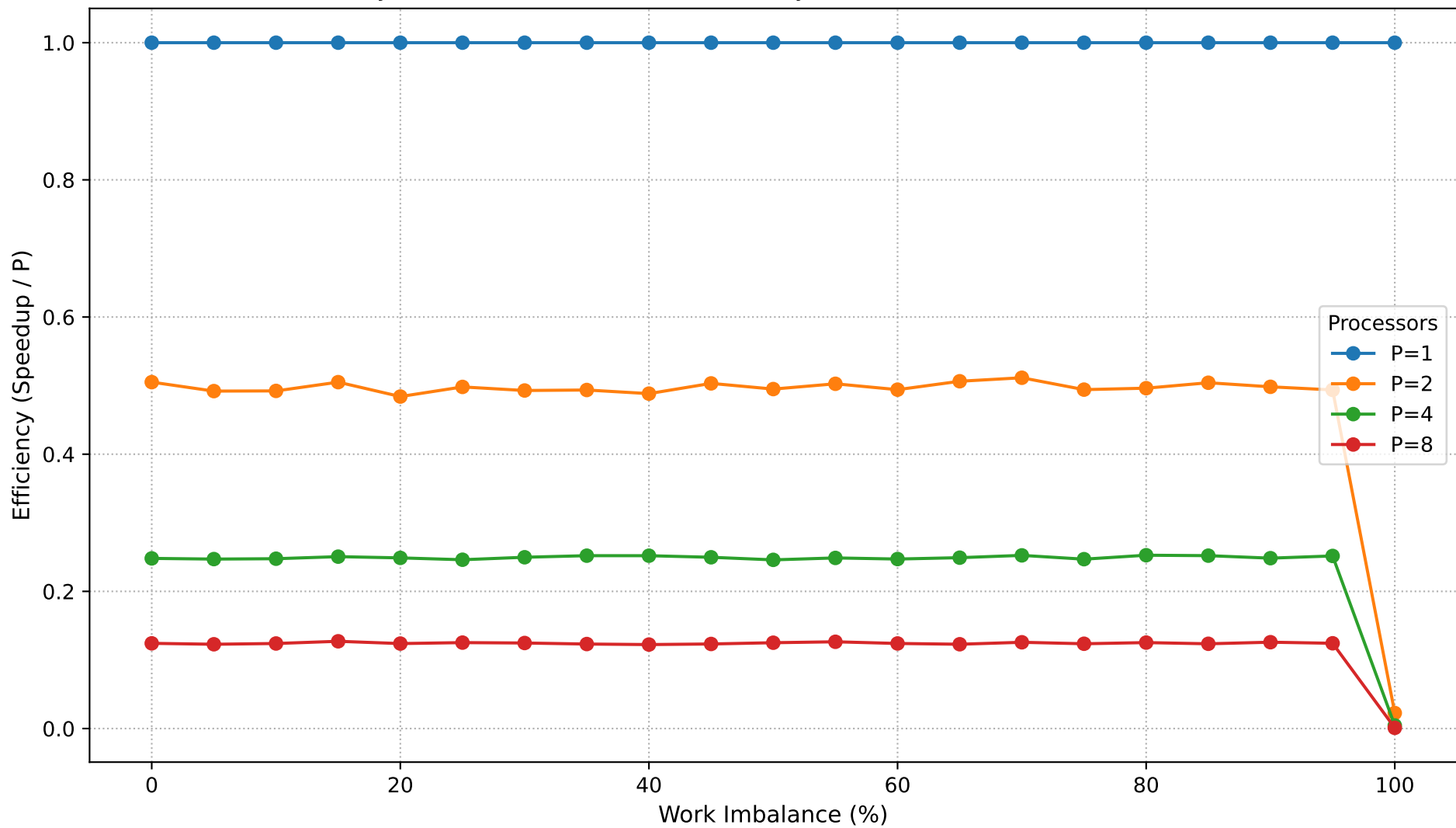
Dyck Path Validation: Parallel Efficiency vs Work Imbalance (N=500,000)
