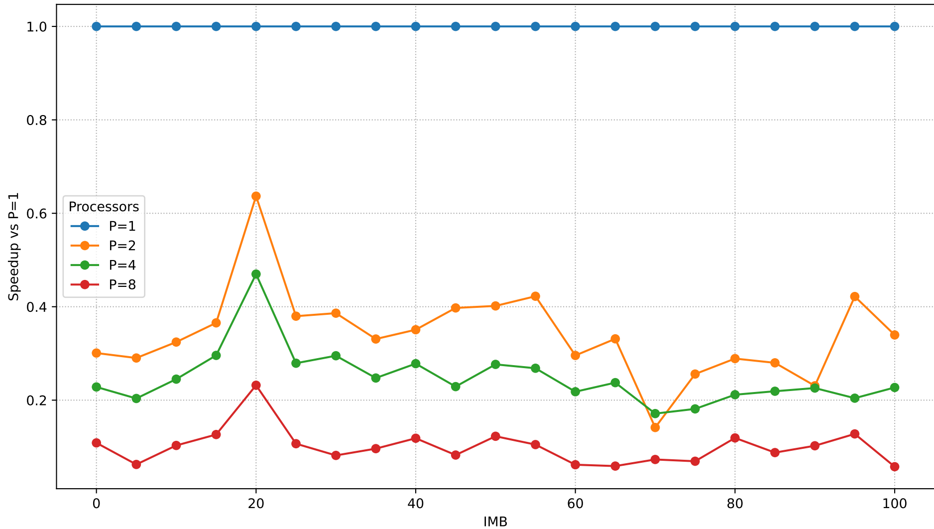
Speedup vs IMB (N=250,000)
