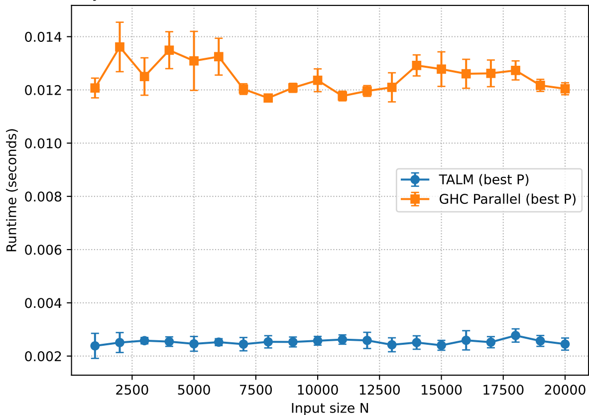
Dyck Path: Best-of-Breed Runtime vs N (imb=25, delta=1000)
