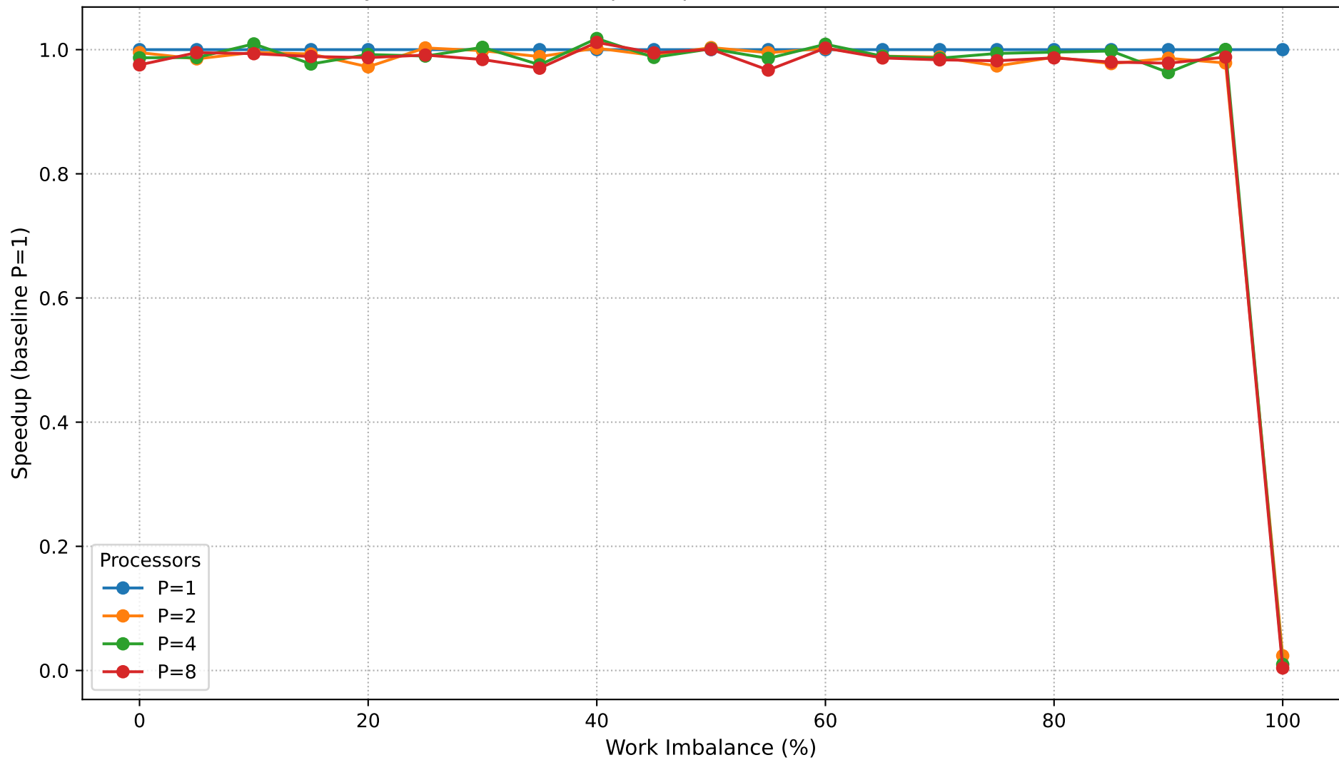
Dyck Path Validation: Speedup vs Work Imbalance (N=950,000)
