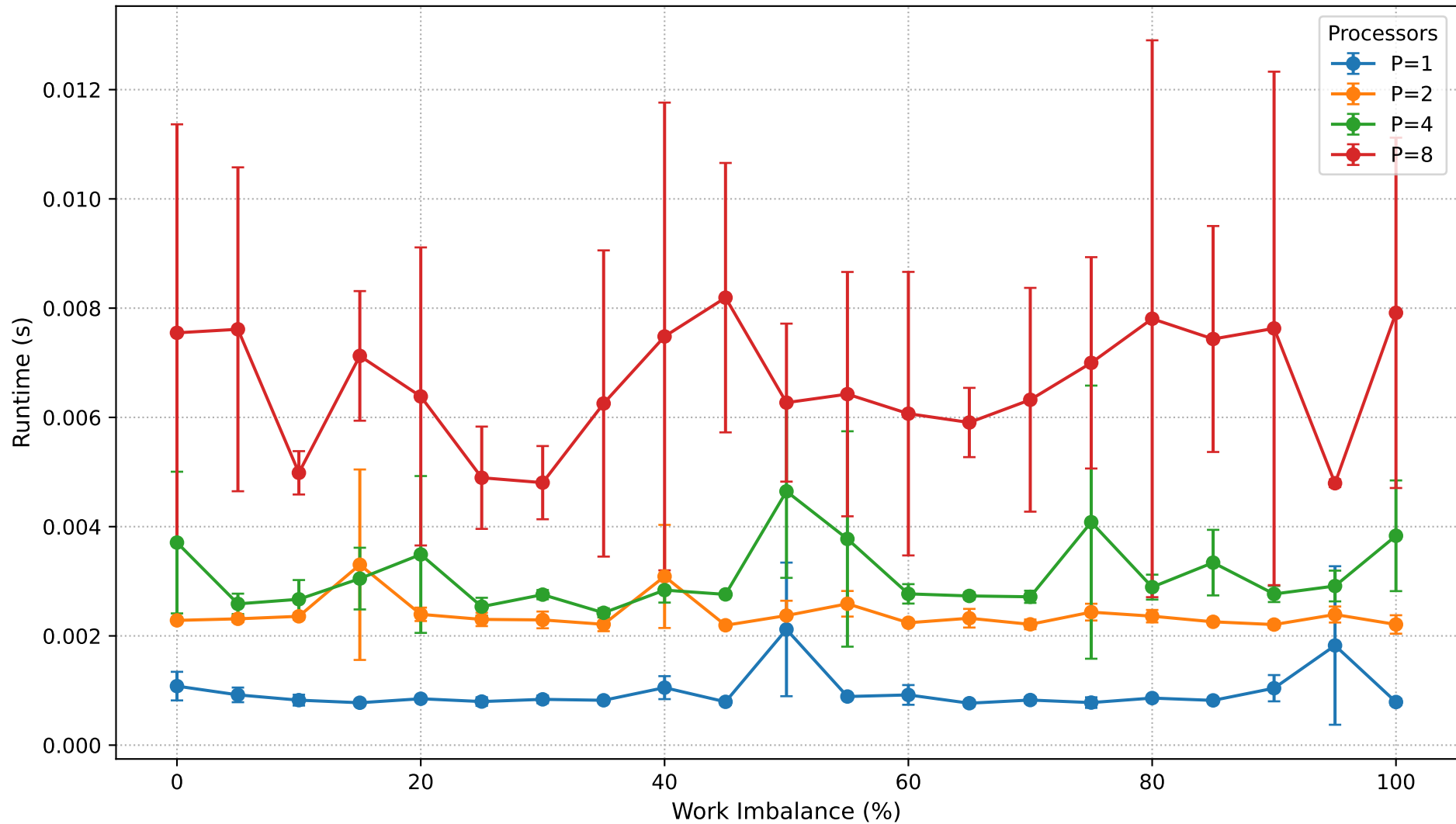
Dyck Path Validation: Runtime vs Work Imbalance (N=850,000)
