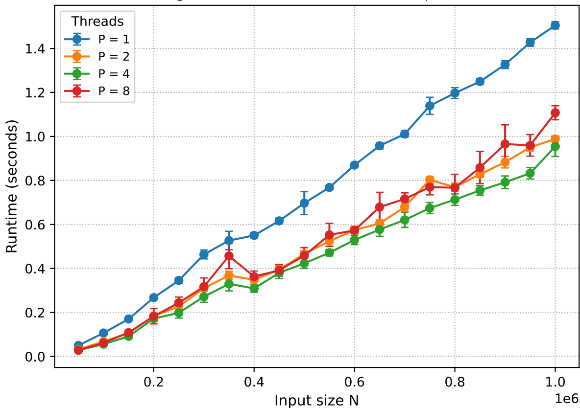
Merge Sort (GHC -N): Runtime vs Input Size
