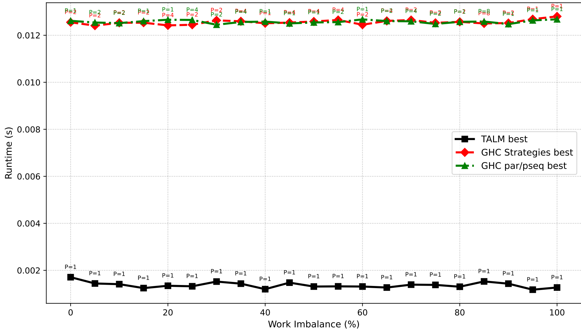
Dyck Path Validation: Best Runtime per System (N=350,000)
