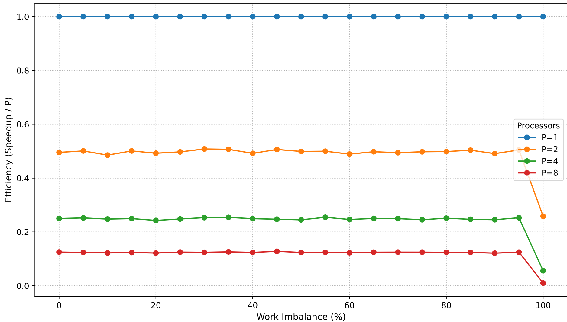
Dyck Path Validation: Parallel Efficiency vs Work Imbalance (N=100,000)
