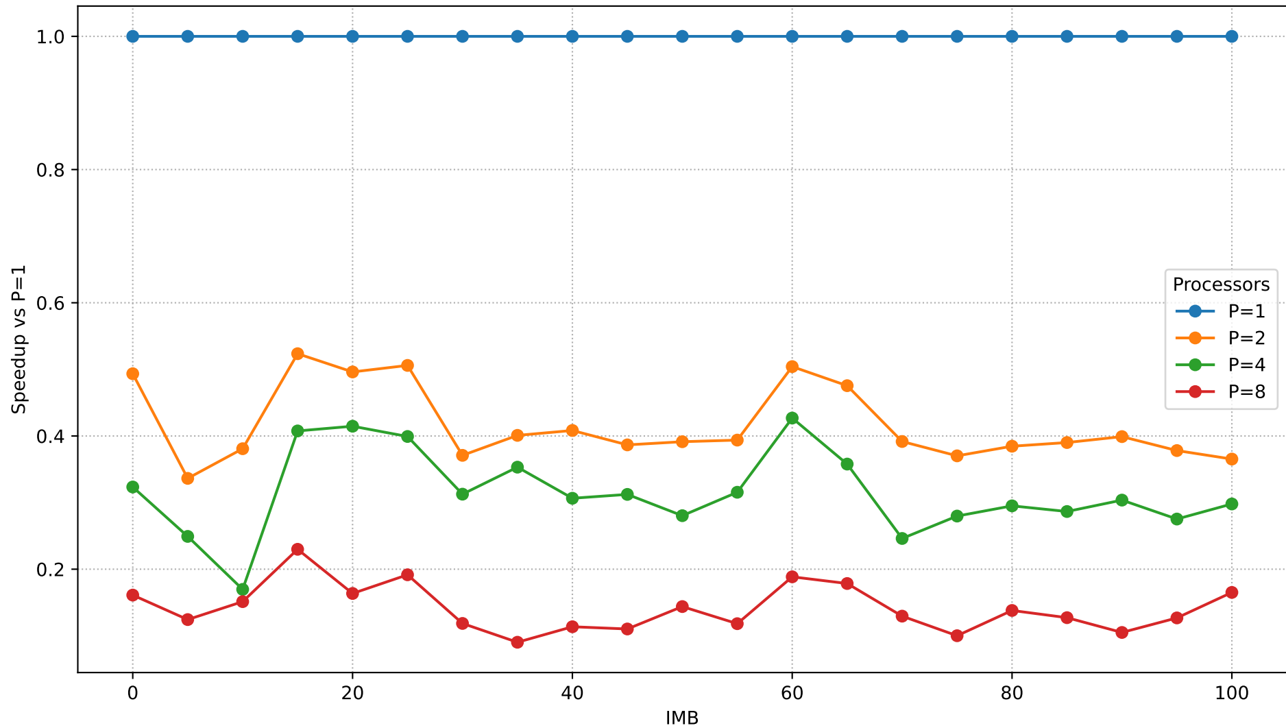
Speedup vs IMB (N=900,000)
