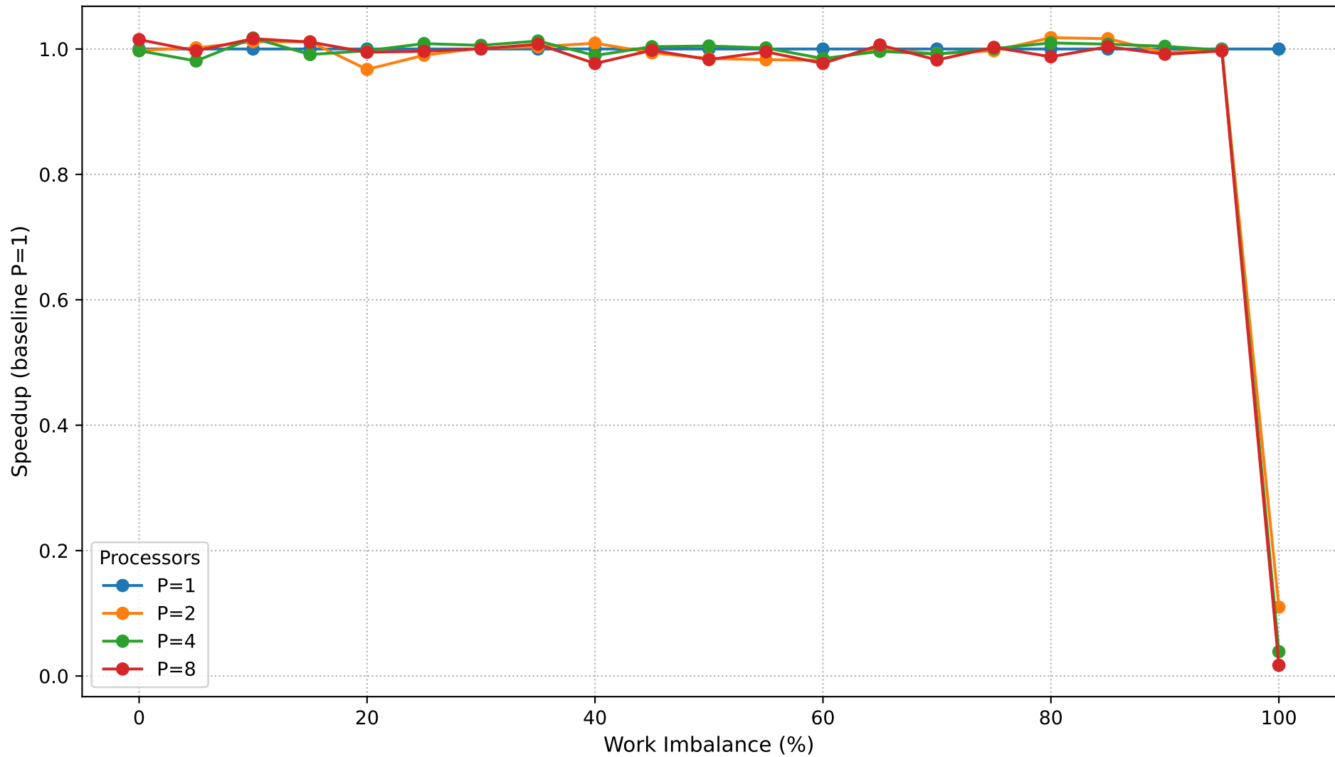
Dyck Path Validation: Speedup vs Work Imbalance (N=550,000)
