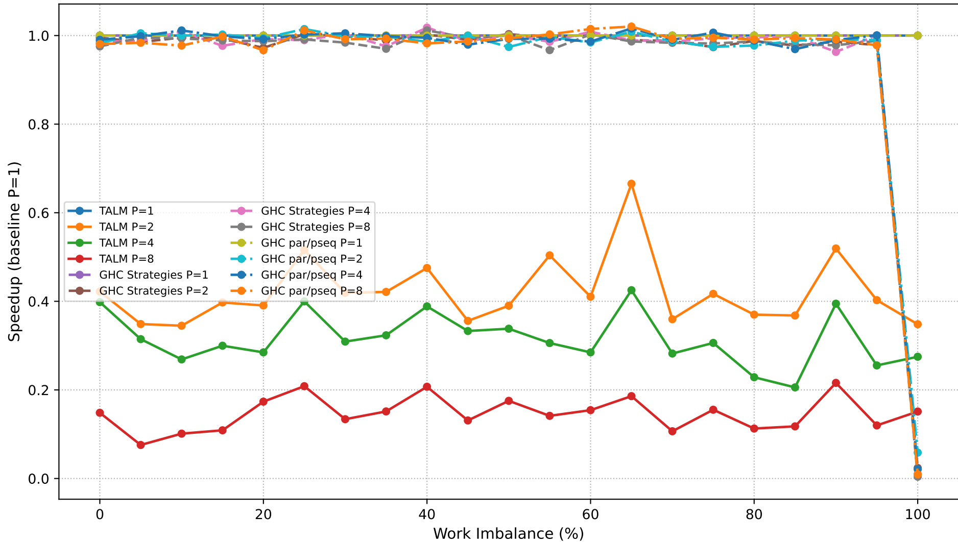
Dyck Path Validation: Speedup Comparison (N=950,000)
