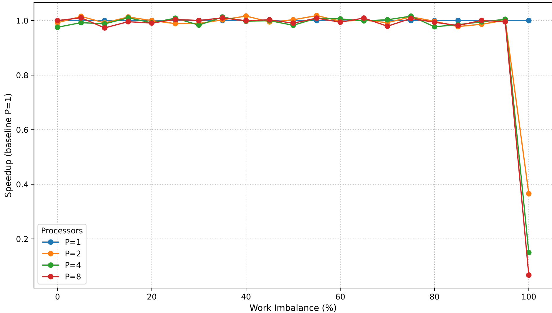
Dyck Path Validation: Speedup vs Work Imbalance (N=150,000)
