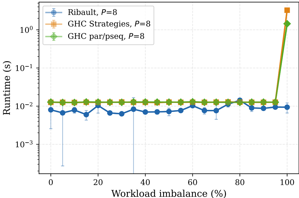
Dyck Paths: Runtime vs. Workload Imbalance ( P = 8 )
