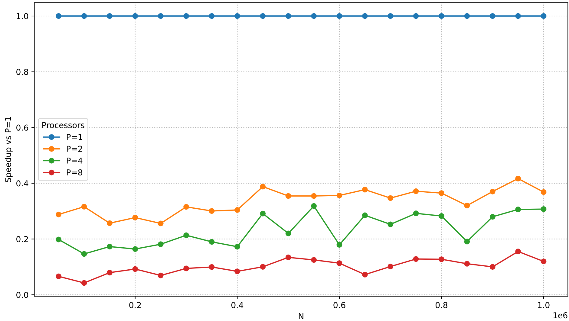
Speedup vs N (IMB=75)
