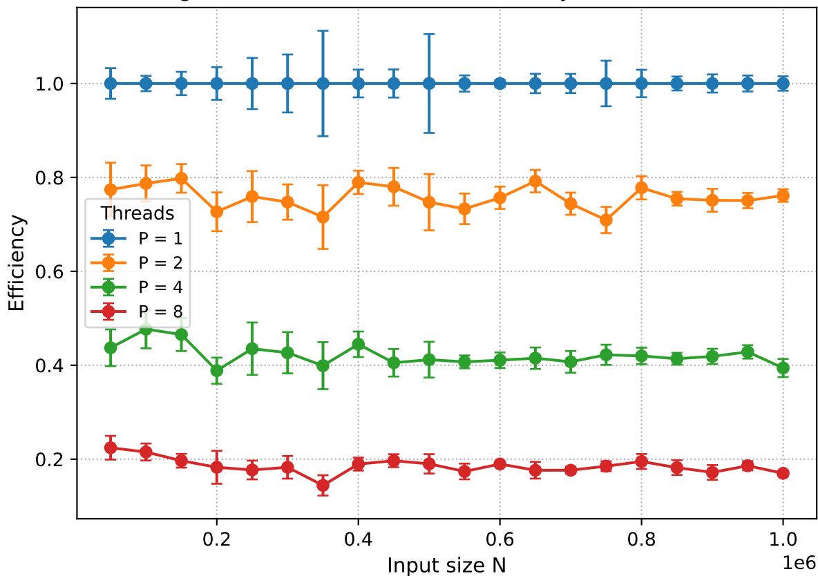
Merge Sort (GHC -N): Parallel Efficiency (baseline P = 1)
