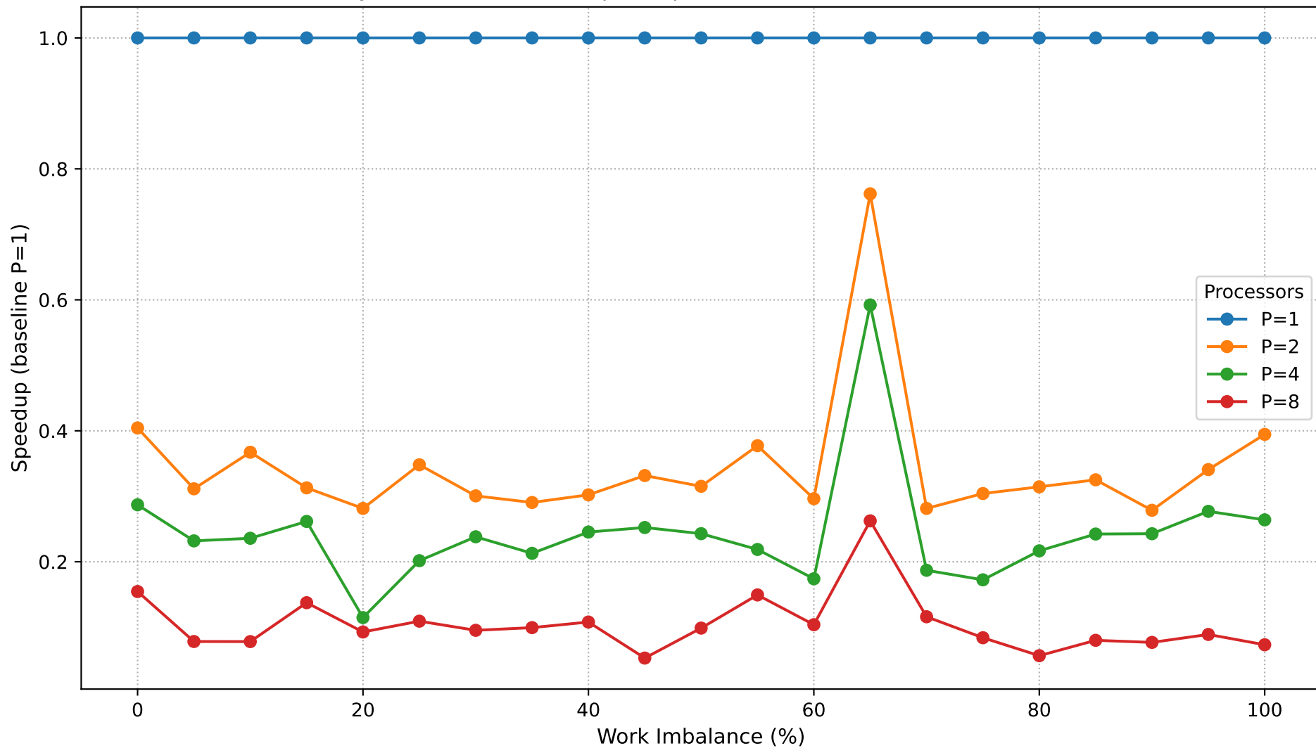
Dyck Path Validation: Speedup vs Work Imbalance (N=400,000)
