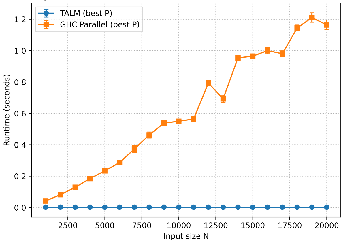
Dyck Path: Best-of-Breed Runtime vs N (imb=100, delta=-1000)
