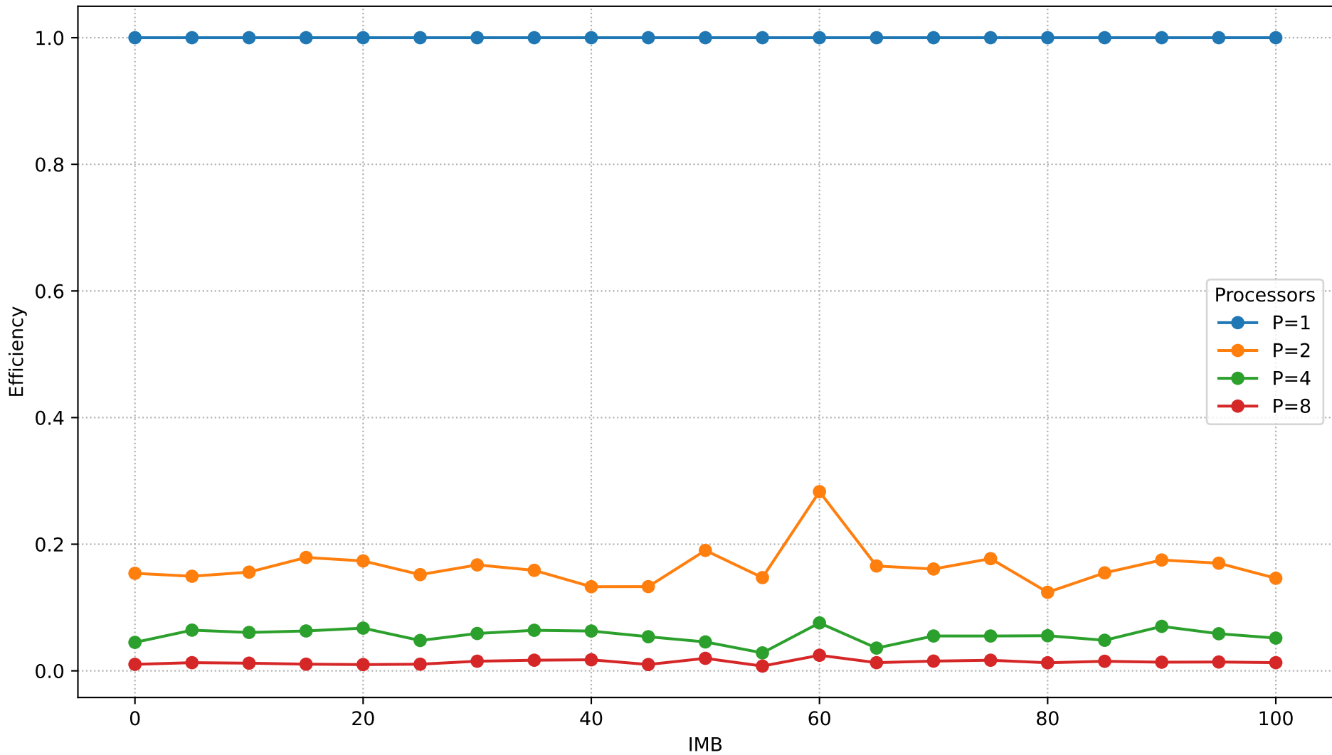
Efficiency vs IMB (N=500,000)
