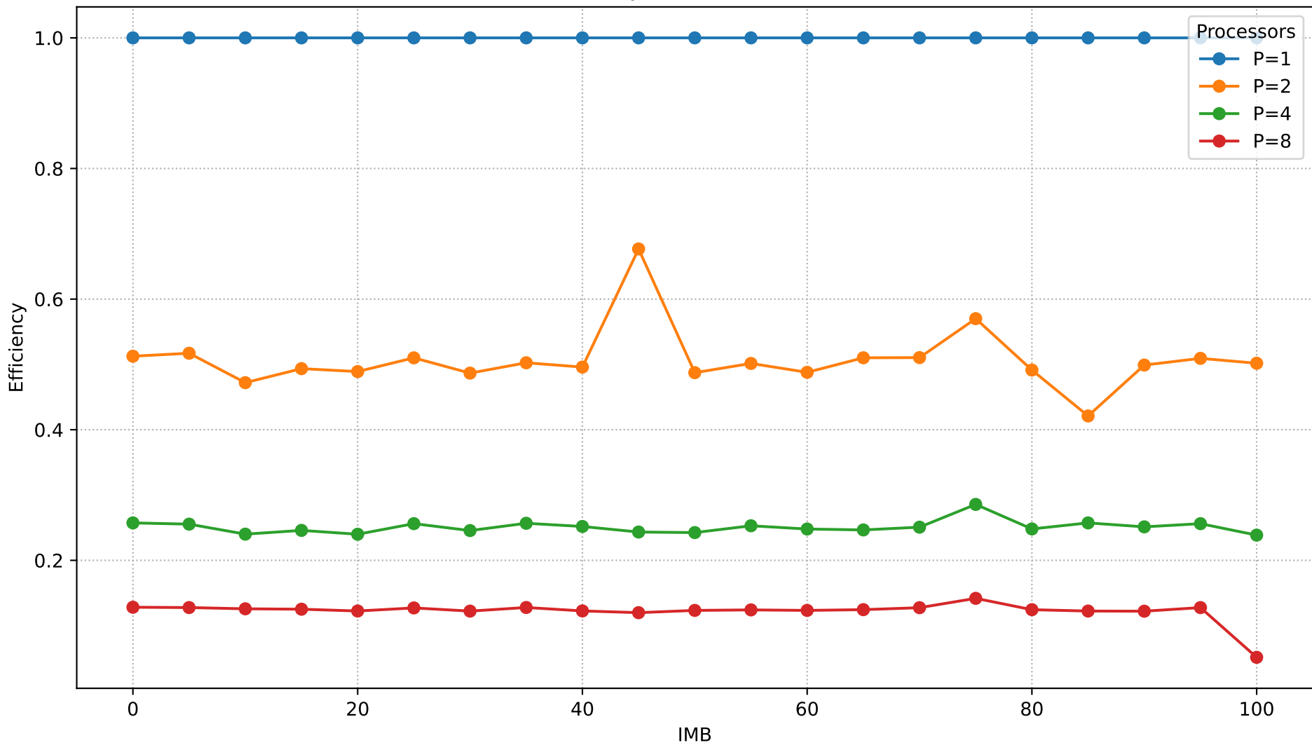
Efficiency vs IMB (N=10000)
