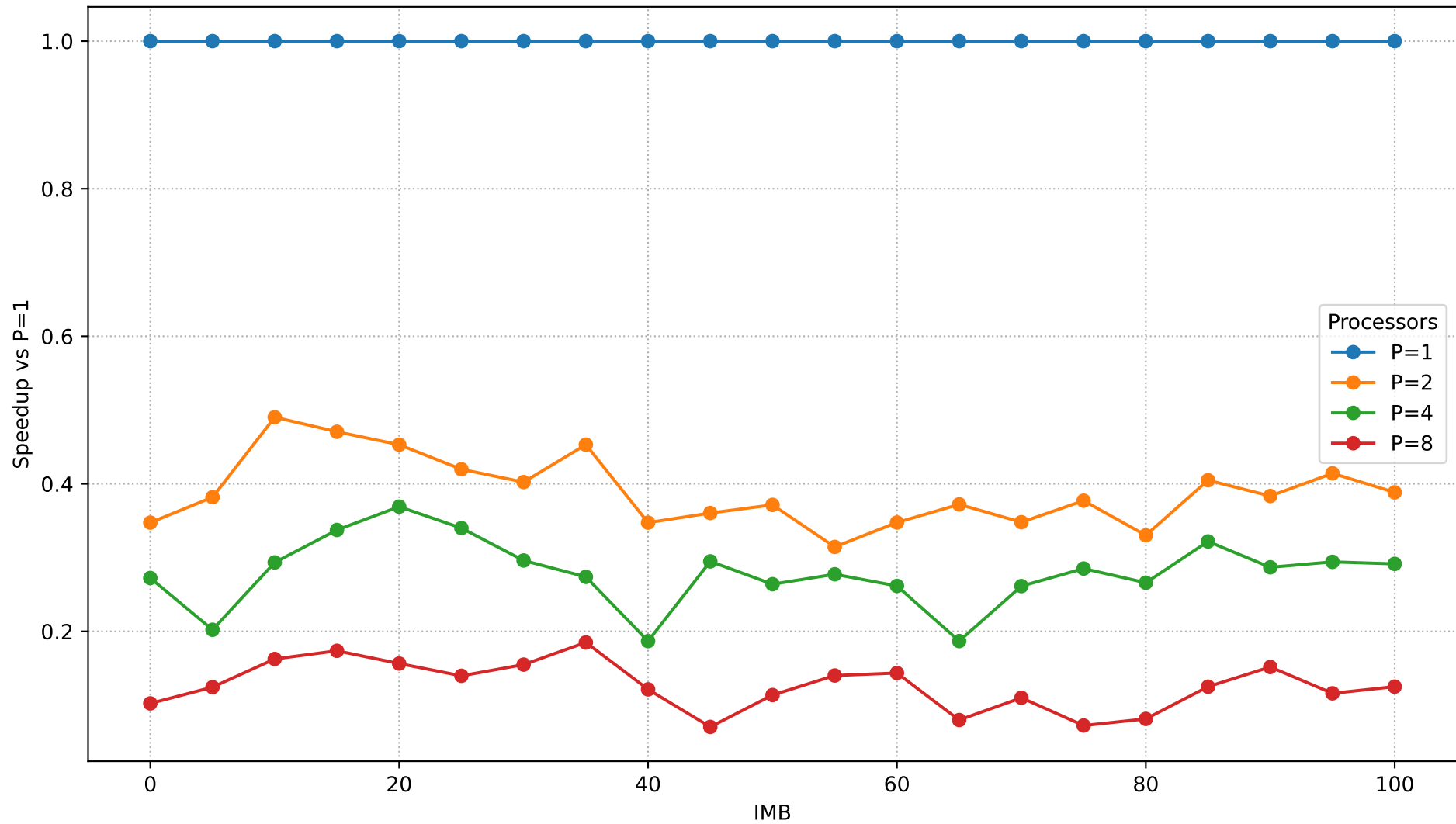
Speedup vs IMB (N=650,000)
