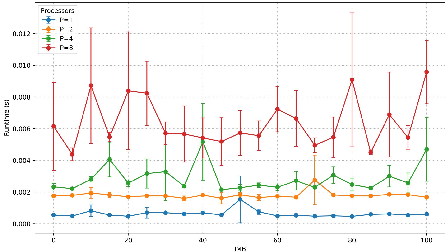
Runtime vs IMB (N=200,000)
