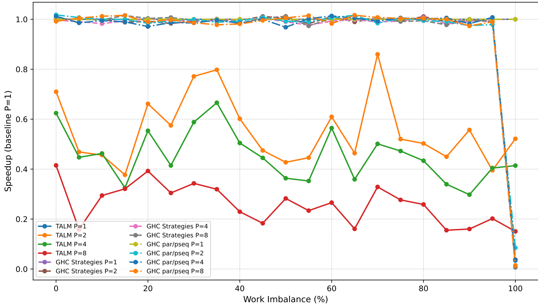
Dyck Path Validation: Speedup Comparison (N=650,000)
