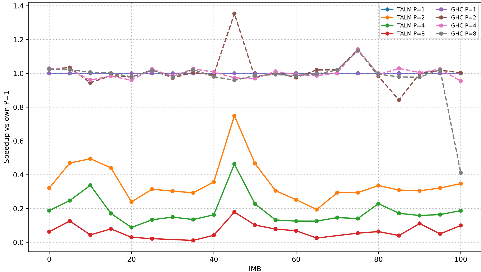
TALM vs GHC - Speedup (N=10000)
