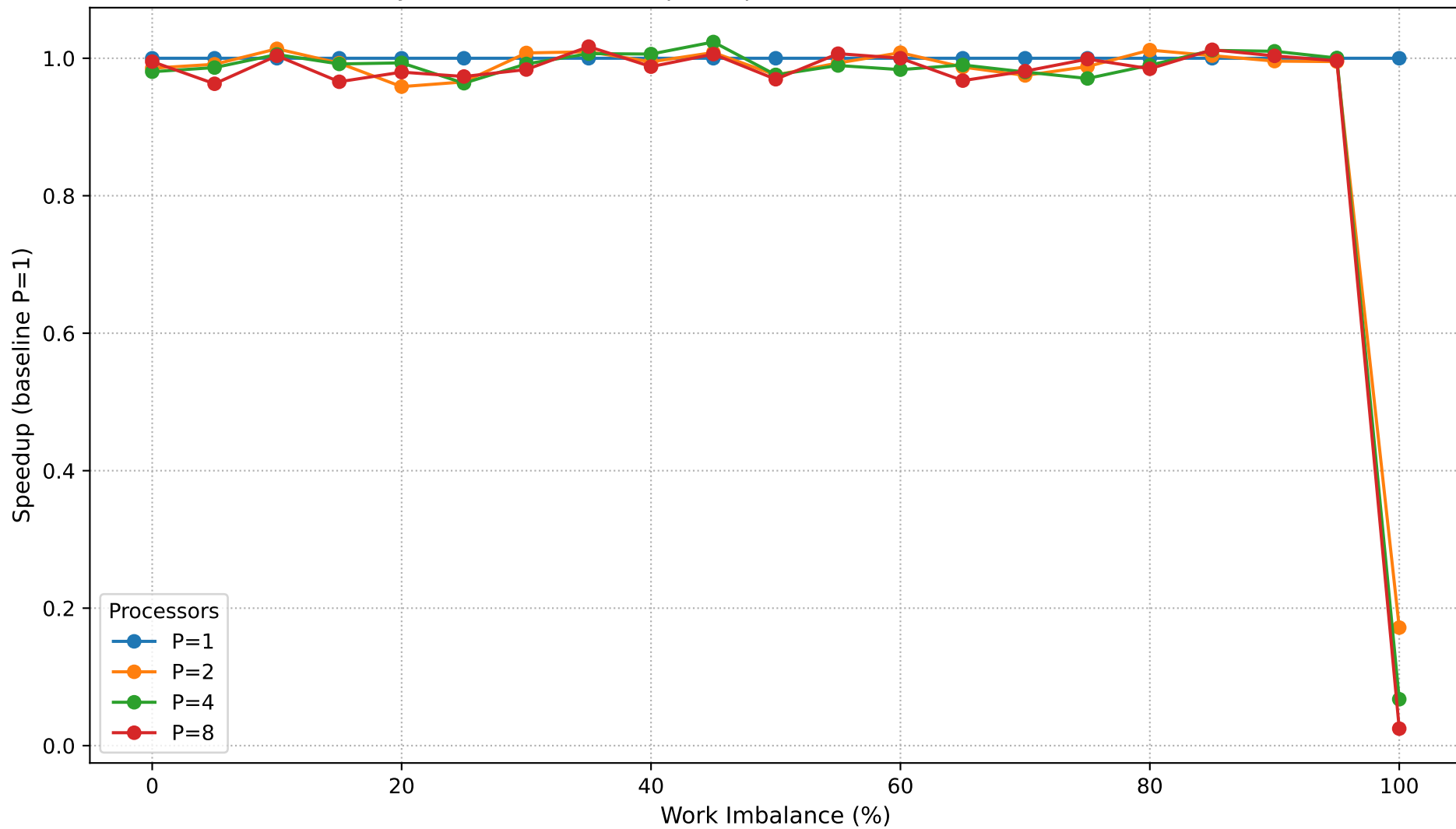
Dyck Path Validation: Speedup vs Work Imbalance (N=300,000)
