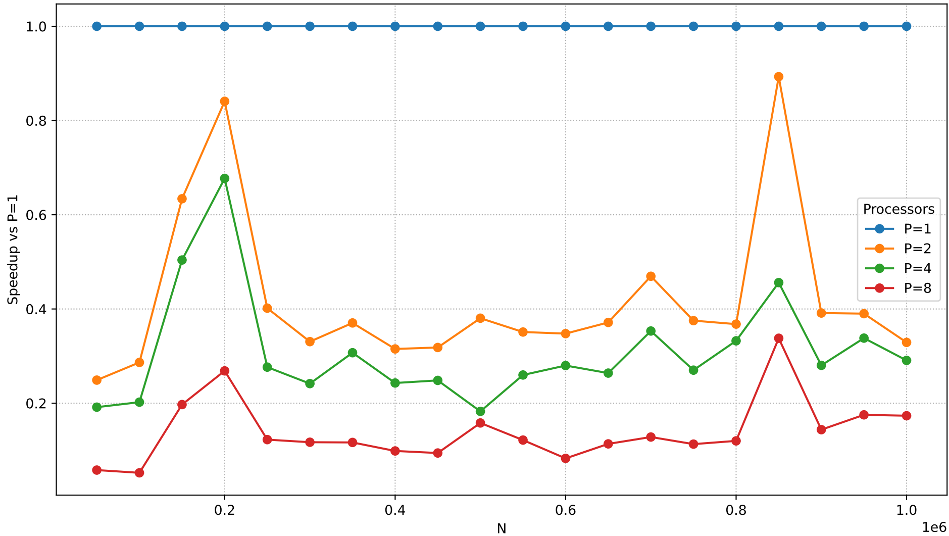
Speedup vs N (IMB=50)
