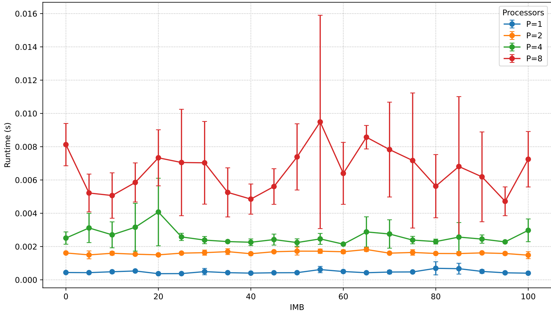
Runtime vs IMB (N=50,000)
