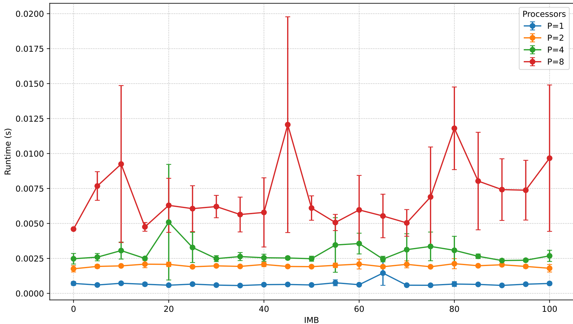
Runtime vs IMB (N=400,000)
