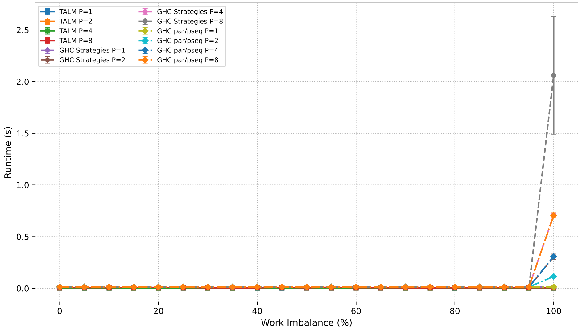
Dyck Path Validation: Runtime Comparison (N=500,000)
