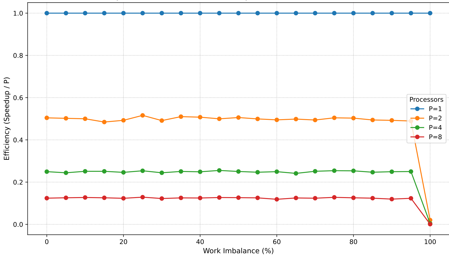
Dyck Path Validation: Parallel Efficiency vs Work Imbalance (N=450,000)
