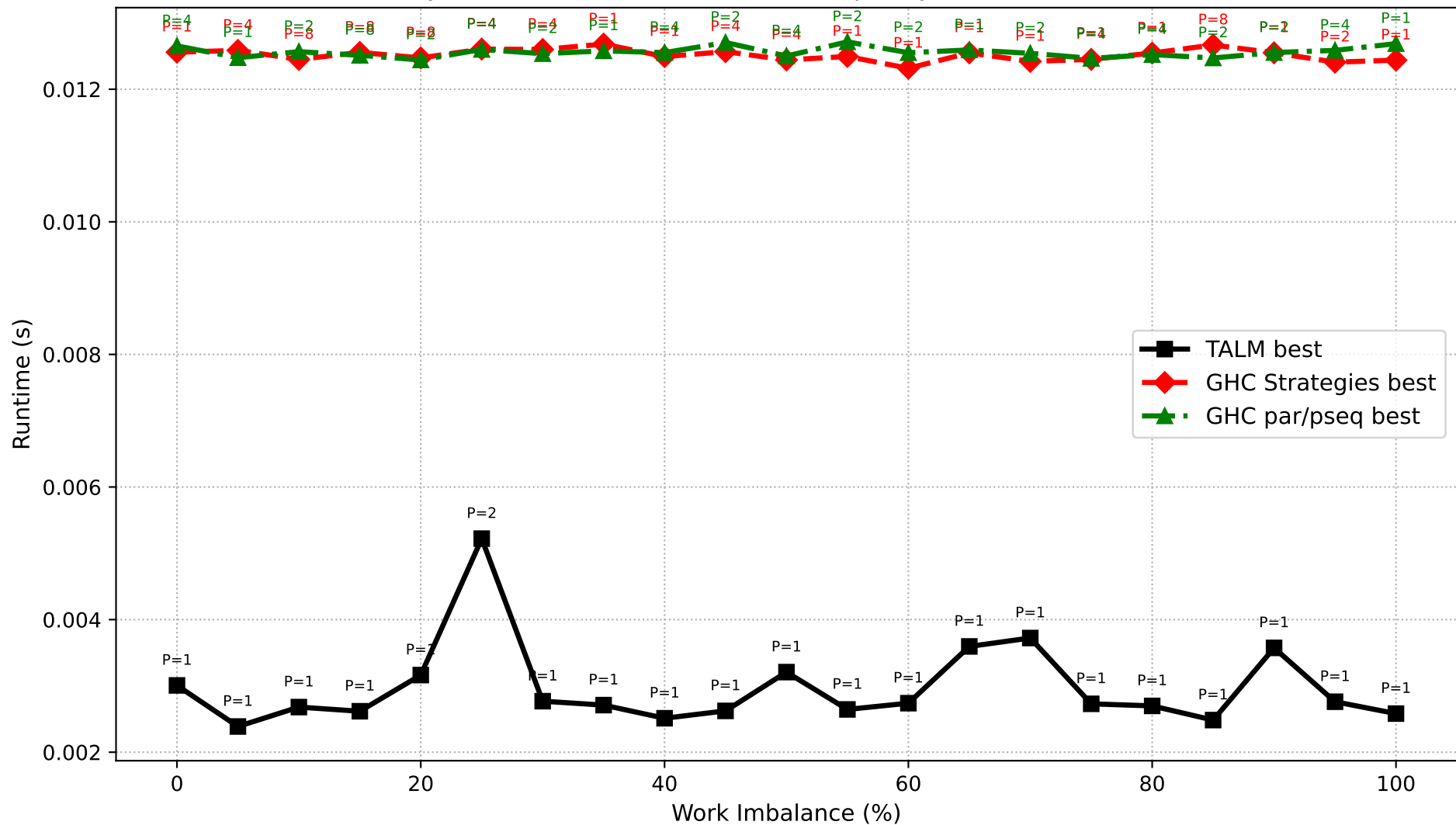
Dyck Path Validation: Best Runtime per System (N=700,000)
