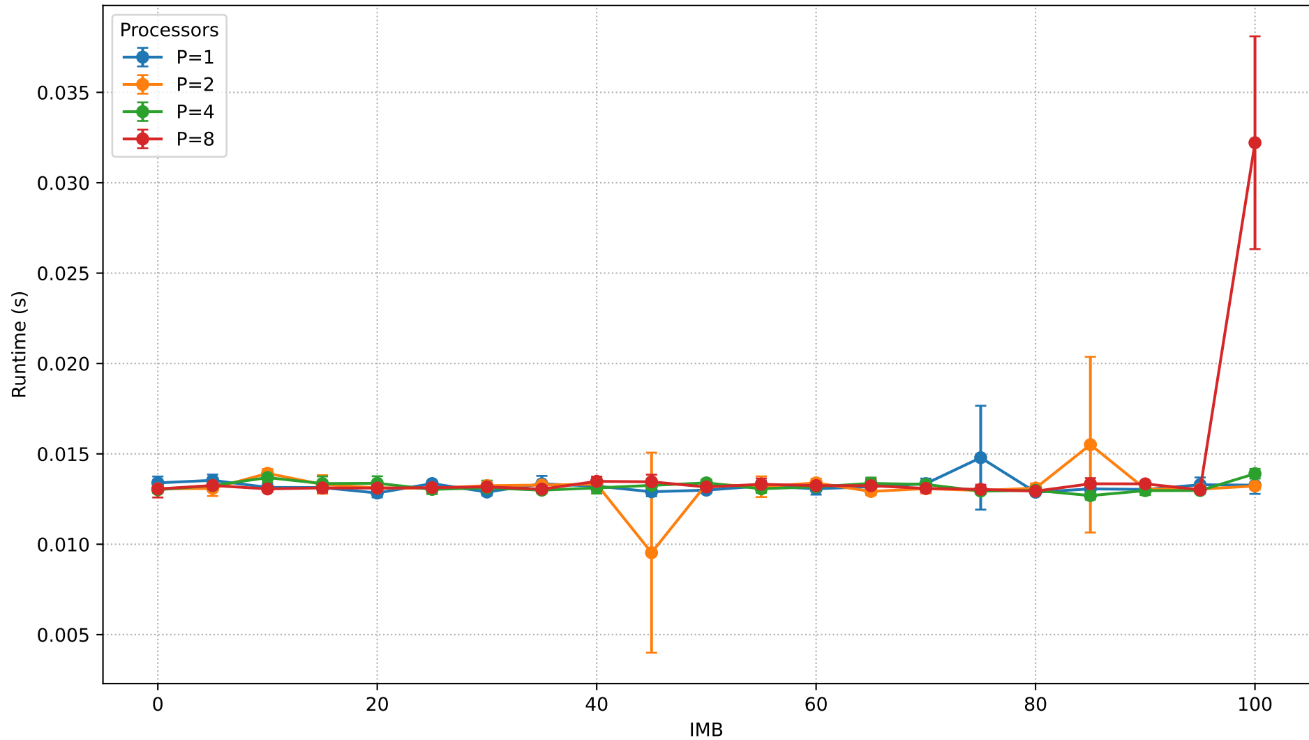
Runtime vs IMB (N=10000)
