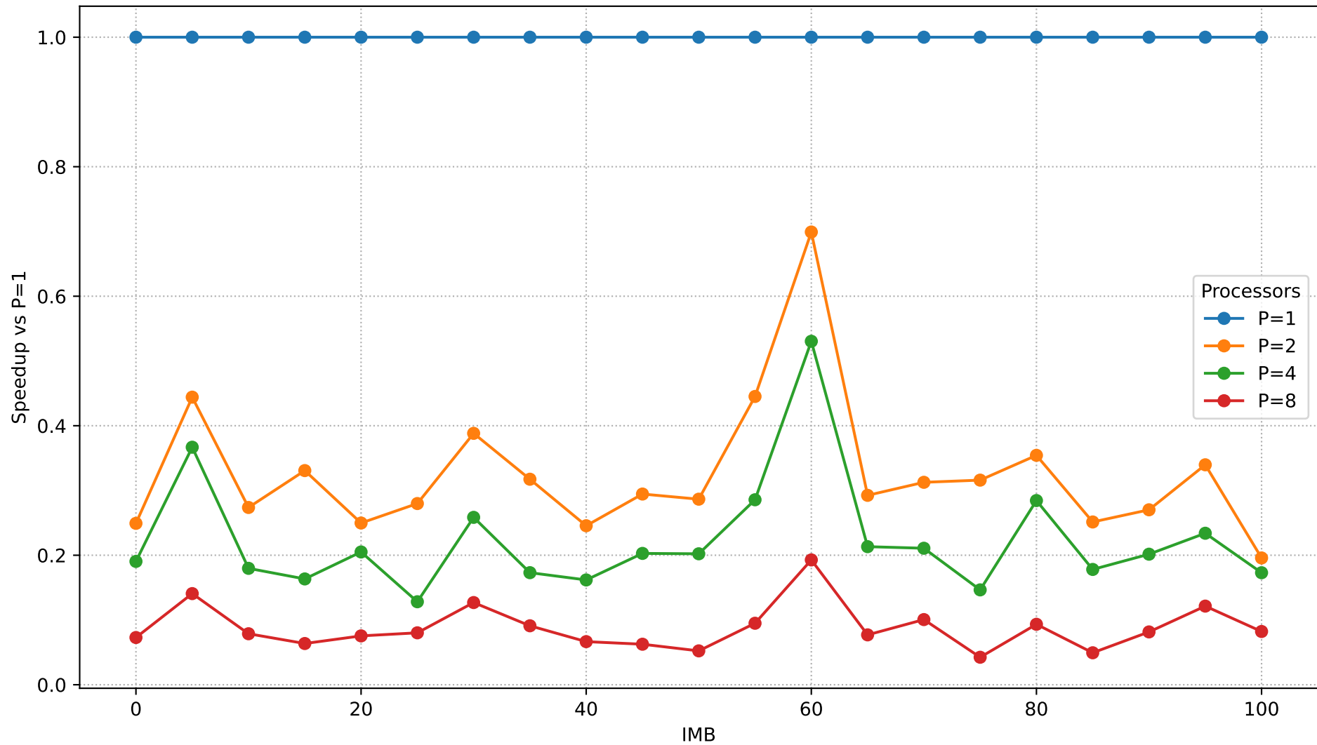
Speedup vs IMB (N=100,000)
