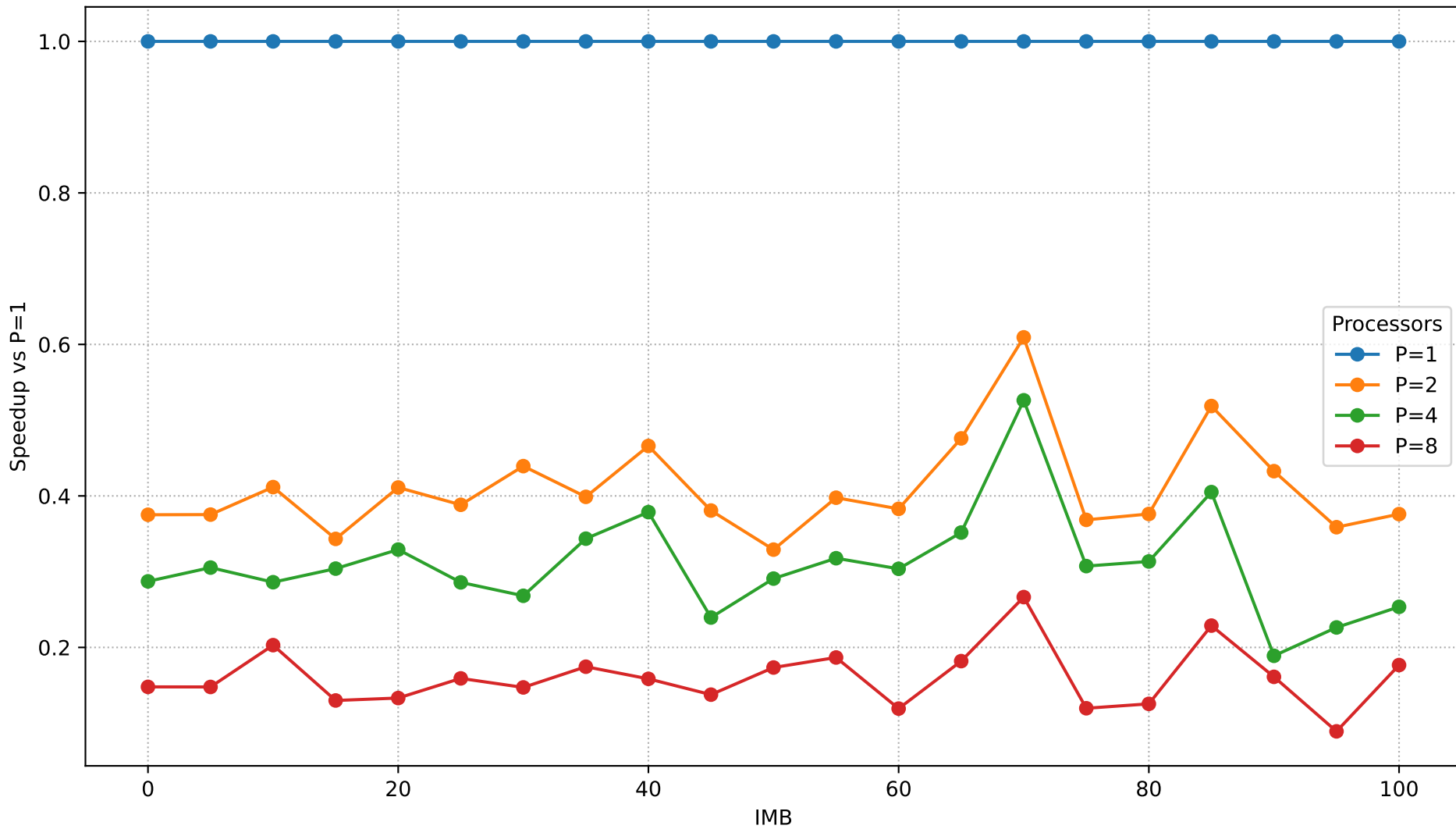
Speedup vs IMB (N=1,000,000)
