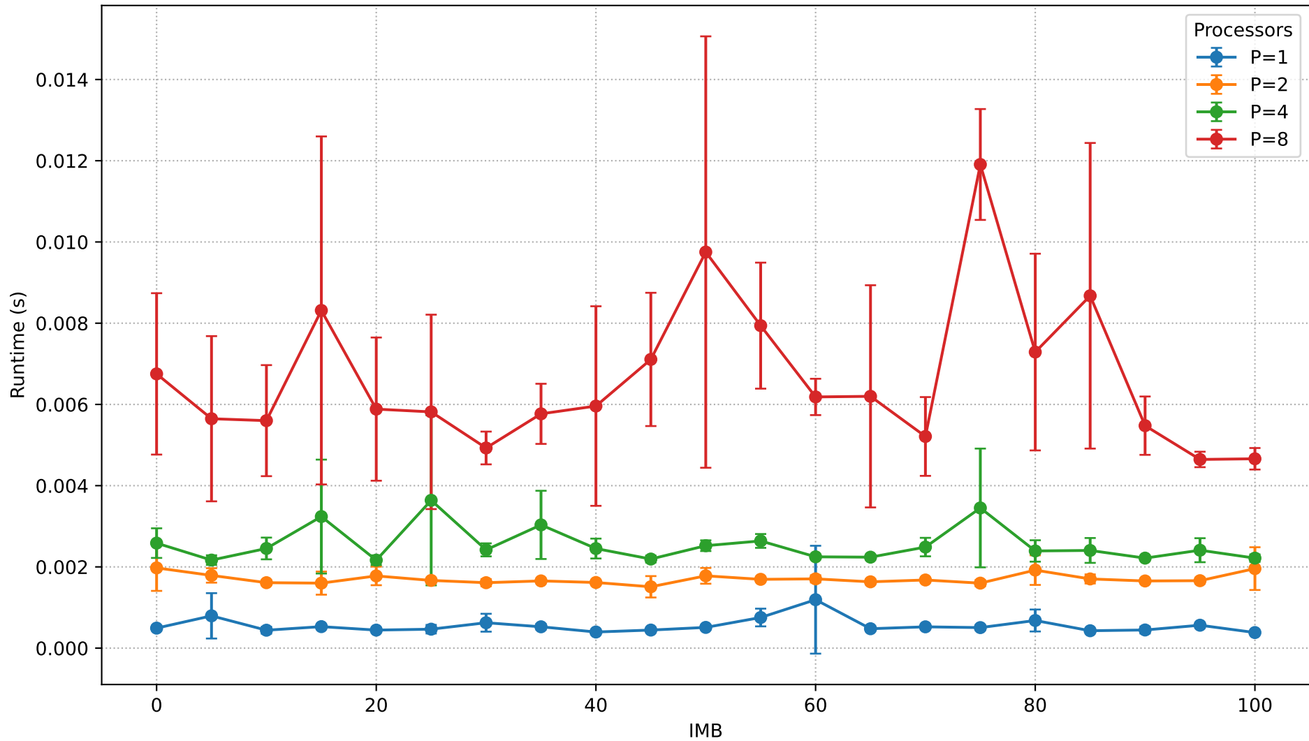
Runtime vs IMB (N=100,000)
