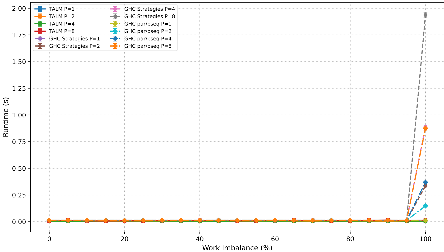
Dyck Path Validation: Runtime Comparison (N=650,000)
