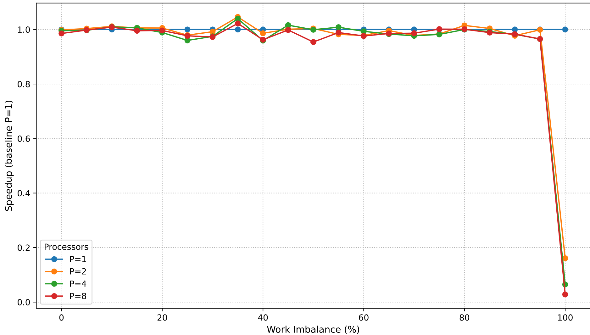
Dyck Path Validation: Speedup vs Work Imbalance (N=350,000)
