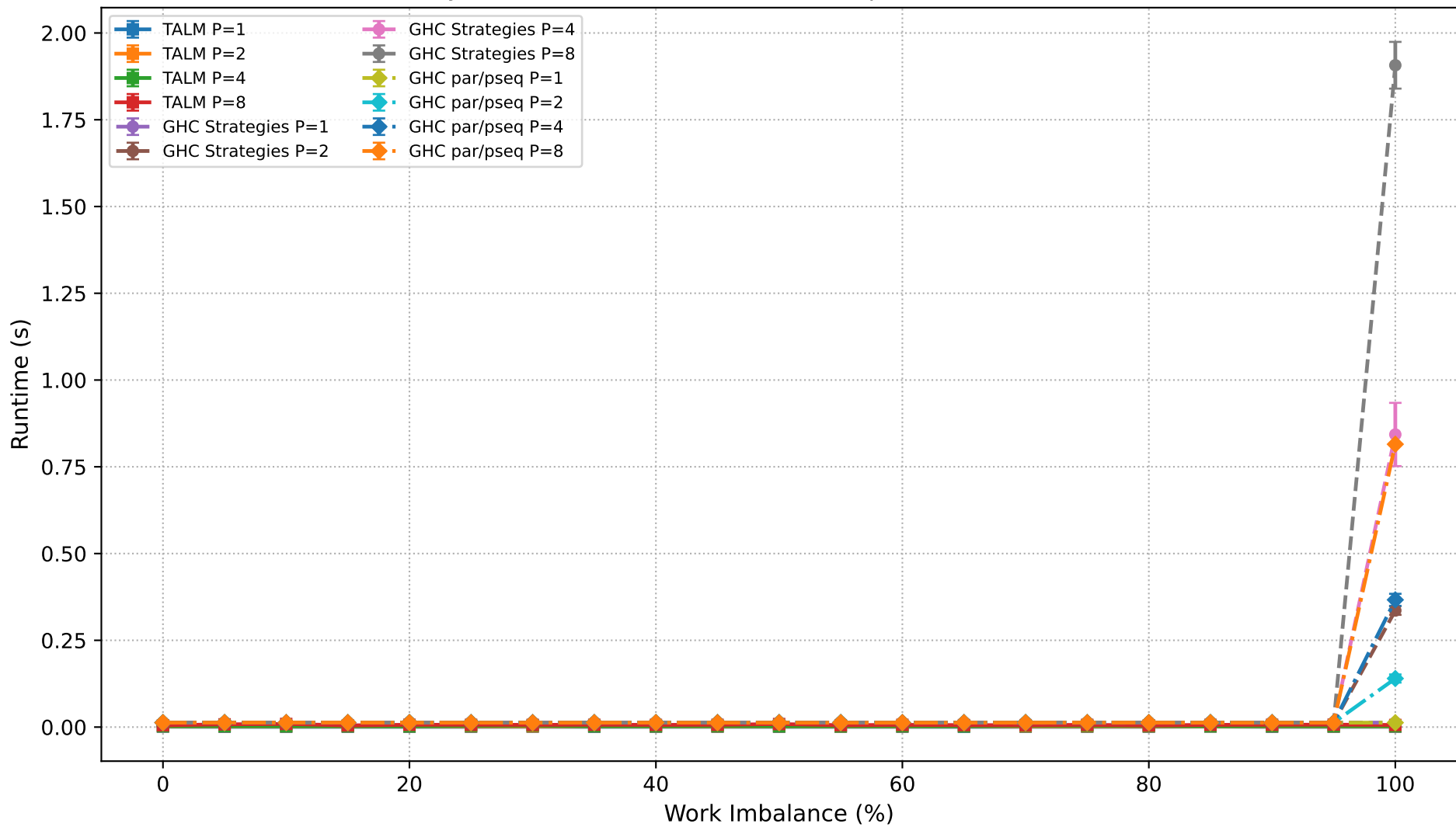
Dyck Path Validation: Runtime Comparison (N=600,000)
