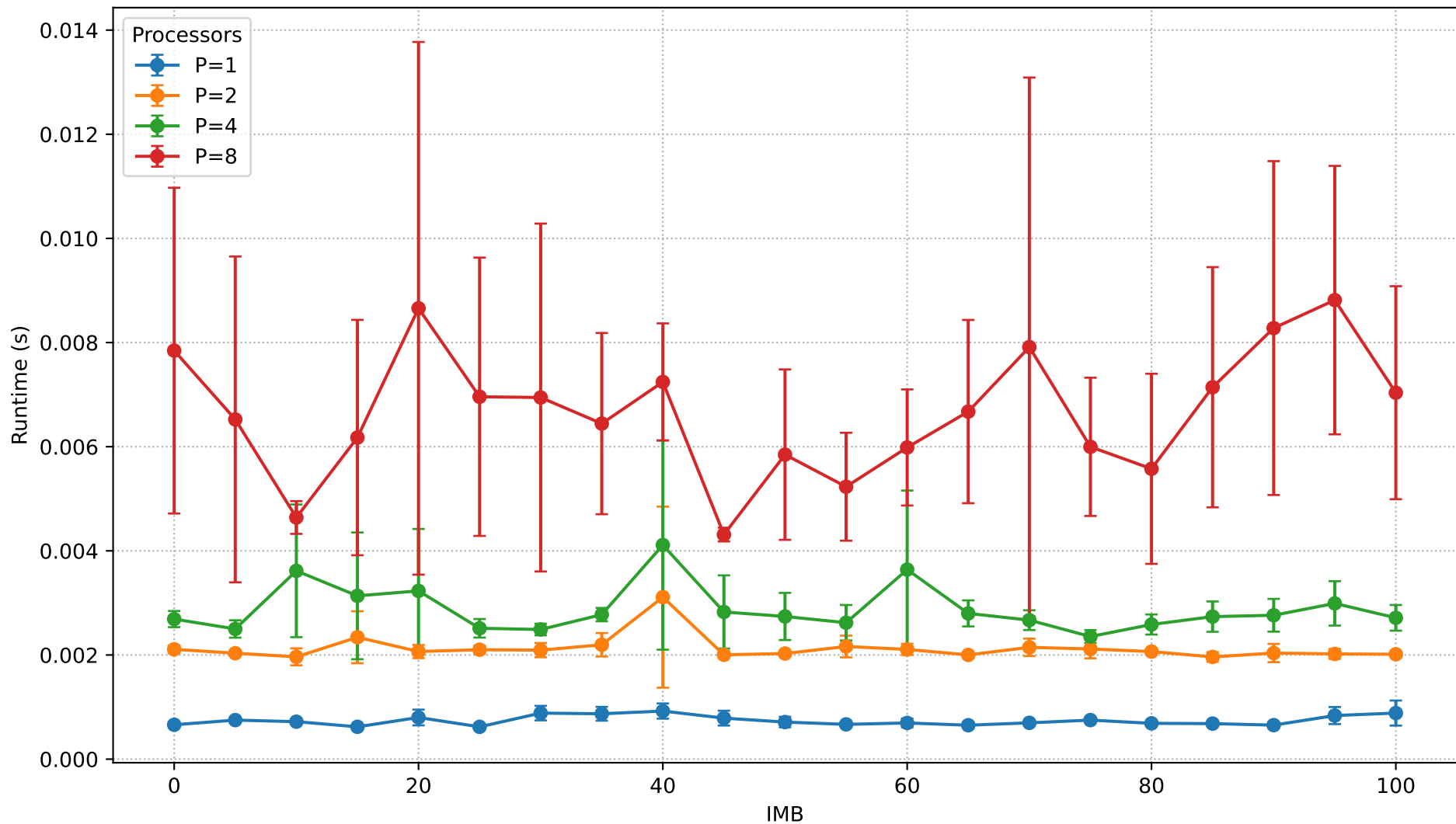
Runtime vs IMB (N=550,000)
