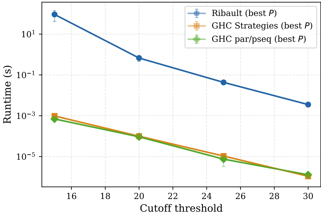
Fibonacci: Best Runtime vs. Cutoff
