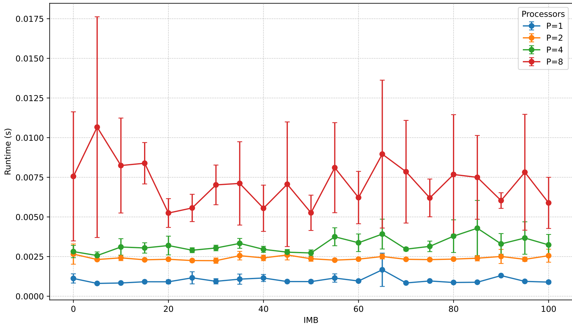
Runtime vs IMB (N=950,000)
