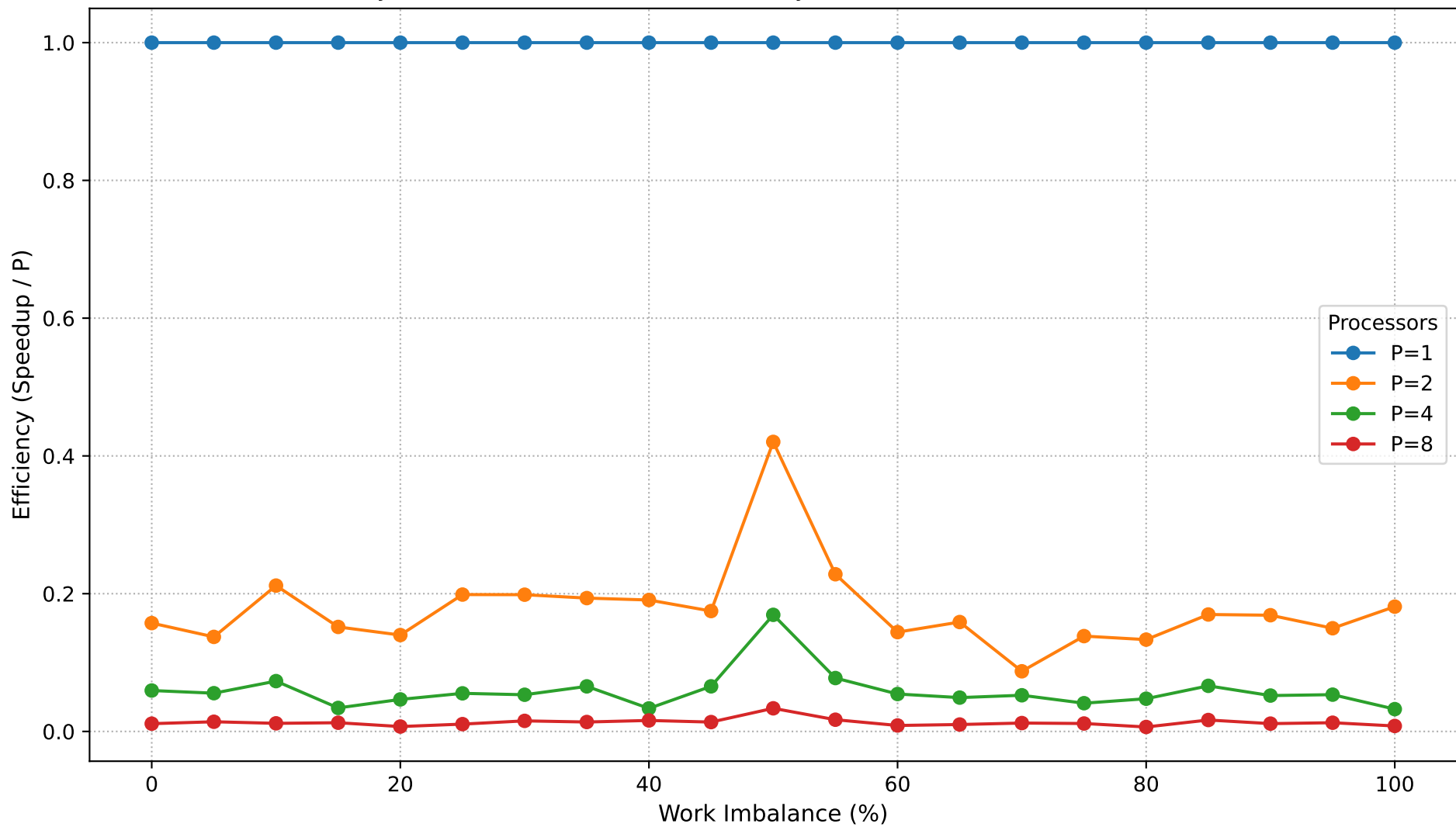
Dyck Path Validation: Parallel Efficiency vs Work Imbalance (N=200,000)
