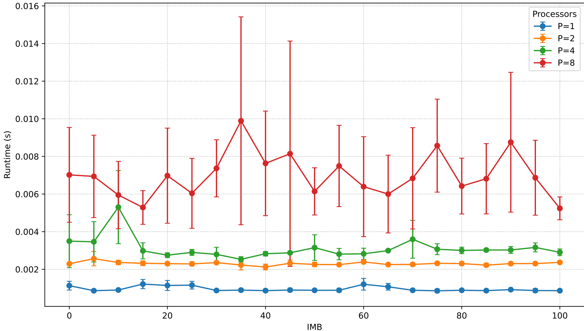
Runtime vs IMB (N=900,000)
