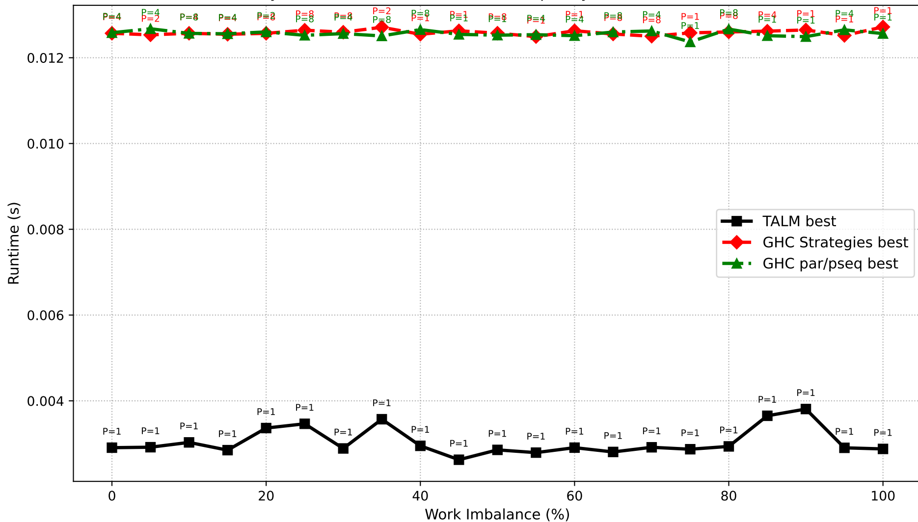
Dyck Path Validation: Best Runtime per System (N=950,000)
