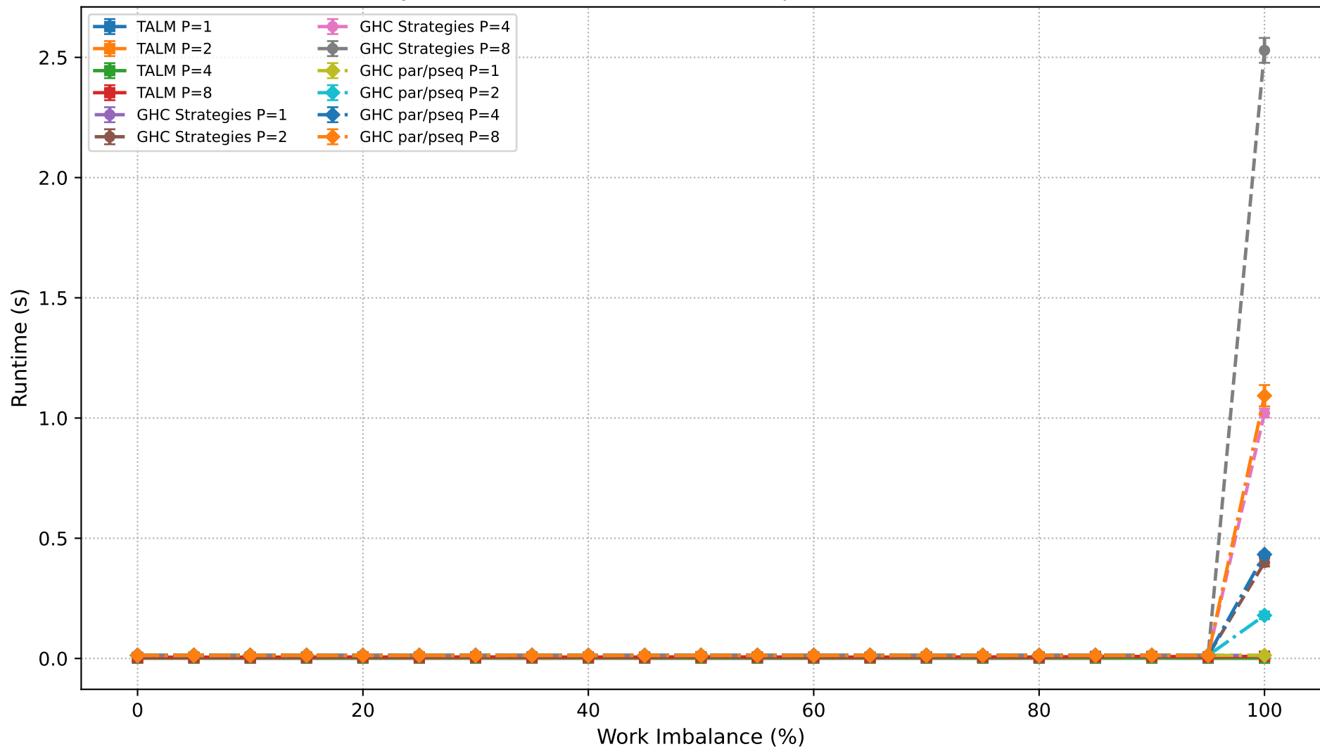
Dyck Path Validation: Runtime Comparison (N=750,000)
