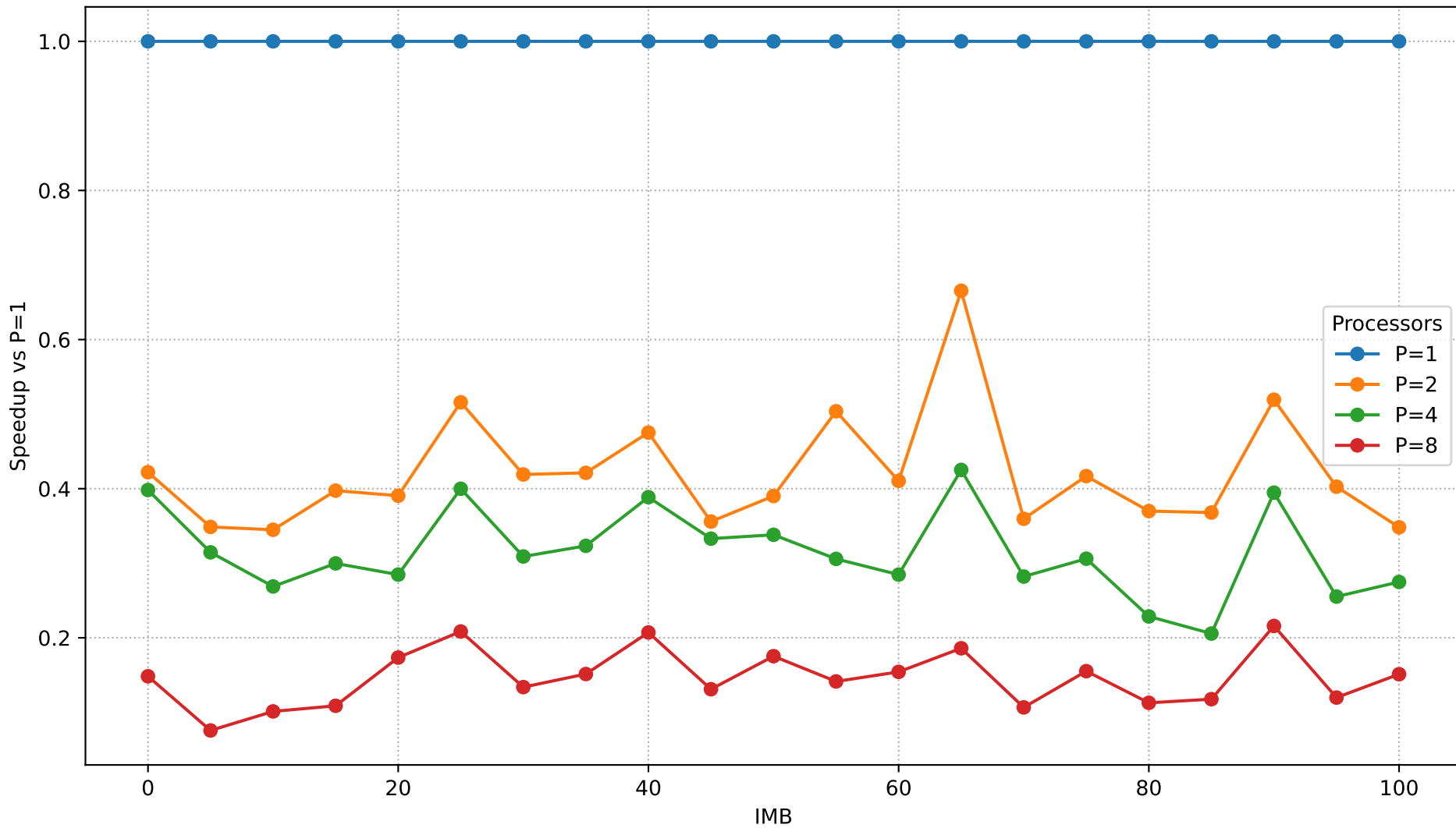
Speedup vs IMB (N=950,000)
