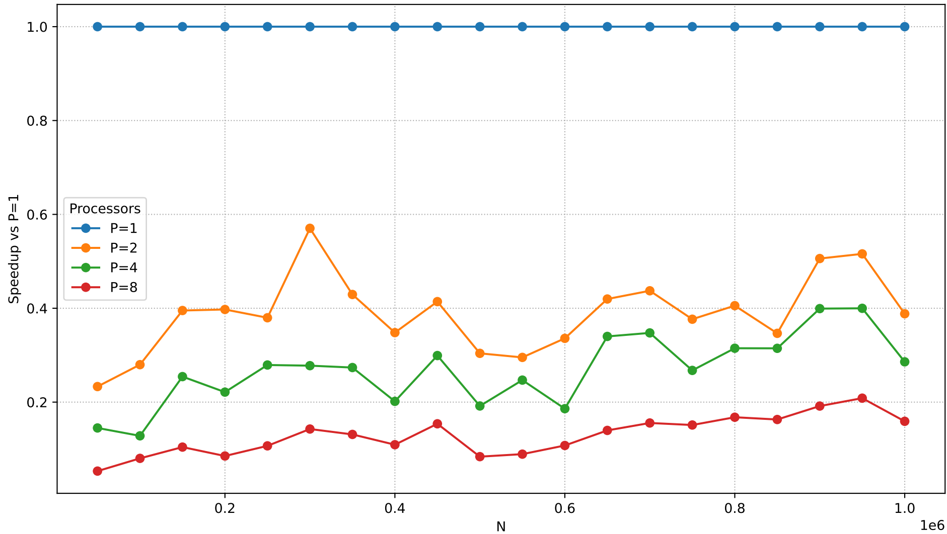
Speedup vs N (IMB=25)
