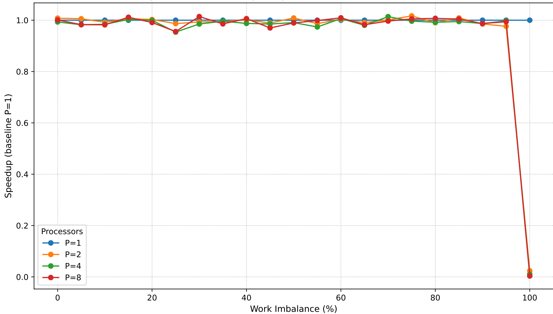
Dyck Path Validation: Speedup vs Work Imbalance (N=850,000)
