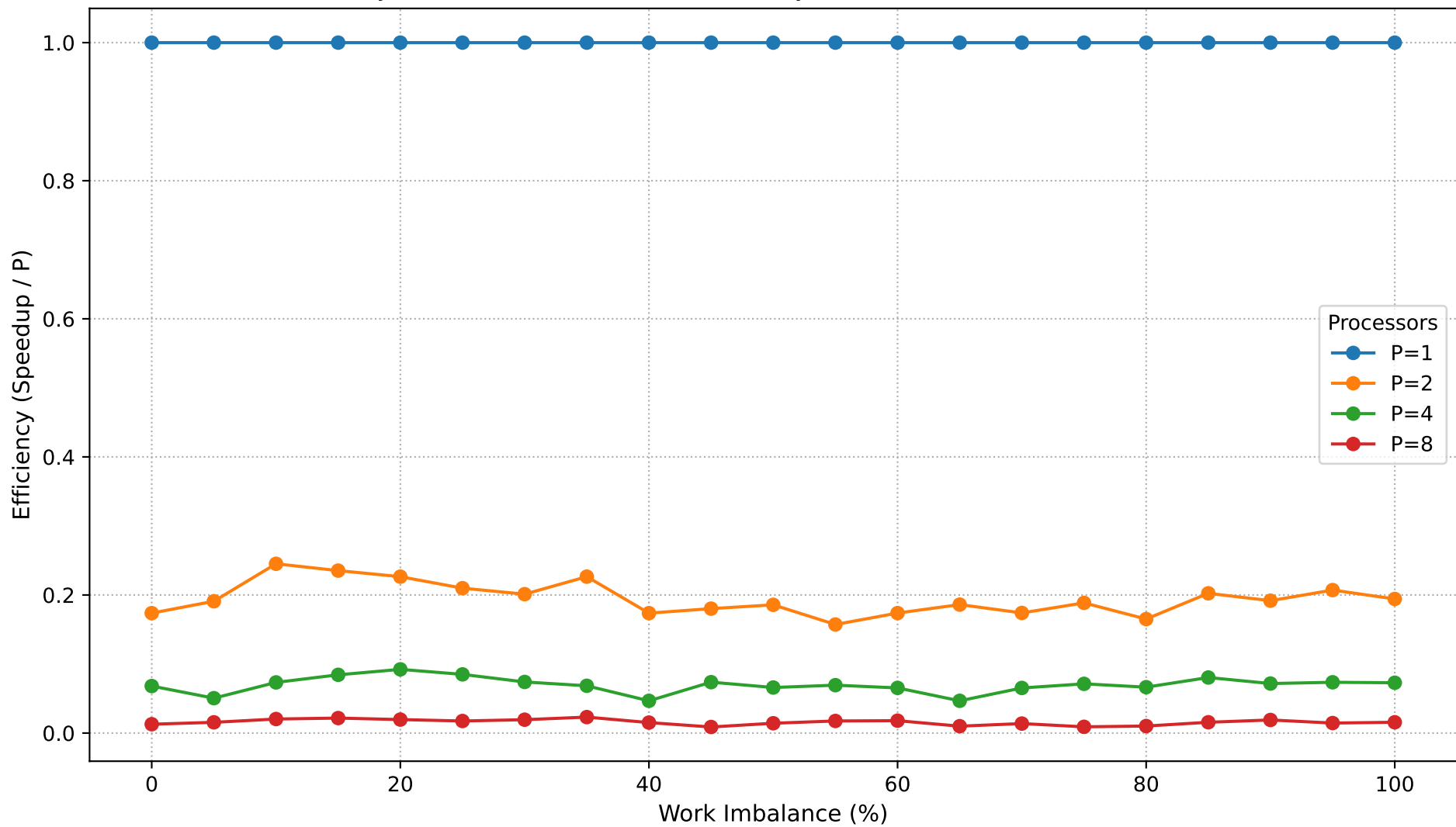
Dyck Path Validation: Parallel Efficiency vs Work Imbalance (N=650,000)
