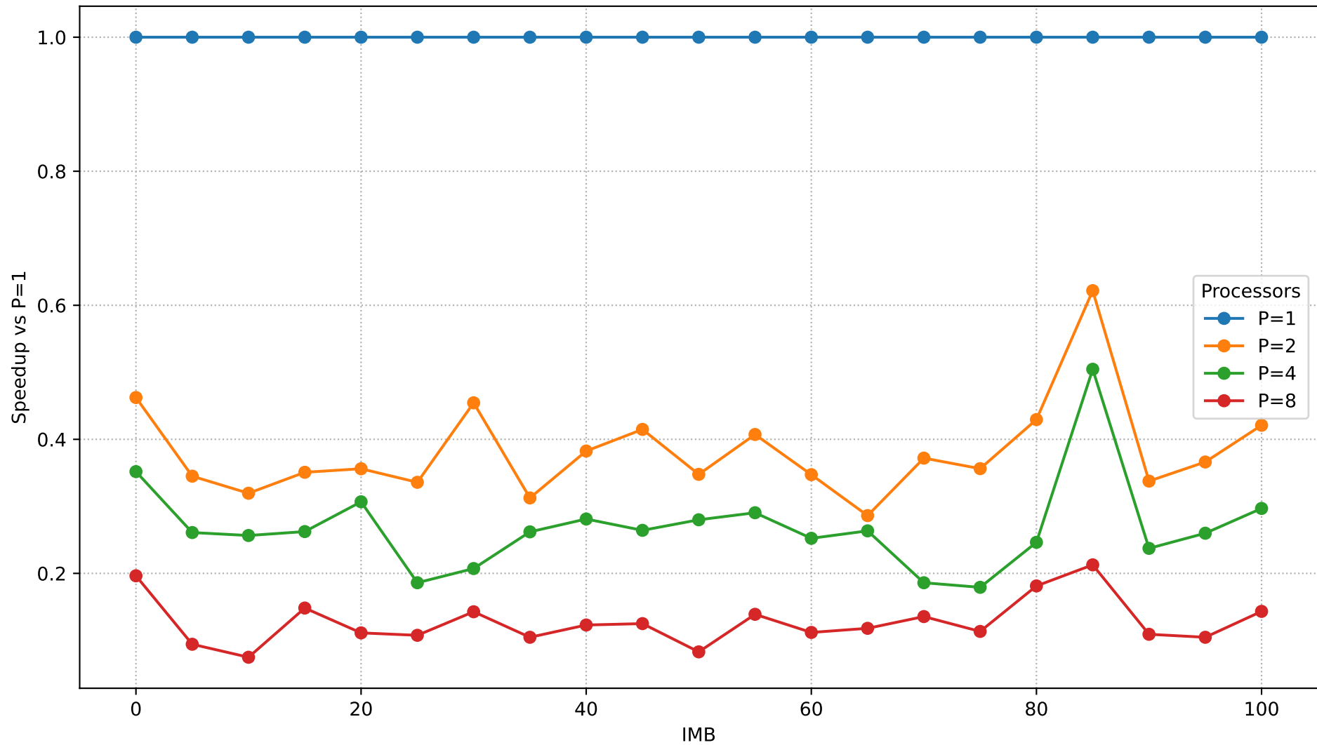
Speedup vs IMB (N=600,000)
