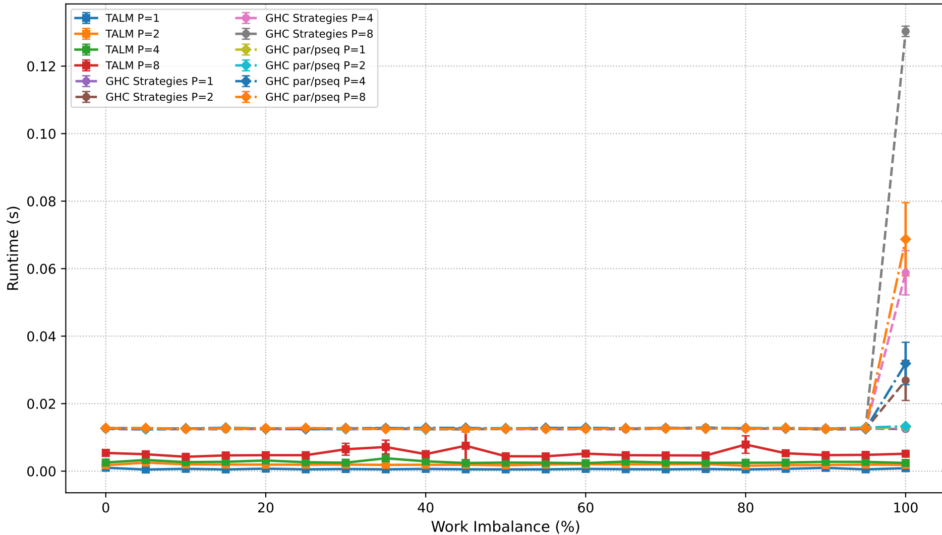
Dyck Path Validation: Runtime Comparison (N=50,000)
