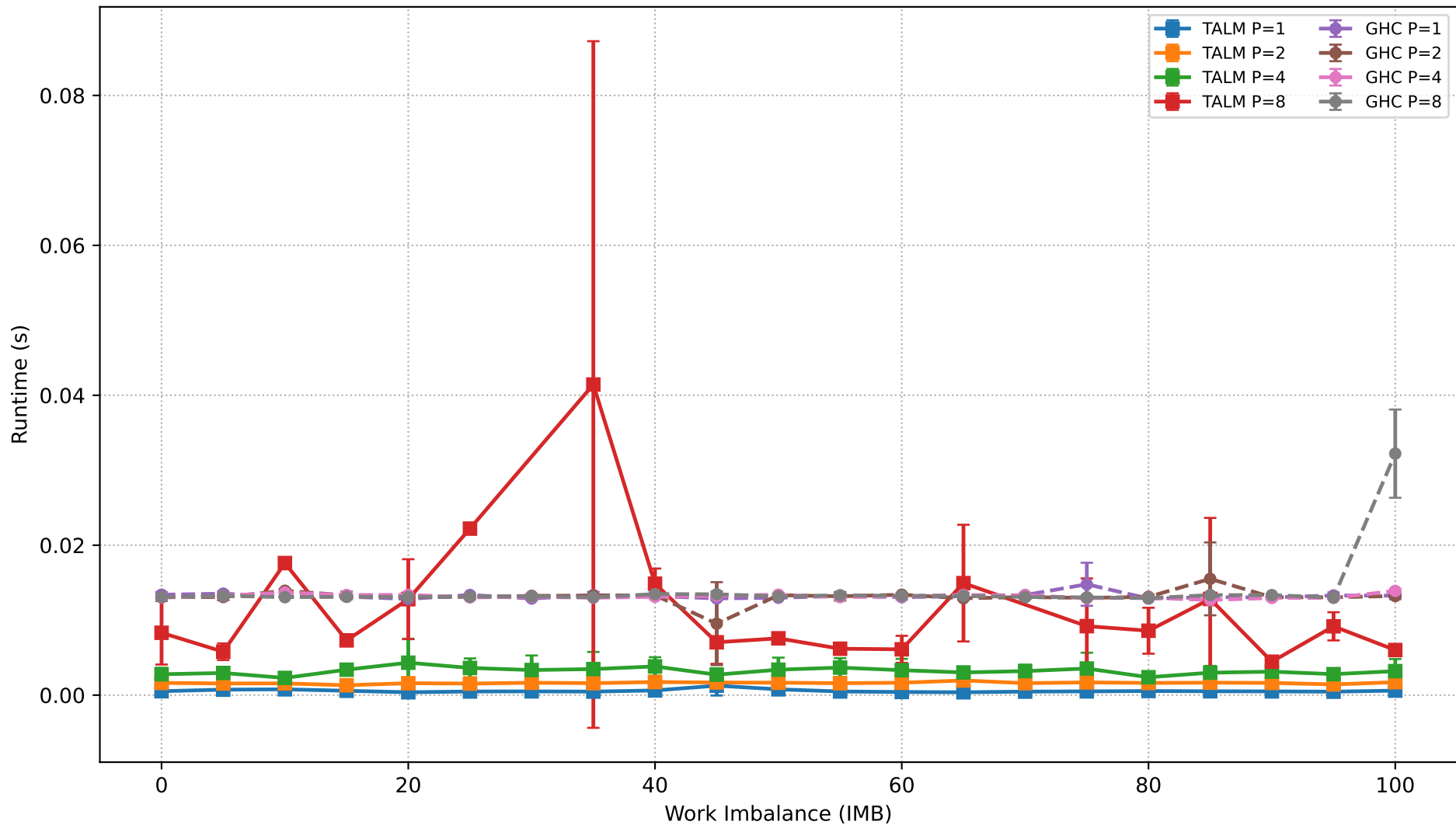
TALM vs GHC - Runtime (N=10000)
