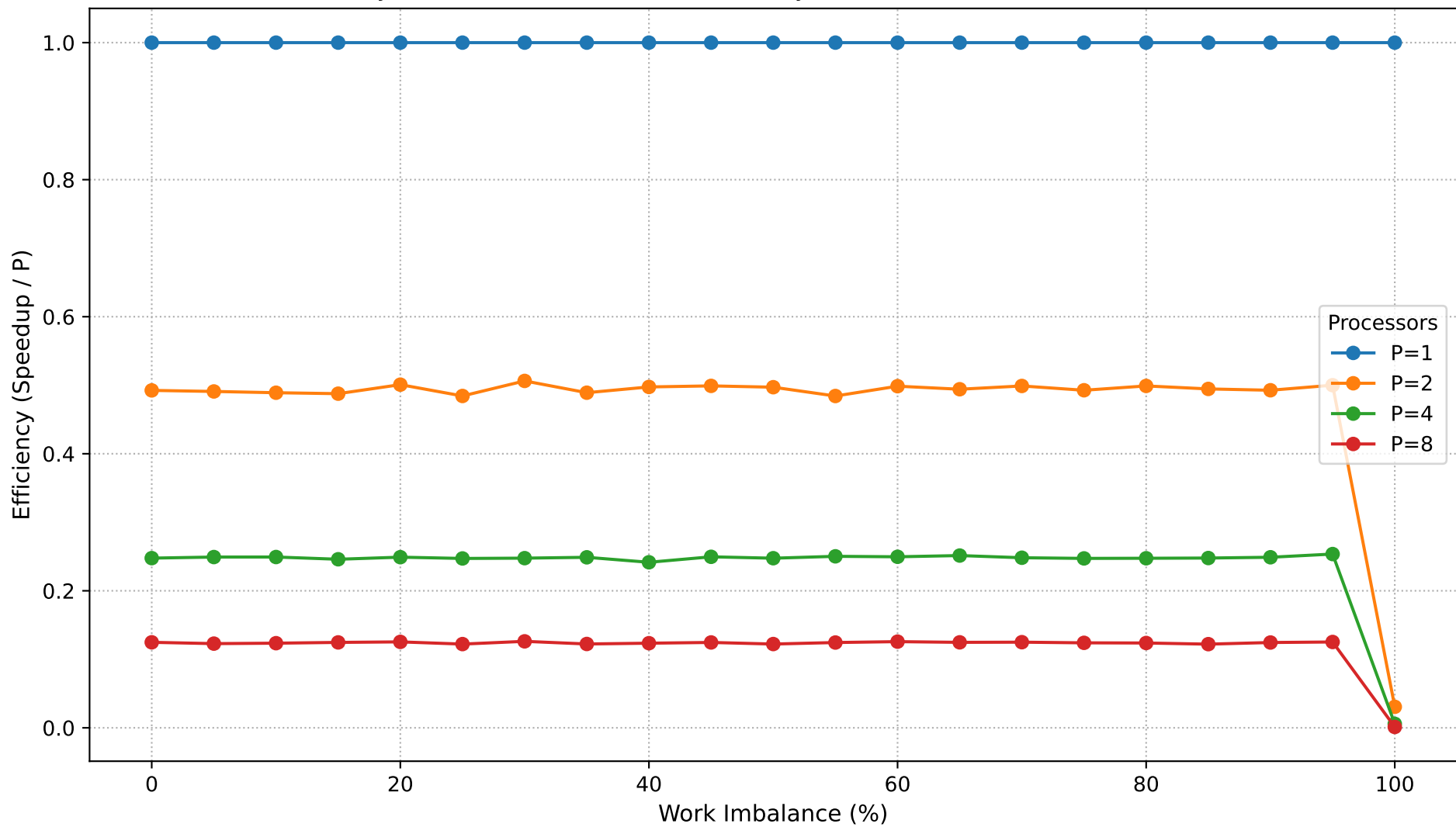
Dyck Path Validation: Parallel Efficiency vs Work Imbalance (N=900,000)
