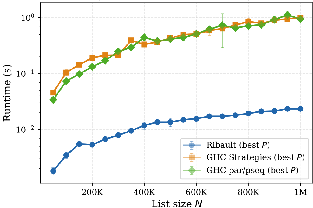
Merge Sort: Best Runtime per System
