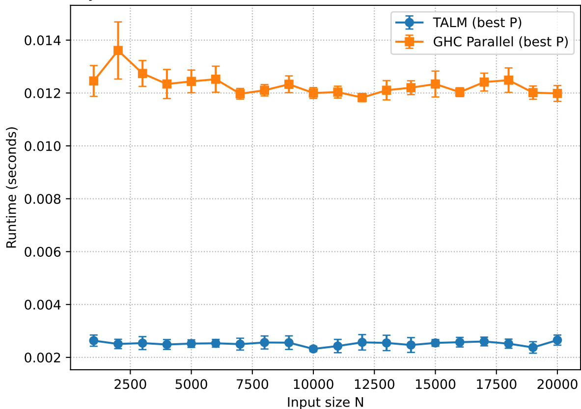
Dyck Path: Best-of-Breed Runtime vs N (imb=75, delta=-1000)
