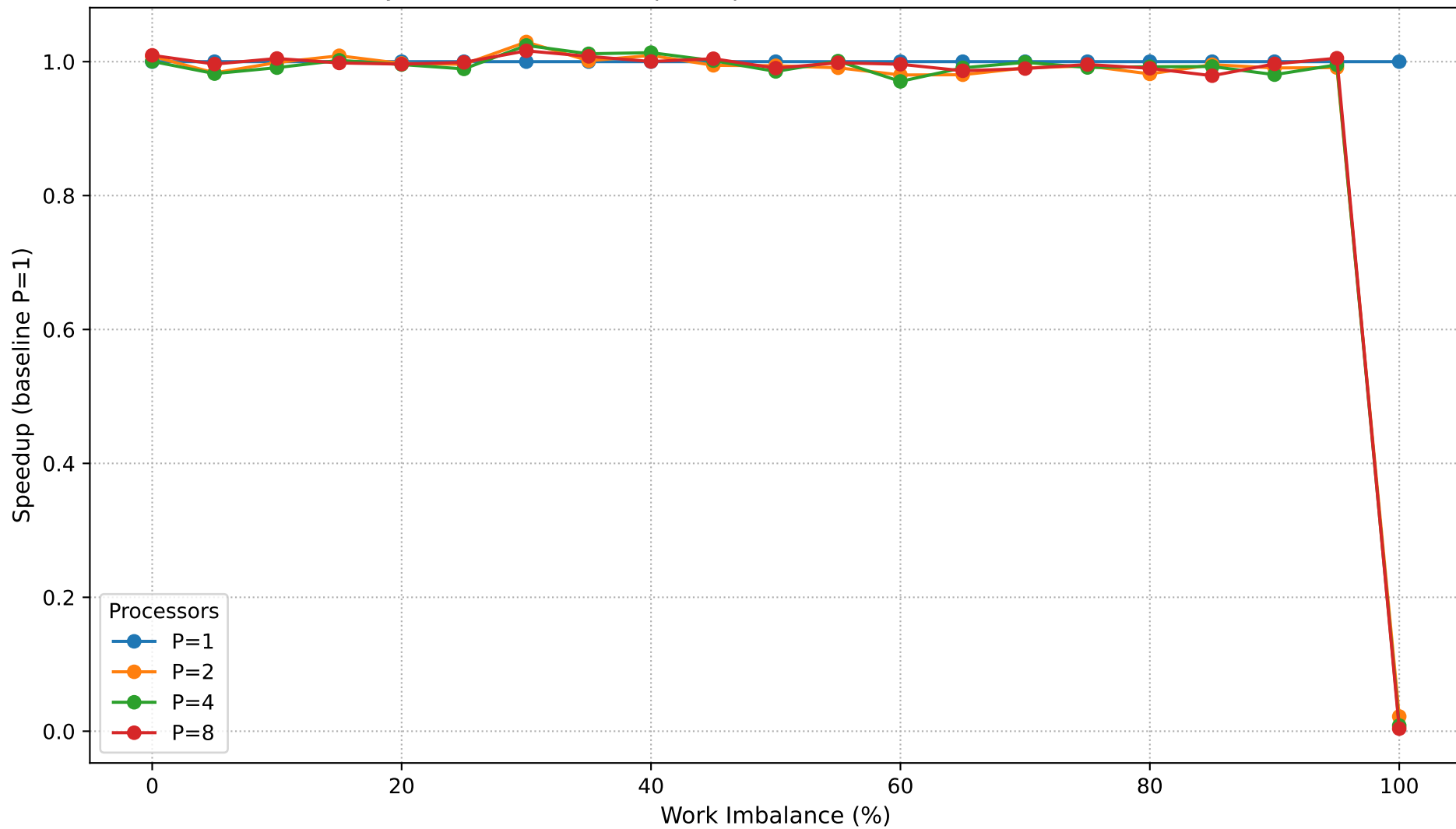
Dyck Path Validation: Speedup vs Work Imbalance (N=1,000,000)
