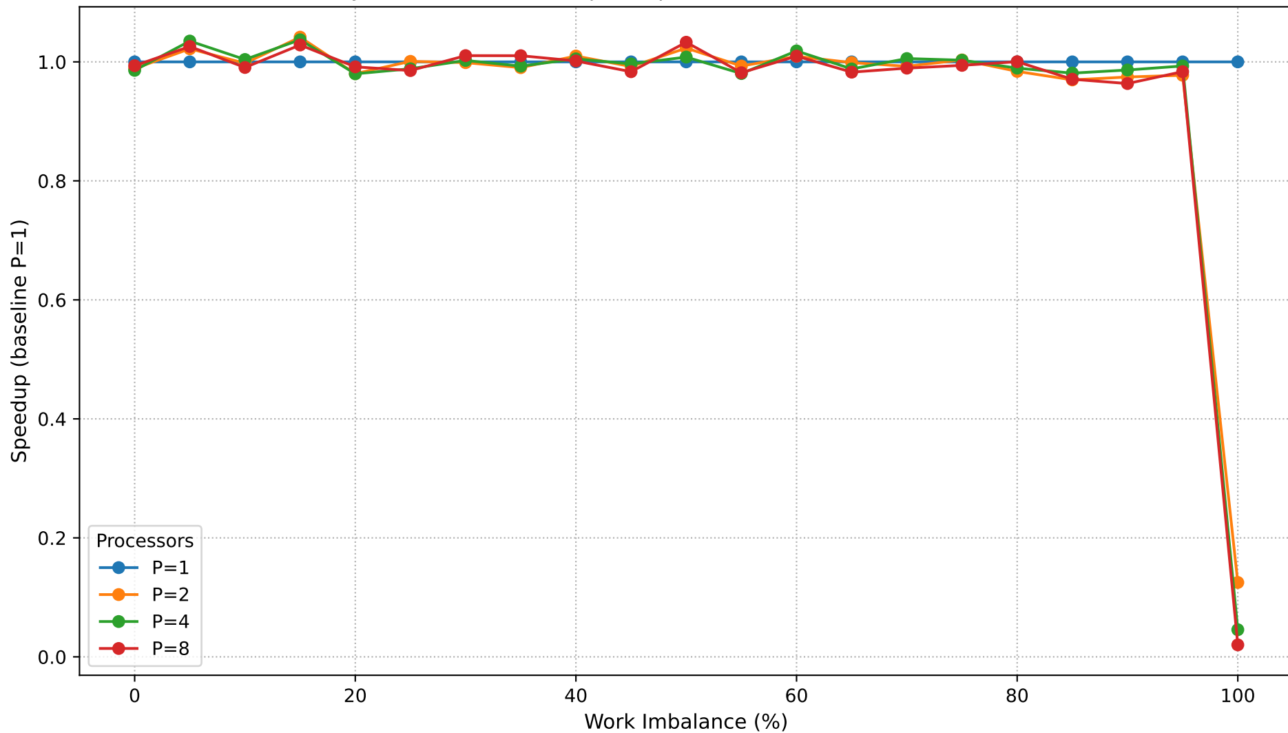
Dyck Path Validation: Speedup vs Work Imbalance (N=450,000)
