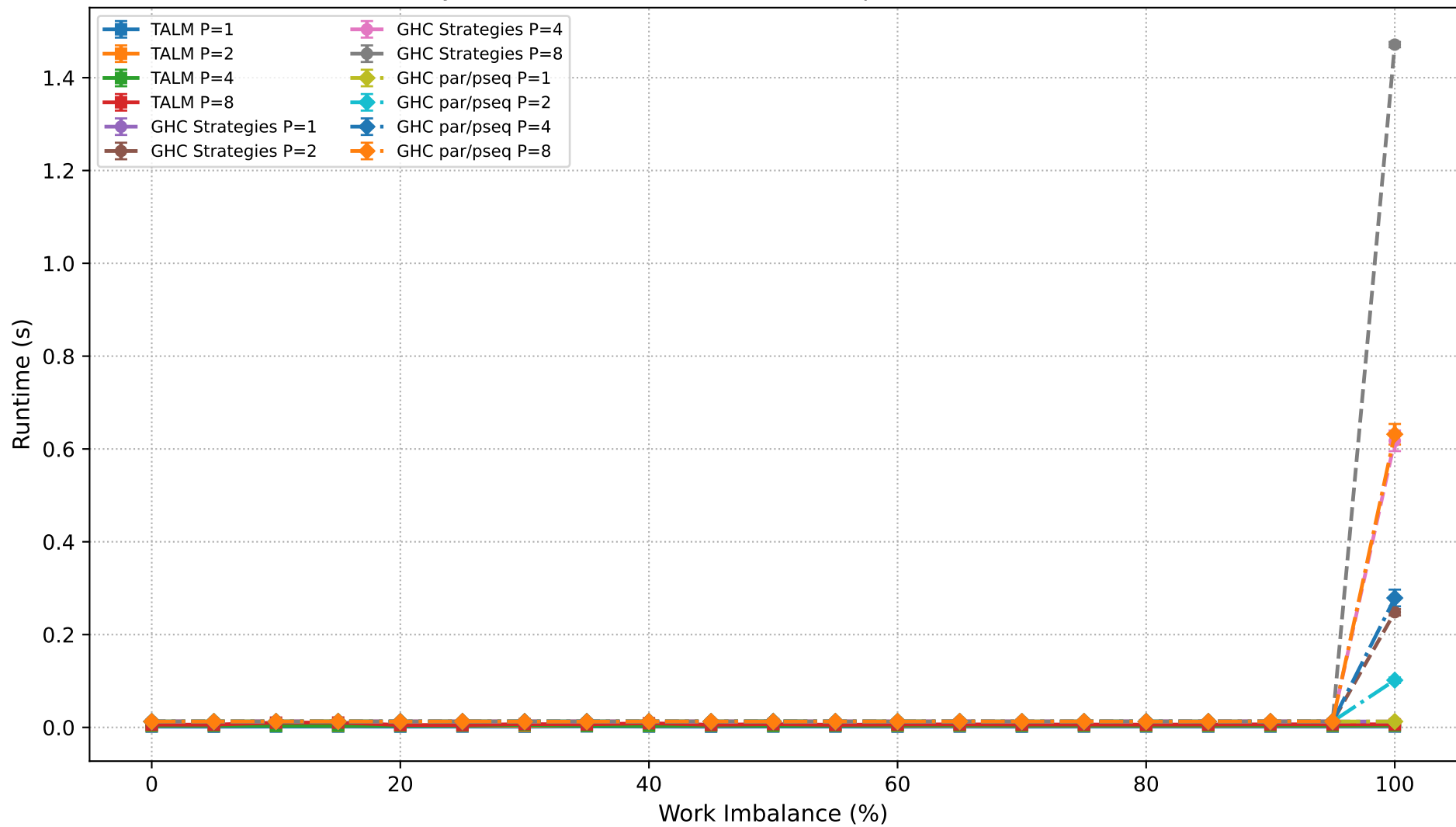
Dyck Path Validation: Runtime Comparison (N=450,000)
