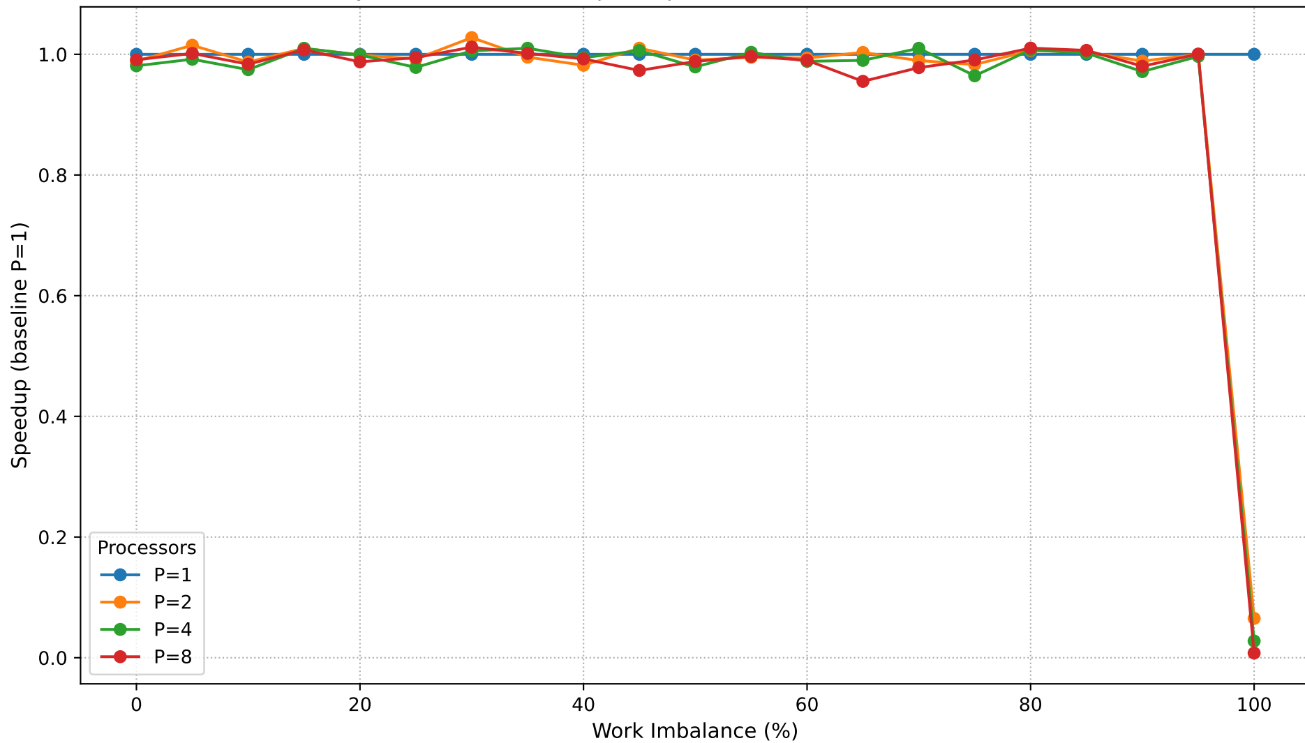
Dyck Path Validation: Speedup vs Work Imbalance (N=800,000)
