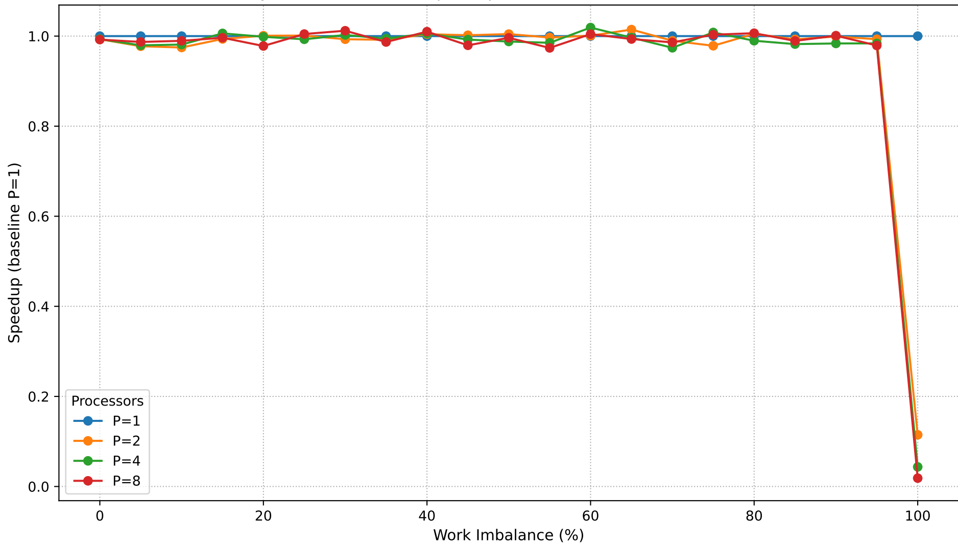
Dyck Path Validation: Speedup vs Work Imbalance (N=500,000)
