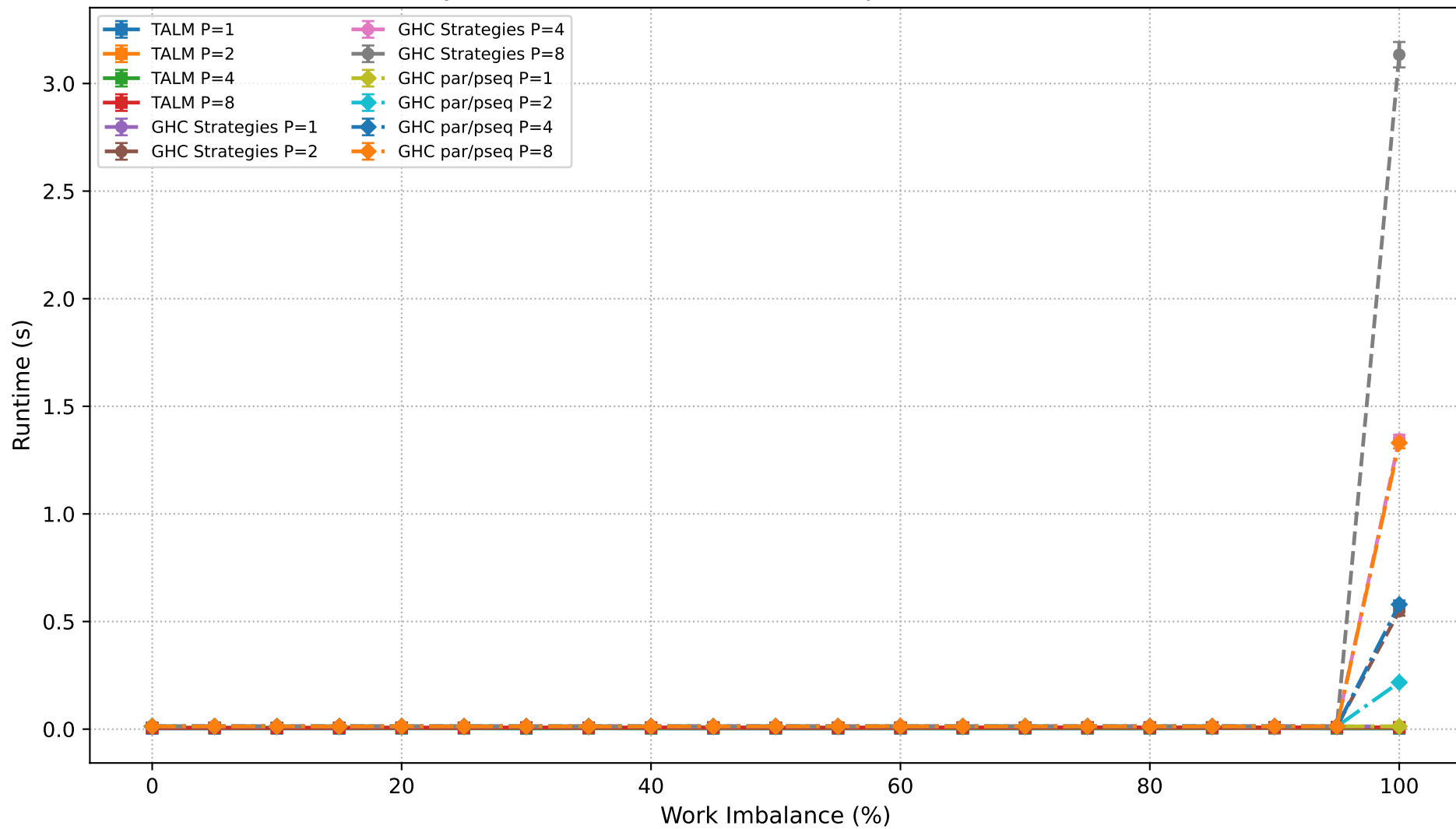
Dyck Path Validation: Runtime Comparison (N=950,000)
