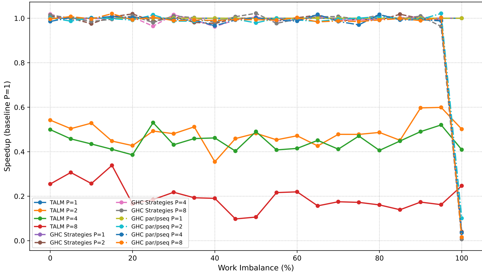
Dyck Path Validation: Speedup Comparison (N=600,000)
