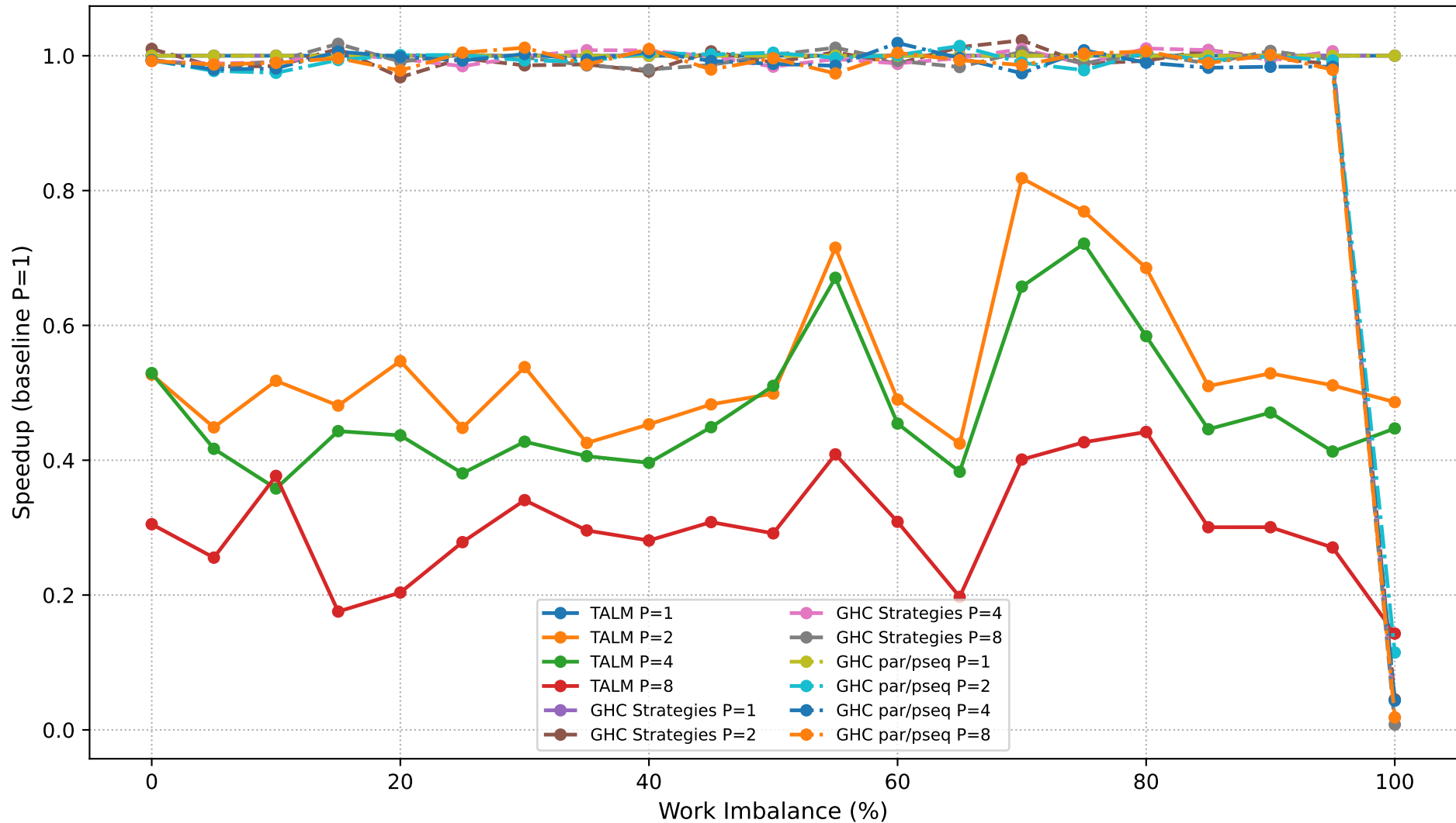
Dyck Path Validation: Speedup Comparison (N=500,000)
