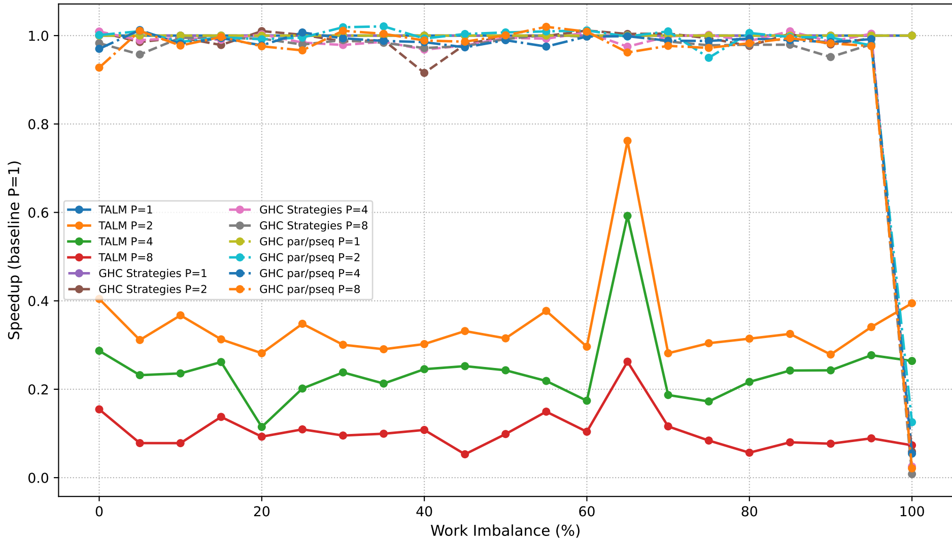
Dyck Path Validation: Speedup Comparison (N=400,000)
