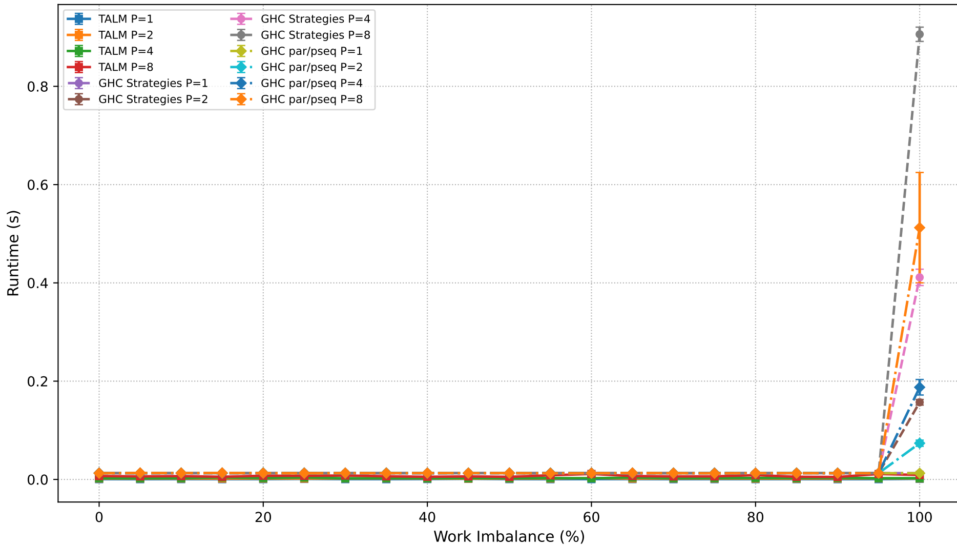
Dyck Path Validation: Runtime Comparison (N=300,000)
