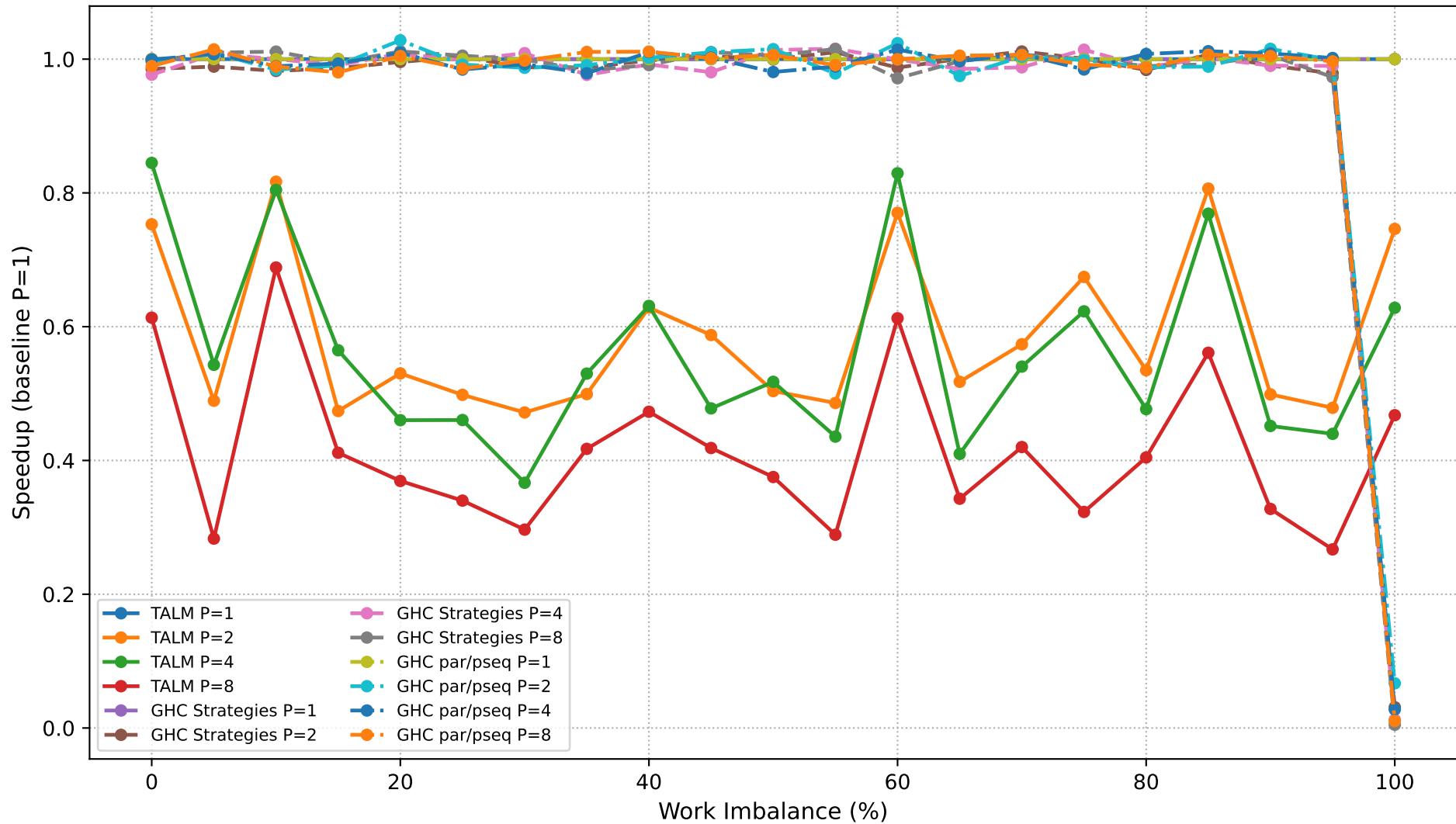
Dyck Path Validation: Speedup Comparison (N=800,000)
