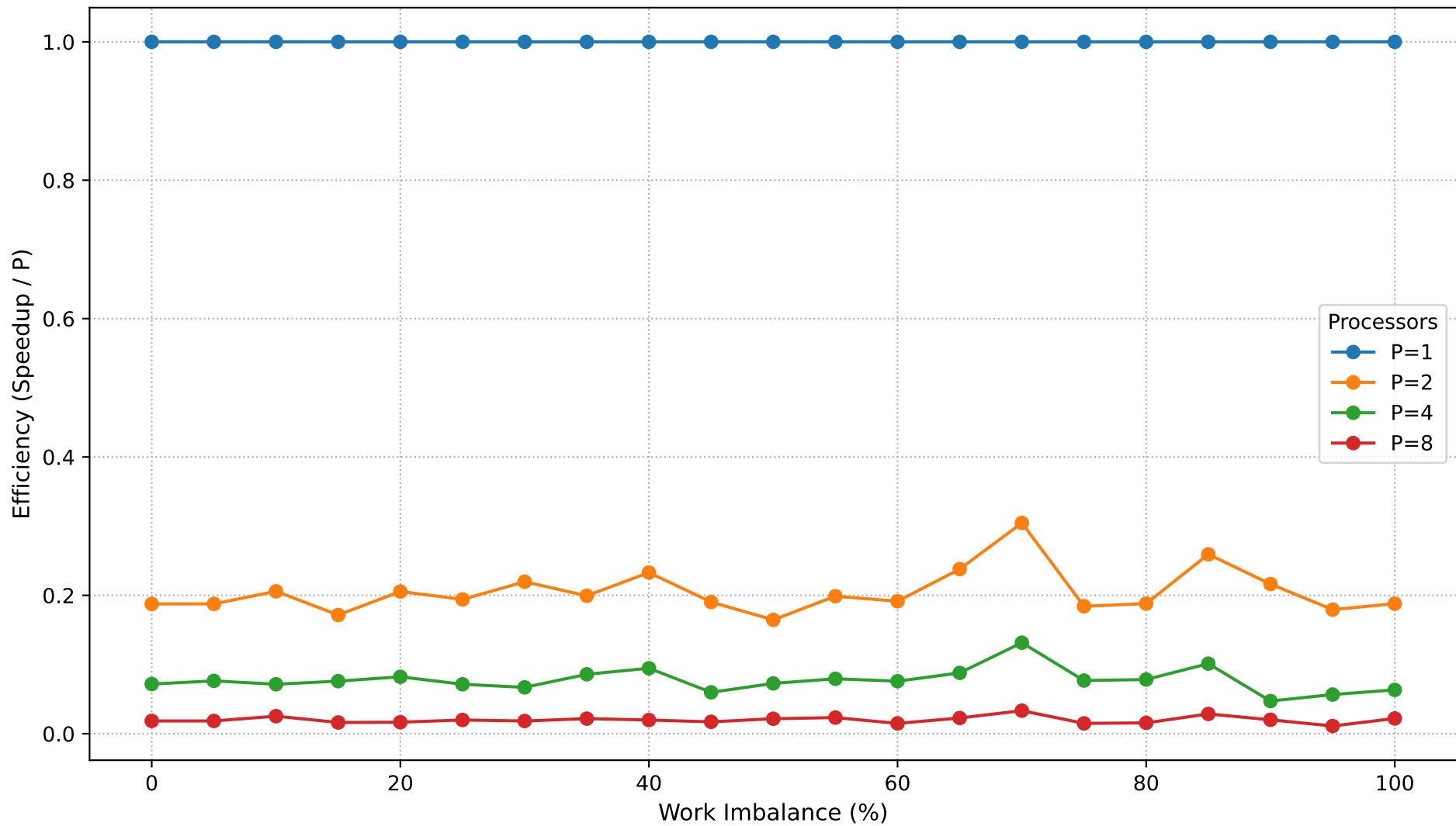
Dyck Path Validation: Parallel Efficiency vs Work Imbalance (N=1,000,000)
