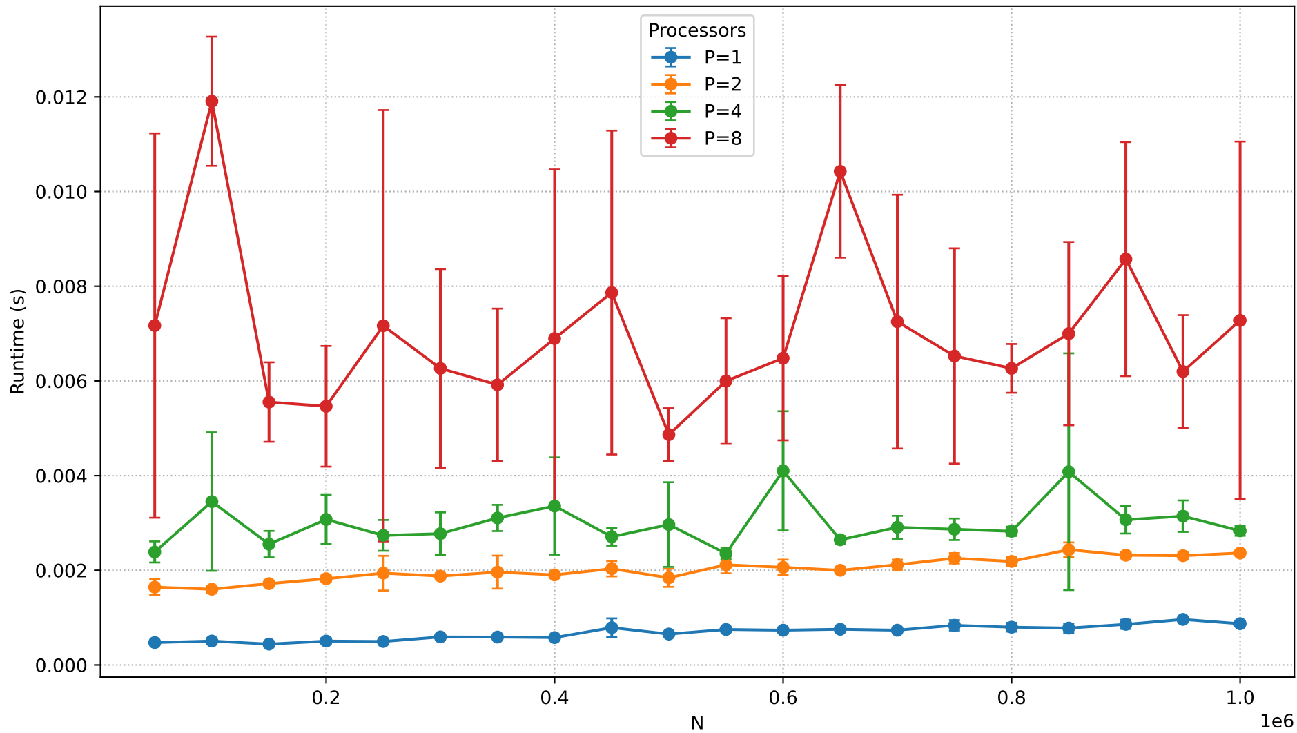
Runtime vs N (IMB=75)
