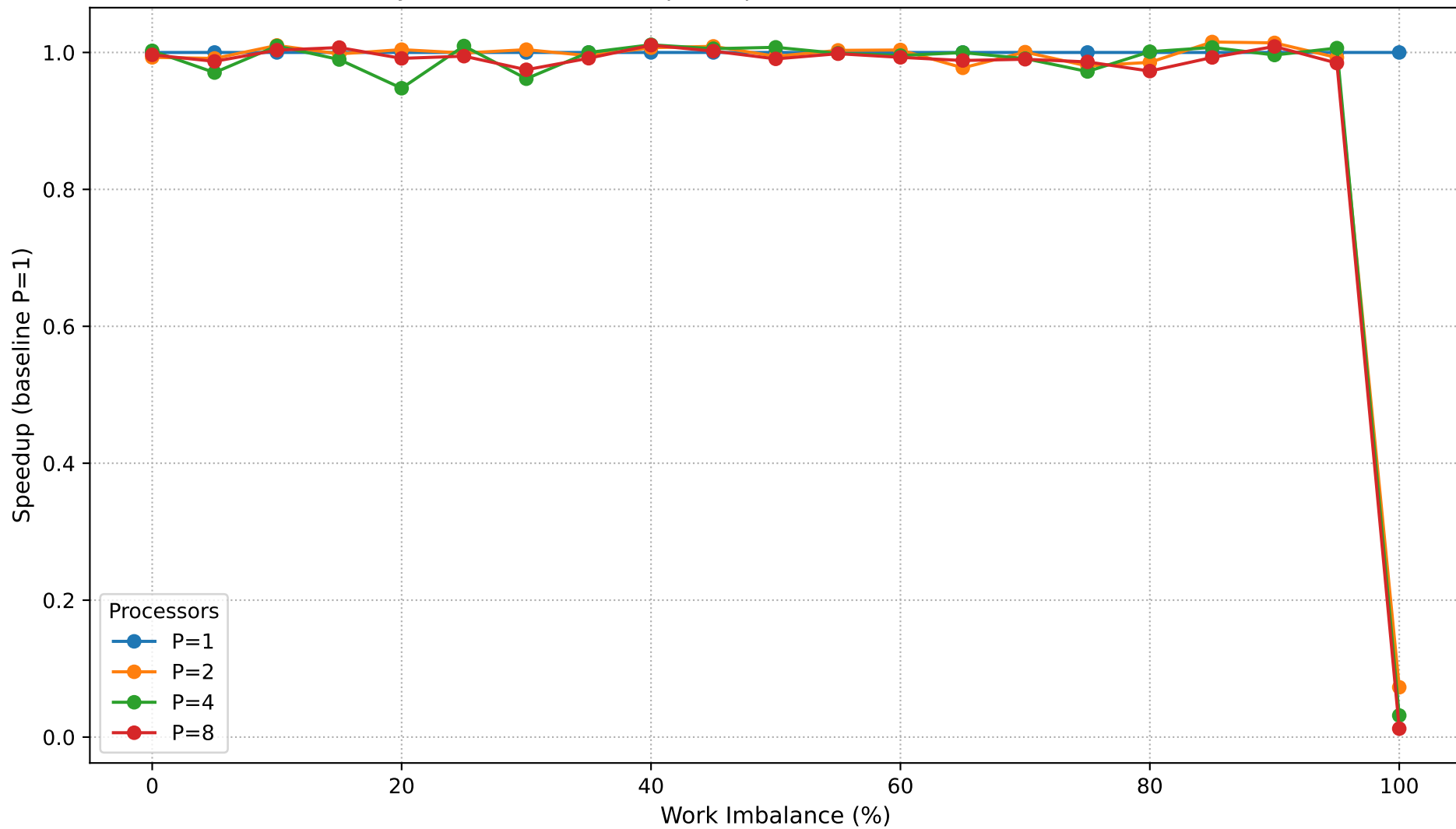
Dyck Path Validation: Speedup vs Work Imbalance (N=700,000)
