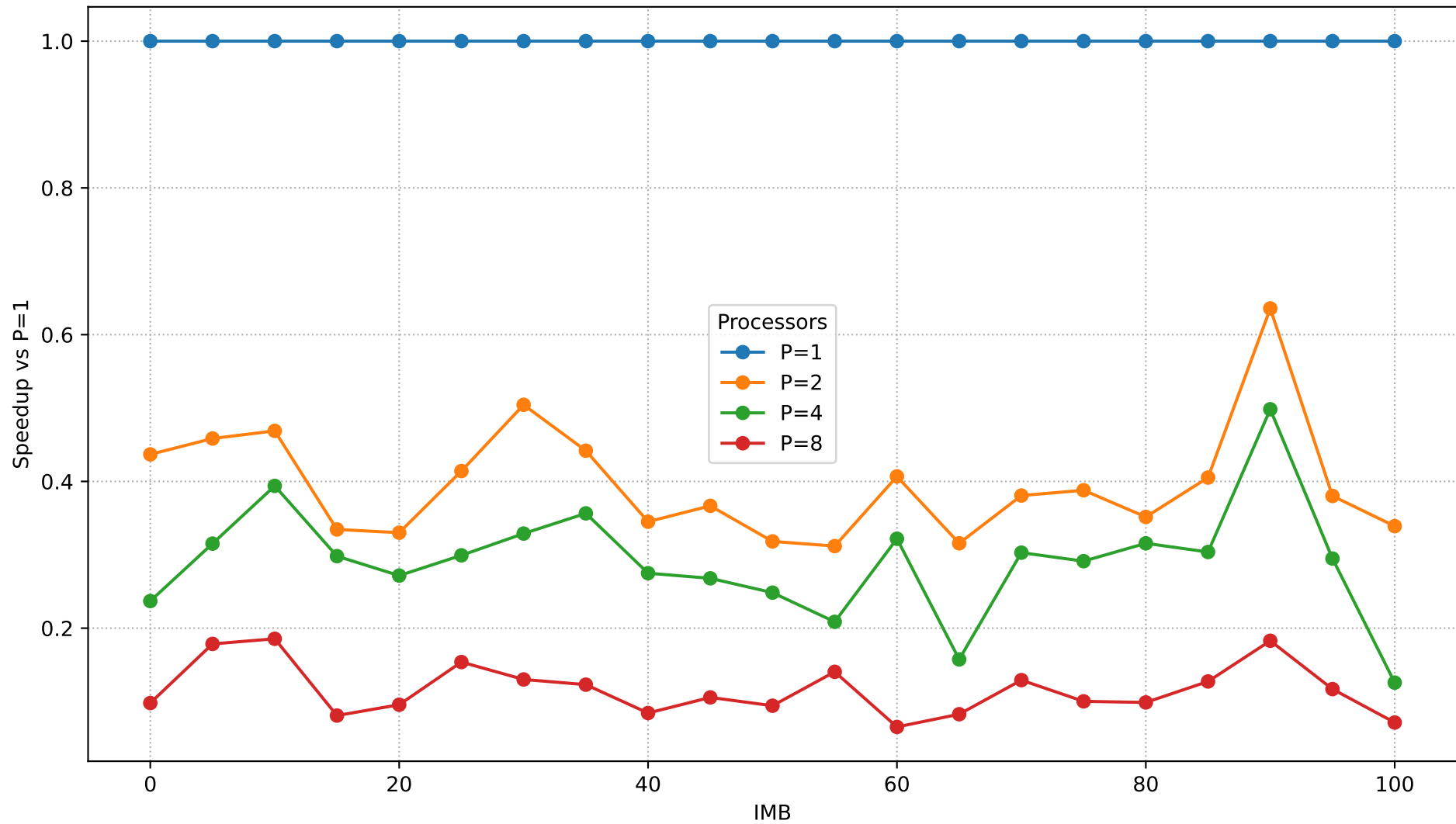
Speedup vs IMB (N=450,000)
