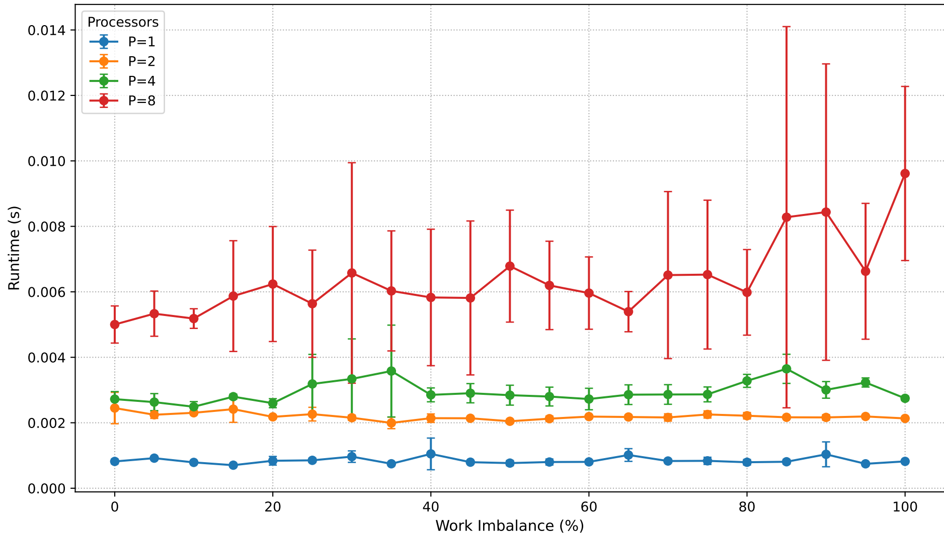
Dyck Path Validation: Runtime vs Work Imbalance (N=750,000)
