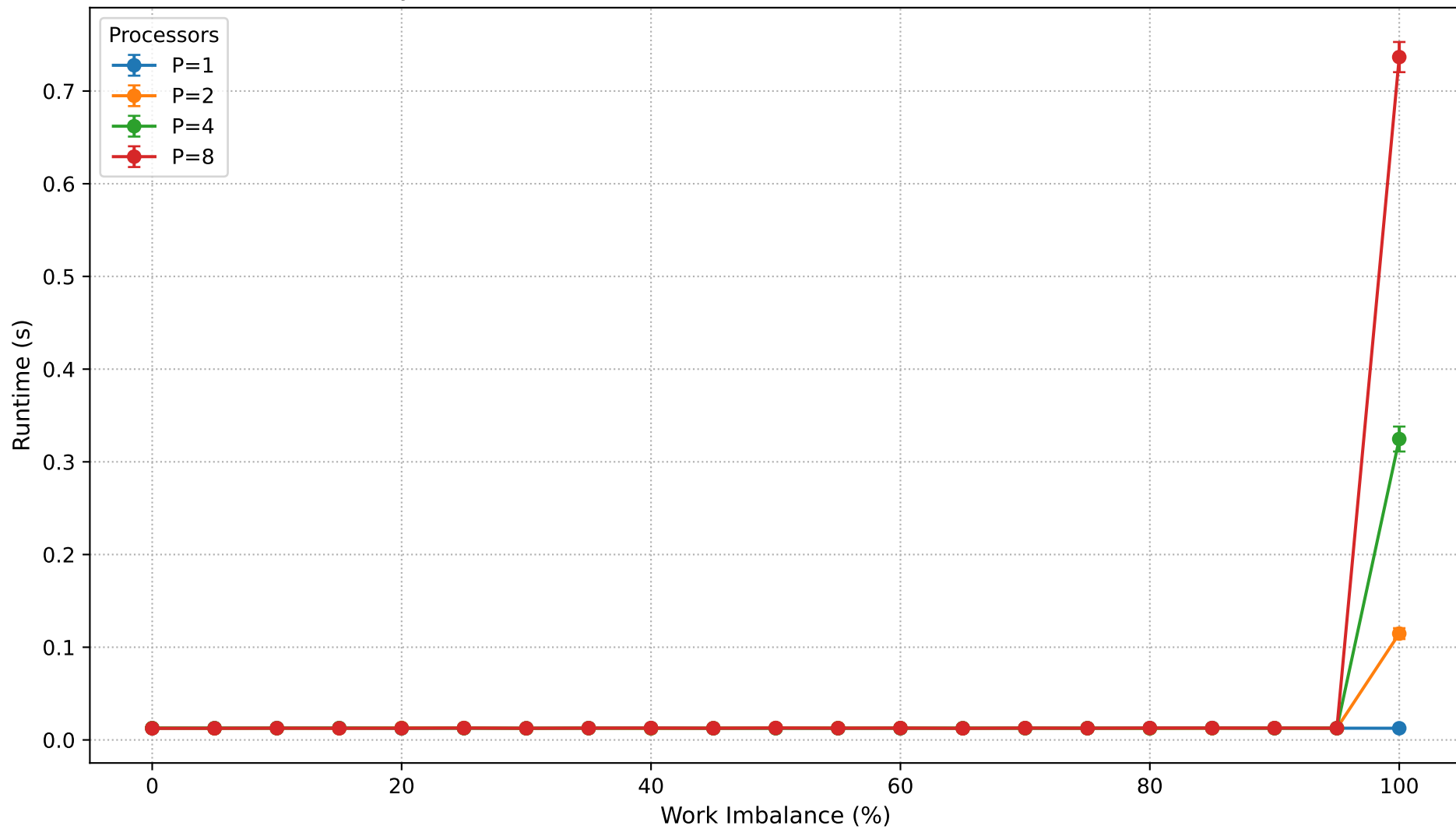
Dyck Path Validation: Runtime vs Work Imbalance (N=550,000)
