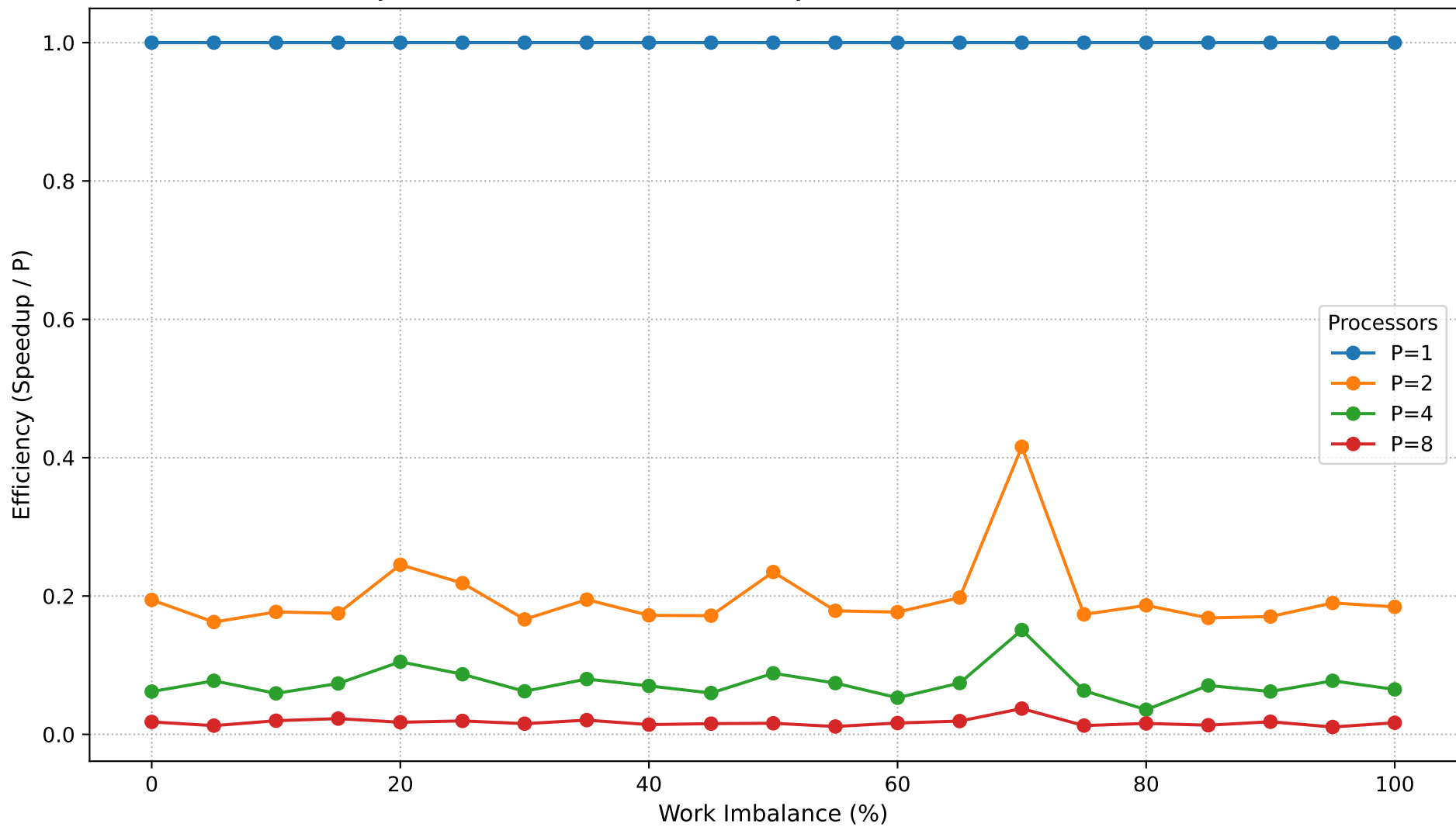
Dyck Path Validation: Parallel Efficiency vs Work Imbalance (N=700,000)
