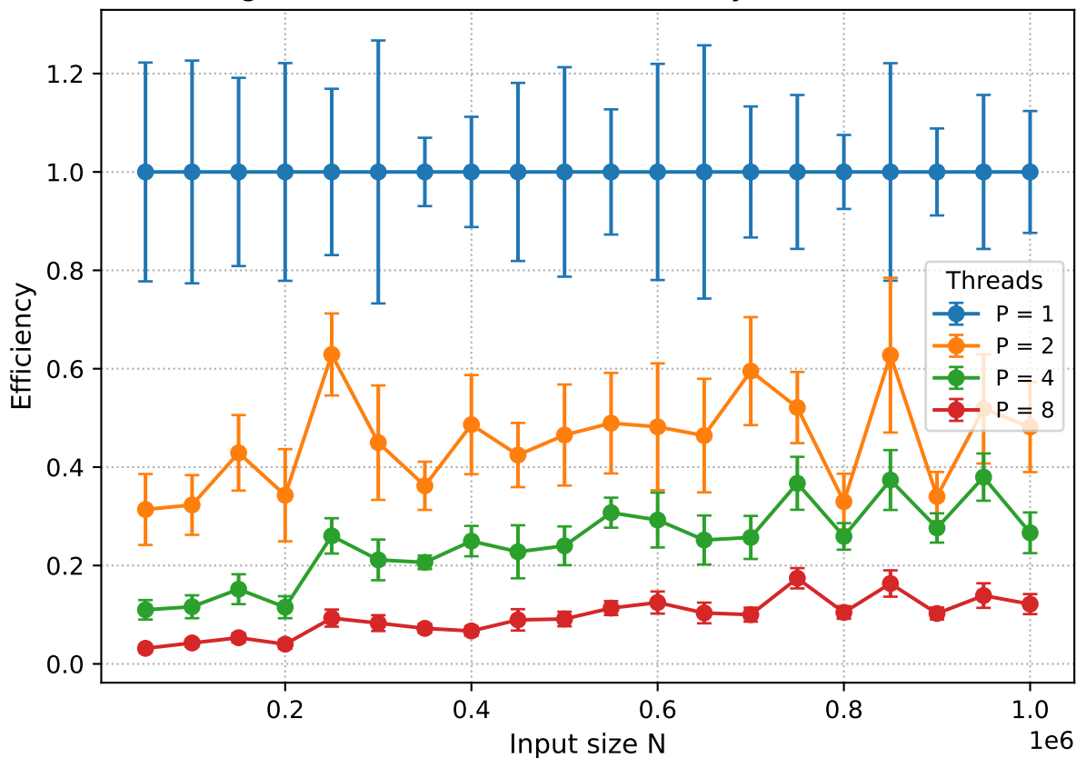
Merge Sort (SUPER): Parallel Efficiency (baseline P = 1)
