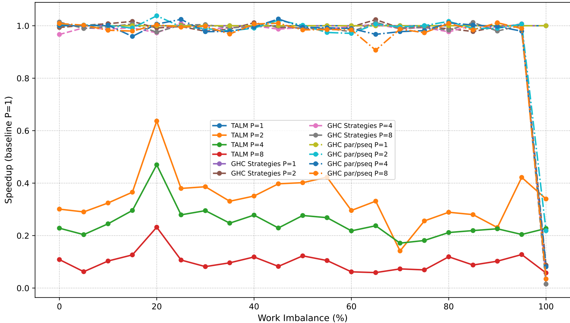
Dyck Path Validation: Speedup Comparison (N=250,000)
