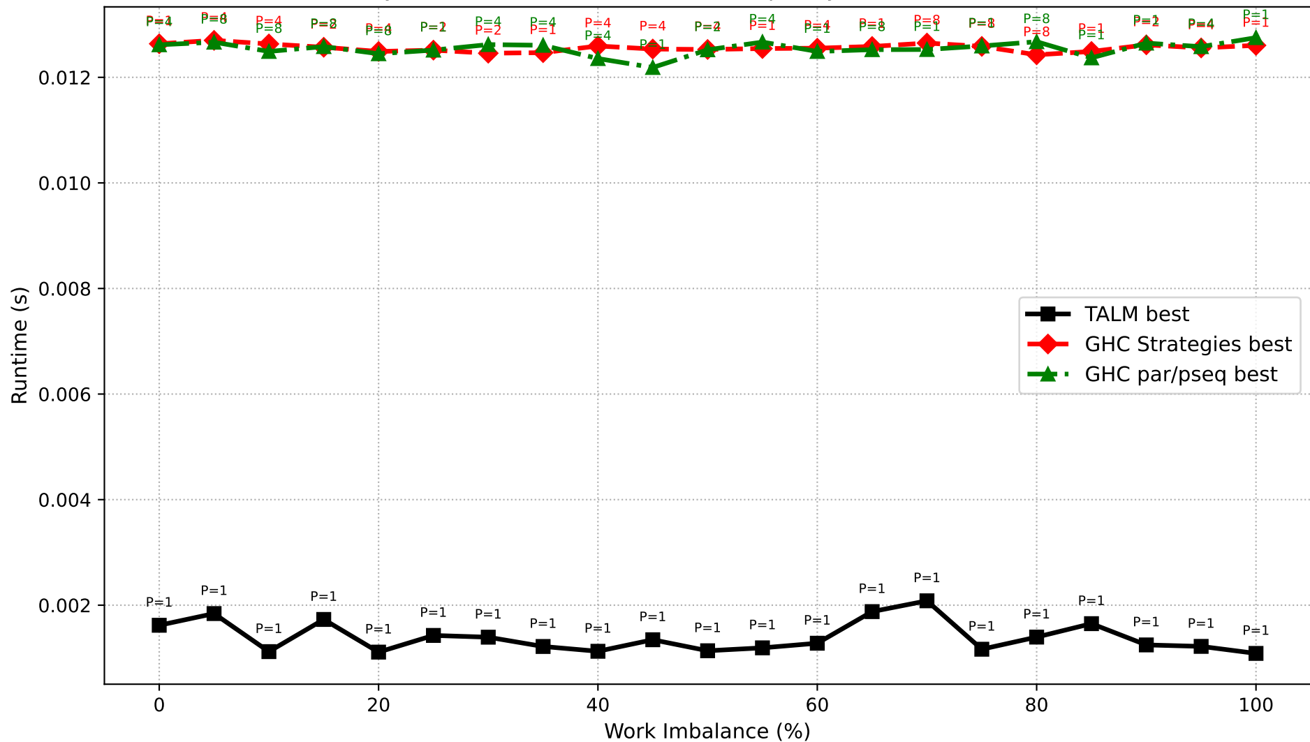
Dyck Path Validation: Best Runtime per System (N=300,000)
