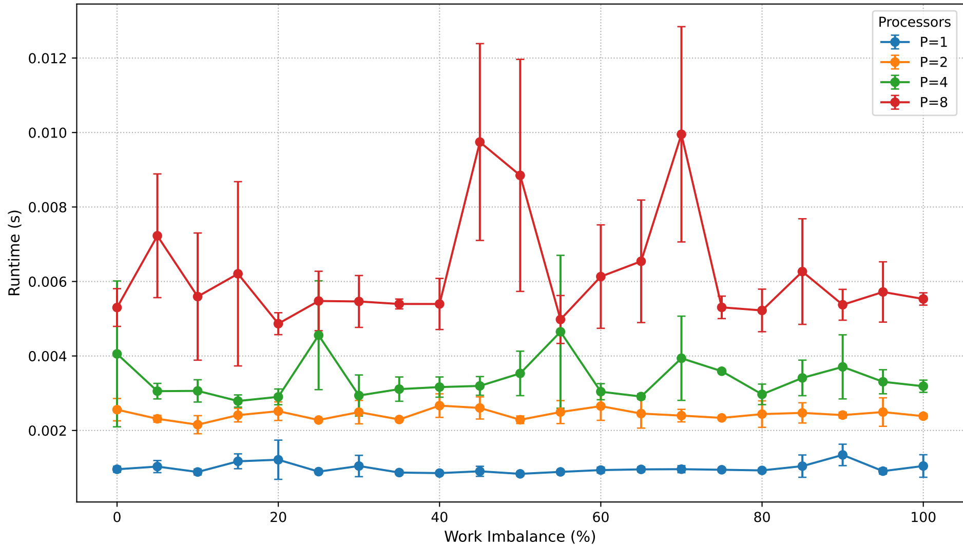
Dyck Path Validation: Runtime vs Work Imbalance (N=200,000)
