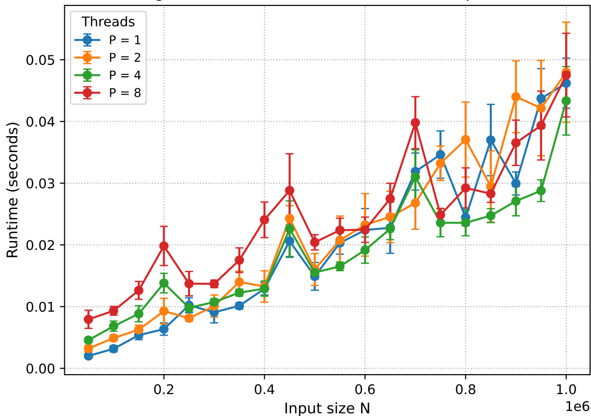
Merge Sort (SUPER): Median Runtime vs Input Size
