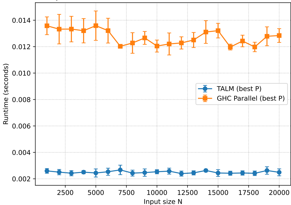
Dyck Path: Best-of-Breed Runtime vs N (imb=0, delta=0)
