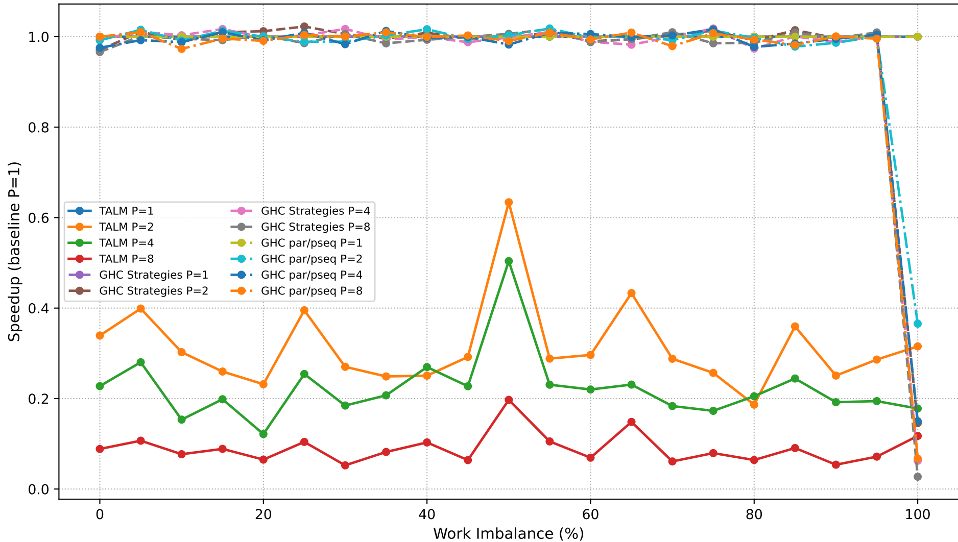
Dyck Path Validation: Speedup Comparison (N=150,000)
