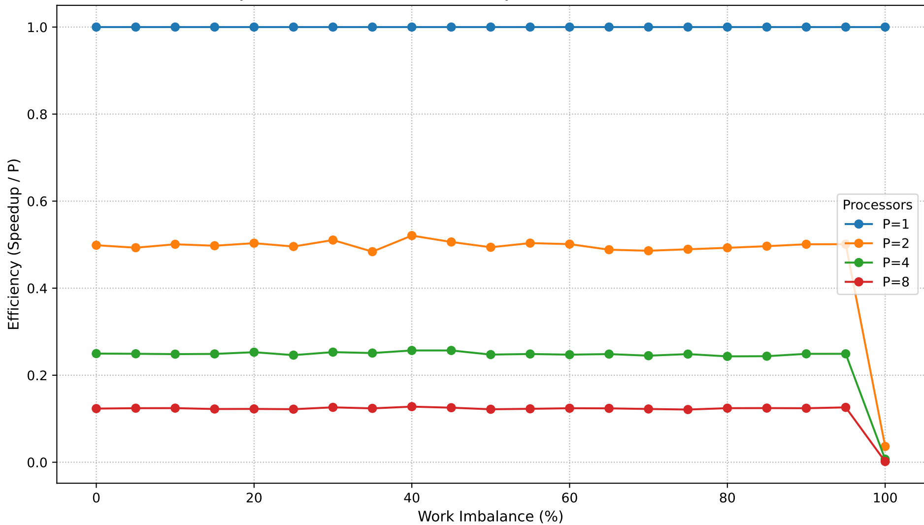
Dyck Path Validation: Parallel Efficiency vs Work Imbalance (N=350,000)
