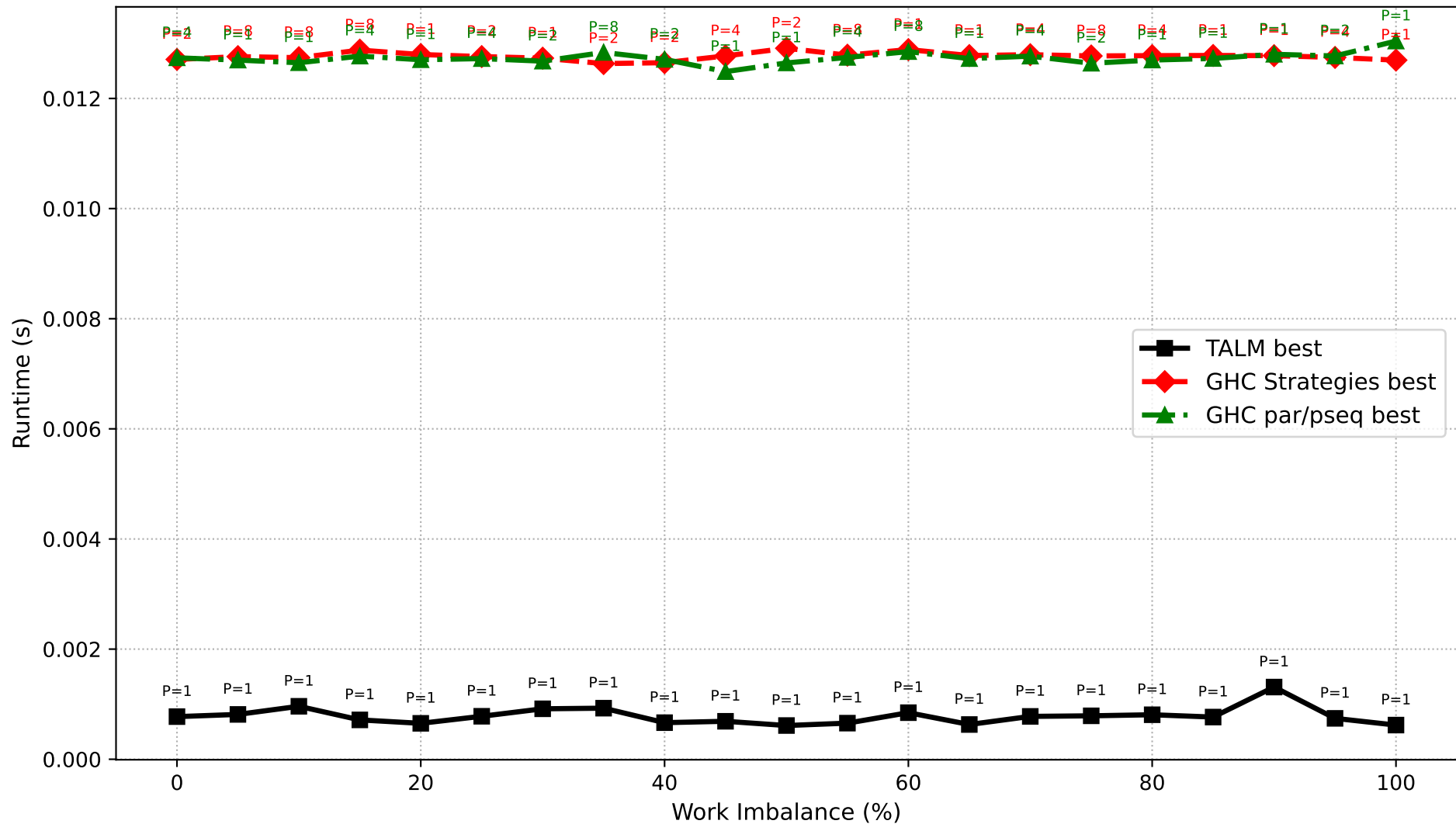
Dyck Path Validation: Best Runtime per System (N=450,000)
