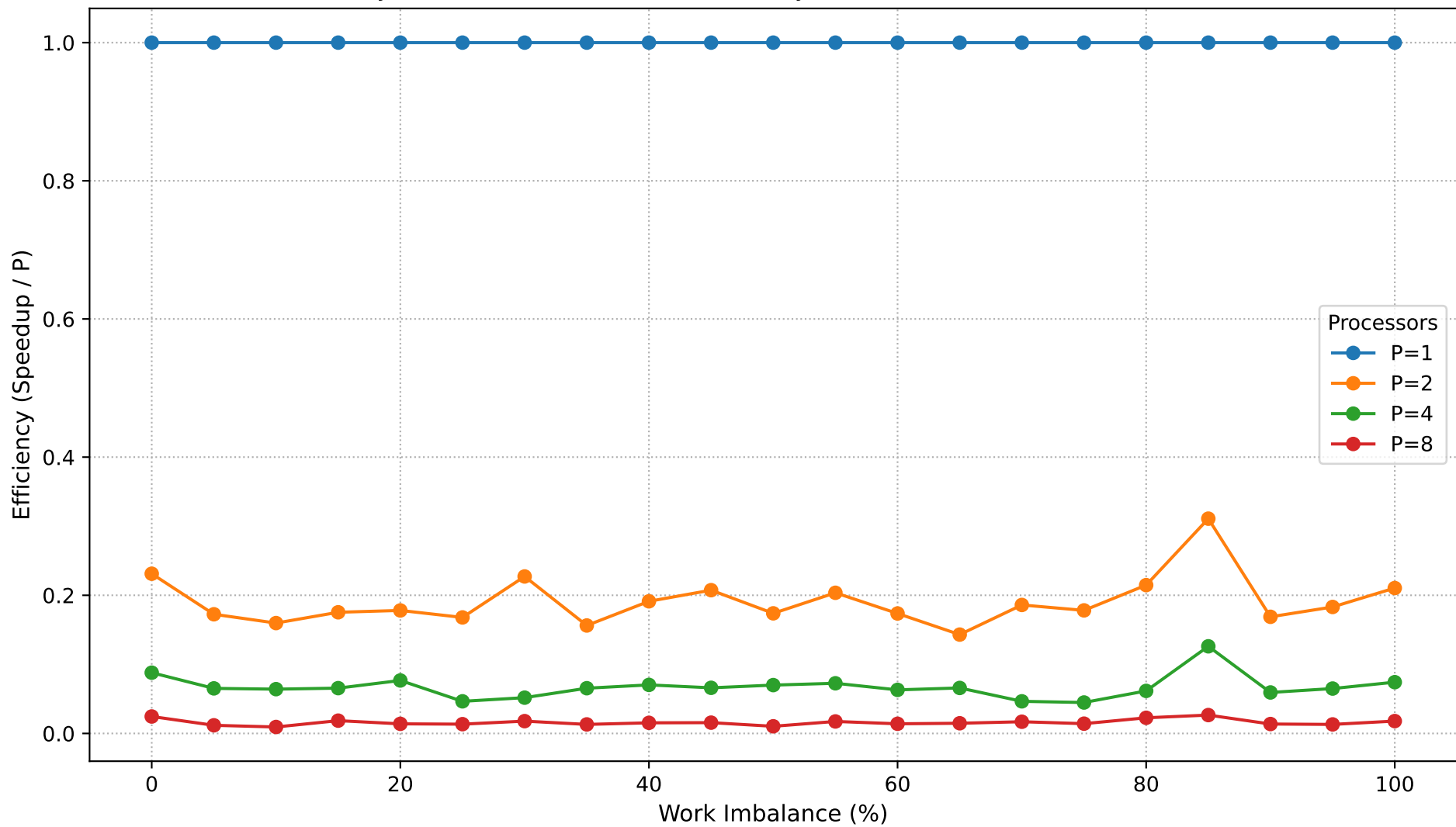
Dyck Path Validation: Parallel Efficiency vs Work Imbalance (N=600,000)
