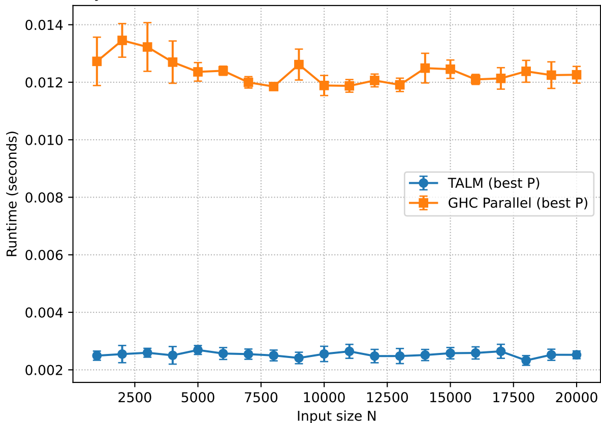
Dyck Path: Best-of-Breed Runtime vs N (imb=50, delta=5000)
