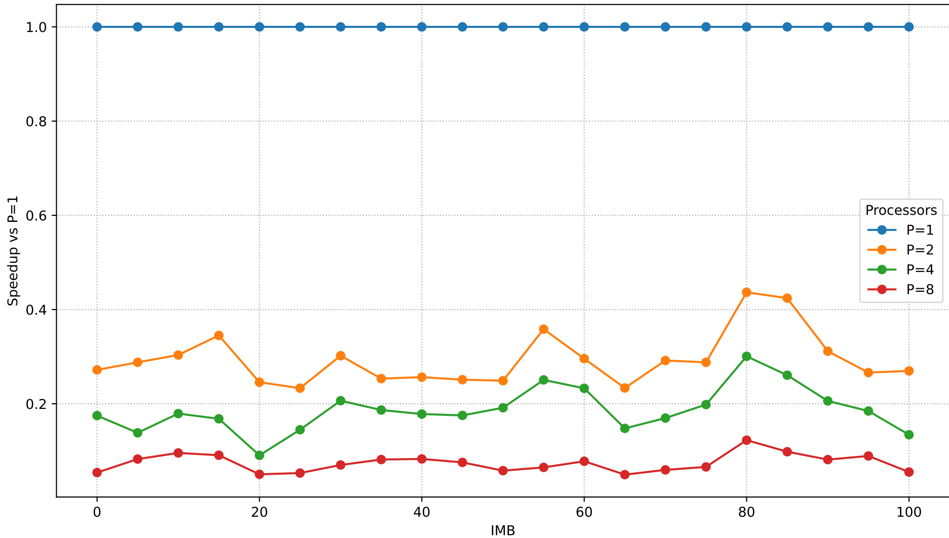
Speedup vs IMB (N=50,000)
