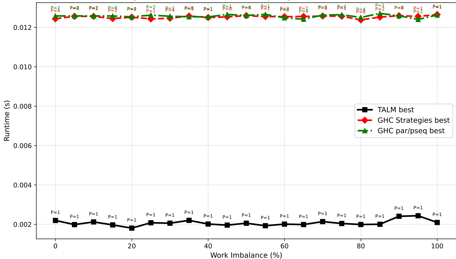
Dyck Path Validation: Best Runtime per System (N=600,000)
