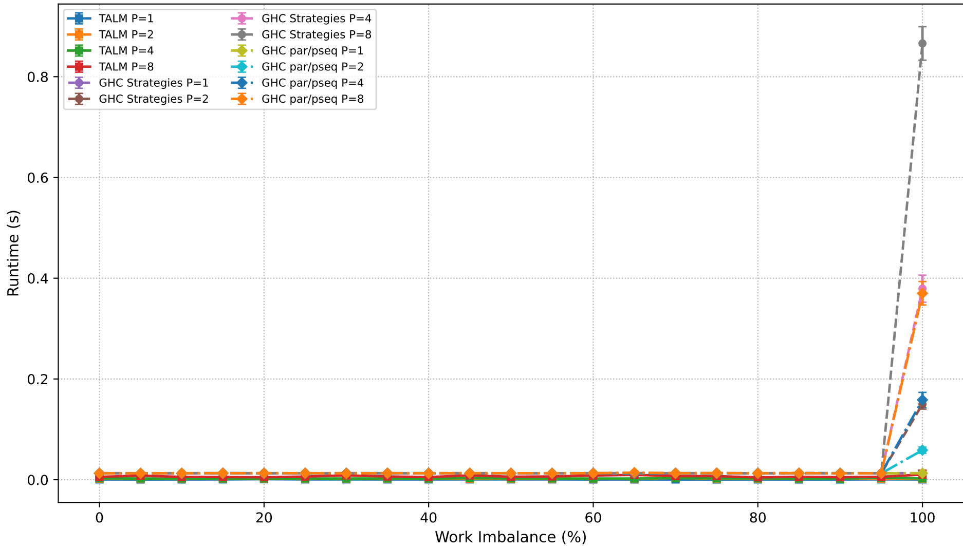
Dyck Path Validation: Runtime Comparison (N=250,000)
