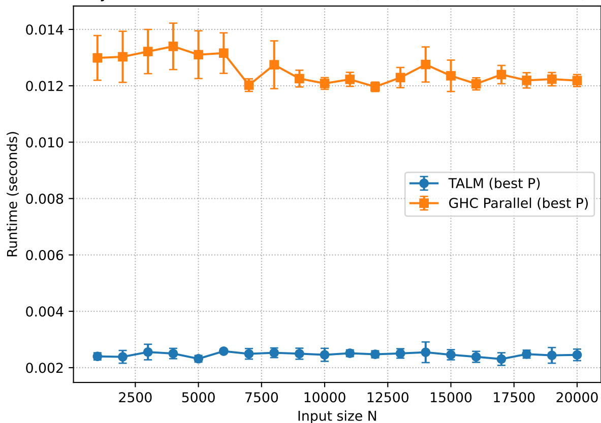
Dyck Path: Best-of-Breed Runtime vs N (imb=0, delta=5000)
