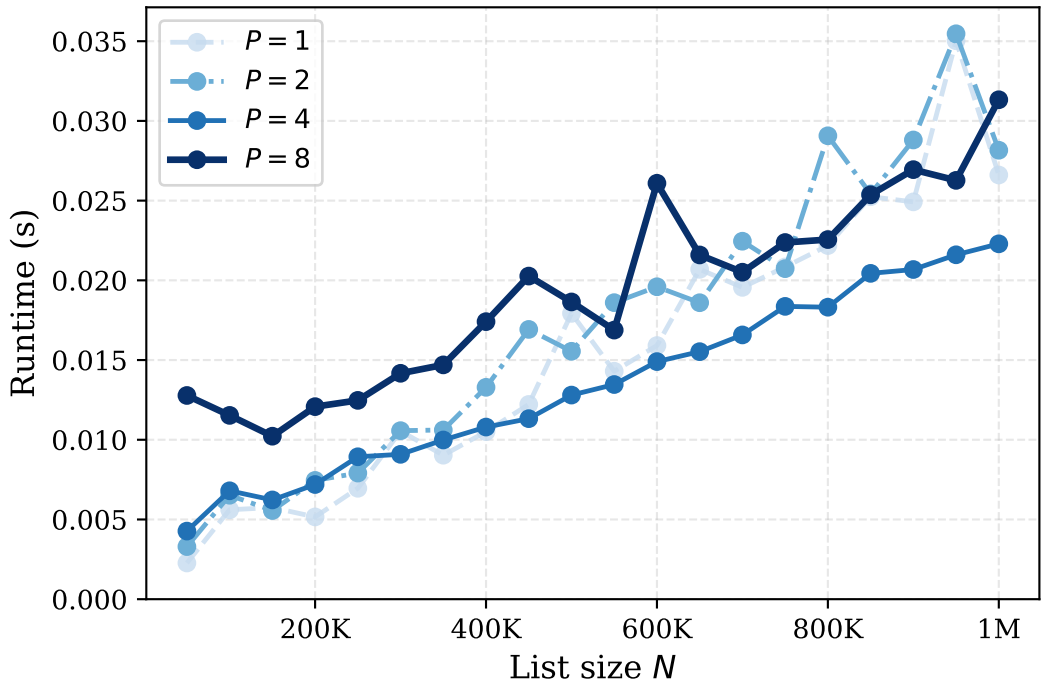
Merge Sort: Ribault Scaling by P
