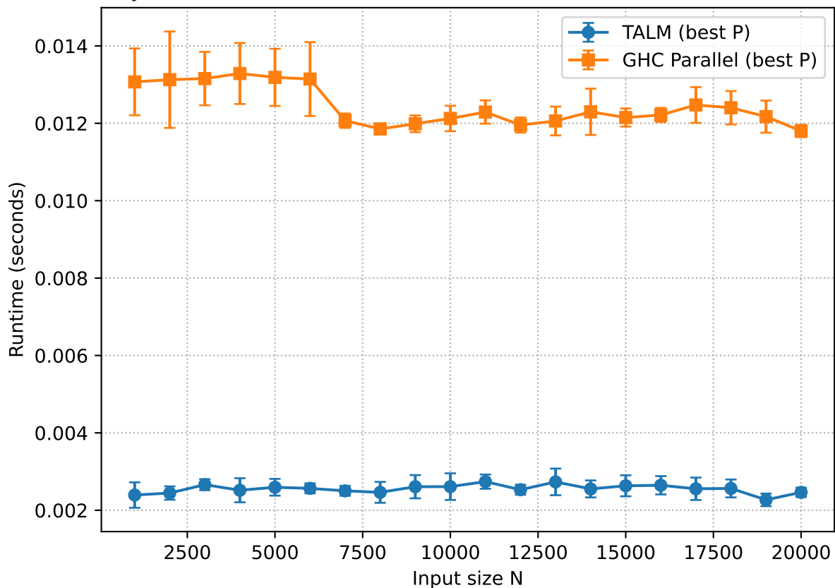
Dyck Path: Best-of-Breed Runtime vs N (imb=25, delta=5000)
