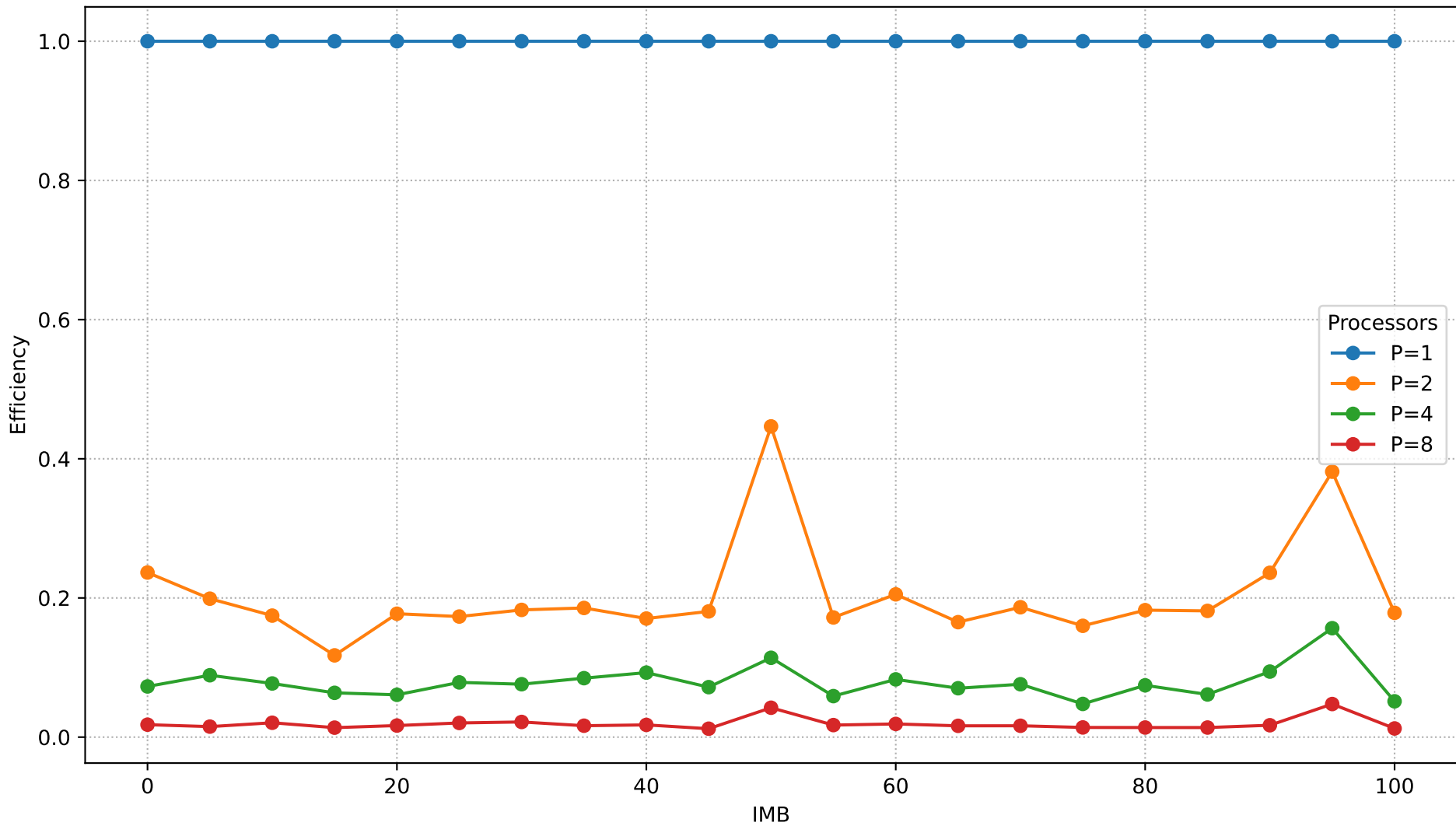
Efficiency vs IMB (N=850,000)
