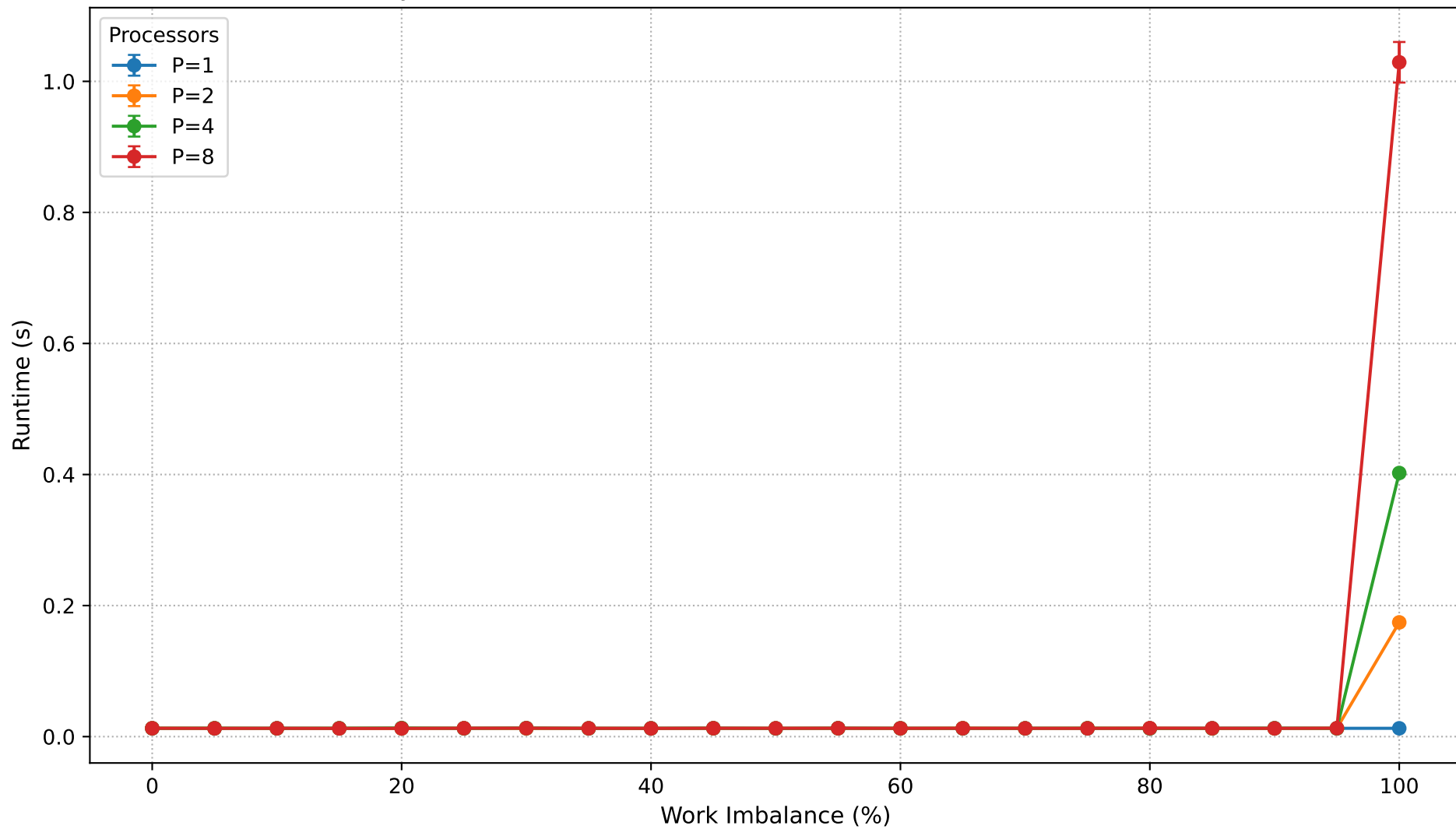
Dyck Path Validation: Runtime vs Work Imbalance (N=700,000)
