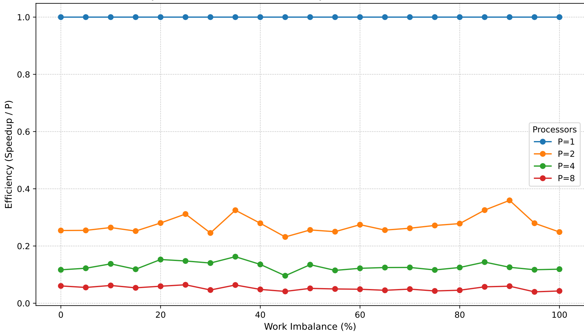
Dyck Path Validation: Parallel Efficiency vs Work Imbalance (N=950,000)
