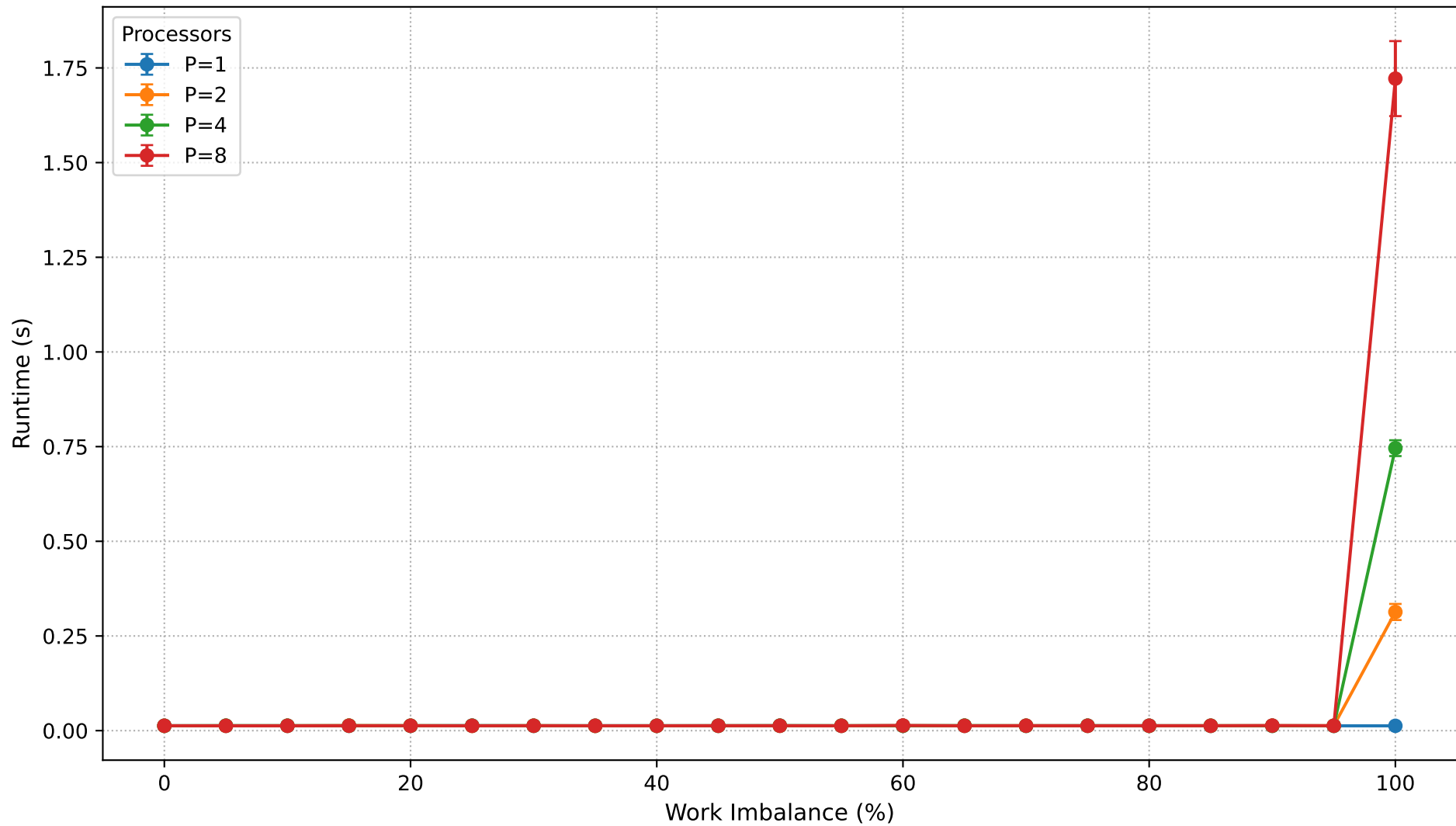
Dyck Path Validation: Runtime vs Work Imbalance (N=450,000)
