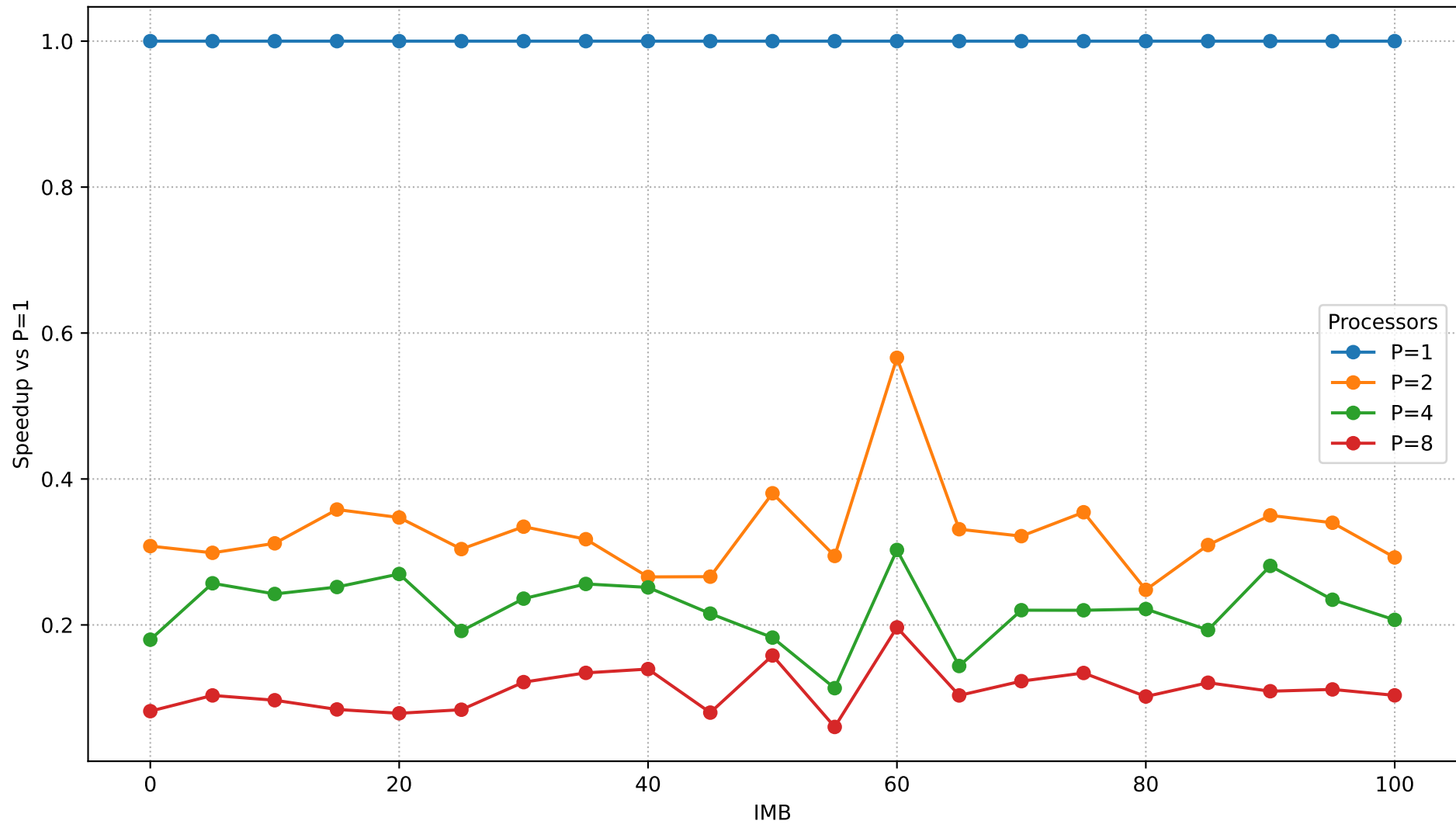
Speedup vs IMB (N=500,000)
