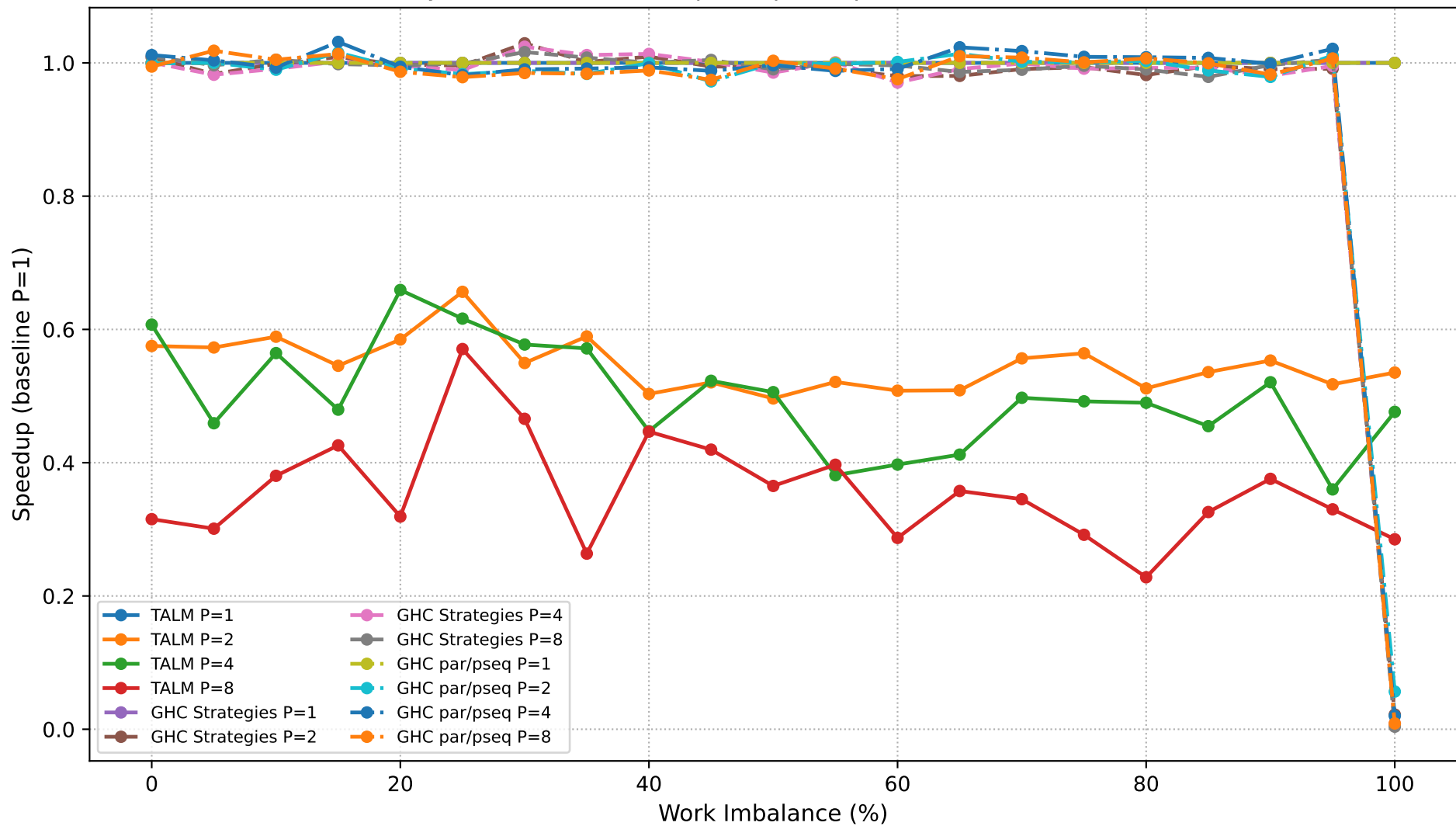
Dyck Path Validation: Speedup Comparison (N=1,000,000)
