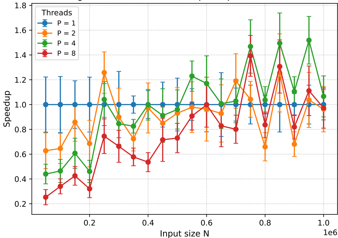
Merge Sort (SUPER): Parallel Speedup (baseline P = 1)
