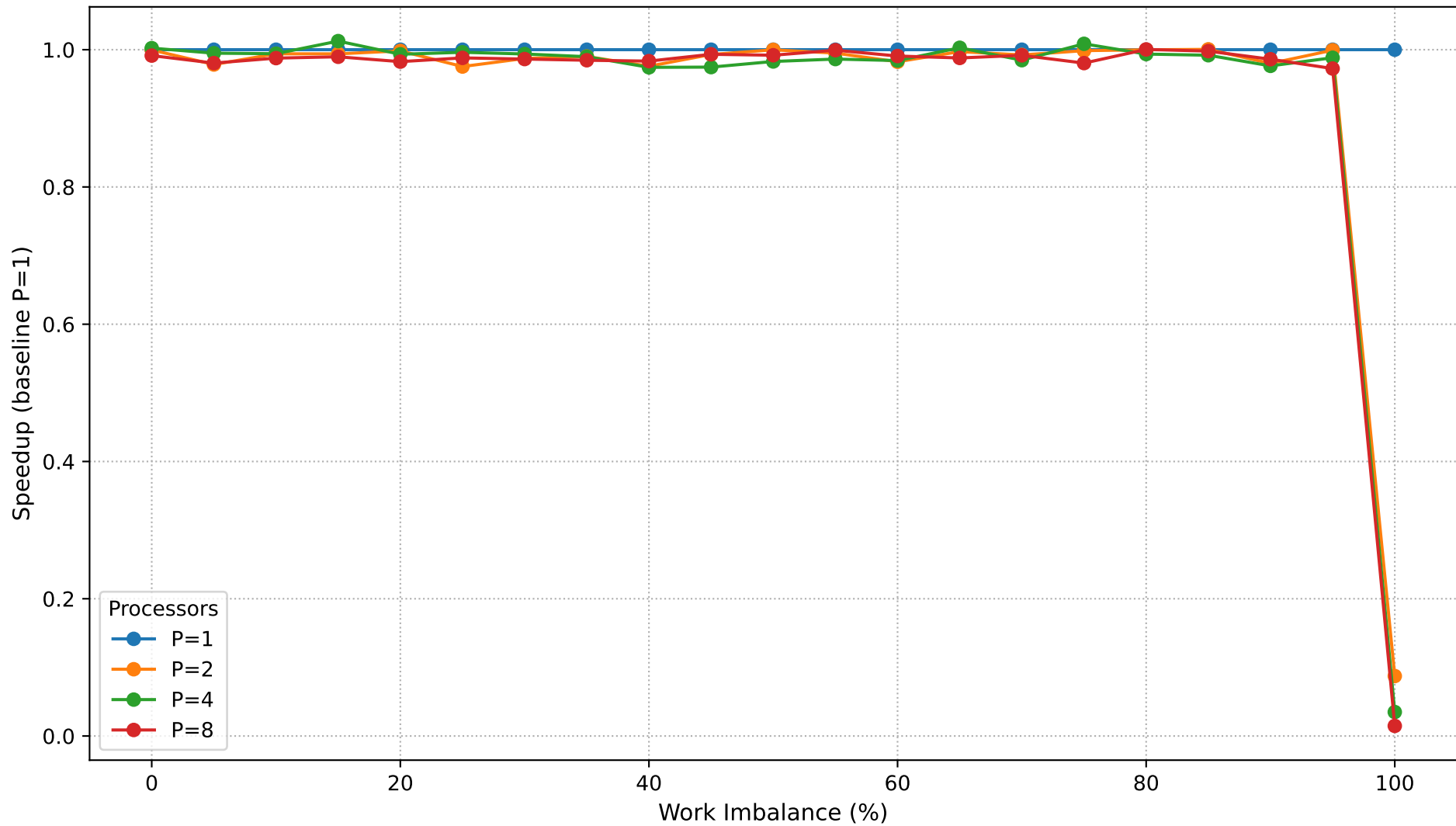
Dyck Path Validation: Speedup vs Work Imbalance (N=650,000)
