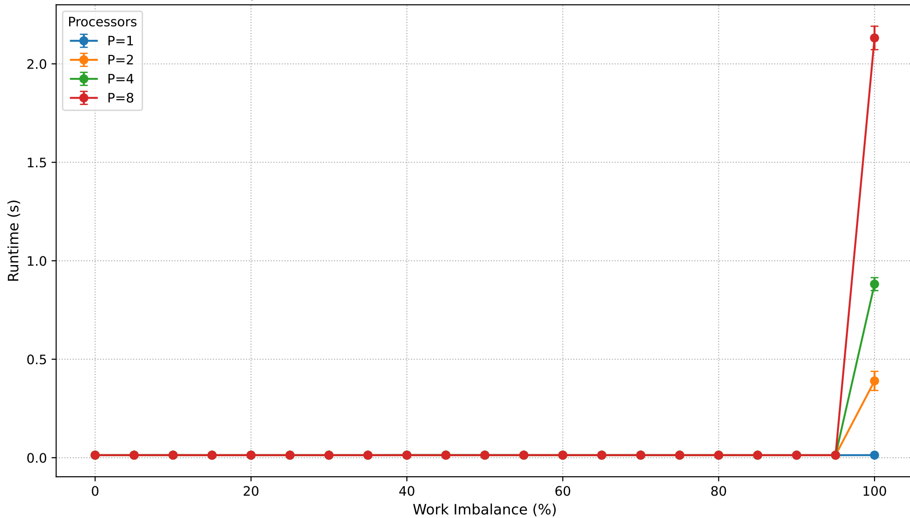
Dyck Path Validation: Runtime vs Work Imbalance (N=650,000)
