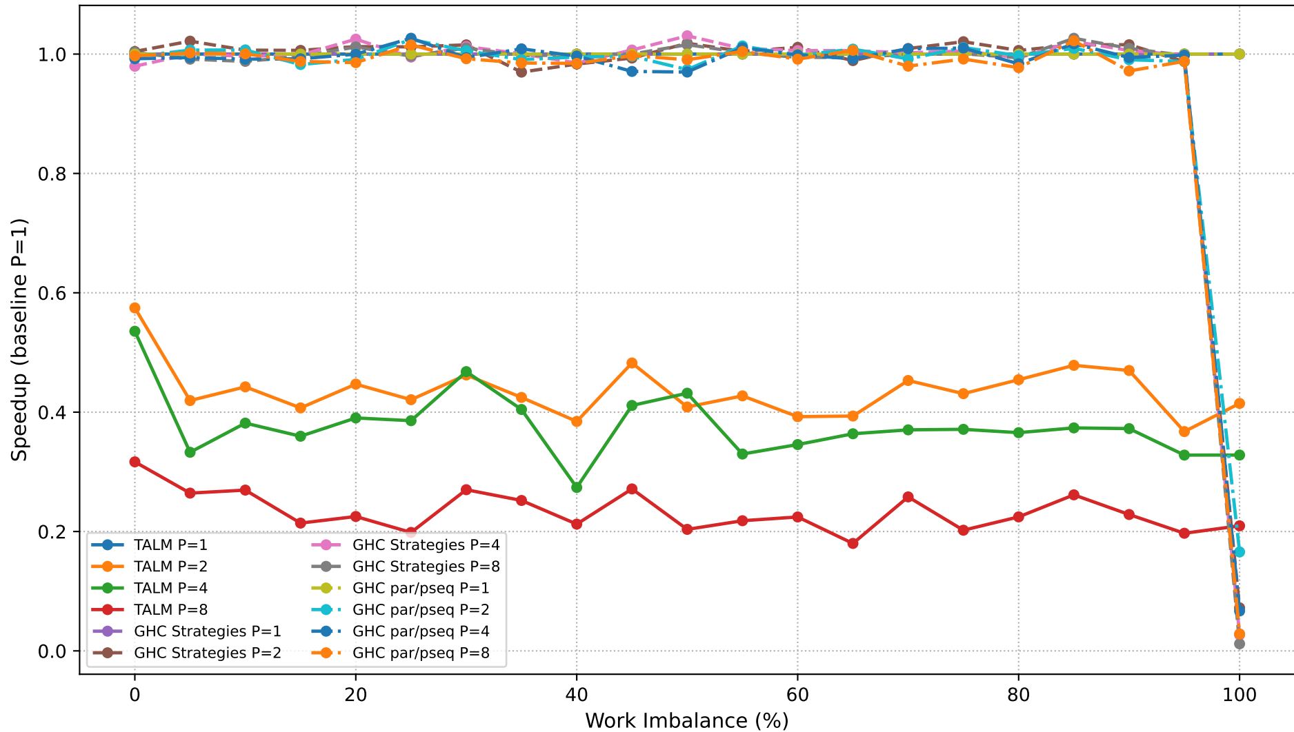
Dyck Path Validation: Speedup Comparison (N=350,000)
