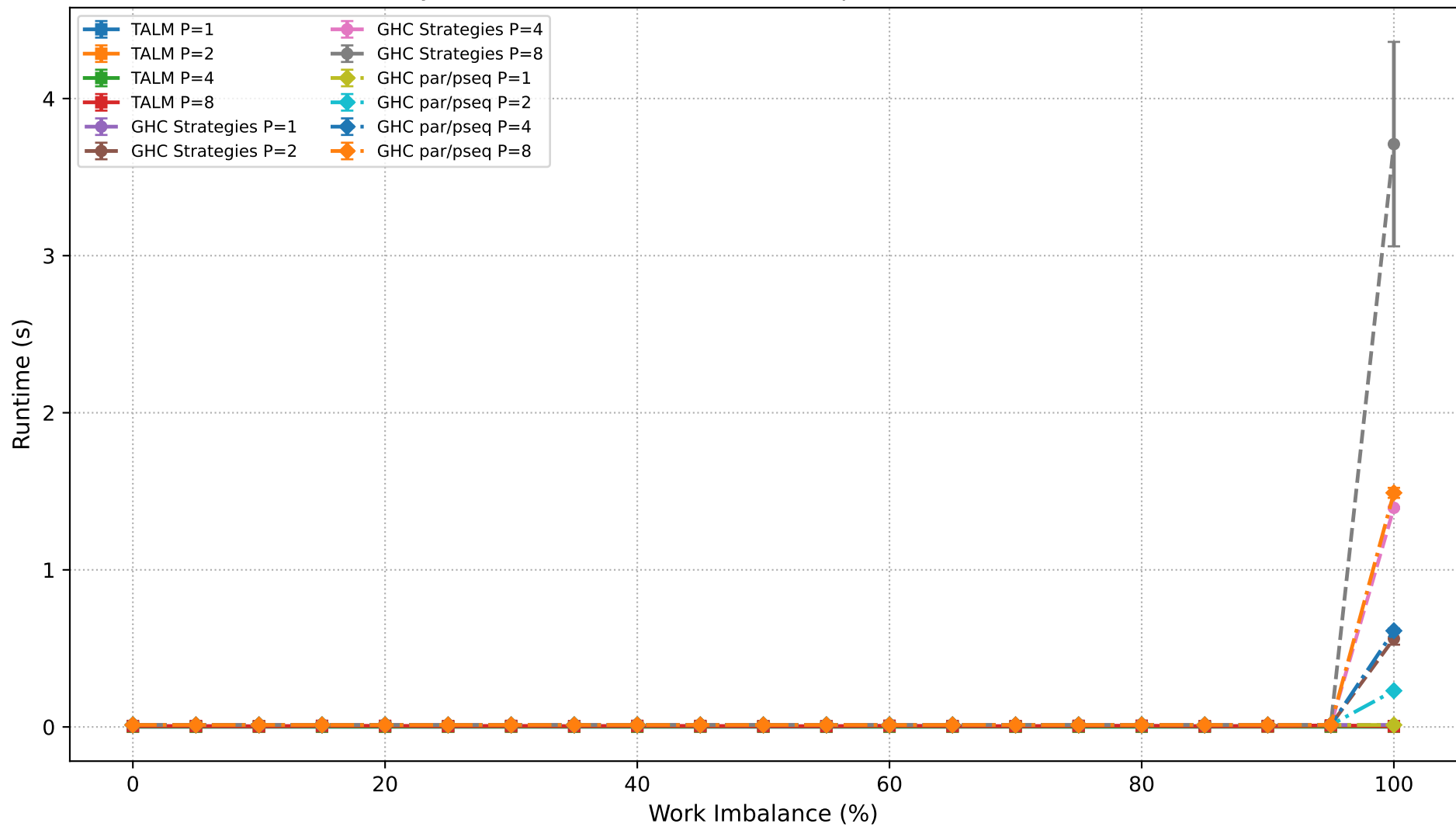
Dyck Path Validation: Runtime Comparison (N=1,000,000)
