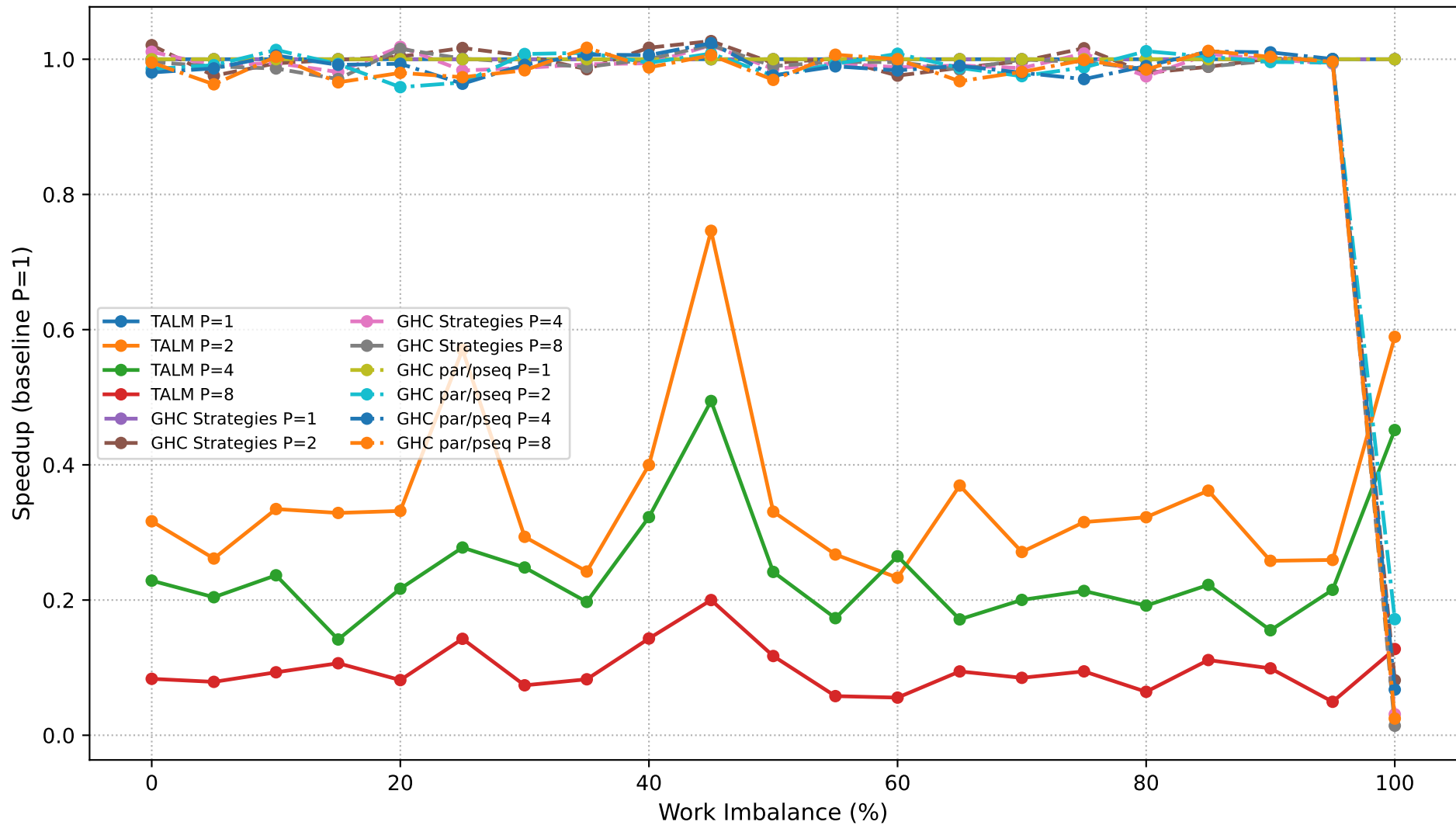
Dyck Path Validation: Speedup Comparison (N=300,000)
