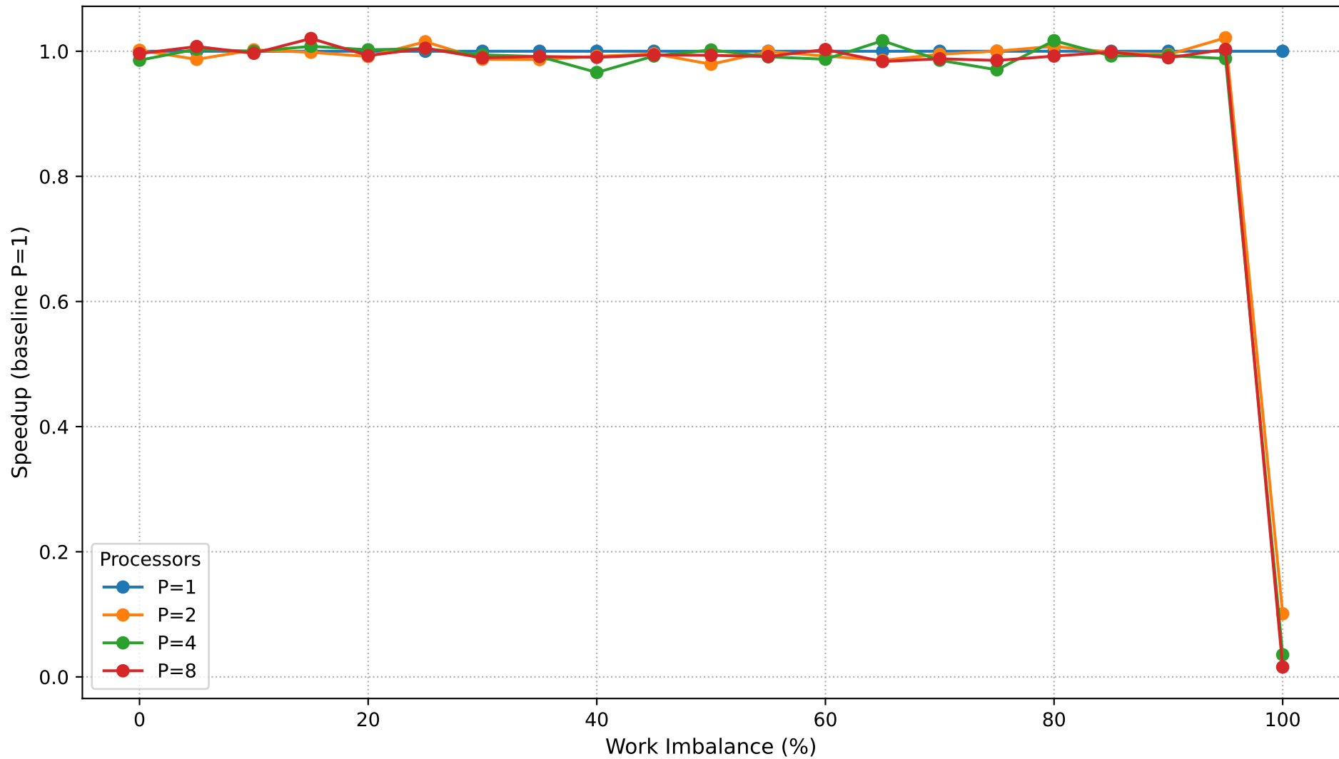
Dyck Path Validation: Speedup vs Work Imbalance (N=600,000)
