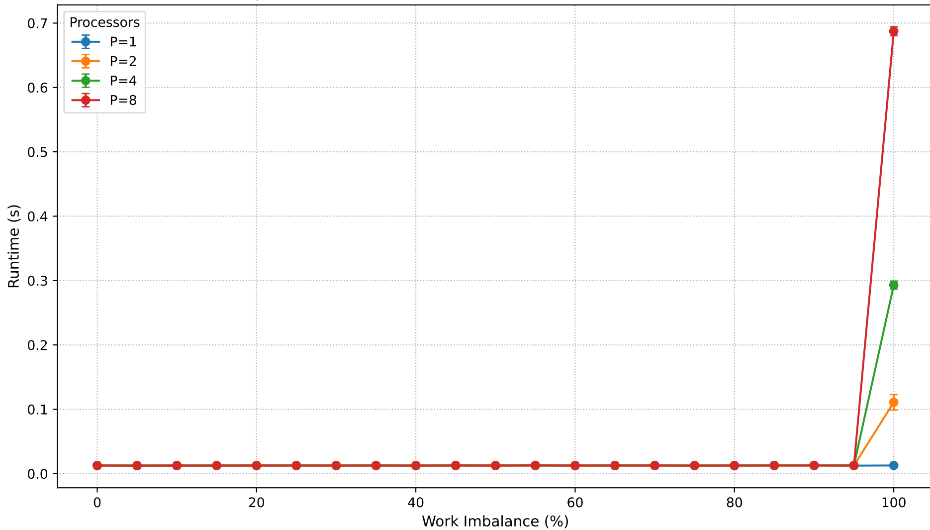
Dyck Path Validation: Runtime vs Work Imbalance (N=500,000)
