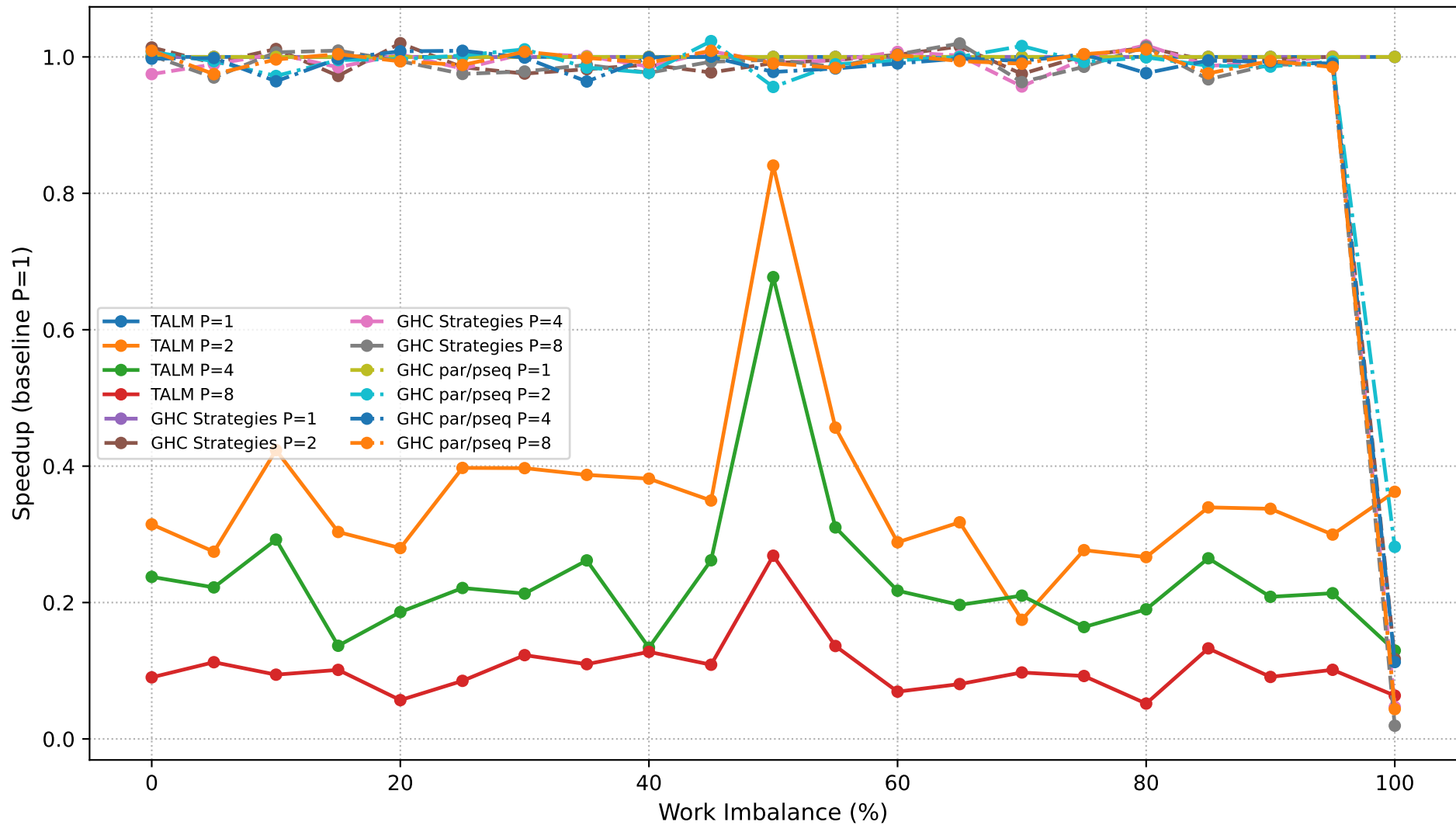
Dyck Path Validation: Speedup Comparison (N=200,000)
