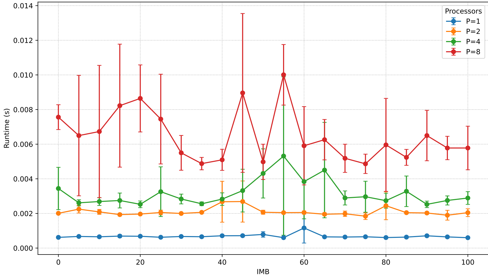
Runtime vs IMB (N=500,000)
