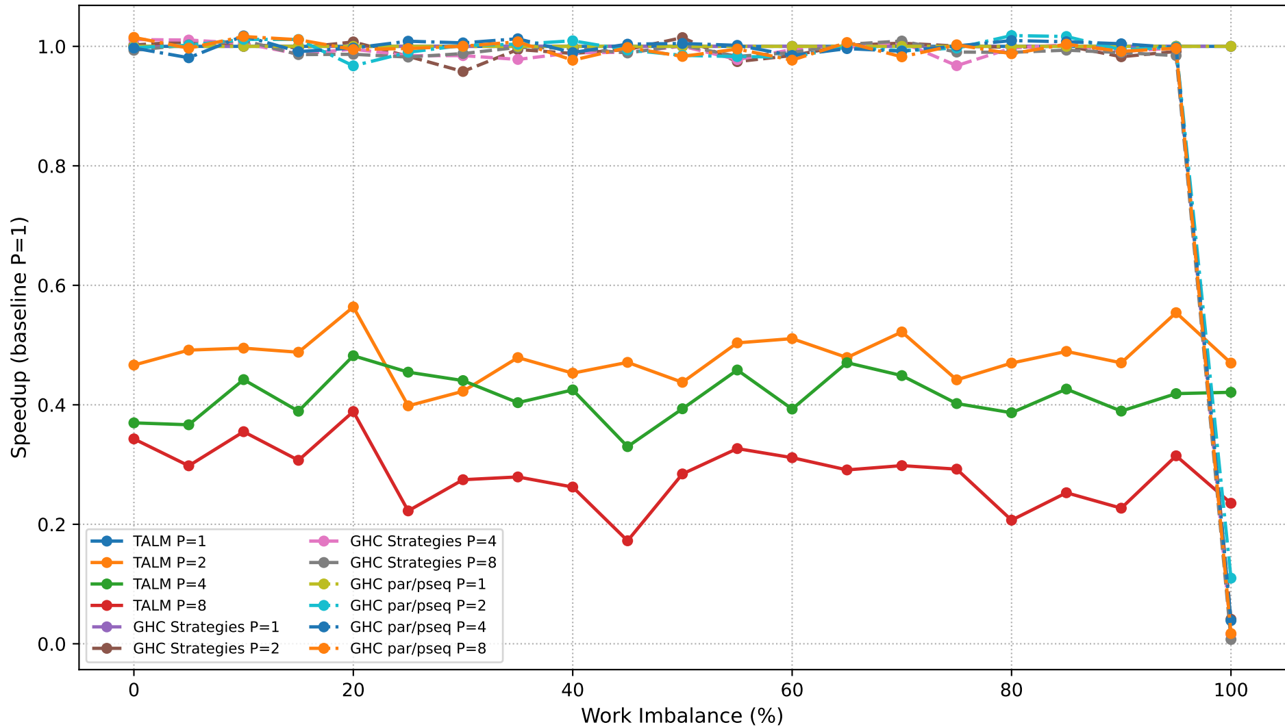
Dyck Path Validation: Speedup Comparison (N=550,000)
