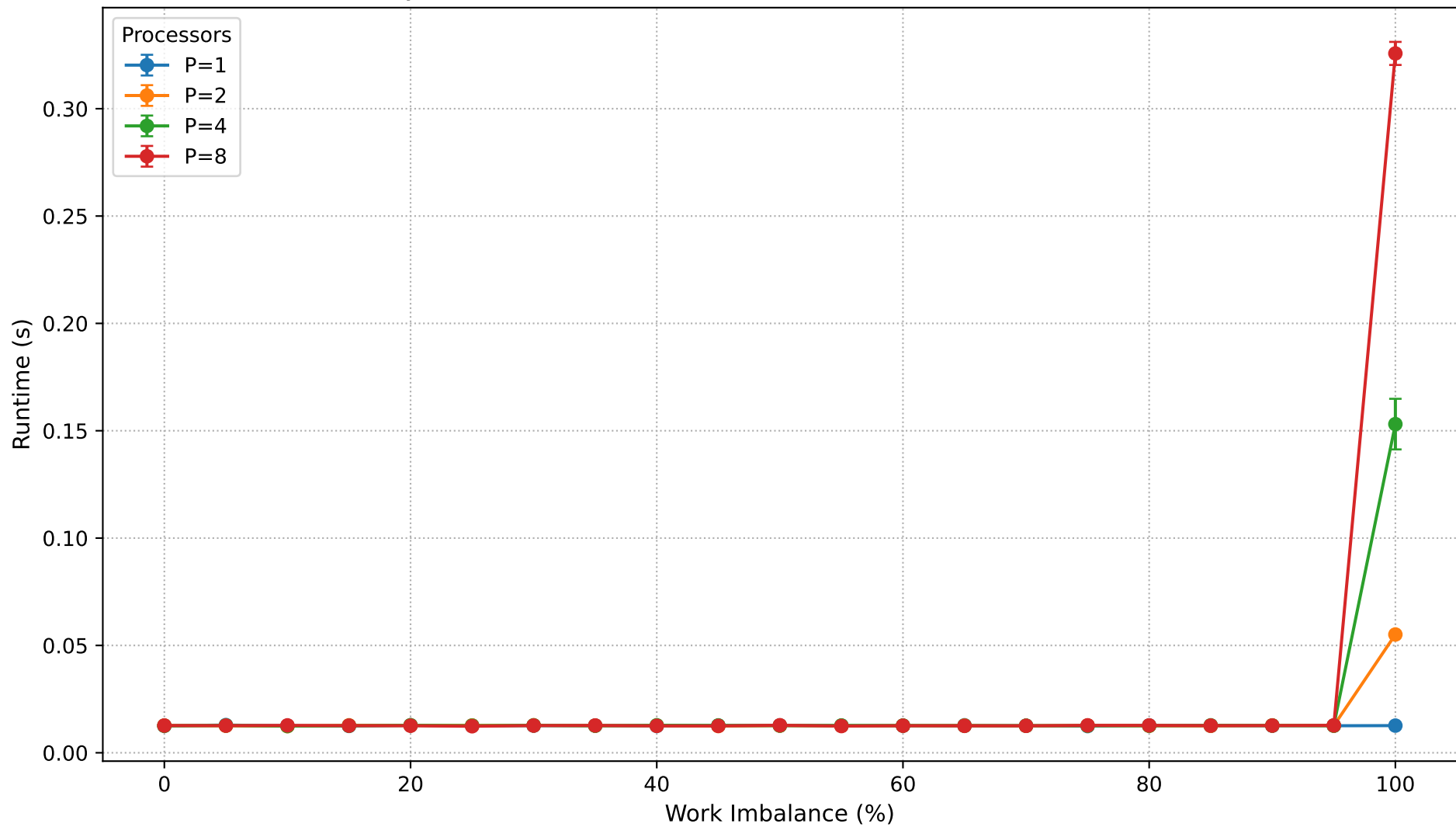
Dyck Path Validation: Runtime vs Work Imbalance (N=250,000)
