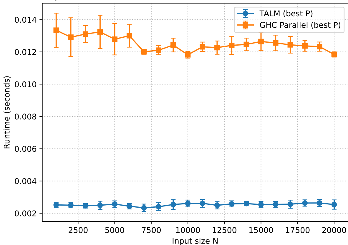
Dyck Path: Best-of-Breed Runtime vs N (imb=50, delta=1000)
