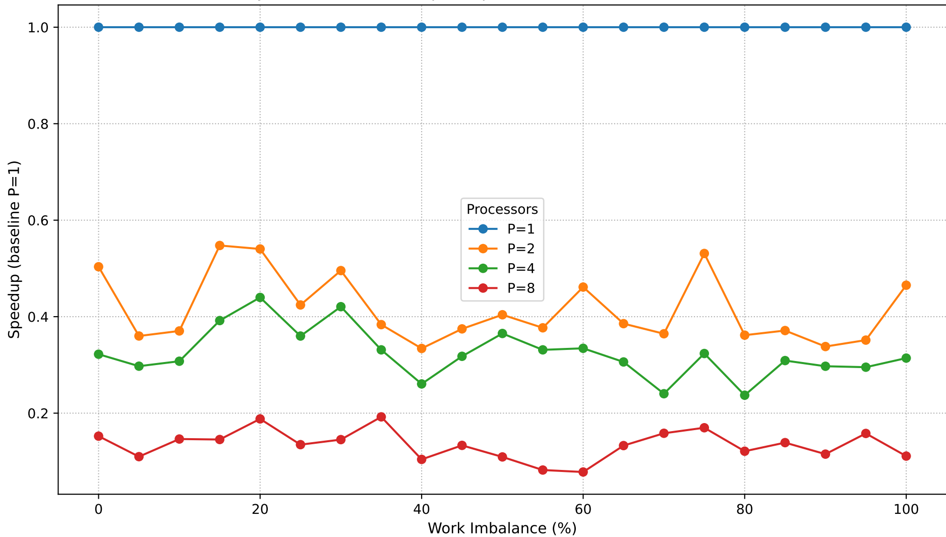
Dyck Path Validation: Speedup vs Work Imbalance (N=250,000)
