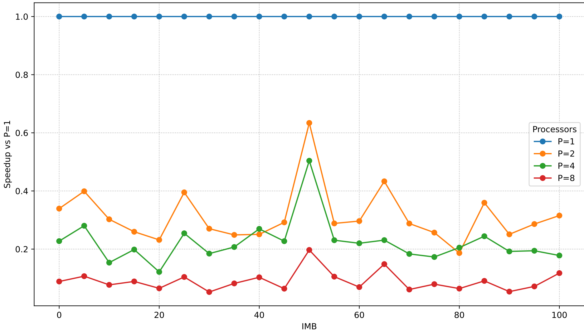
Speedup vs IMB (N=150,000)
