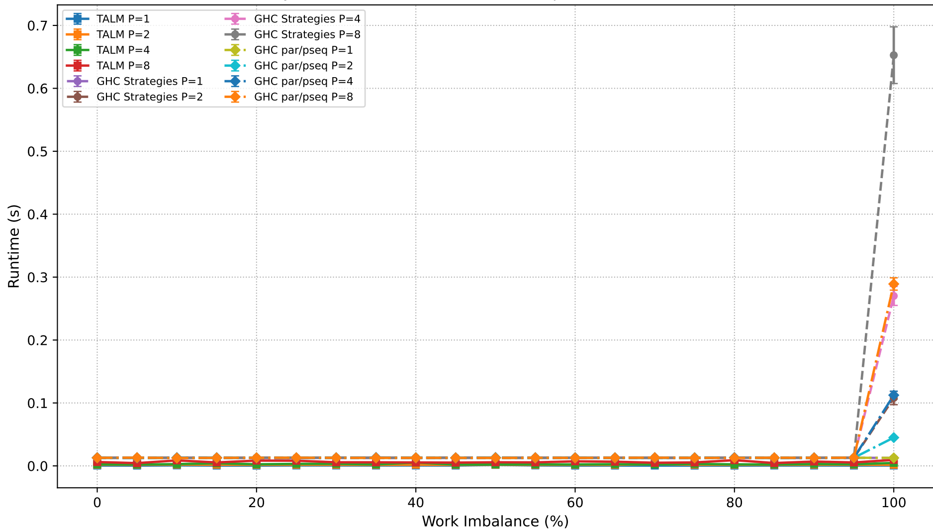
Dyck Path Validation: Runtime Comparison (N=200,000)
