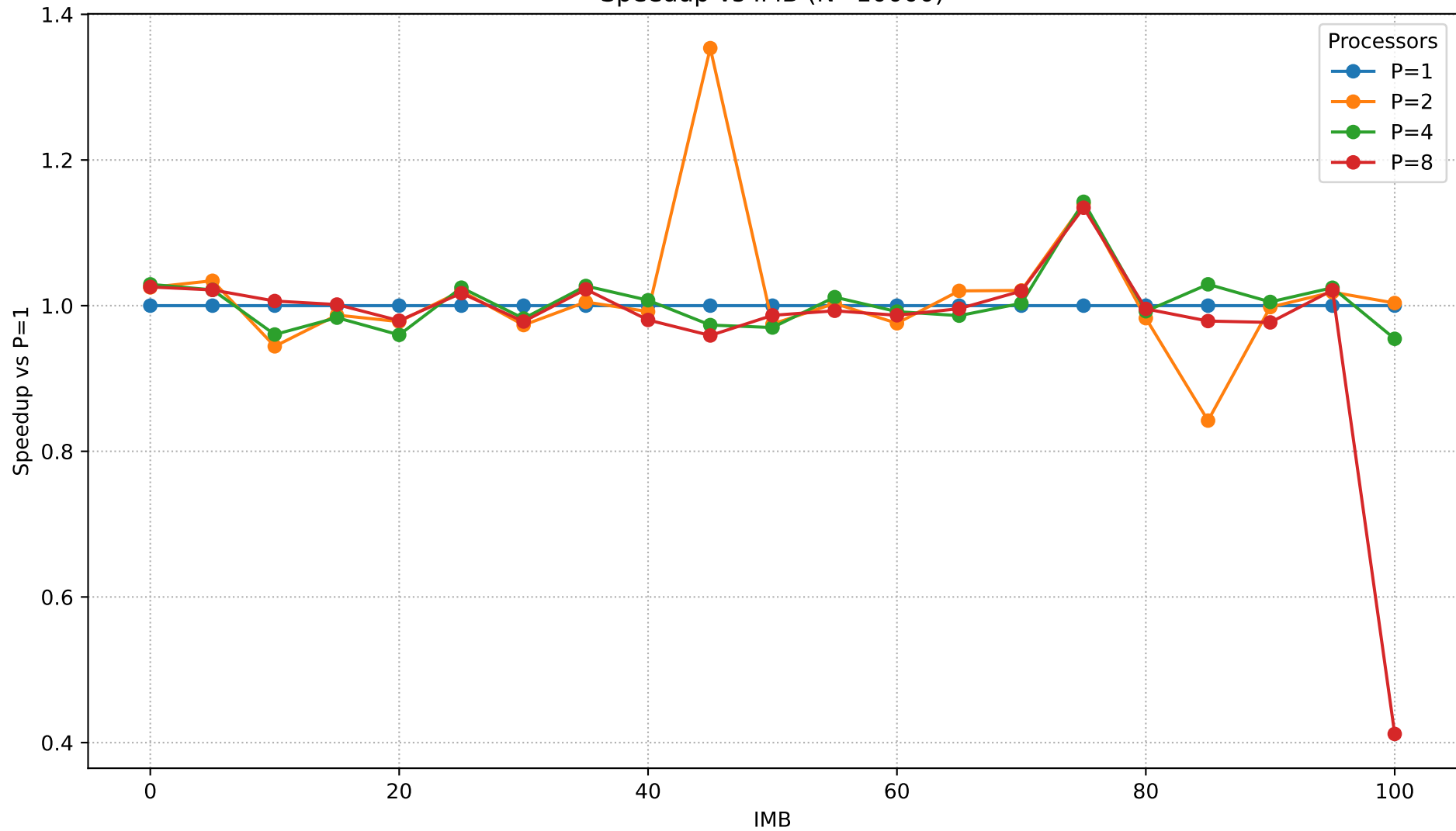
Speedup vs IMB (N=10000)
