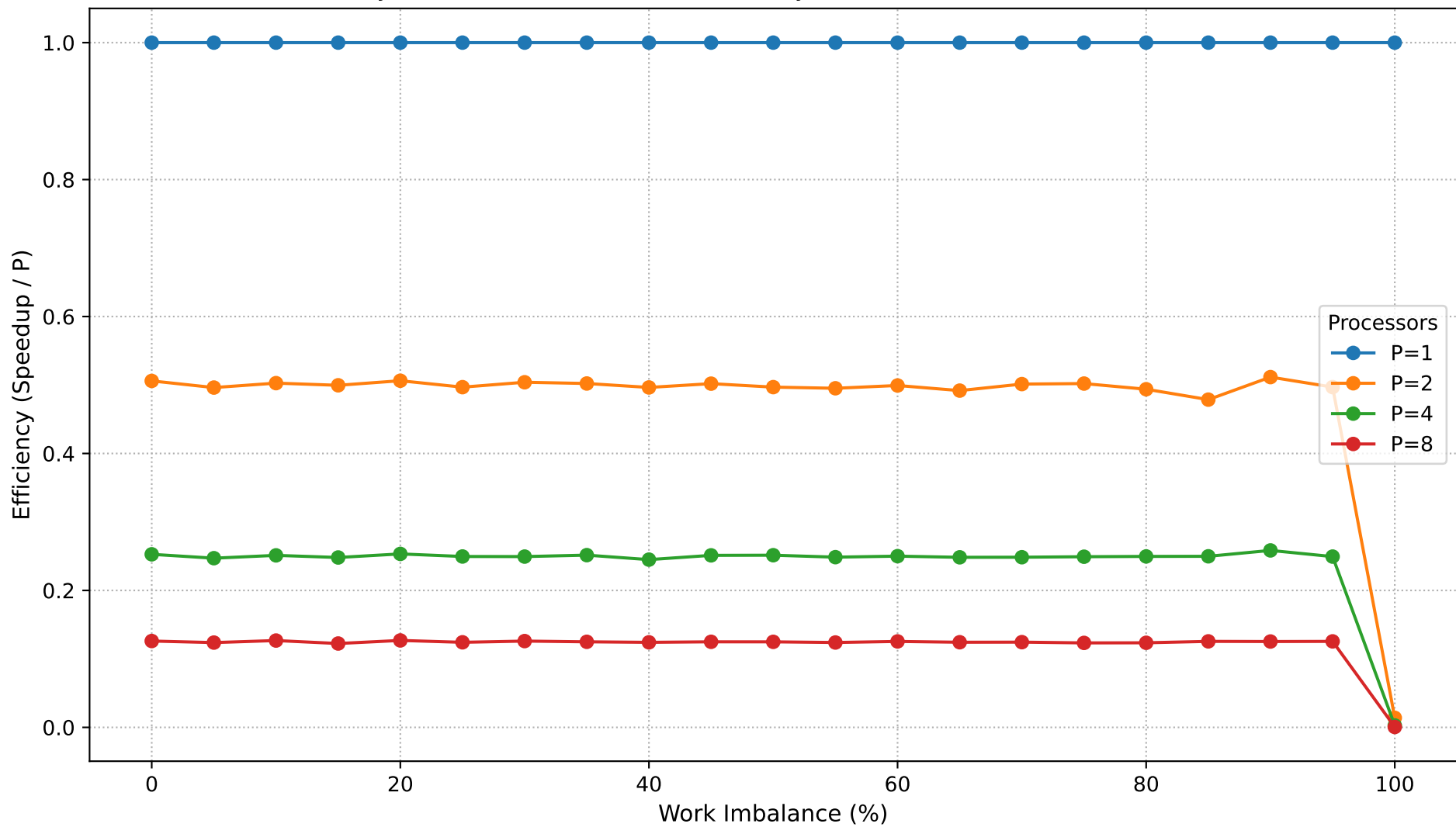
Dyck Path Validation: Parallel Efficiency vs Work Imbalance (N=850,000)
