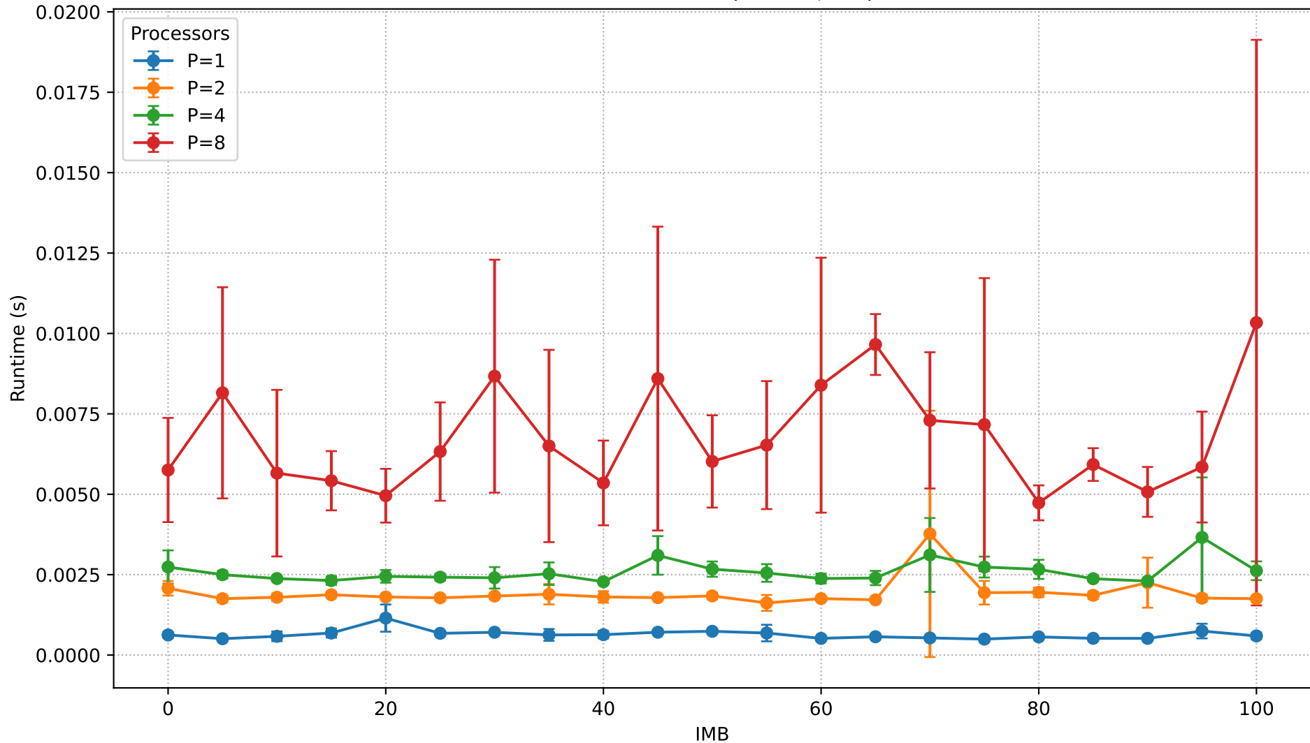
Runtime vs IMB (N=250,000)
