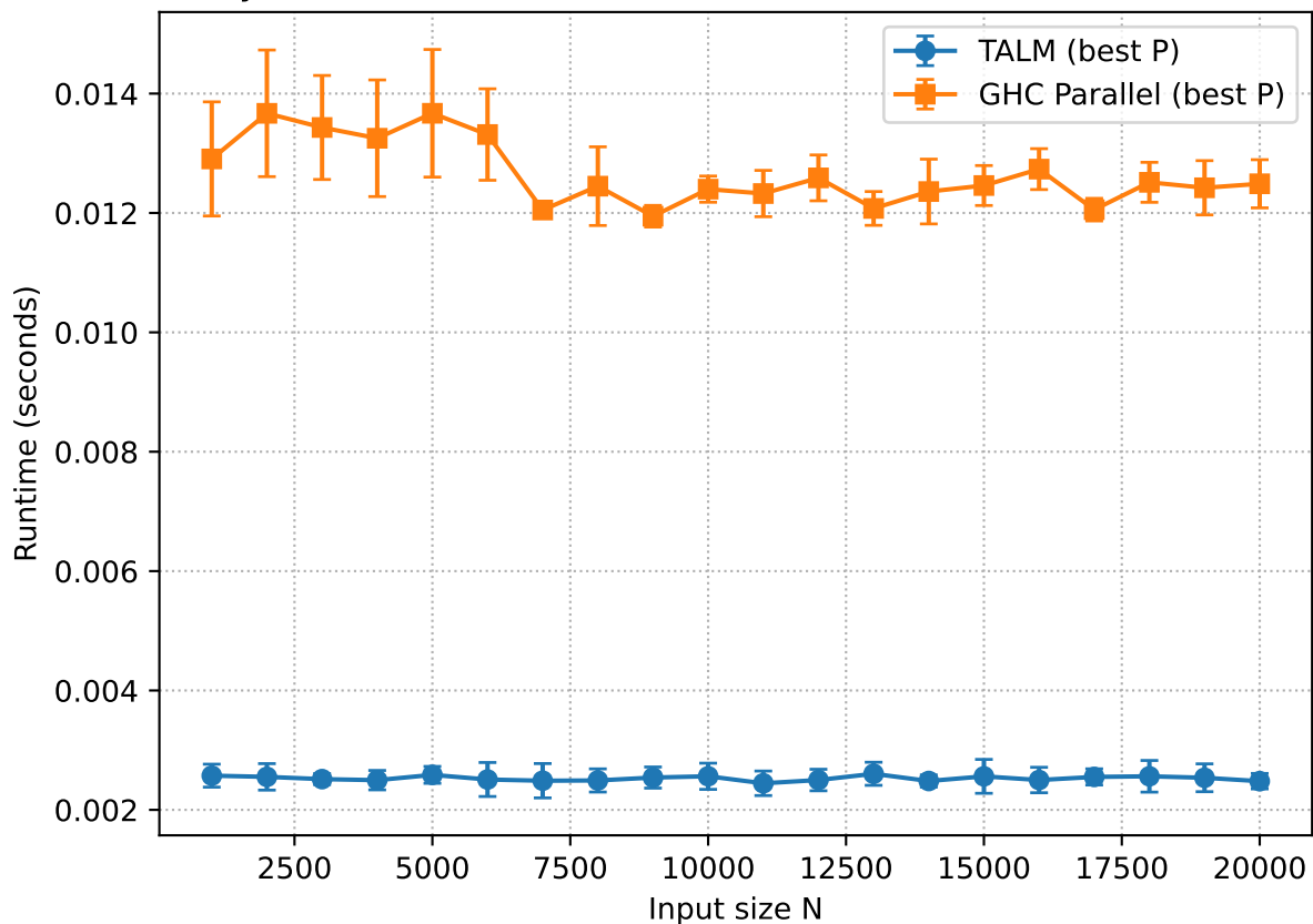
Dyck Path: Best-of-Breed Runtime vs N (imb=75, delta=0)
