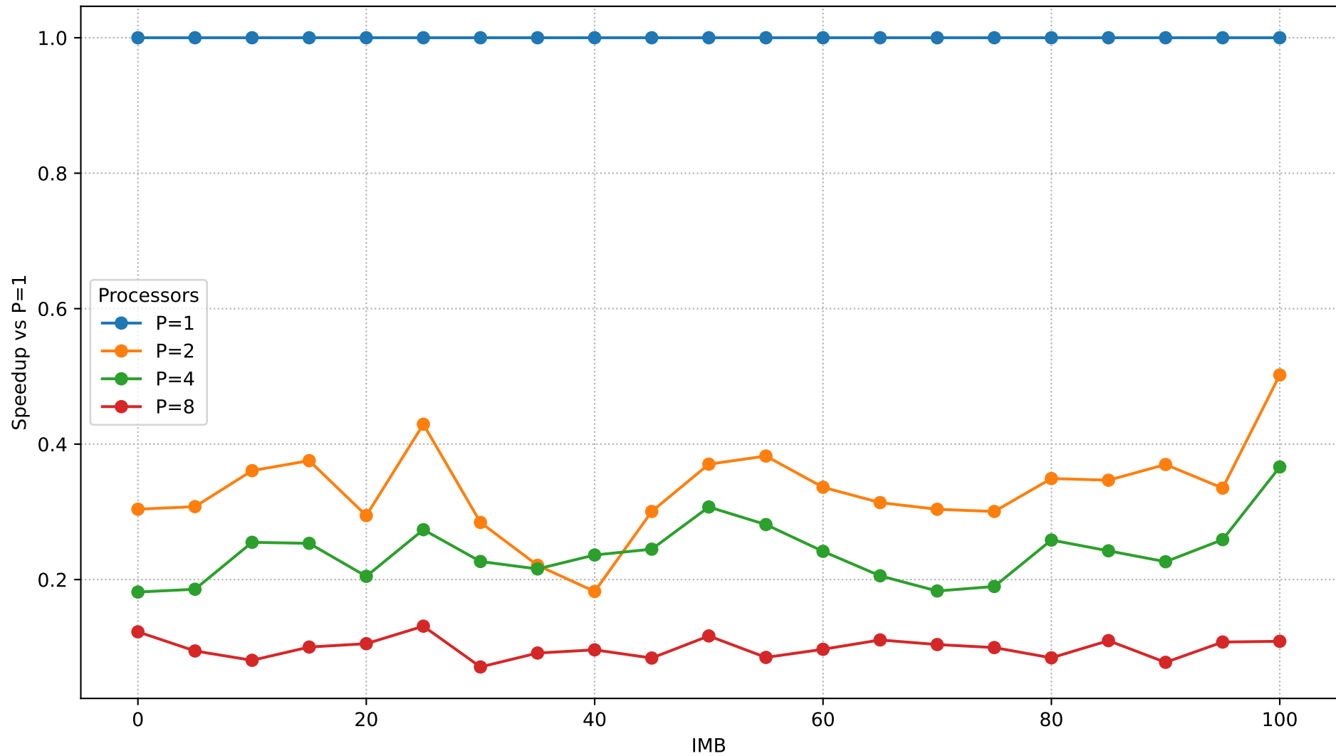
Speedup vs IMB (N=350,000)
