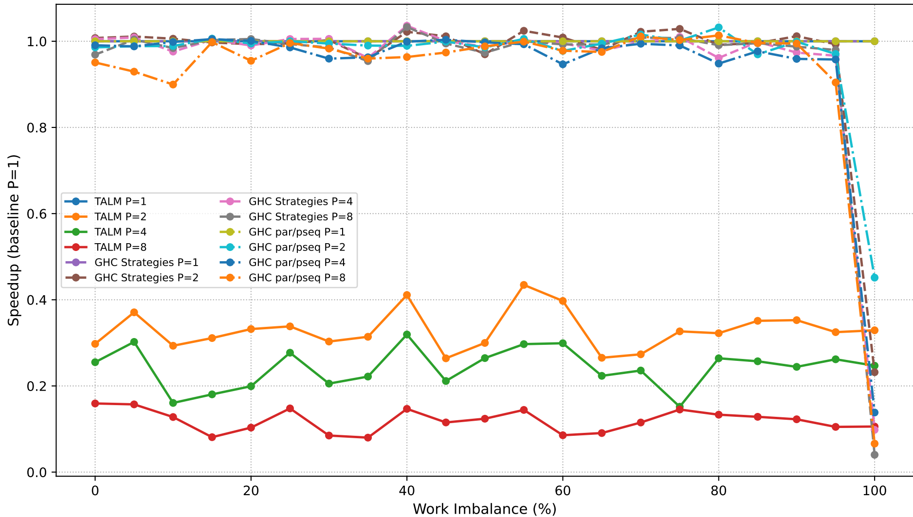
Dyck Path Validation: Speedup Comparison (N=100,000)
