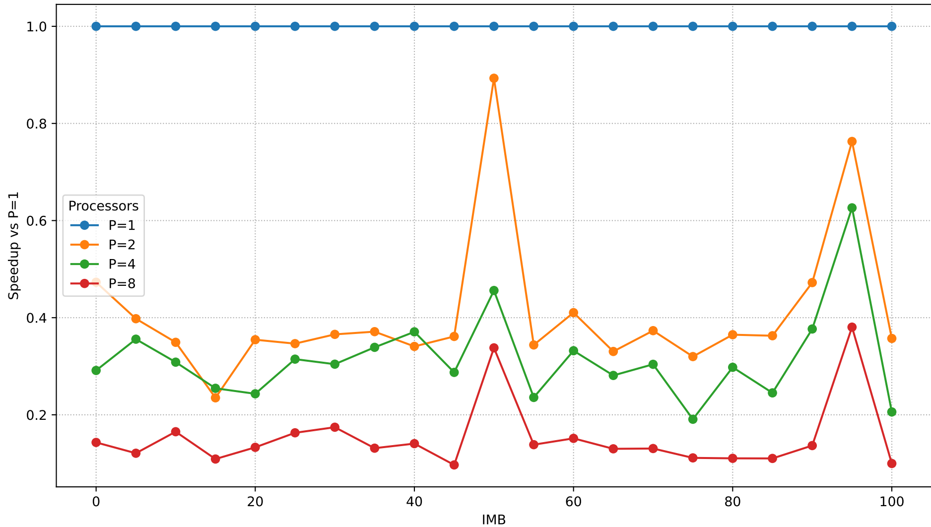
Speedup vs IMB (N=850,000)
