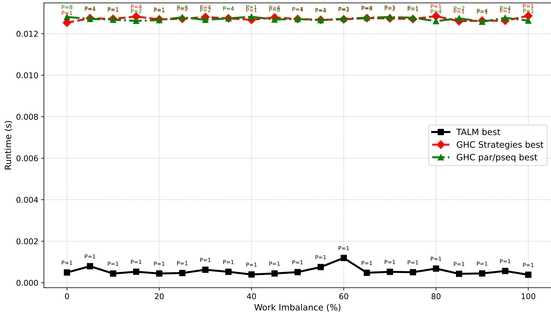
Dyck Path Validation: Best Runtime per System (N=100,000)
