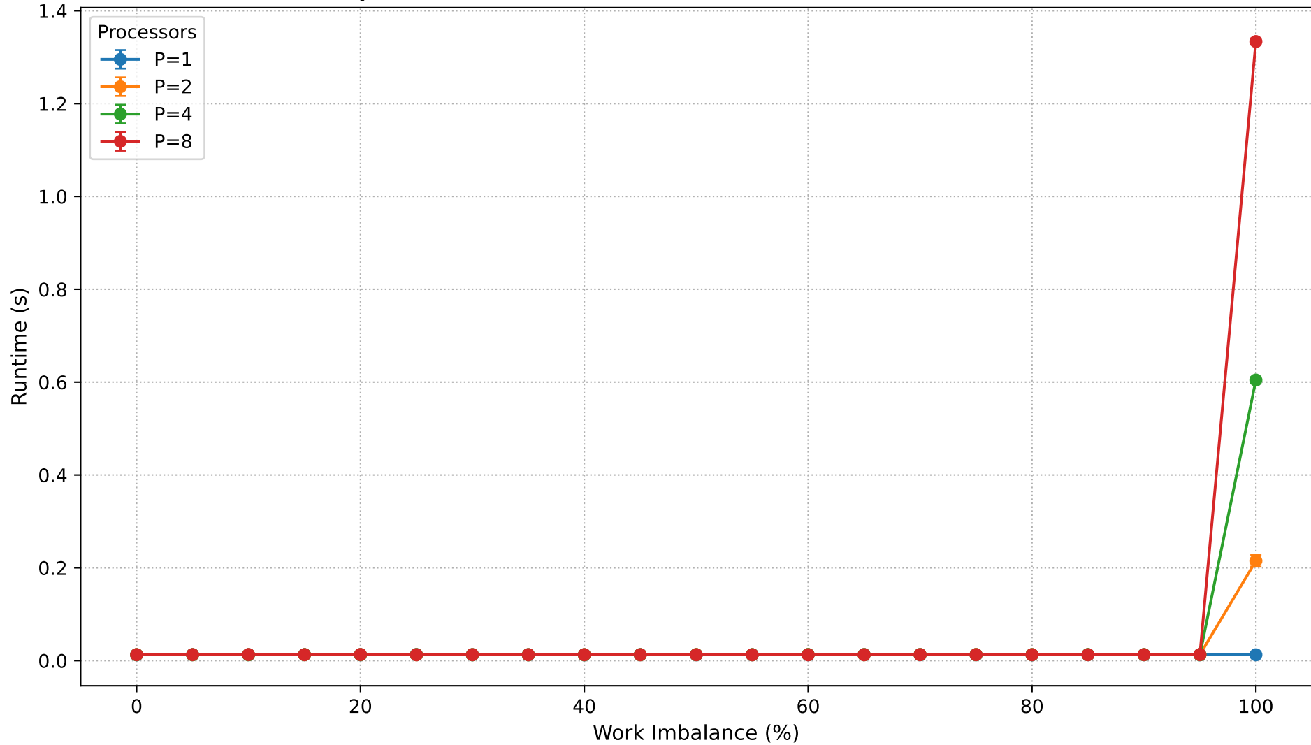
Dyck Path Validation: Runtime vs Work Imbalance (N=950,000)
