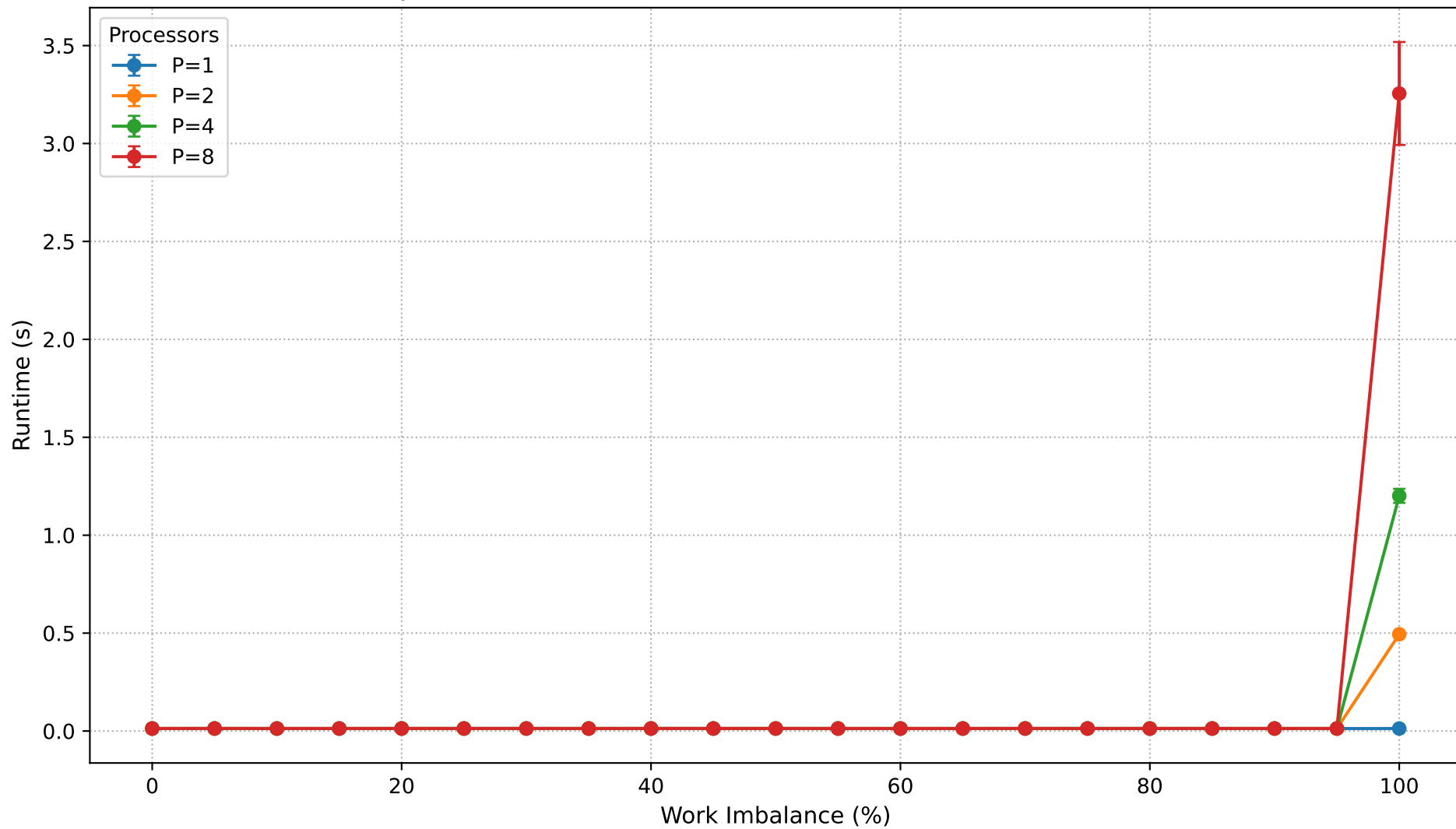
Dyck Path Validation: Runtime vs Work Imbalance (N=900,000)
