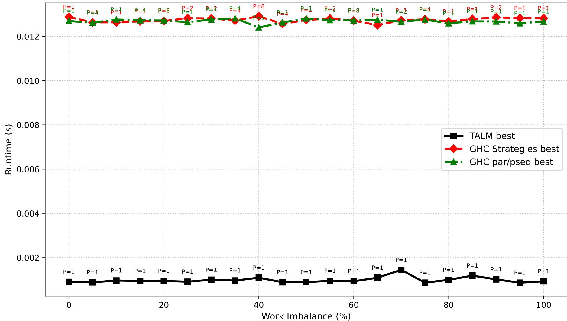
Dyck Path Validation: Best Runtime per System (N=1,000,000)
