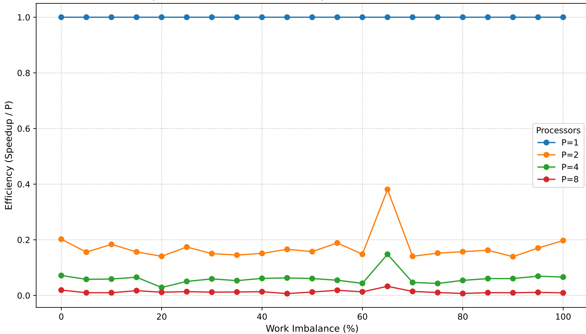
Dyck Path Validation: Parallel Efficiency vs Work Imbalance (N=400,000)
