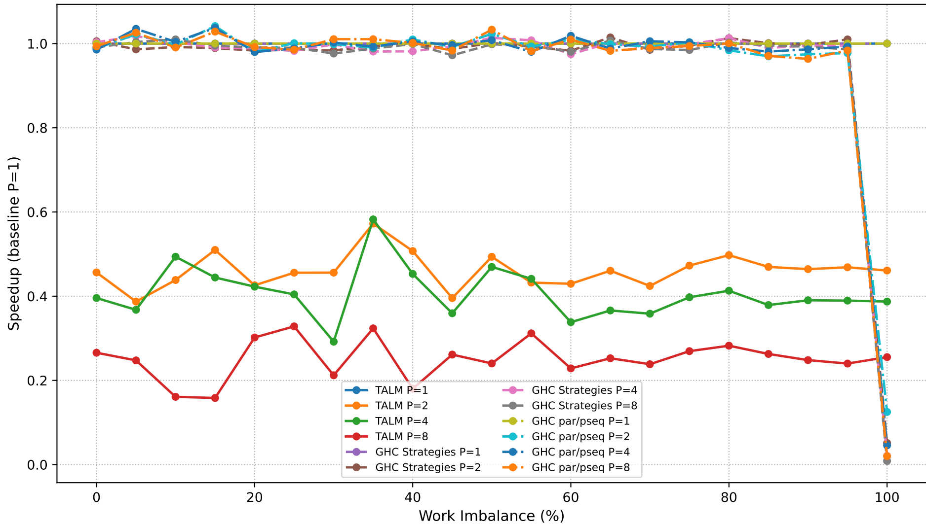
Dyck Path Validation: Speedup Comparison (N=450,000)
