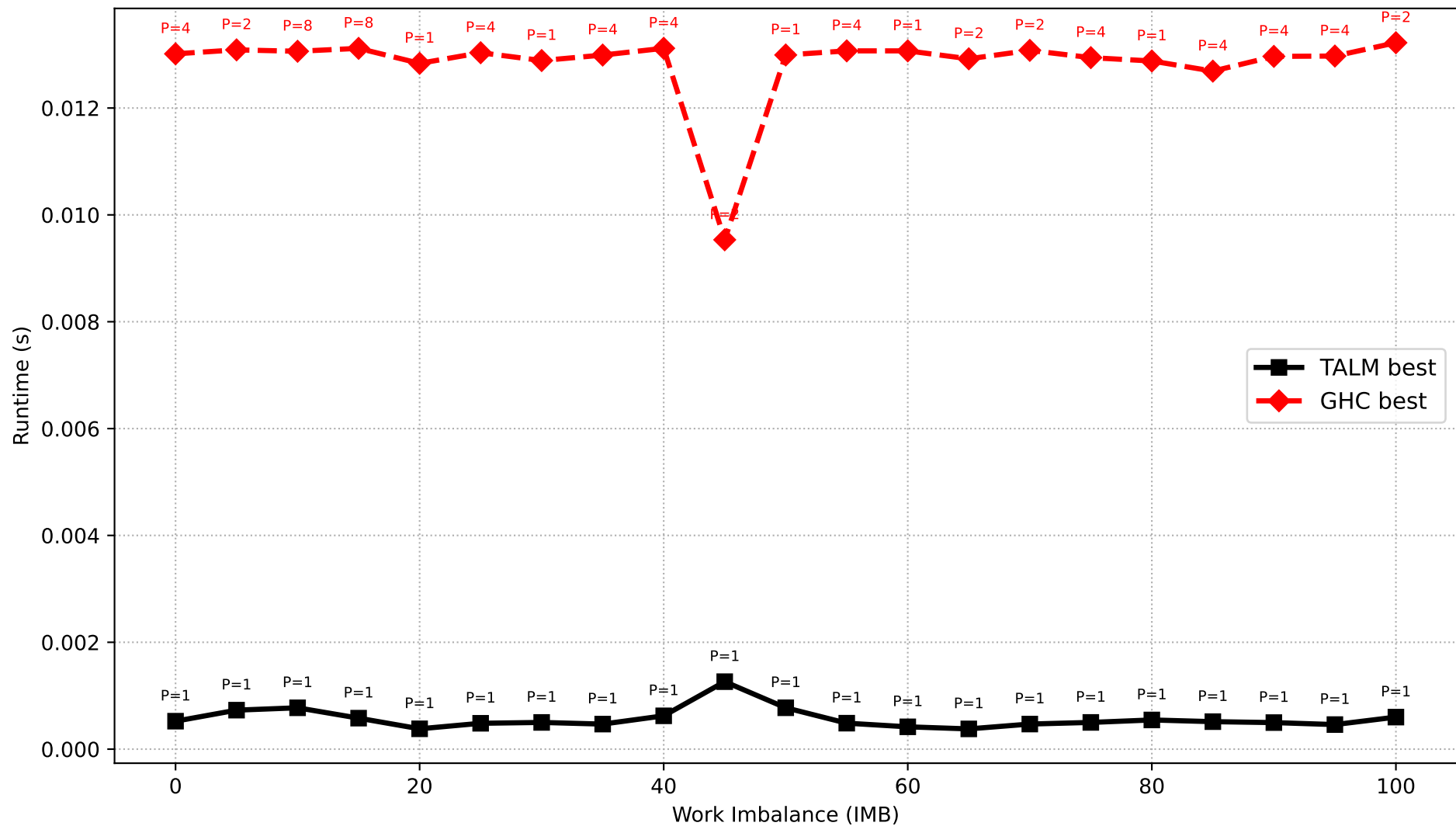
Best TALM vs Best GHC - Runtime (N=10000)
