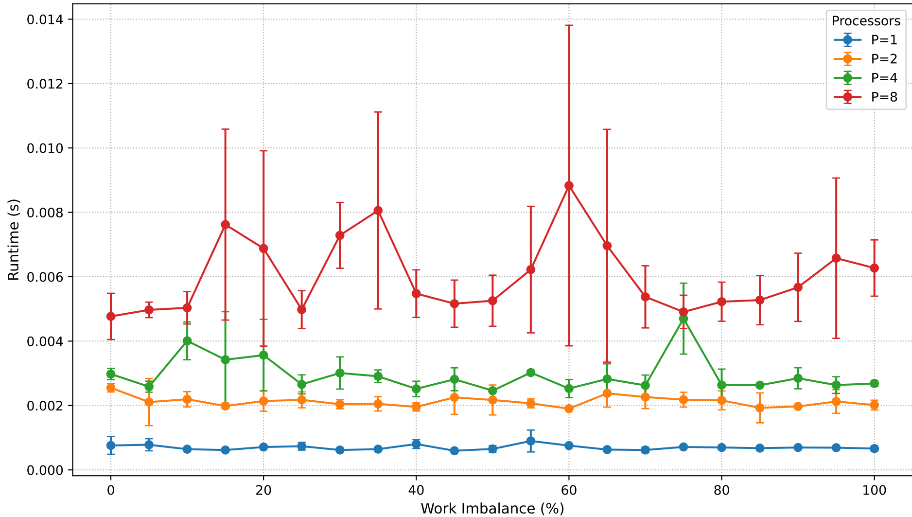
Dyck Path Validation: Runtime vs Work Imbalance (N=100,000)
