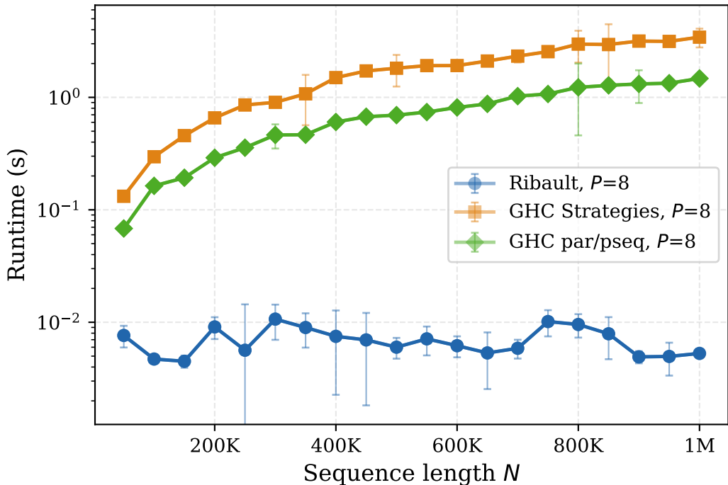
Dyck Paths: Worst-Case Scaling ( P = 8 , 100% Imbalance)
