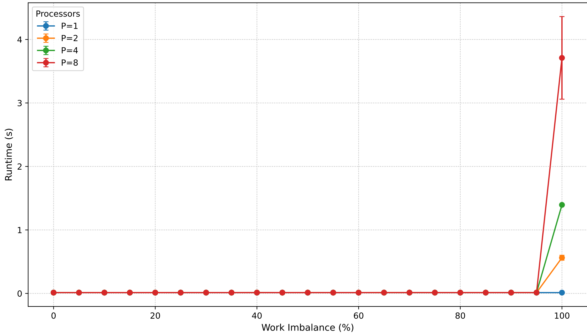
Dyck Path Validation: Runtime vs Work Imbalance (N=1,000,000)
