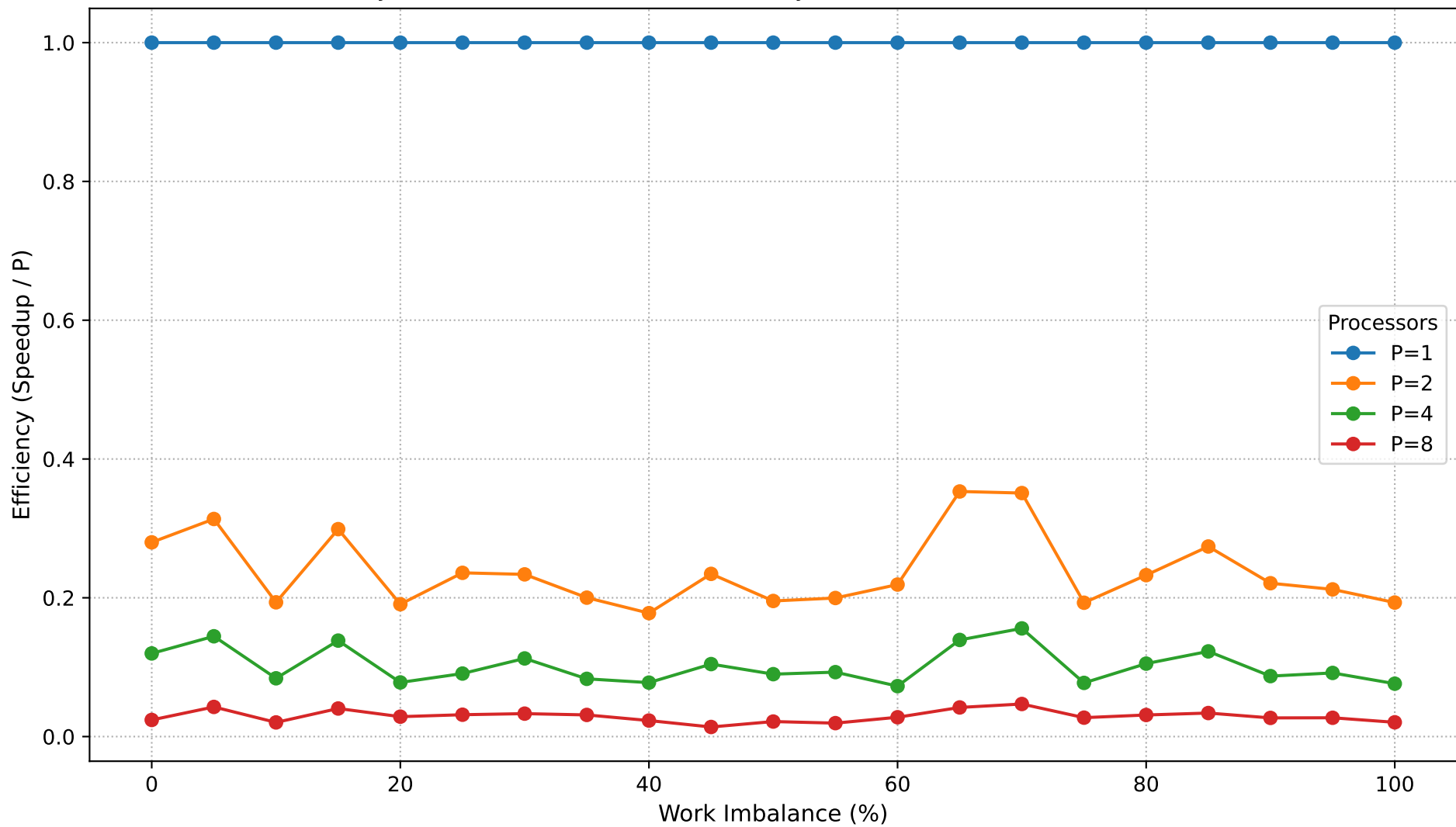
Dyck Path Validation: Parallel Efficiency vs Work Imbalance (N=300,000)
