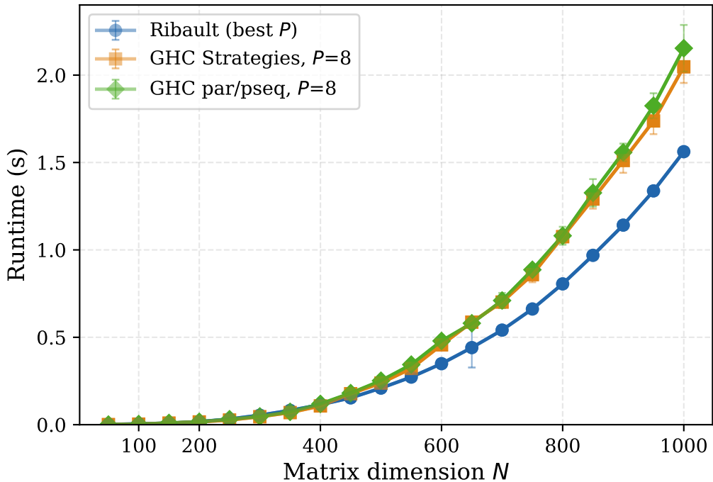
Matrix Multiply: Best Runtime per System
