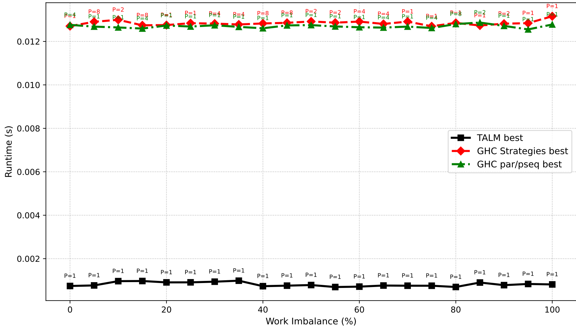
Dyck Path Validation: Best Runtime per System (N=650,000)
