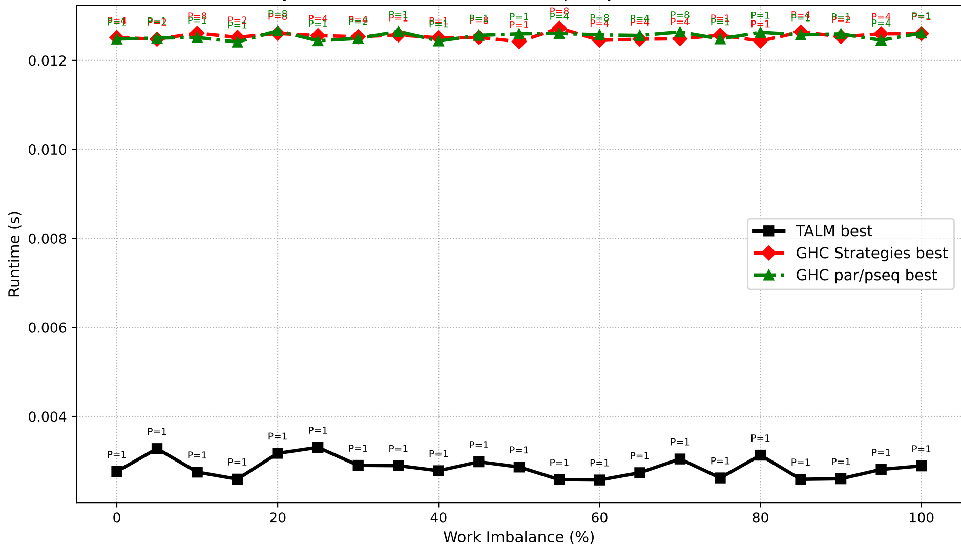
Dyck Path Validation: Best Runtime per System (N=900,000)
