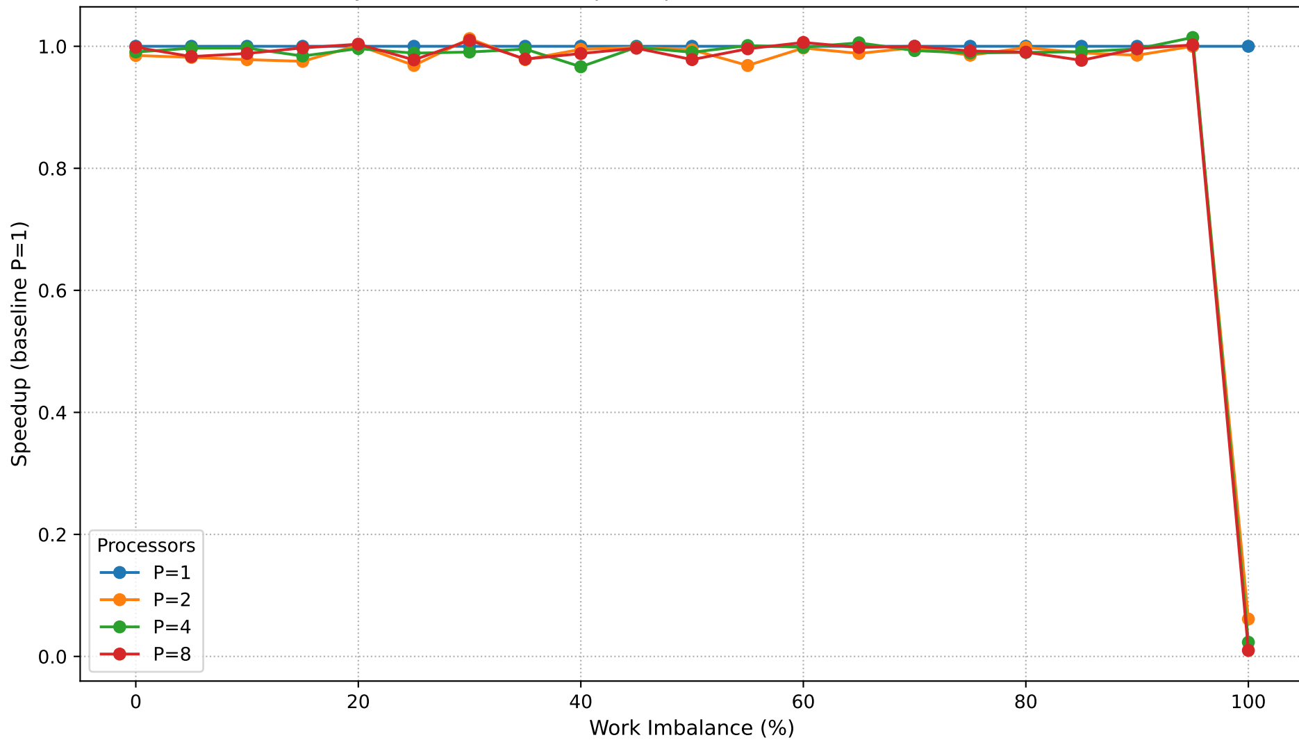
Dyck Path Validation: Speedup vs Work Imbalance (N=900,000)
