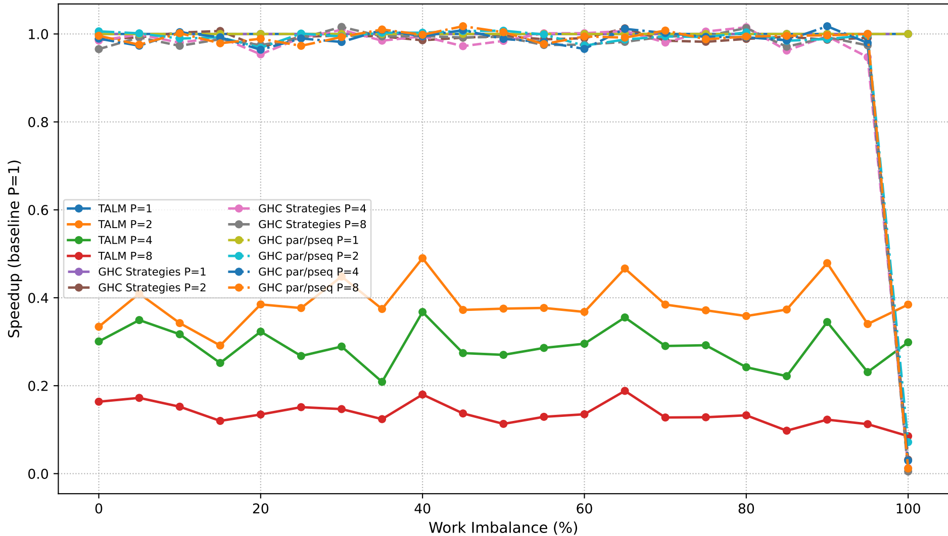
Dyck Path Validation: Speedup Comparison (N=750,000)
