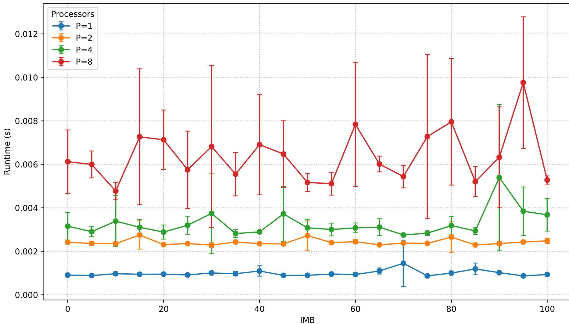
Runtime vs IMB (N=1,000,000)
