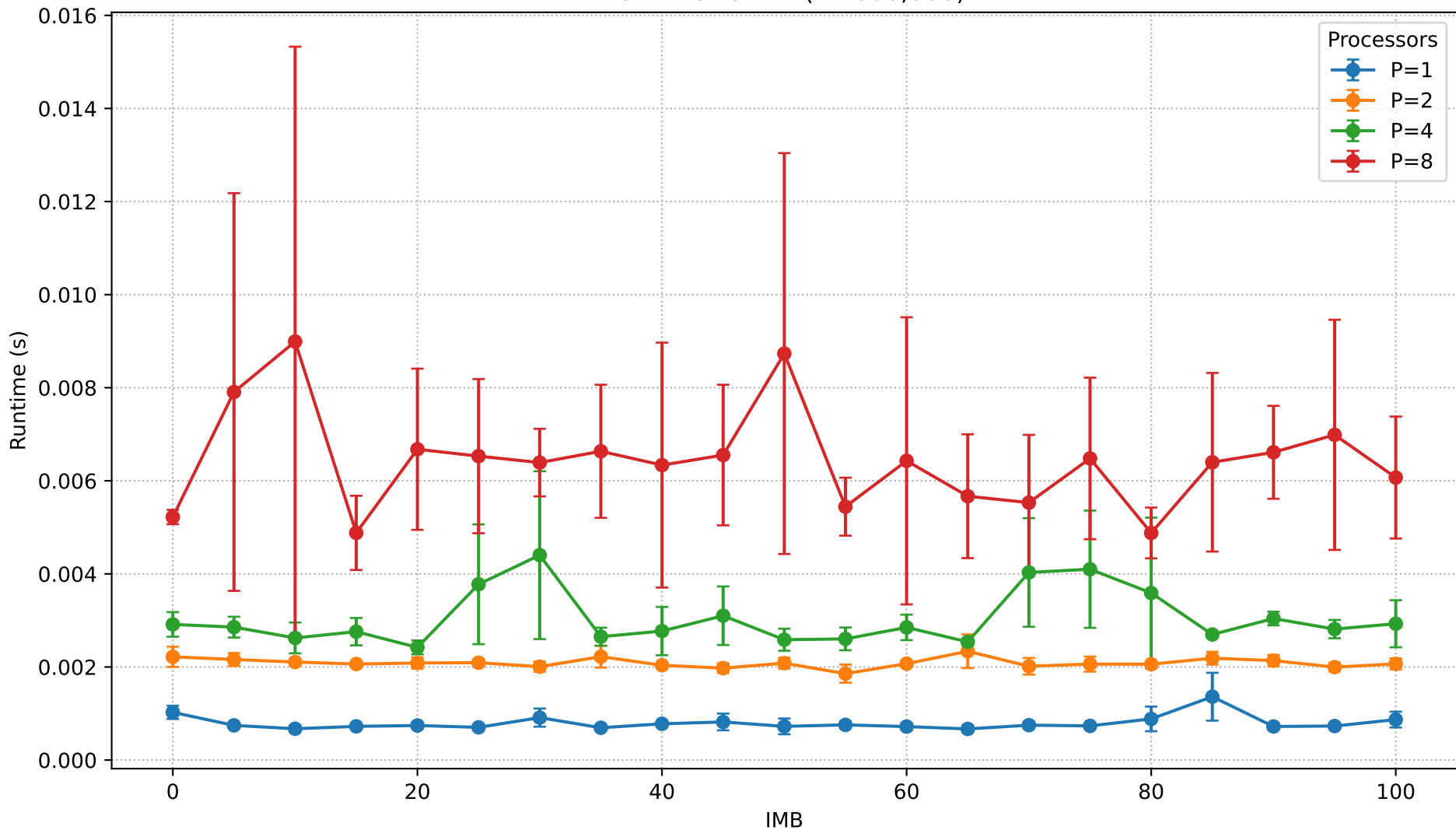
Runtime vs IMB (N=600,000)
