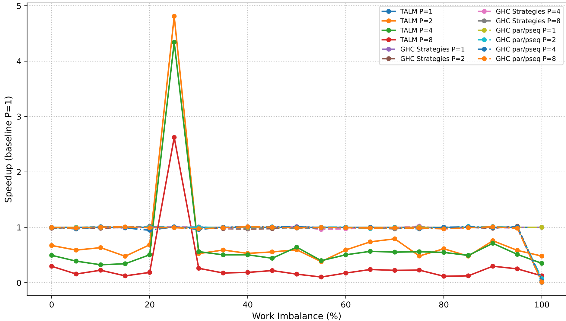
Dyck Path Validation: Speedup Comparison (N=700,000)
