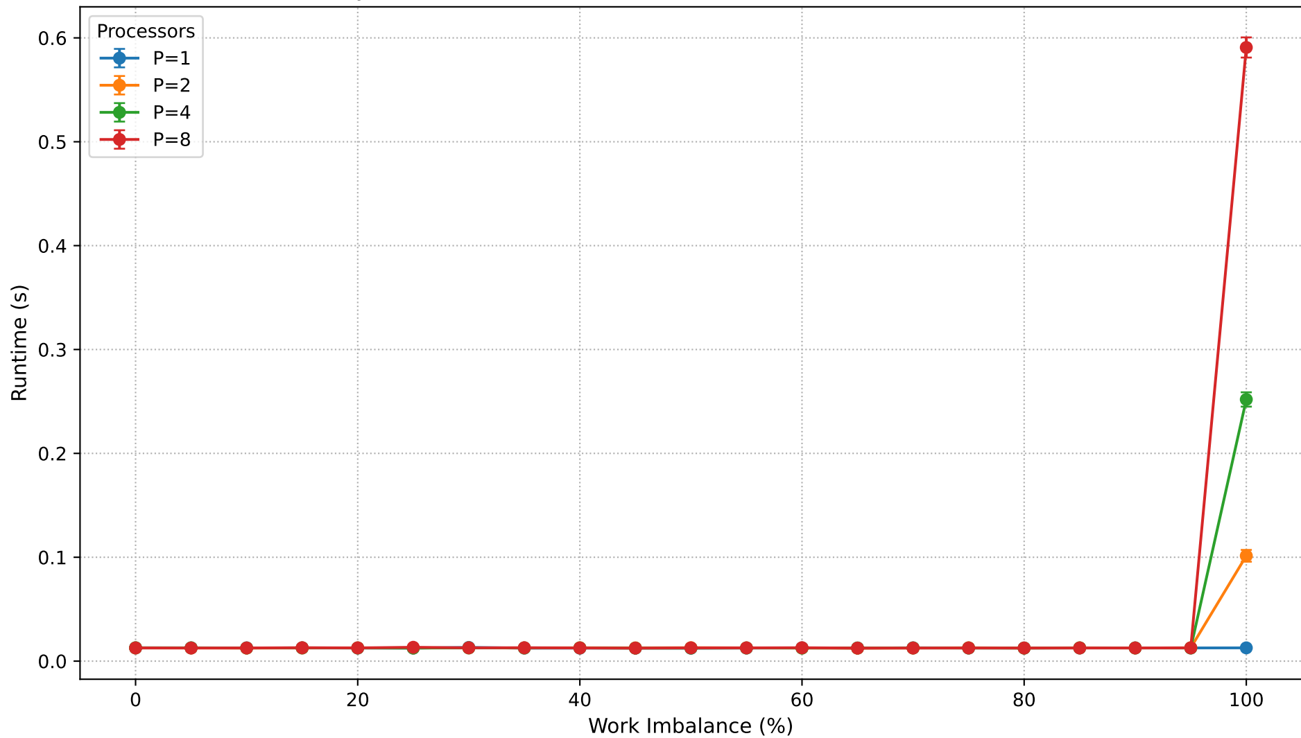
Dyck Path Validation: Runtime vs Work Imbalance (N=400,000)
