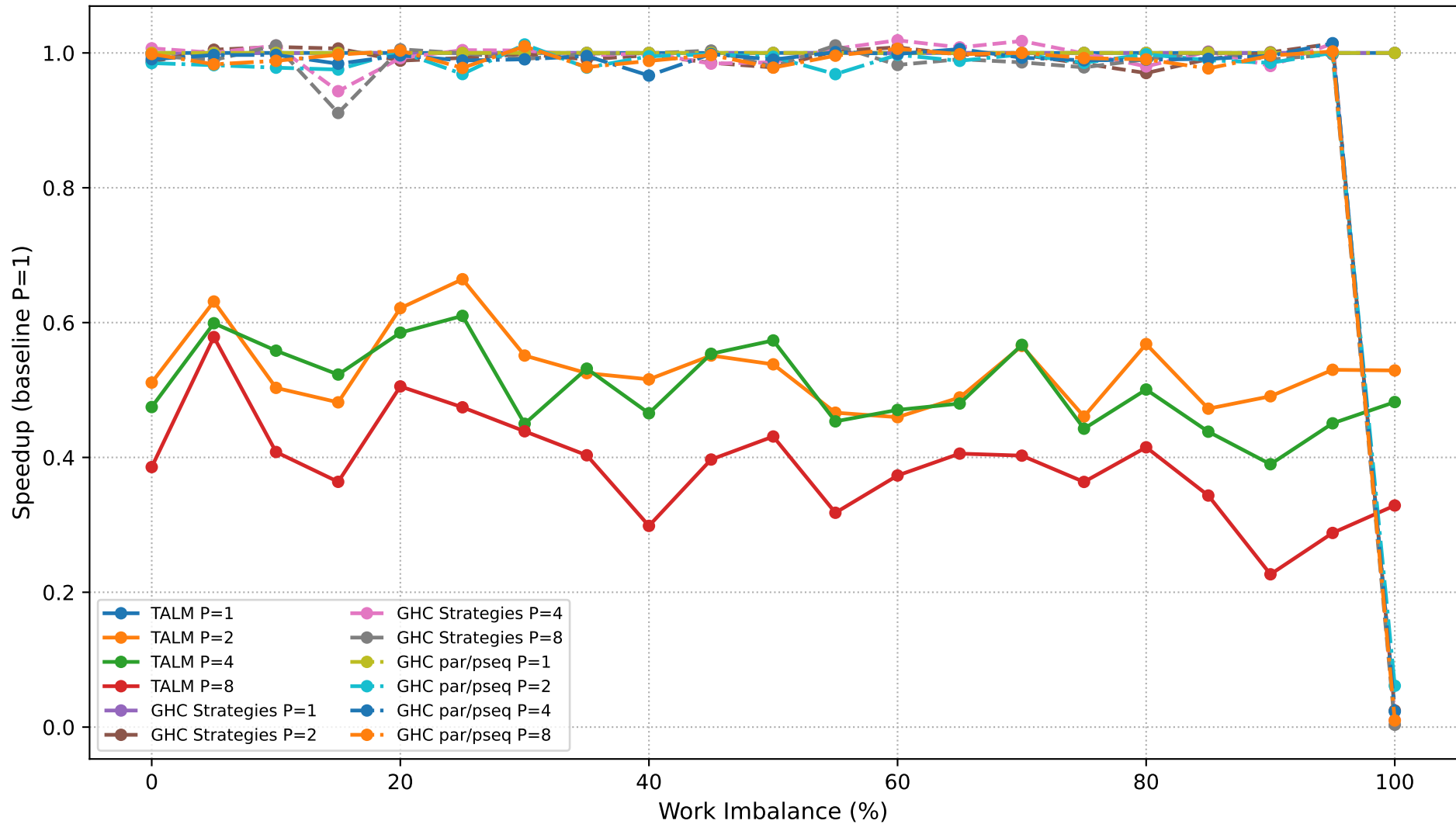
Dyck Path Validation: Speedup Comparison (N=900,000)
