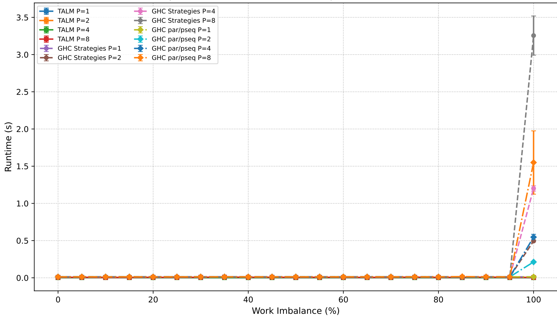
Dyck Path Validation: Runtime Comparison (N=900,000)
