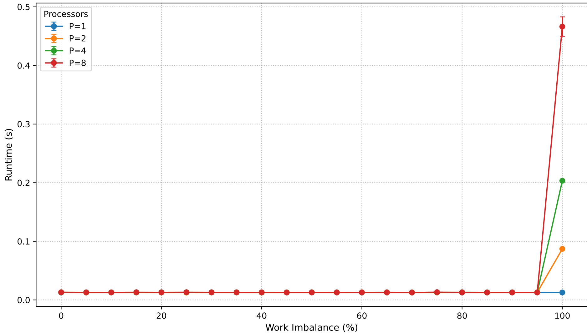
Dyck Path Validation: Runtime vs Work Imbalance (N=150,000)
