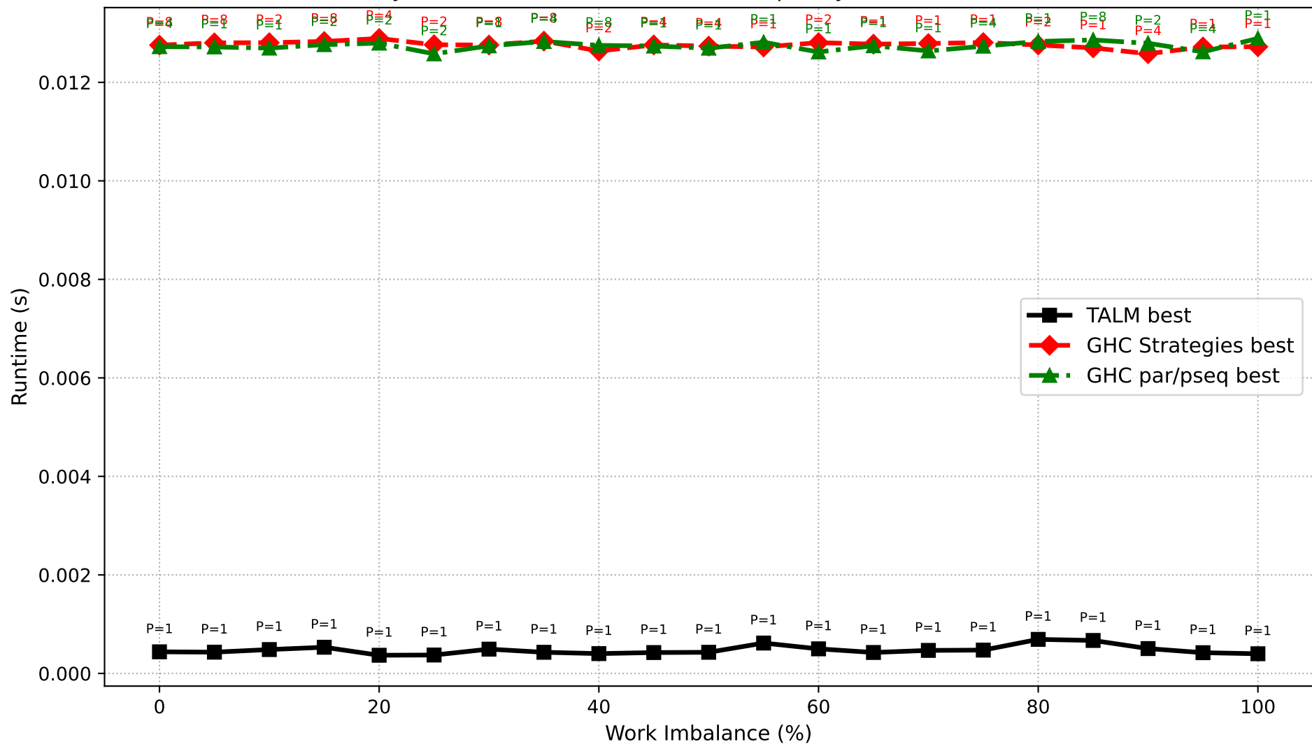
Dyck Path Validation: Best Runtime per System (N=50,000)
