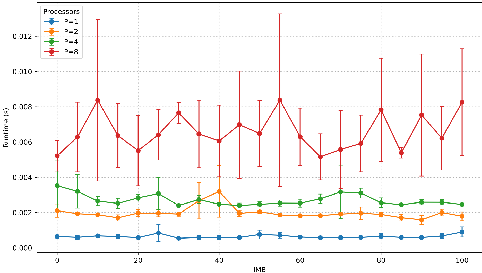
Runtime vs IMB (N=350,000)
