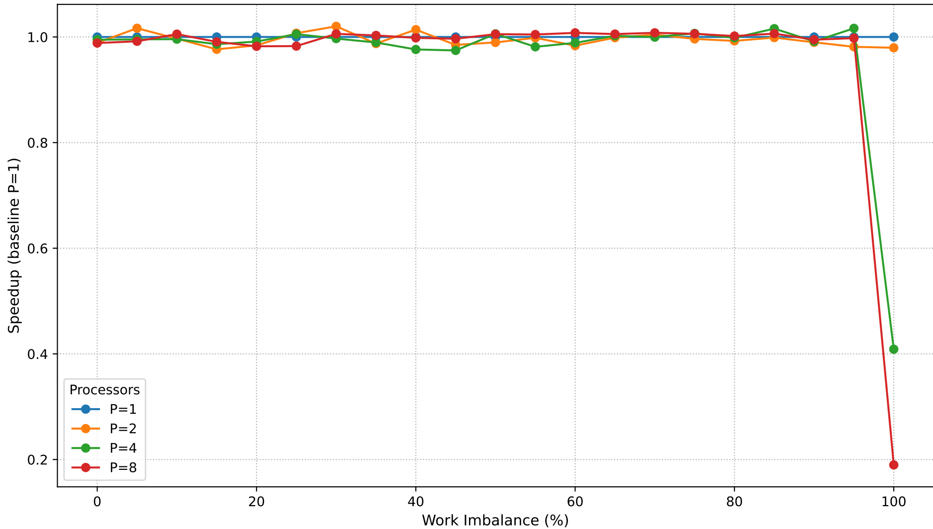
Dyck Path Validation: Speedup vs Work Imbalance (N=50,000)
