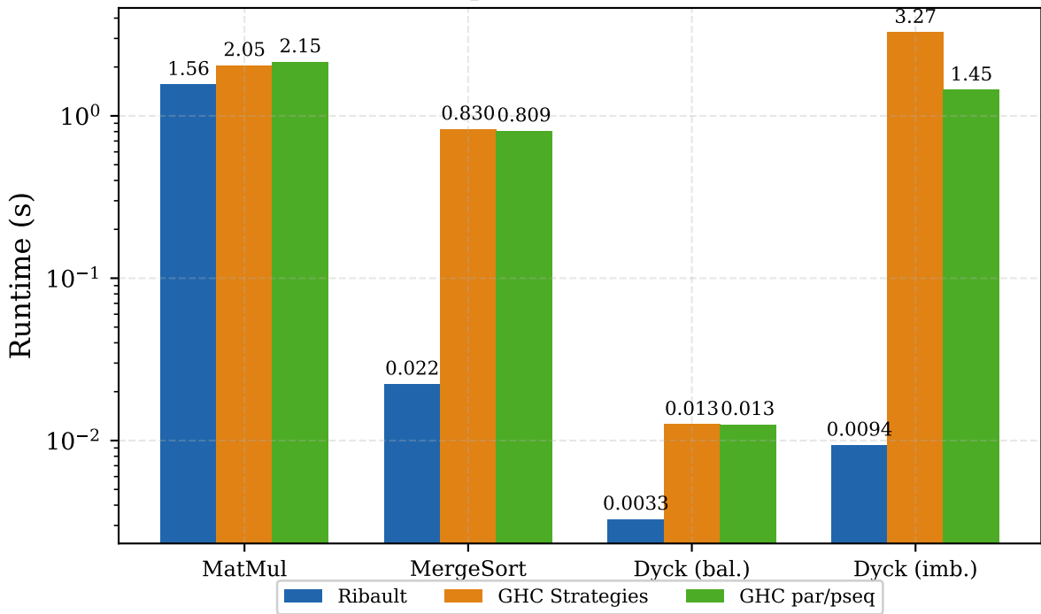
Runtime Comparison Across Benchmarks
