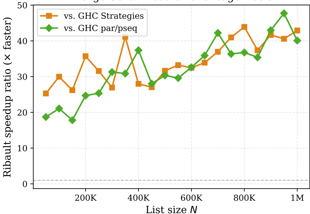
Merge Sort: Ribault Advantage Ratio
