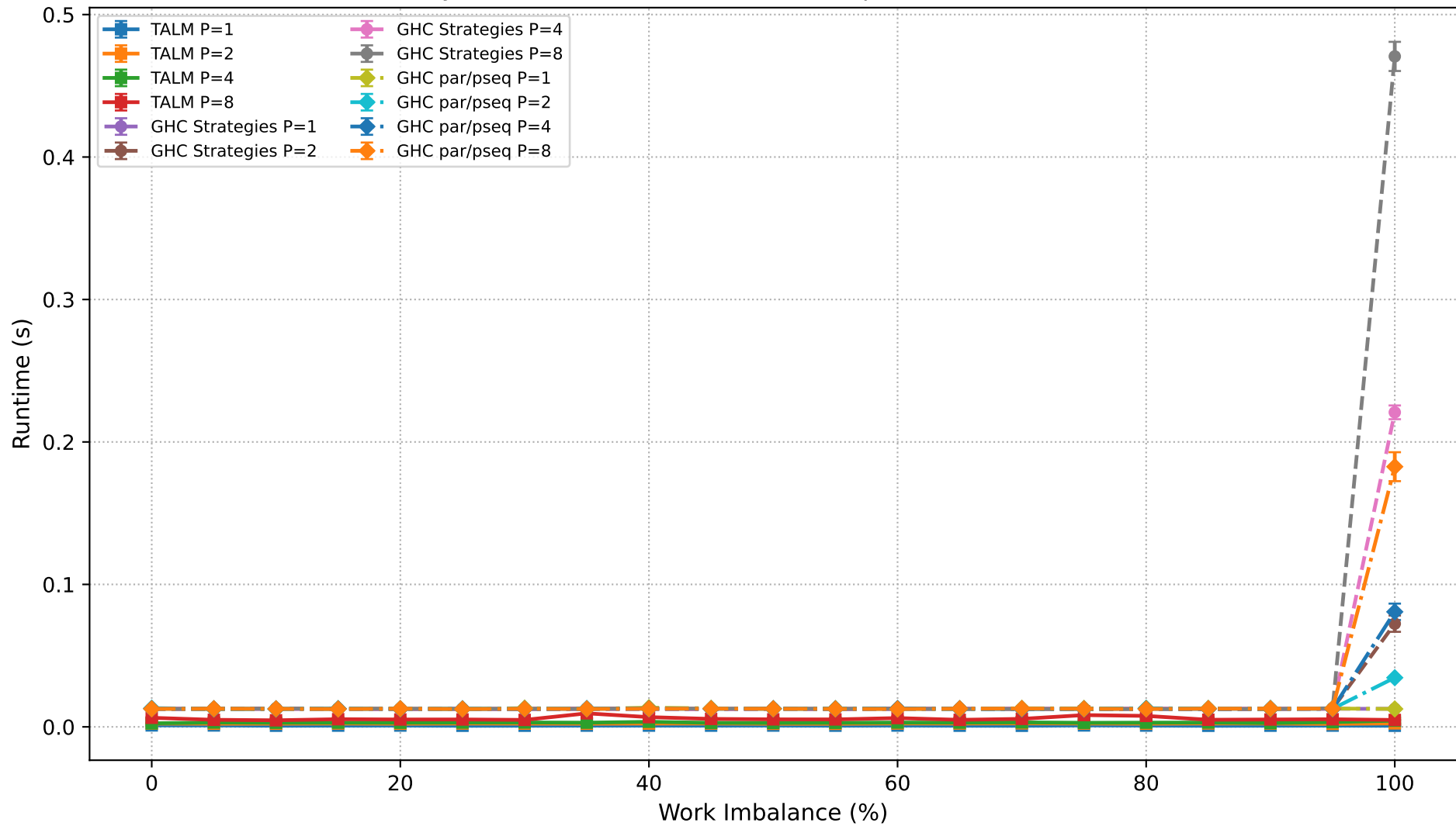
Dyck Path Validation: Runtime Comparison (N=150,000)
