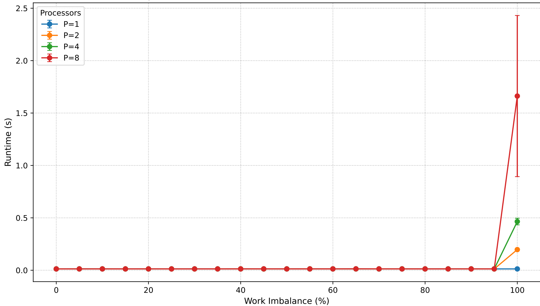
Dyck Path Validation: Runtime vs Work Imbalance (N=800,000)
