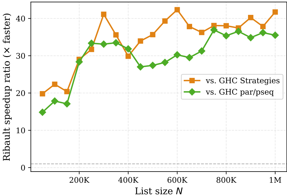
Merge Sort: Ribault Advantage Ratio
