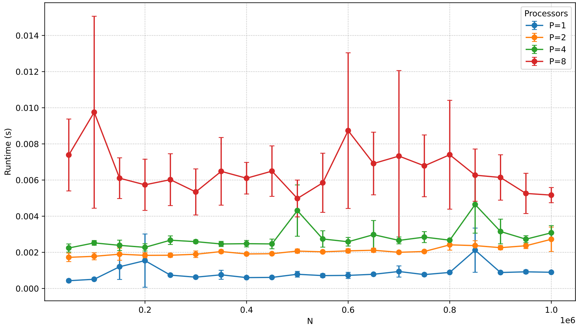
Runtime vs N (IMB=50)
