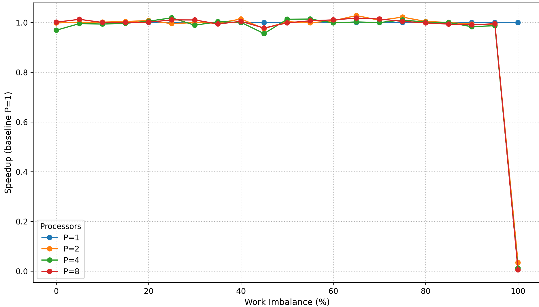
Dyck Path Validation: Speedup vs Work Imbalance (N=750,000)
