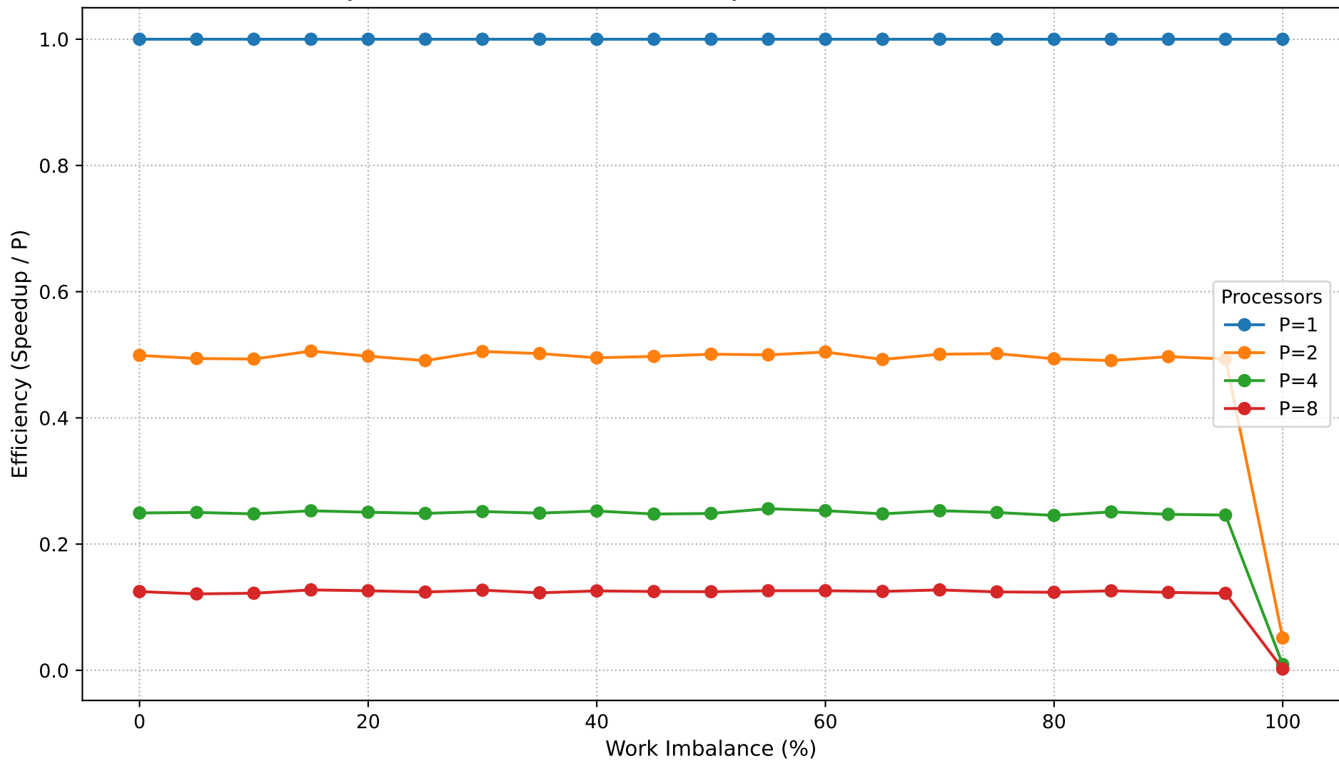
Dyck Path Validation: Parallel Efficiency vs Work Imbalance (N=550,000)
