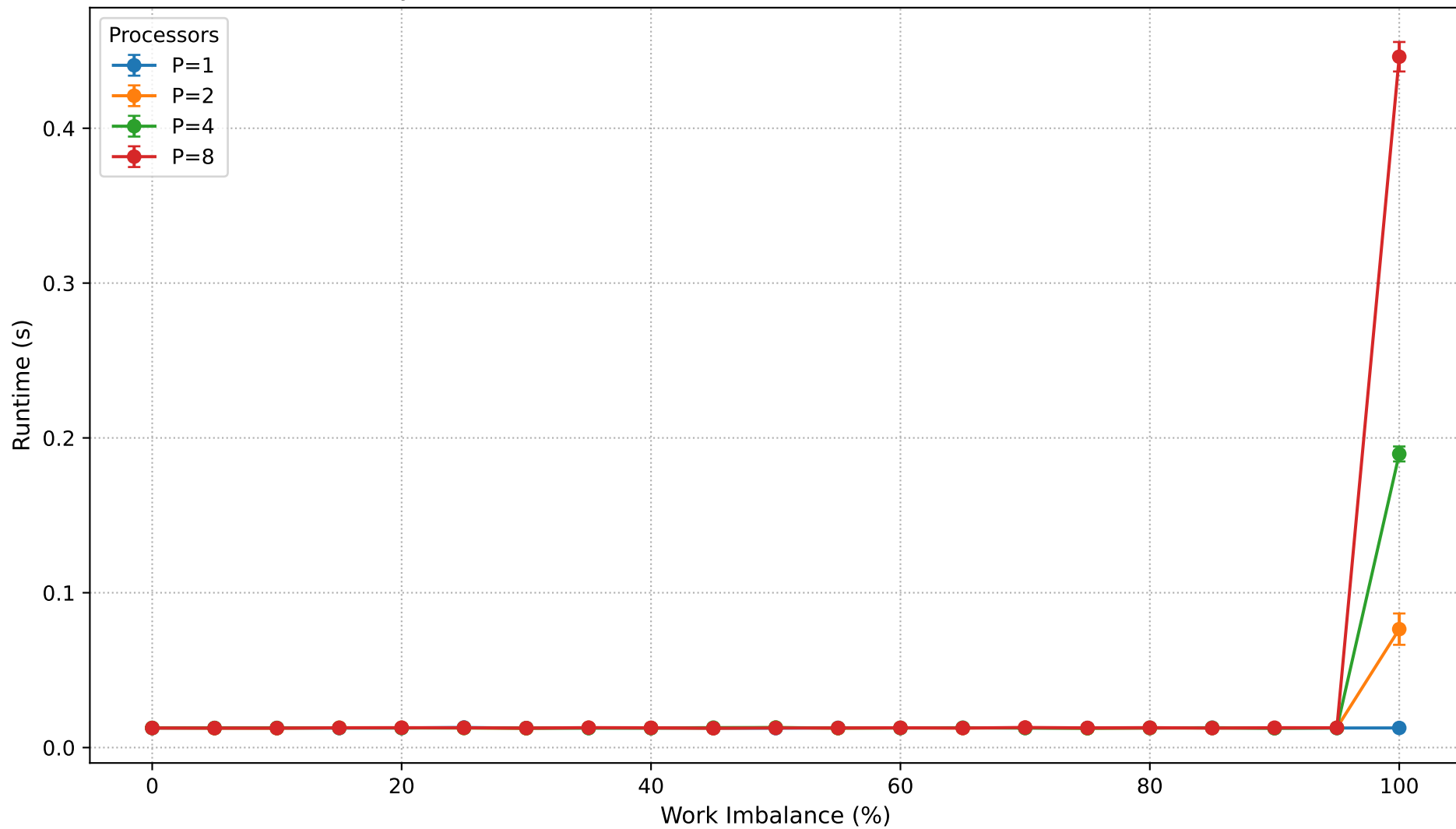
Dyck Path Validation: Runtime vs Work Imbalance (N=350,000)
