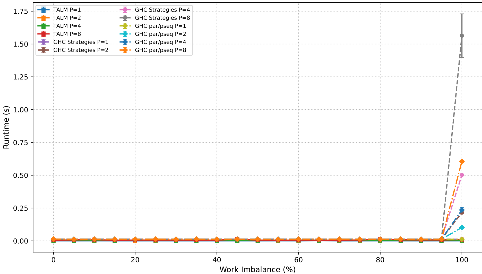
Dyck Path Validation: Runtime Comparison (N=400,000)
