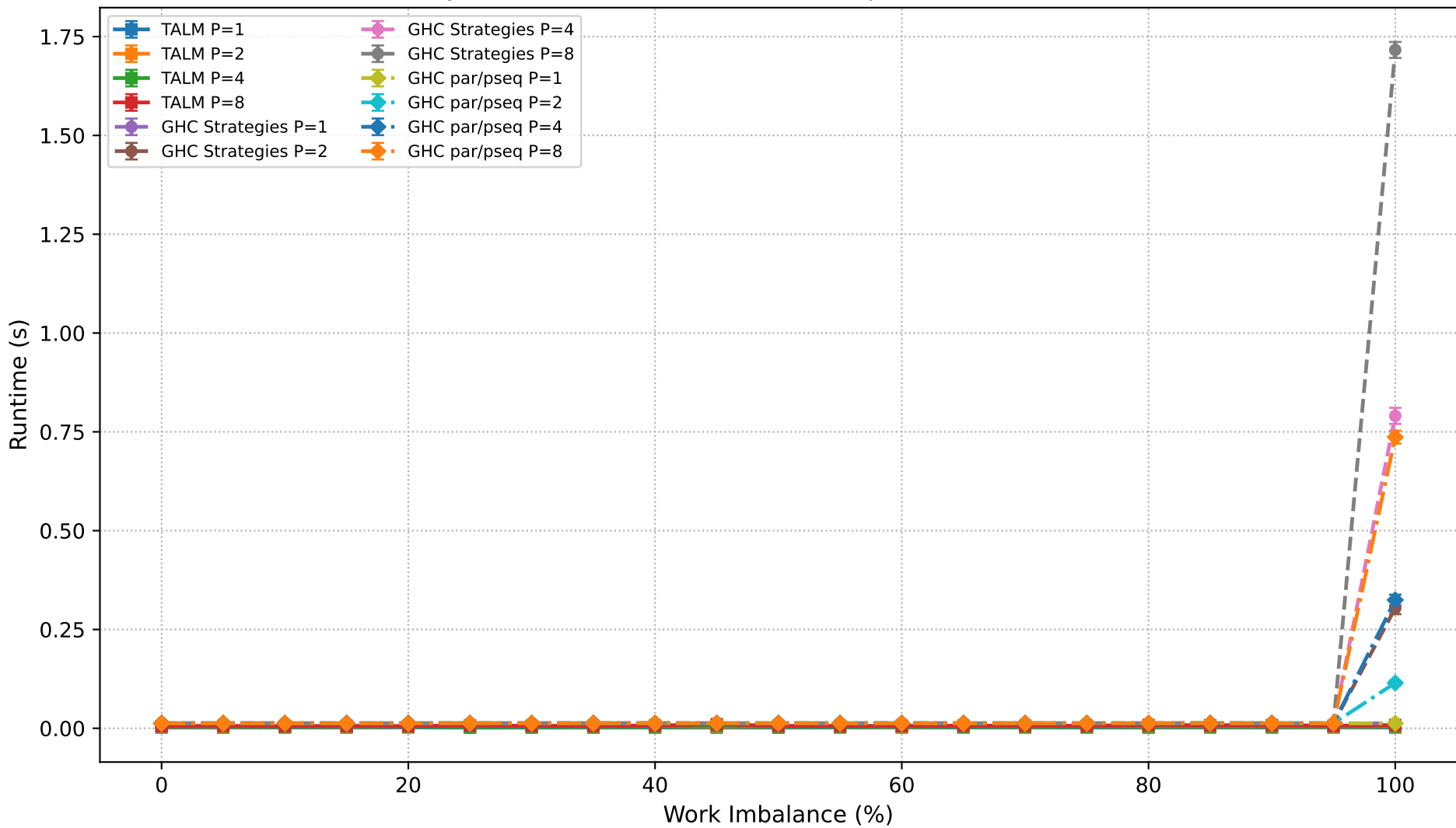
Dyck Path Validation: Runtime Comparison (N=550,000)
