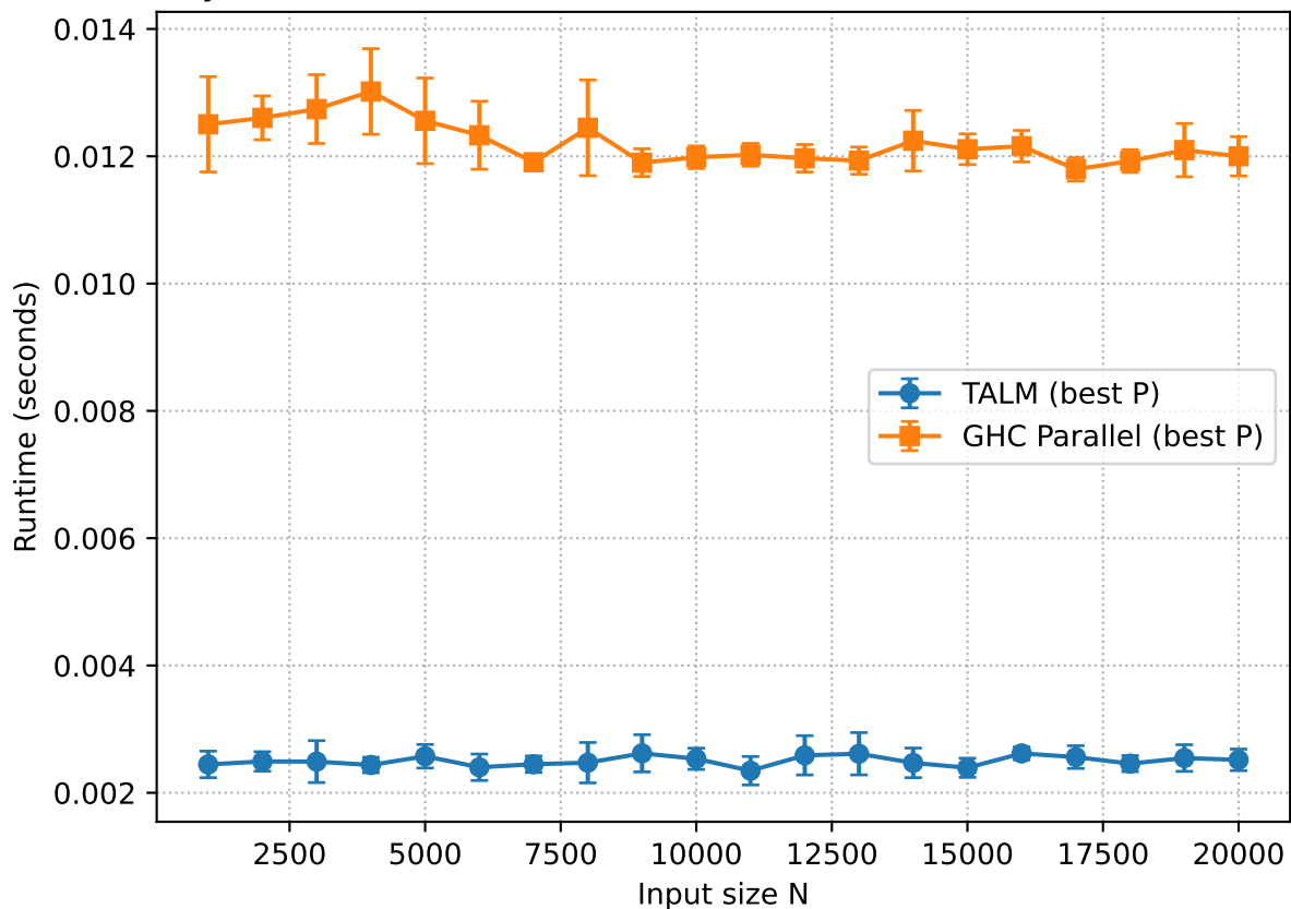
Dyck Path: Best-of-Breed Runtime vs N (imb=75, delta=5000)
