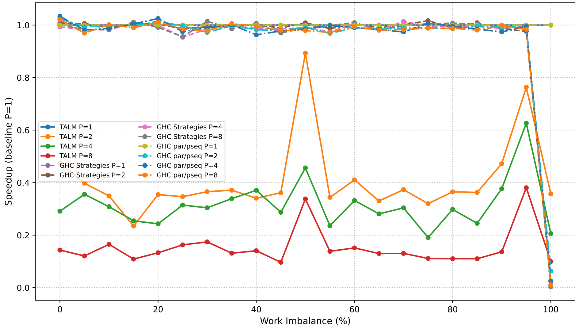
Dyck Path Validation: Speedup Comparison (N=850,000)
