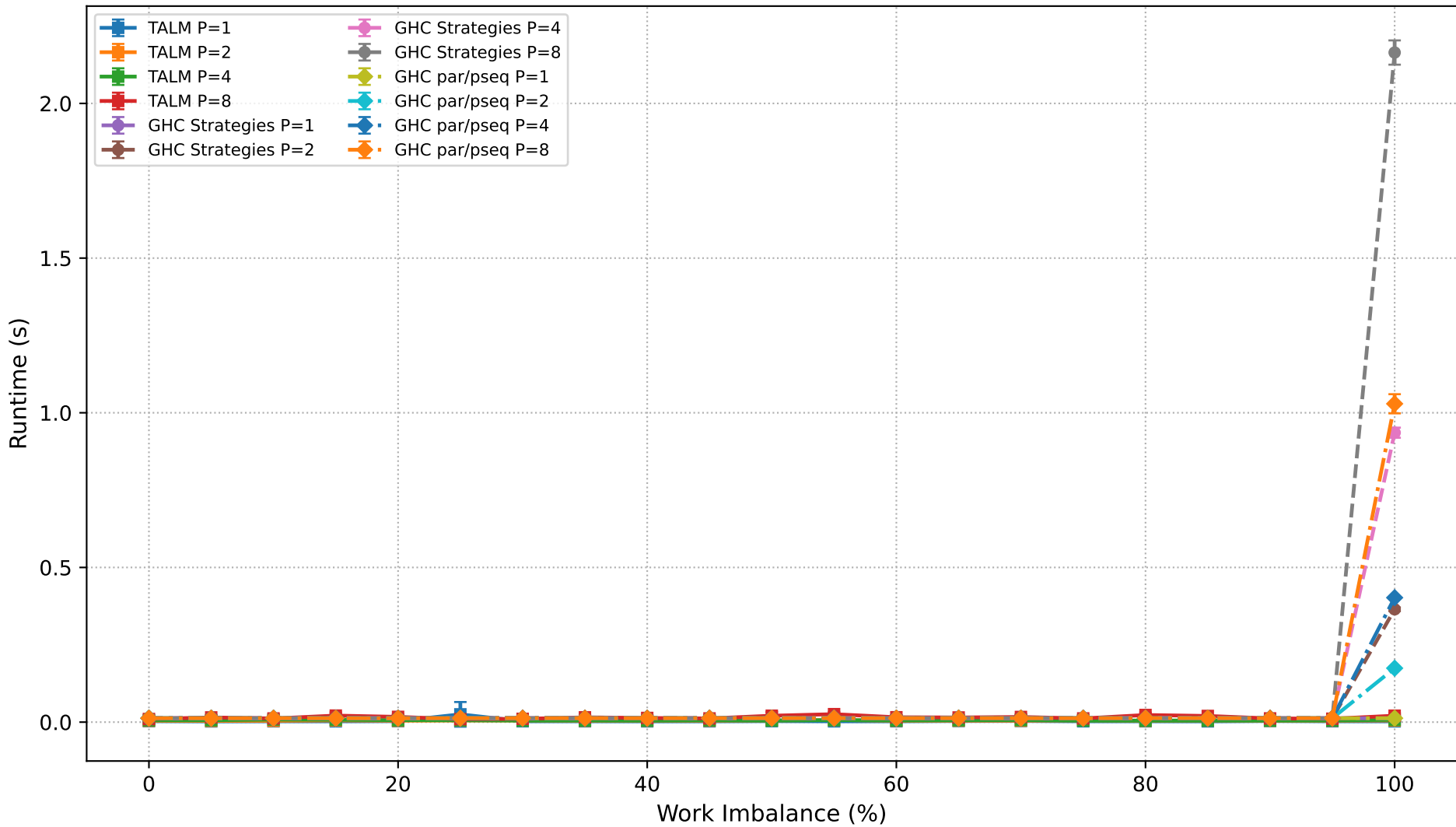
Dyck Path Validation: Runtime Comparison (N=700,000)
