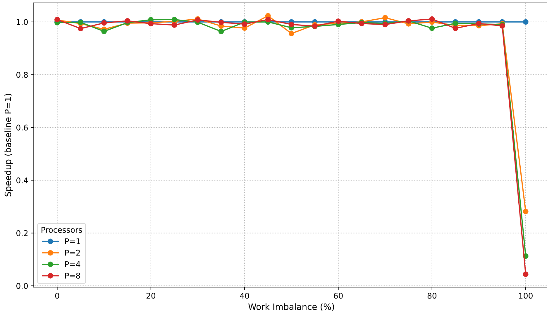
Dyck Path Validation: Speedup vs Work Imbalance (N=200,000)
