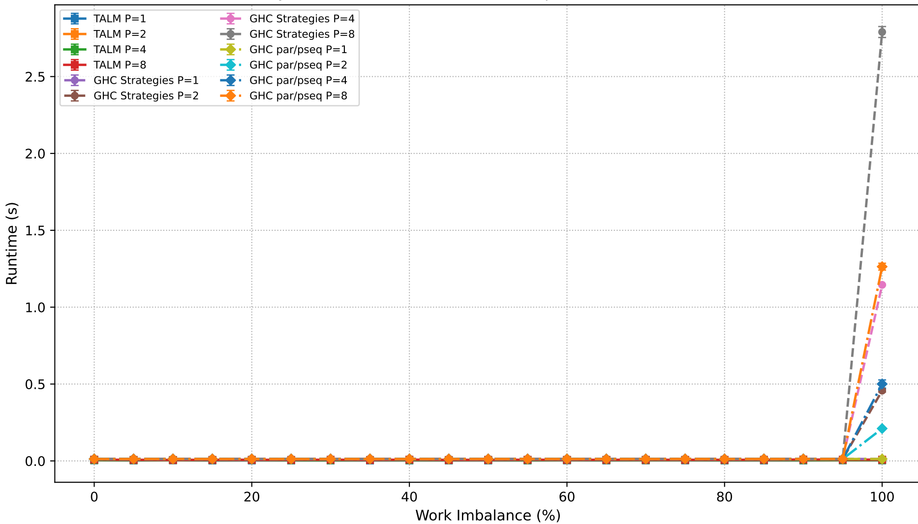
Dyck Path Validation: Runtime Comparison (N=850,000)
