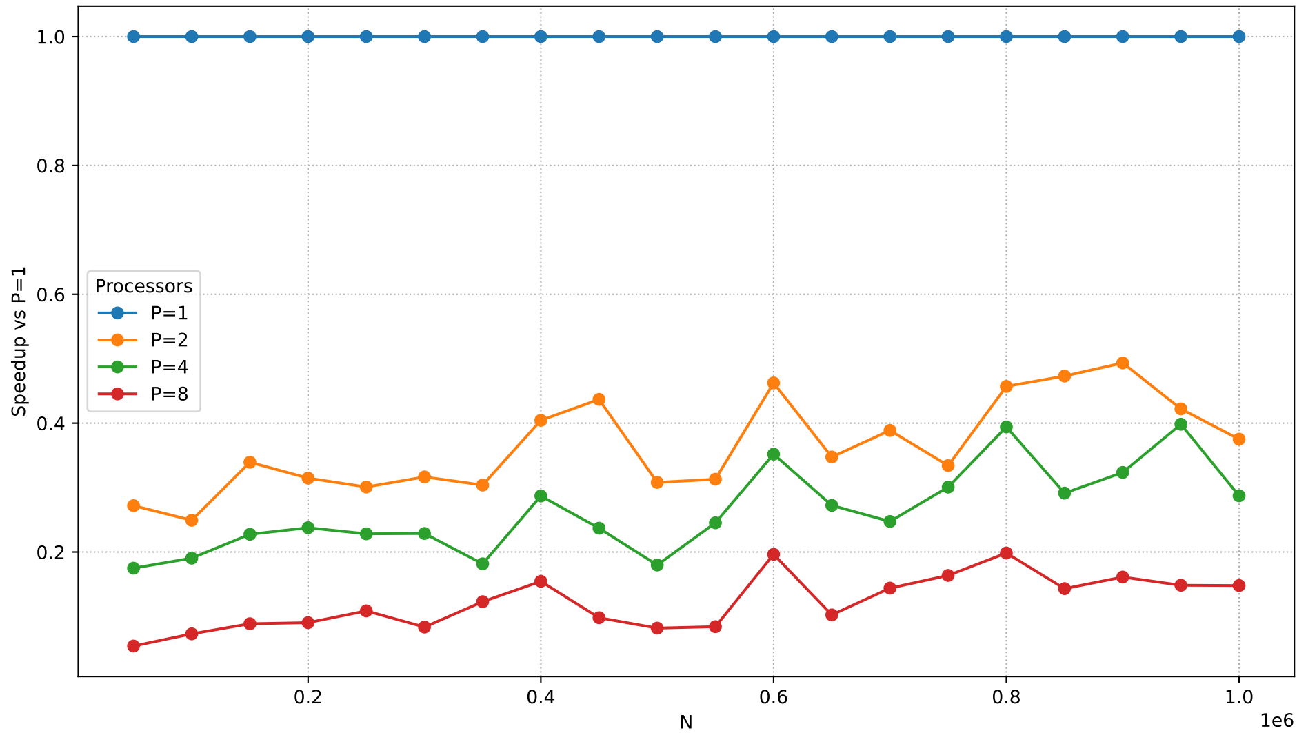
Speedup vs N (IMB=0)
