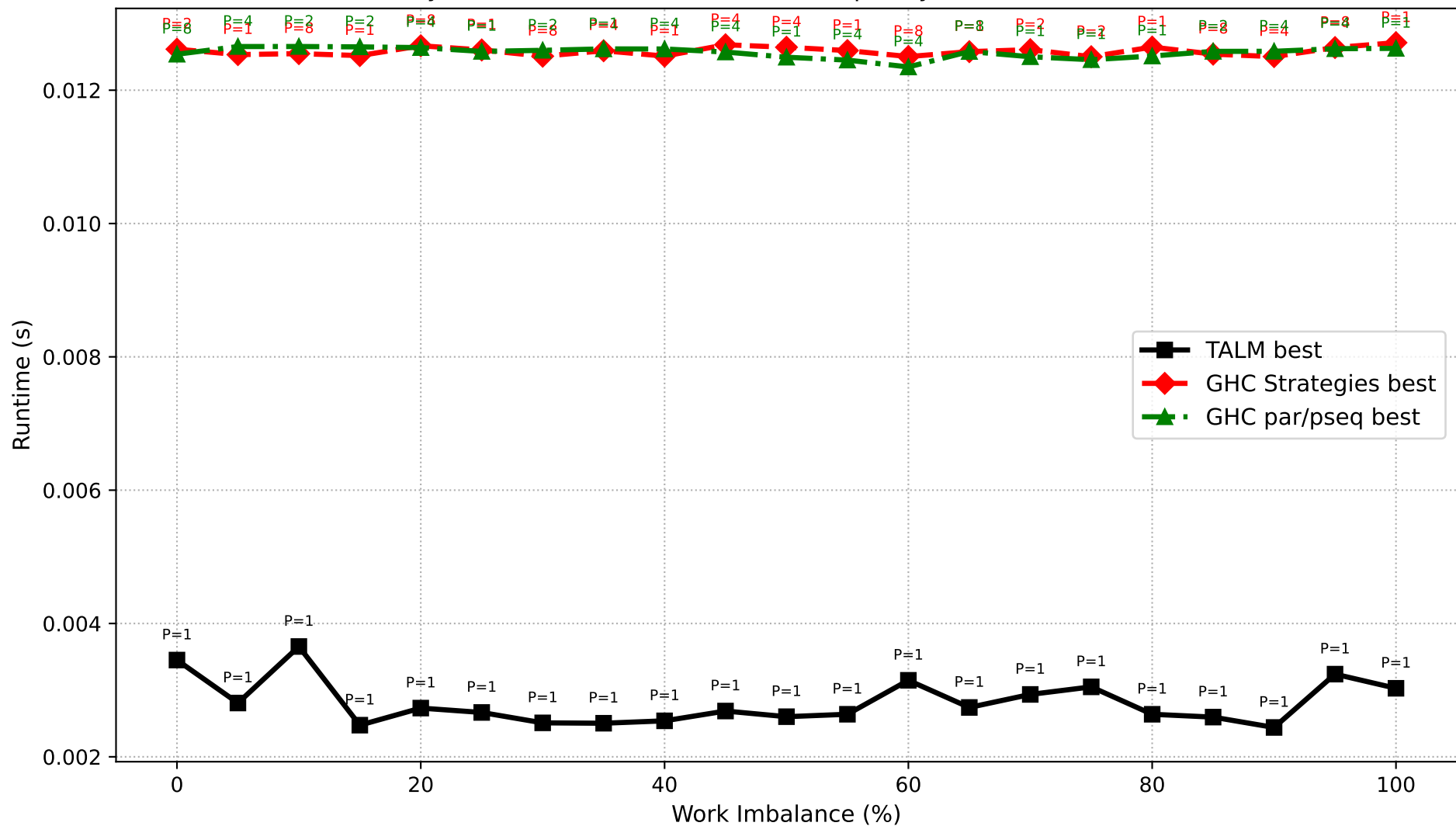
Dyck Path Validation: Best Runtime per System (N=850,000)
