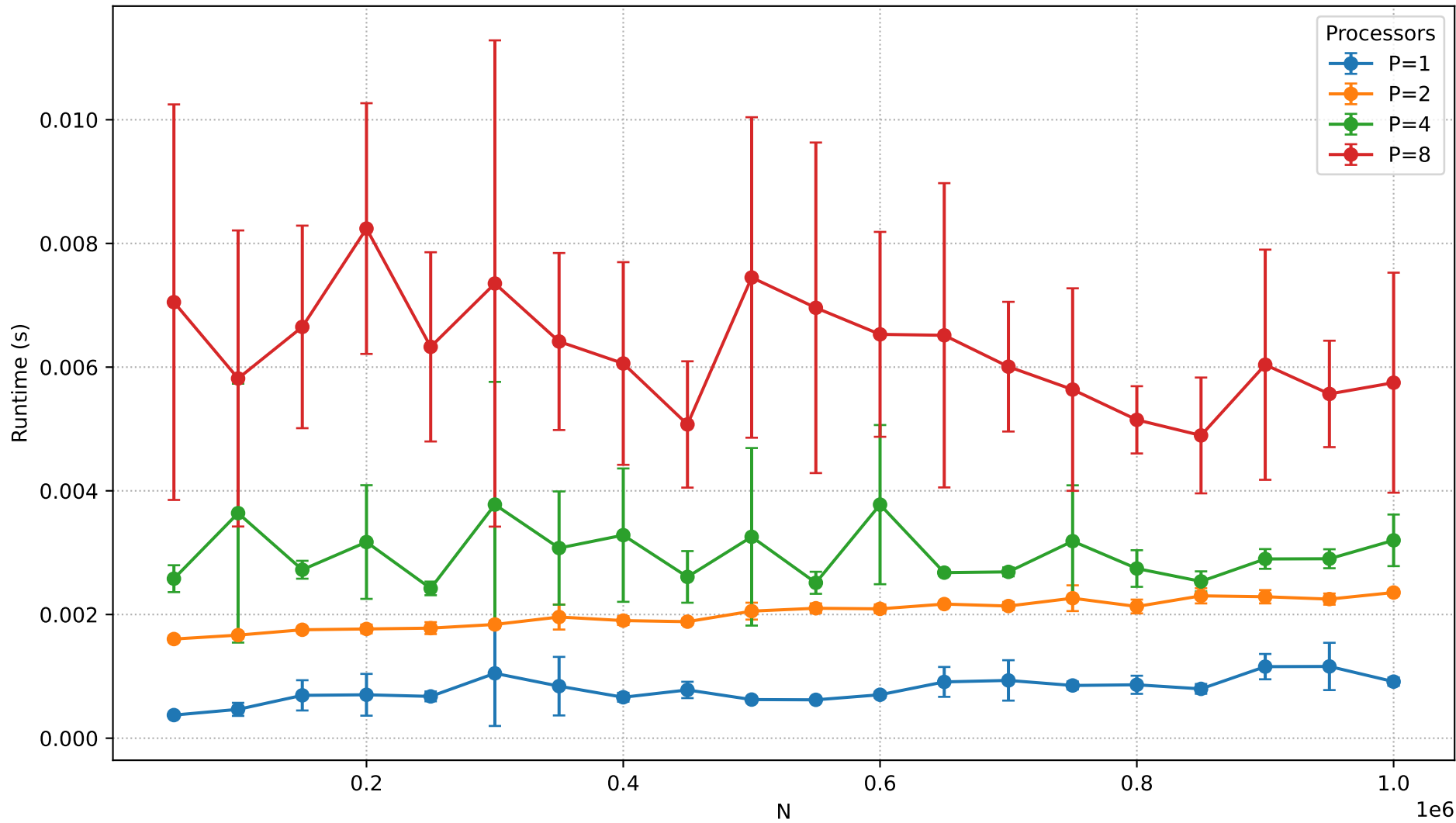
Runtime vs N (IMB=25)
