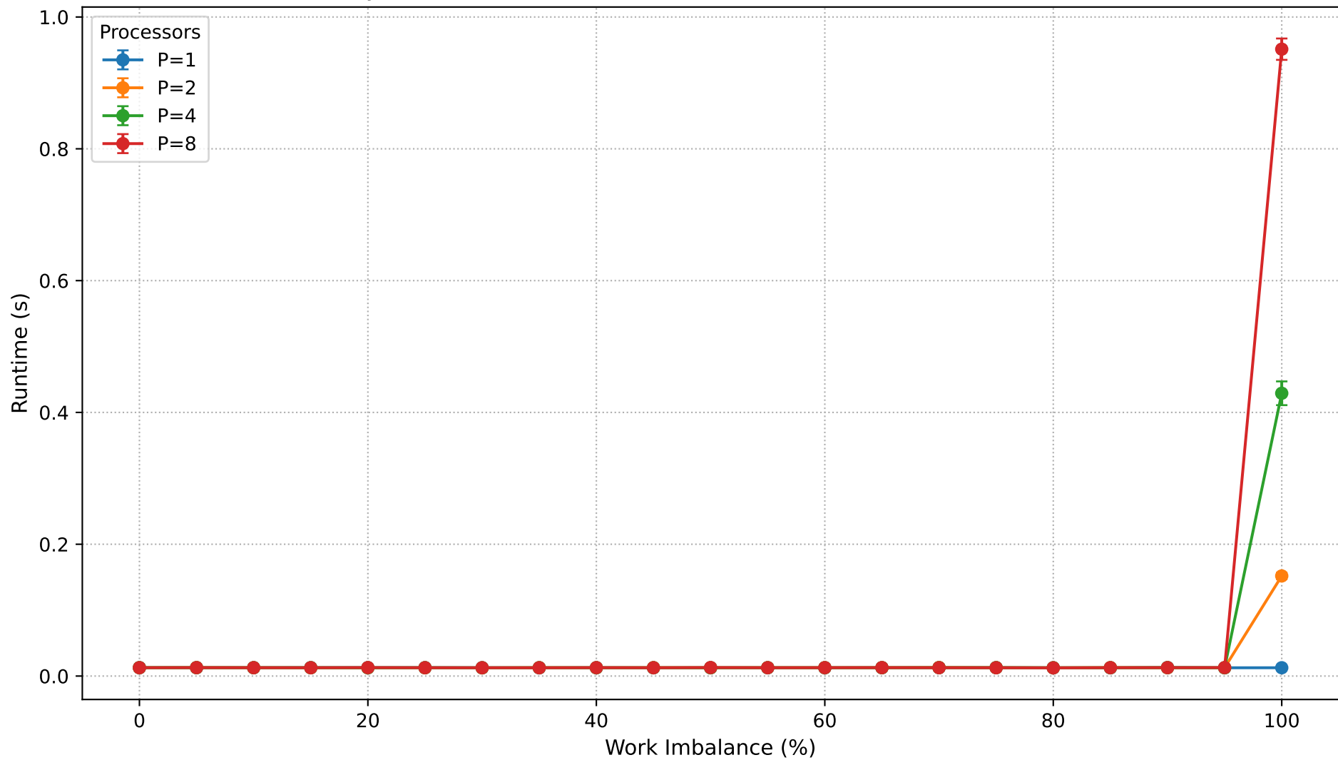
Dyck Path Validation: Runtime vs Work Imbalance (N=300,000)
