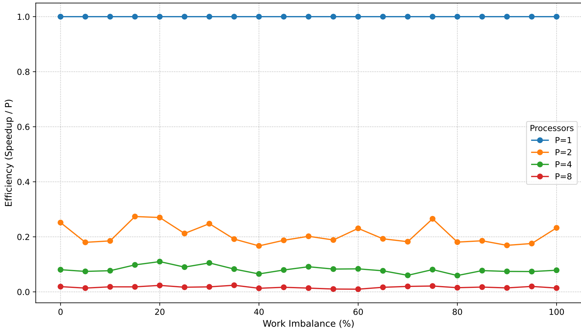
Dyck Path Validation: Parallel Efficiency vs Work Imbalance (N=250,000)
