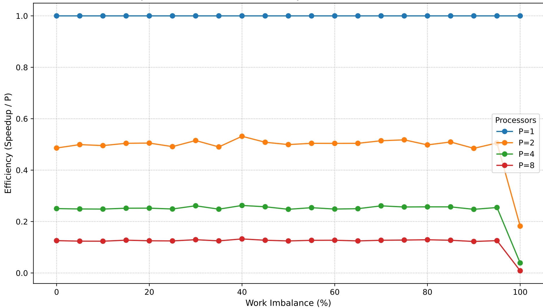
Dyck Path Validation: Parallel Efficiency vs Work Imbalance (N=150,000)
