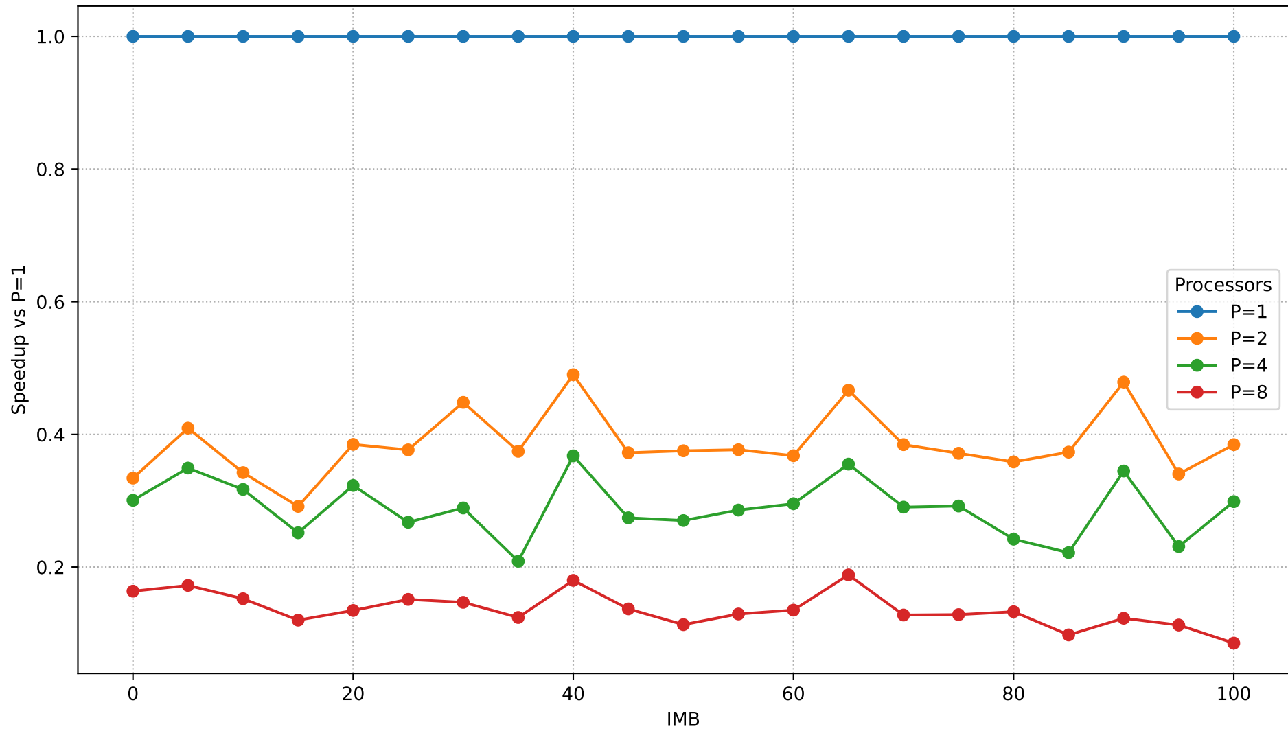
Speedup vs IMB (N=750,000)
