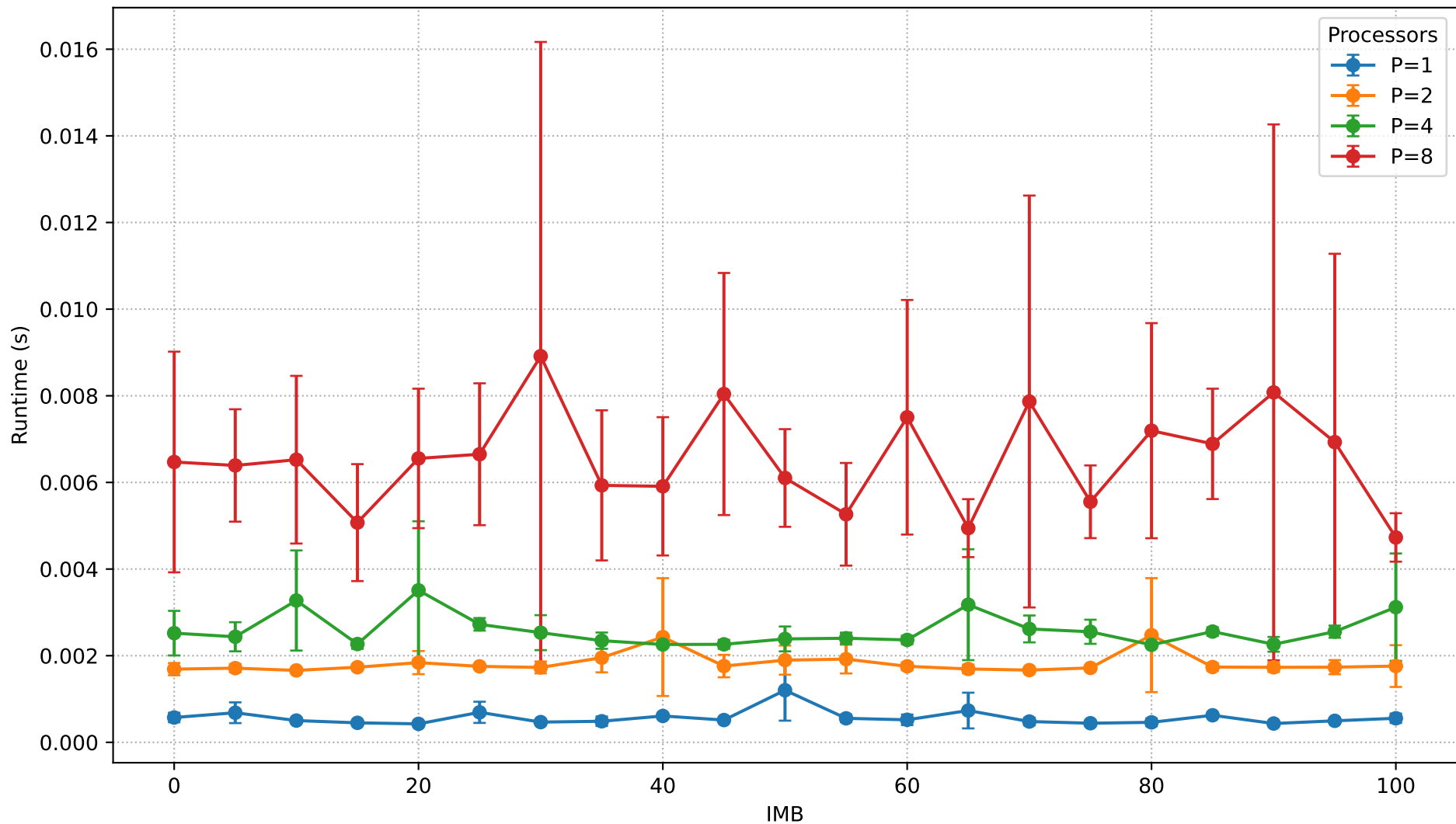
Runtime vs IMB (N=150,000)
