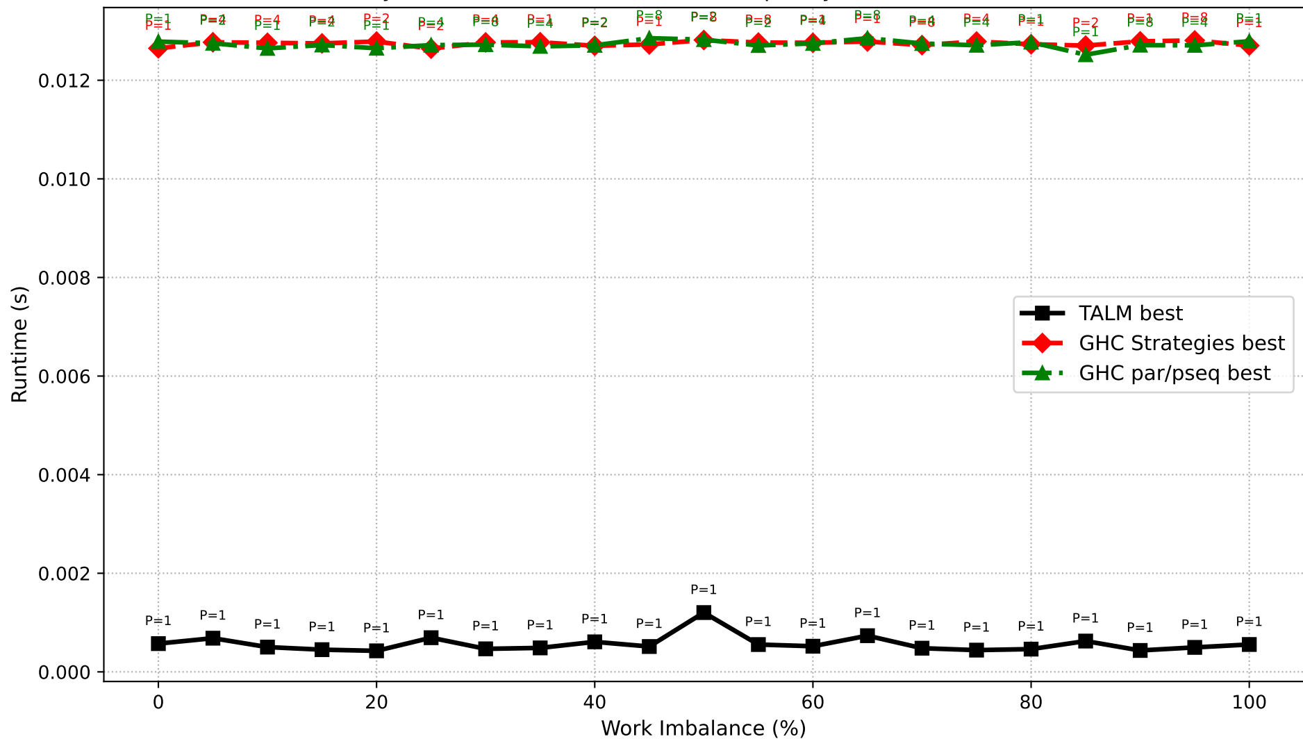
Dyck Path Validation: Best Runtime per System (N=150,000)
