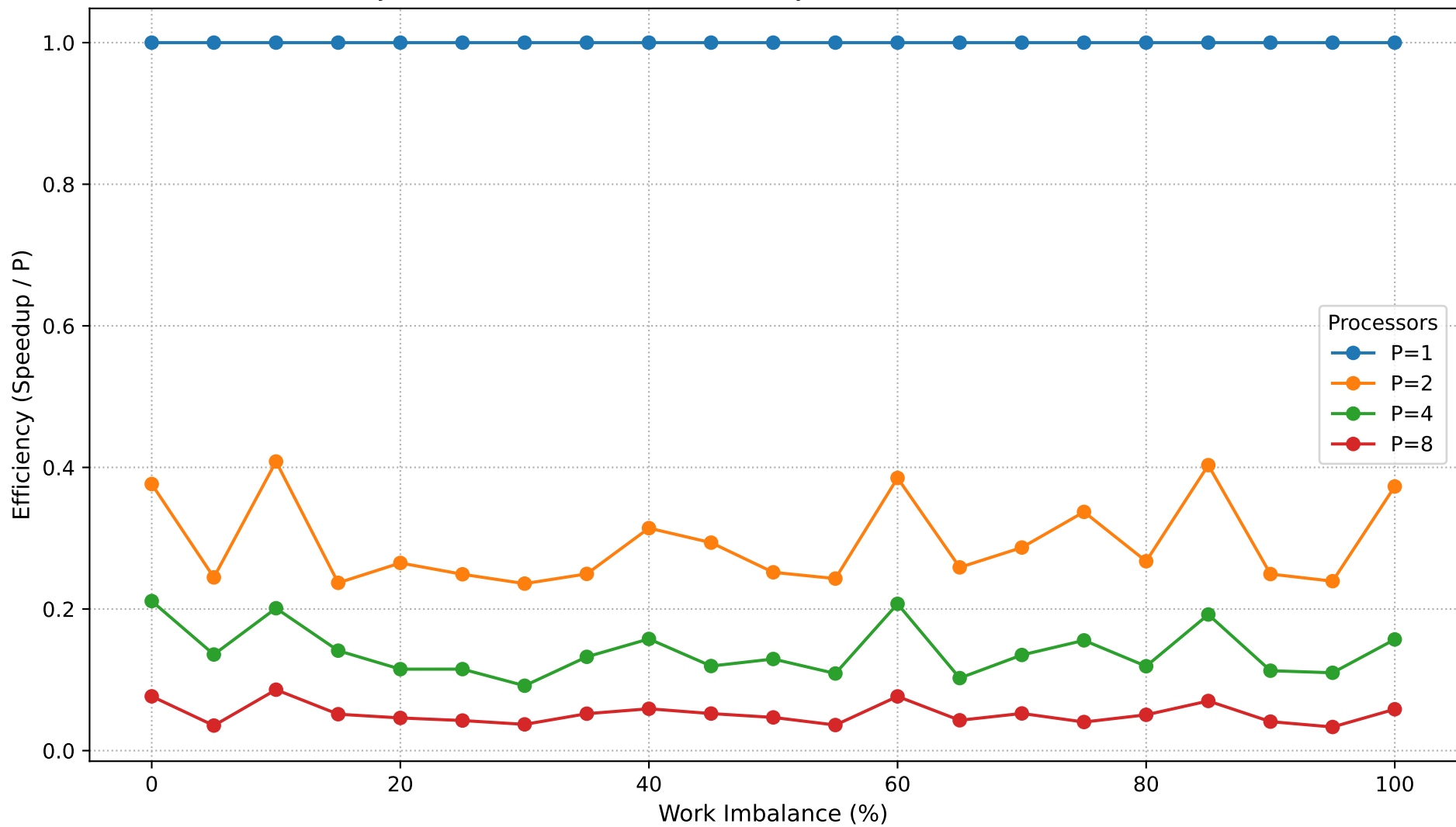
Dyck Path Validation: Parallel Efficiency vs Work Imbalance (N=800,000)
