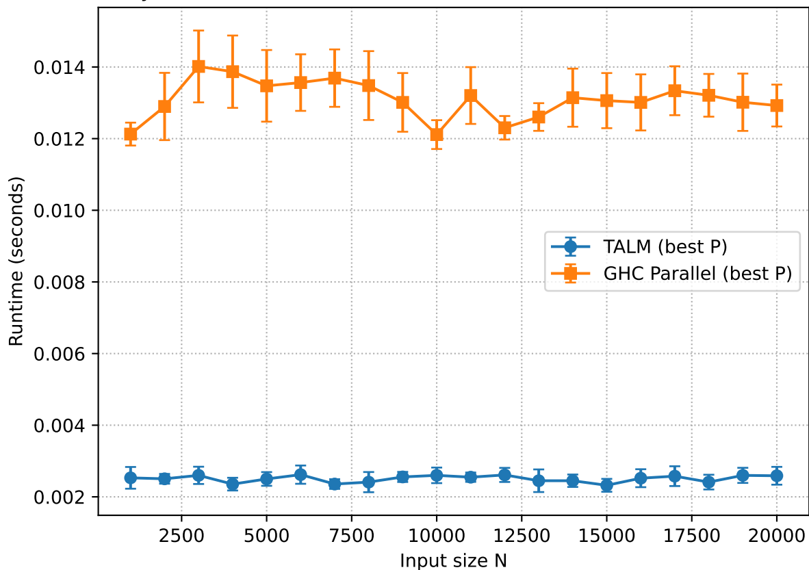
Dyck Path: Best-of-Breed Runtime vs N (imb=100, delta=0)
